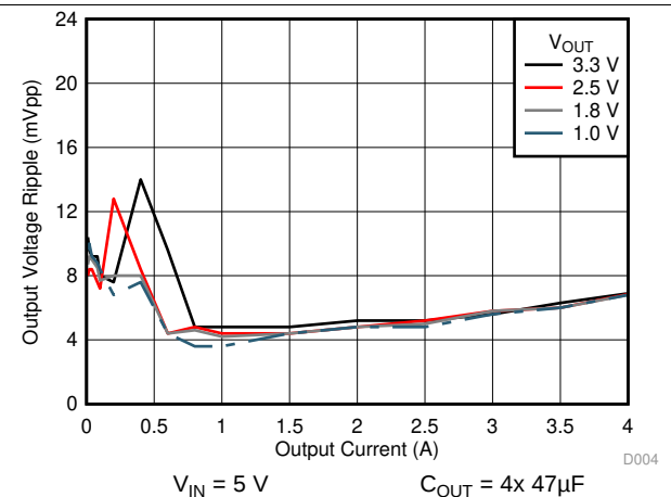
Figure 4. Voltage Ripple versus Output Current
