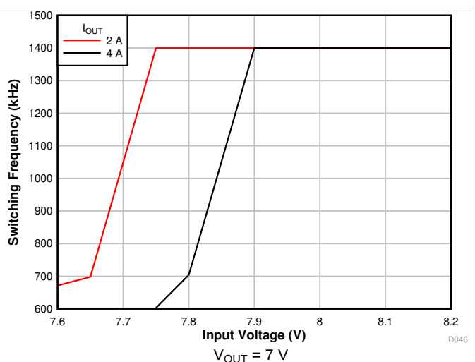
Figure 36. Frequency Foldback
