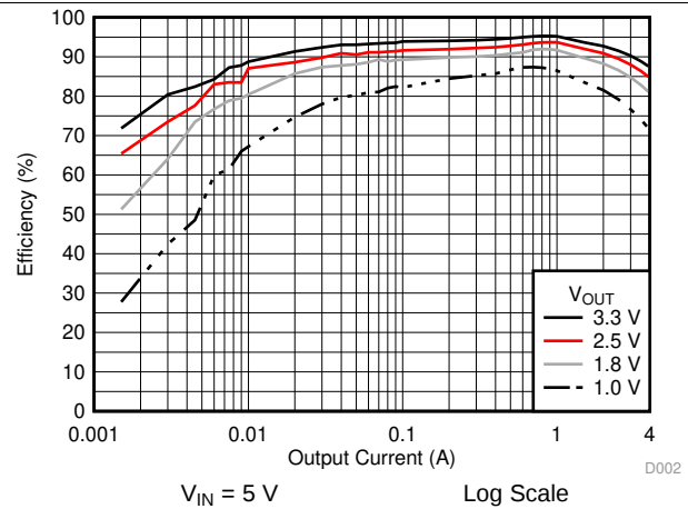
Figure 2. Efficiency versus Output Current
