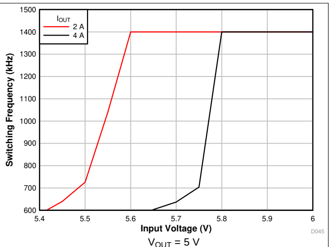
Figure 34. Frequency Foldback
