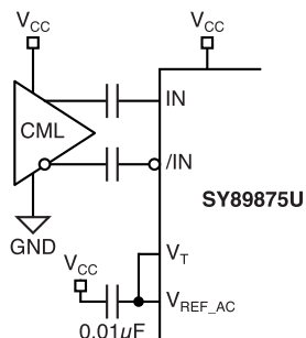
Figure 4b. AC-Coupled CML Input Interface
