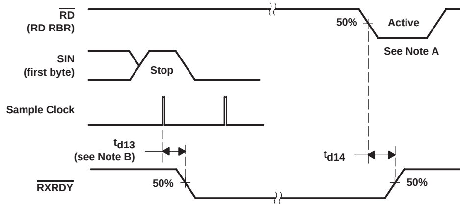
Figure 11. Receiver Ready ( \text{RXRDY} ) Waveforms, \text{FCR0} = 0 or \text{FCR0} = 1 and \text{FCR3} = 0 (Mode 0)
