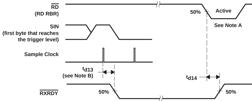
Figure 12. Receiver Ready ( \text{RXRDY} ) Waveforms, \text{FCR0} = 1 and \text{FCR3} = 1 (Mode 1)
