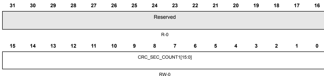
Figure 22-19. CRC Sector Counter Preload Register1(CRC_SCOUNT_REG1) [offset = 0x44]
