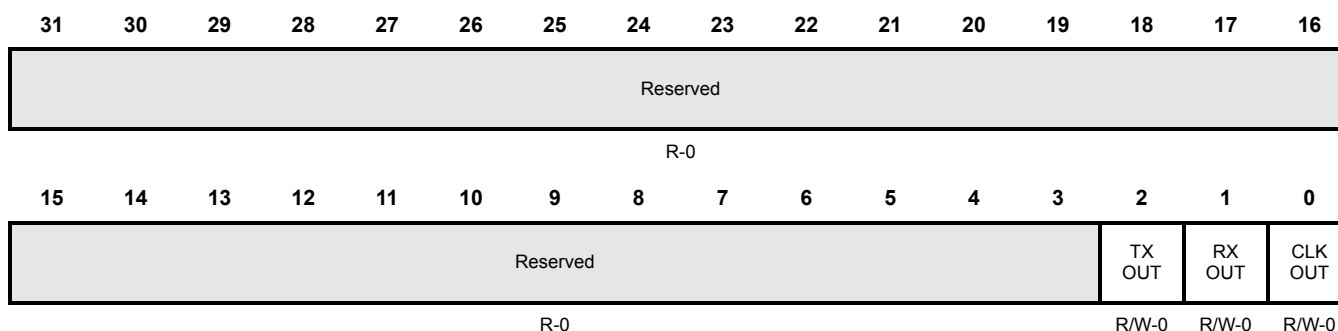
Figure 13-46. SCI Pin I/O Control Register 3 (SCIPIO3) [offset =0x48]
