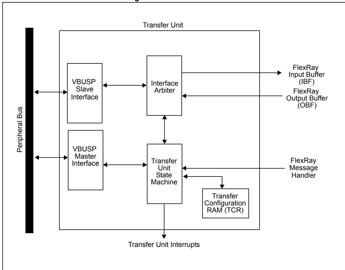
Figure 17-3. Transfer Unit
