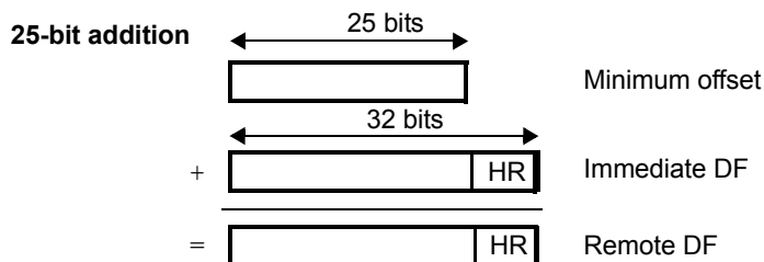
Figure 18-78. ADCNST Operation if Remote Data Field [31:7] Is Zero
