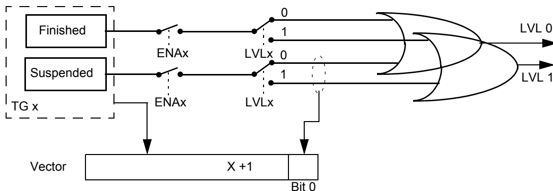
Figure 14-24. TG Interrupt Structure
