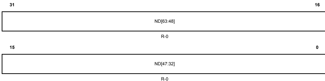
Figure 17-165. New Data Register 2 (NDAT2) [offset_CC = 0x334]
