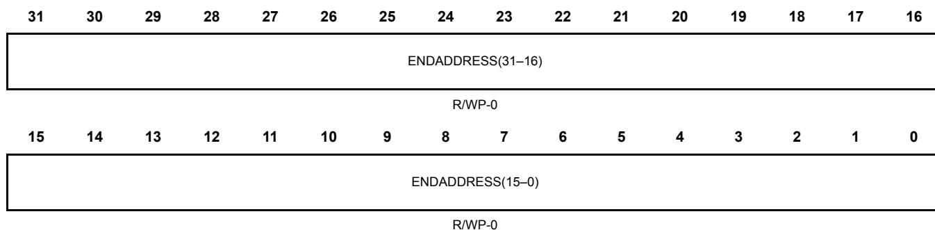
Figure 20-78. DMA Memory Protection Region 0 End Address Register (DMAMPR0E) [offset = 0x1BC]
