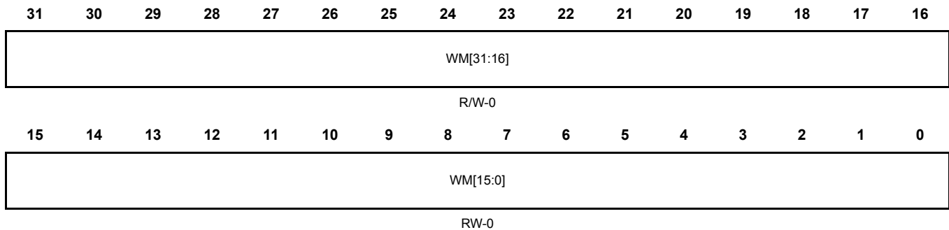
Figure 20-69. Watch Mask Register (WMR) [offset = 0x188]
