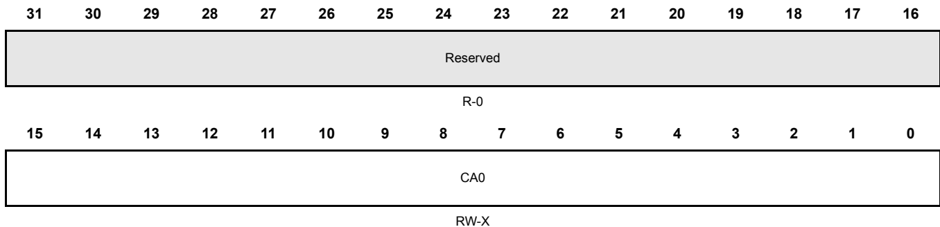
Figure 6-7. Constant Address Register (CA0, CA1, CA2, CA3) [offset = 0x0130 - 0x013C]
