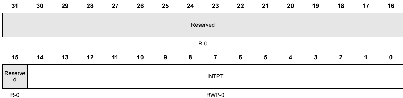
Figure 26-18. DMM Direct Data Mode Interrupt Pointer Register (DMMINTPT) [offset = 28h]
