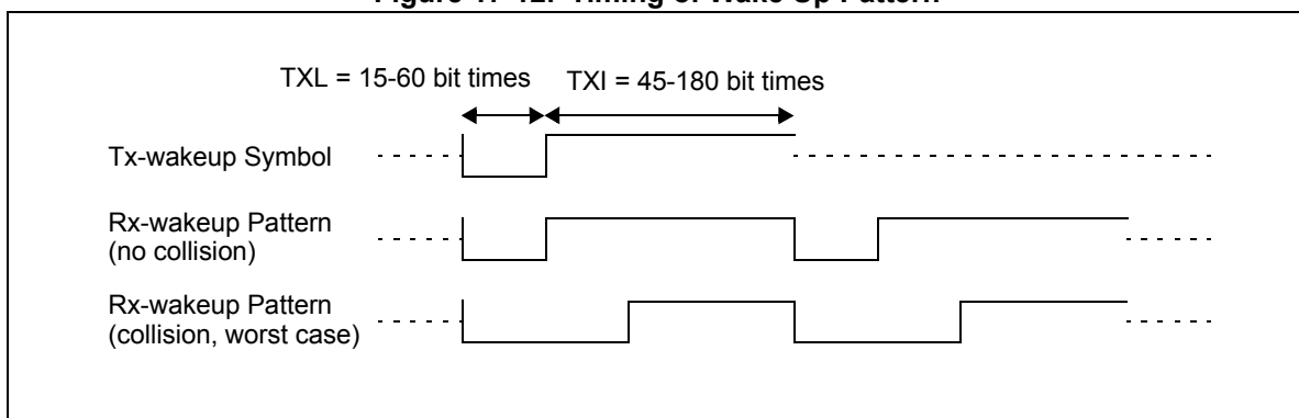
Figure 17-12. Timing of Wake Up Pattern
