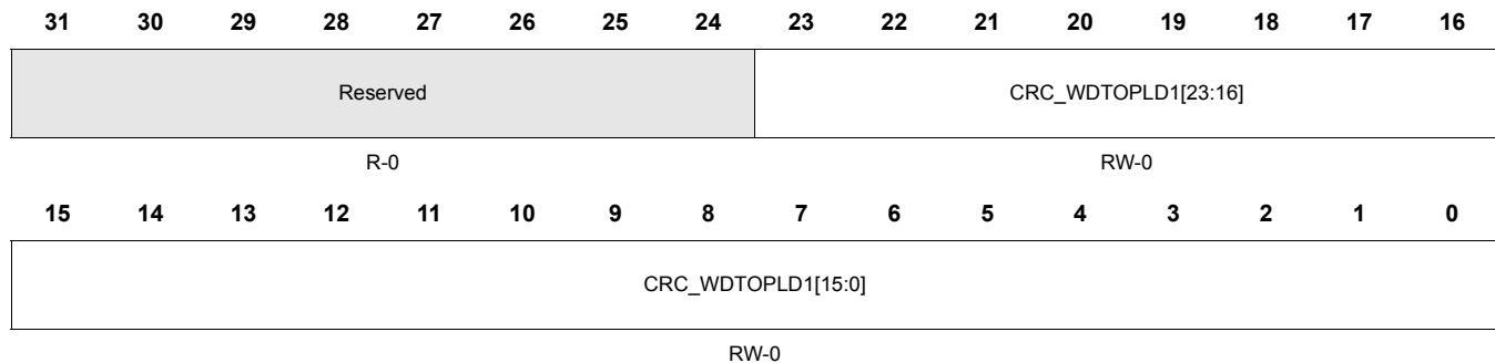
Figure 22-21. CRC Channel 1 Watchdog Timeout Preload Register A(CRC_WDTPLD1) [offset = 0x4C]
