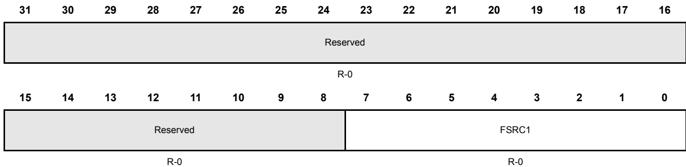
Figure 6-22. Fail Status Count Register 1 (FSRC1) [offset = 0x019C]
