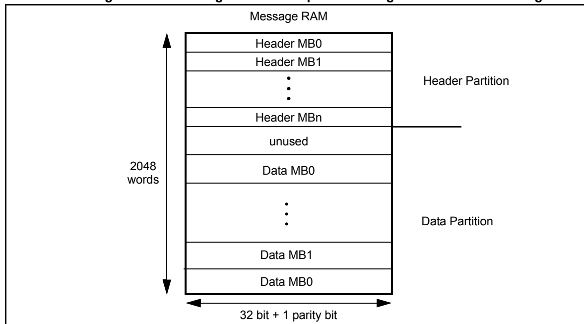
Figure 17-21. Configuration Example of Message Buffers in the Message RAM
