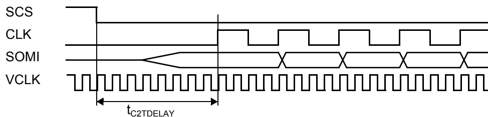
Figure 14-20. Example: t_{C2TDELAY} = 8 VCLK Cycles
