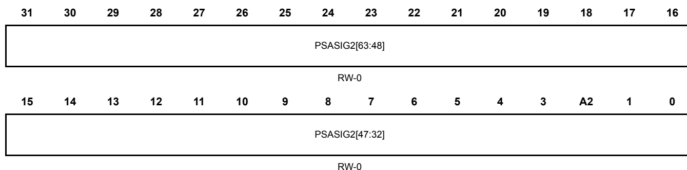
Figure 22-37. Channel 2 PSA signature high register(PSA_SIGREGH2) [offset = 0xA4]
