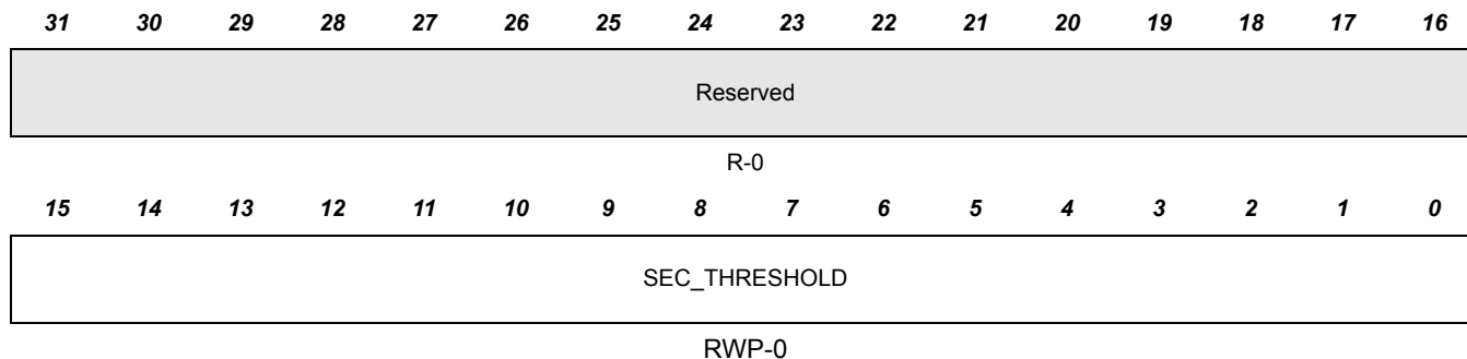
Figure 8-10. Flash Error Correction and Correction Control Register 2 (FEDACCTRL2 - 0xFFFF8700C)
