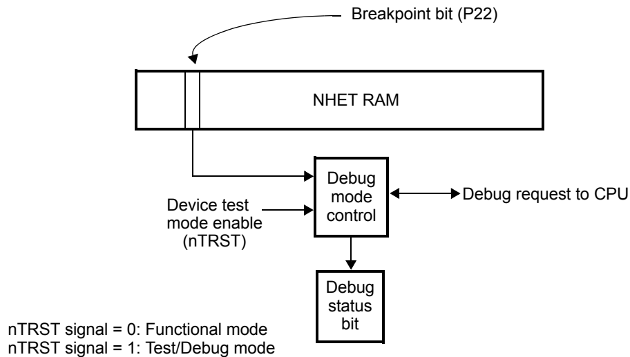
Figure 18-6. Debug Control Configuration
