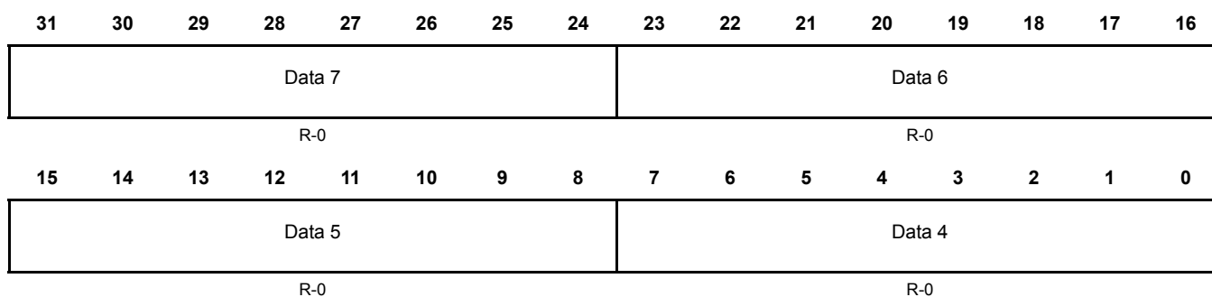
Figure 16-59. IF3 Data A Register (DCAN IF3DATB) [offset = 0x154]
