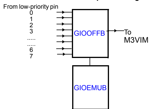
Figure 12-10. Low-Level-Interrupt-Handling Block
