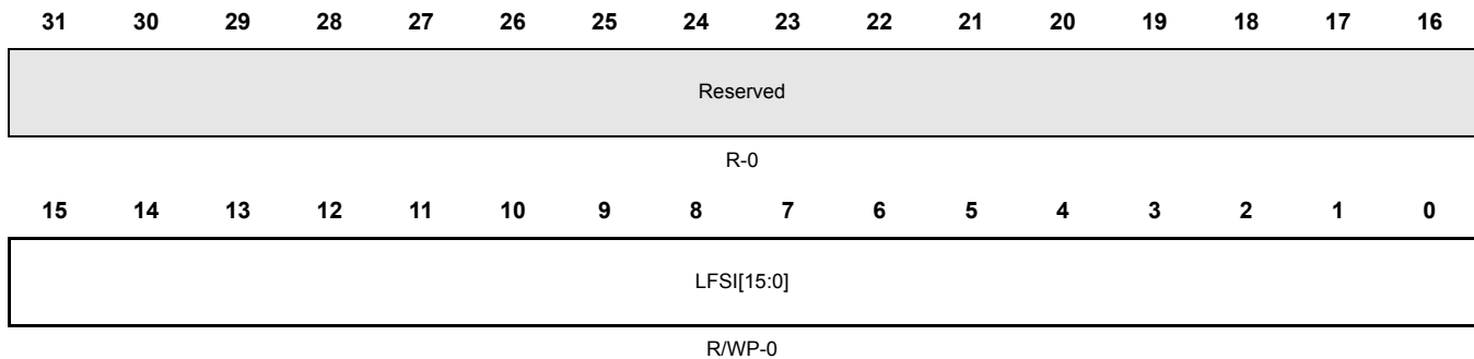
Figure 20-51. LFS Interrupt Flag Register (LFSFLAG) [offset = 0x12C]
