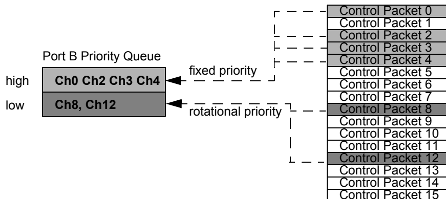
Figure 20-11. Example Channel Assignments
