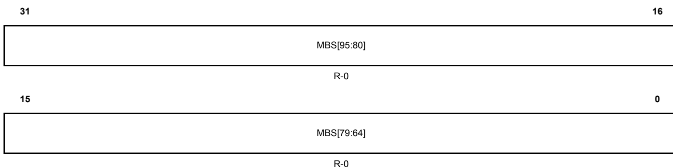
Figure 17-168. Message Buffer Status Changed Register 3 (MBSC3) [offset_CC = 0x348]
