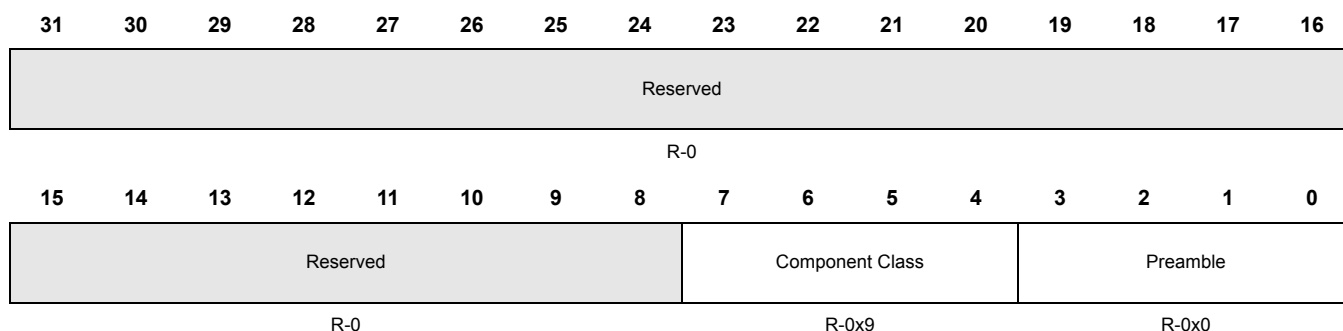
Figure 11-26. POM Component ID 1 Register (POMCPOMPONENTID1) [offset = 0xFF4]
