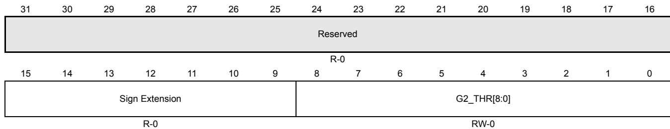
Figure 15-41. ADC Group2 Threshold Interrupt Control Register (ADG2THRINTCR) [offset = 0x48]
