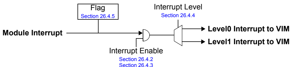
Figure 26-6. Interrupt Structure
