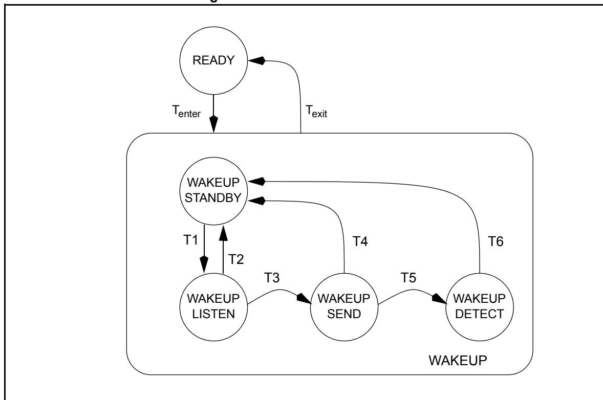
Figure 17-11. Structure of POC State WAKEUP
