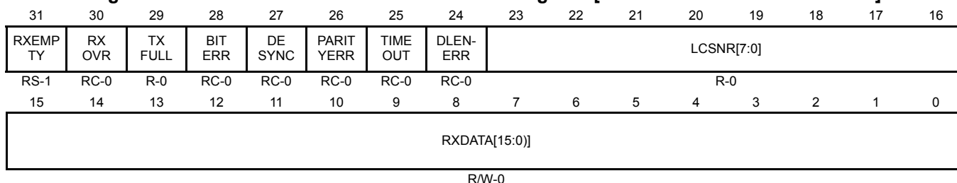
Figure 14-50. Multi-buffer RAM Receive Buffer Register [offset = RAM Base + 200–3FFh]
