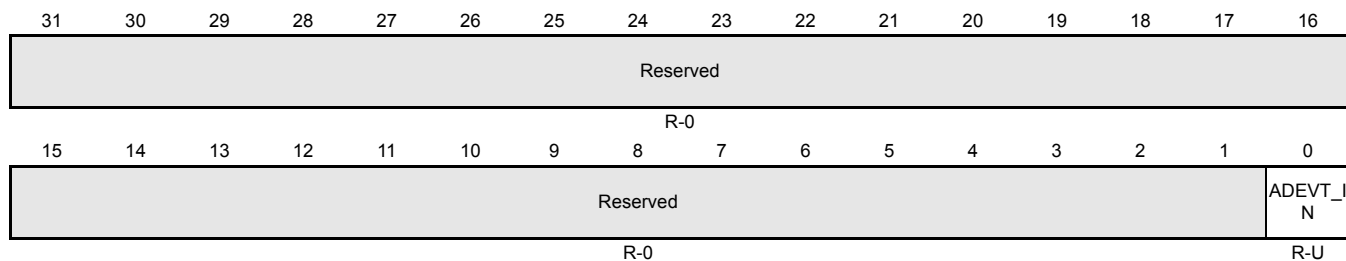
Figure 15-63. ADC ADEVT Pin Input Value Register (ADEVTIN) [offset = 0x104]
