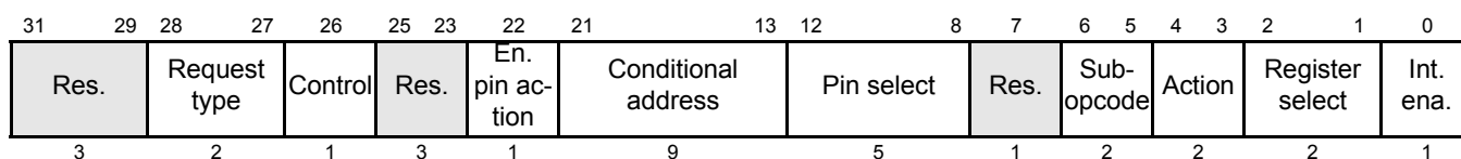
Figure 18-104. ECMP Data Field (D31:D0)
