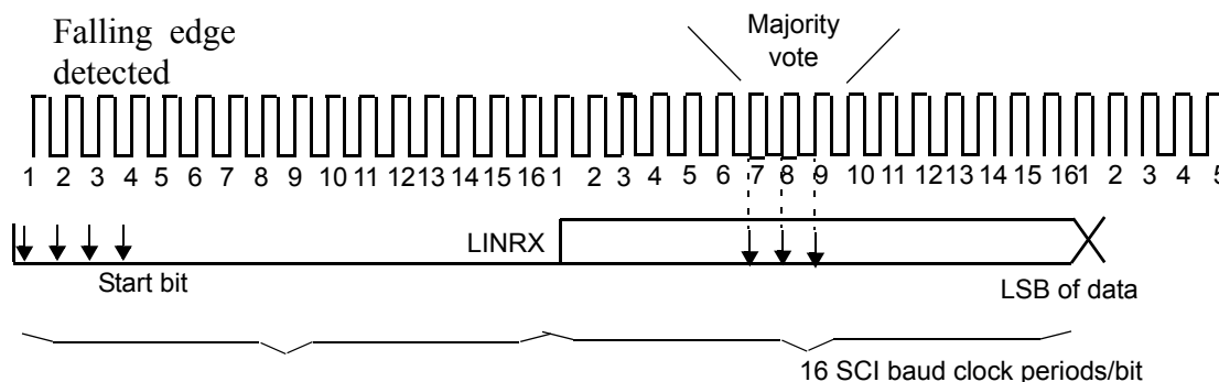
Figure 13-4. Asynchronous Communication Bit Timing
