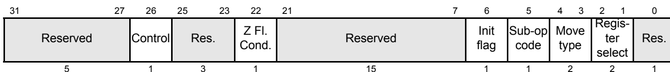
Figure 18-113. MOV32 Data Field (D31:D0)
