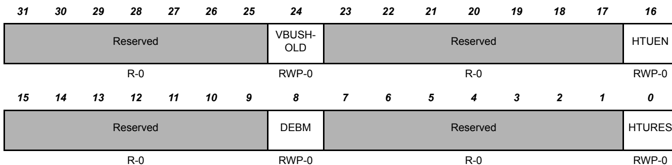
Figure 19-16. Global Control Register (HTU GC) [offset = 0x00]
