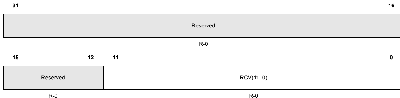
Figure 17-142. Rate Correction Value Register (RCV) [offset_CC = 0x118]
