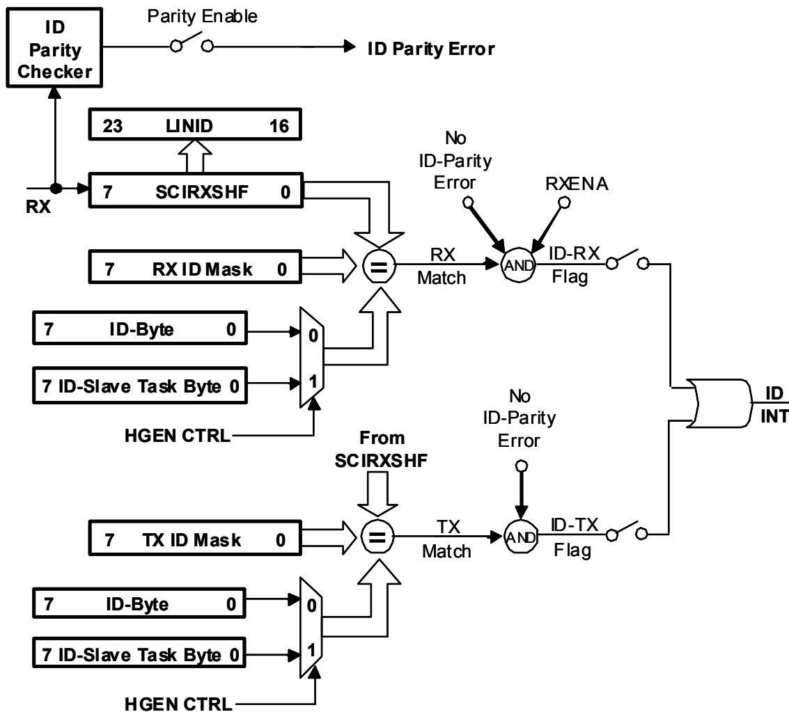
Figure 13-24. ID Reception, Filtering and Validation
