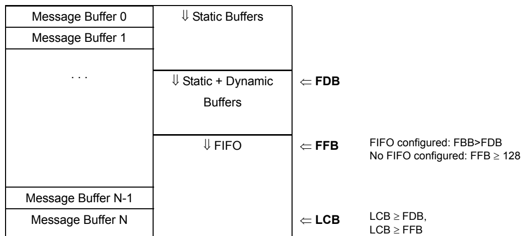
Figure 17-151. Buffer Configuration
