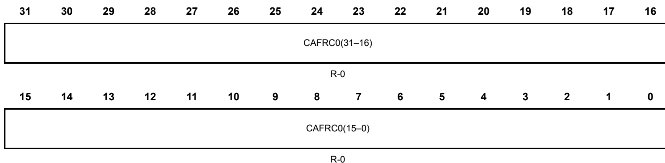
Figure 21-16. RTI Capture Free Running Counter 0 Register (RTICAFRC0) [offset = 0x20h]
