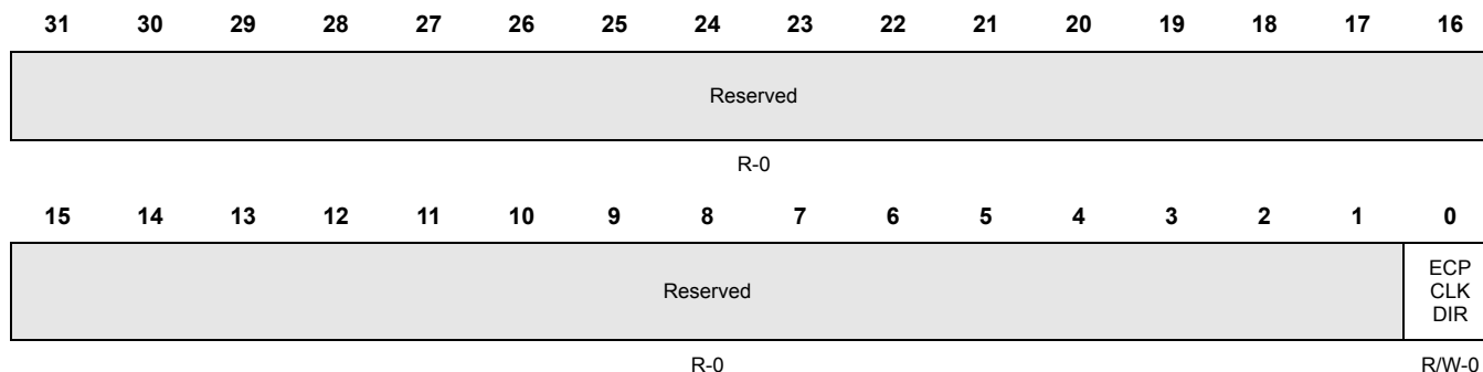
Figure 5-3. SYS Pin Control Register 2 (SYSPC2) [offset = 0x04]
