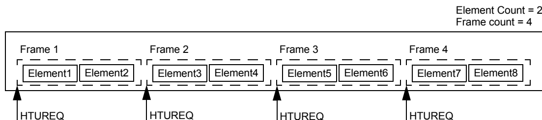
Figure 19-3. Example of a HTU Transfer
