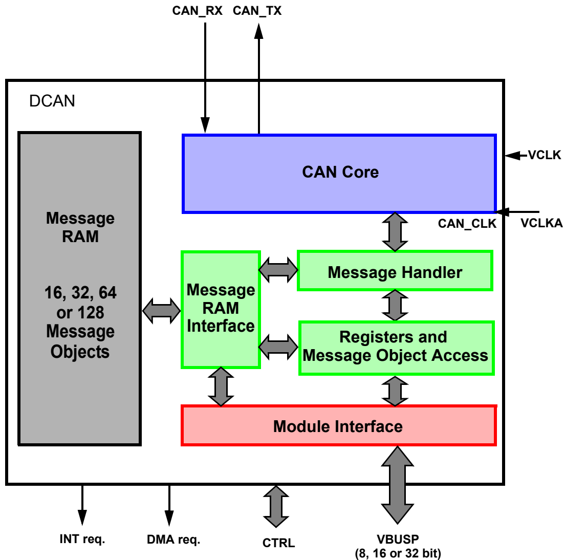
Figure 16-1. Block Diagram
