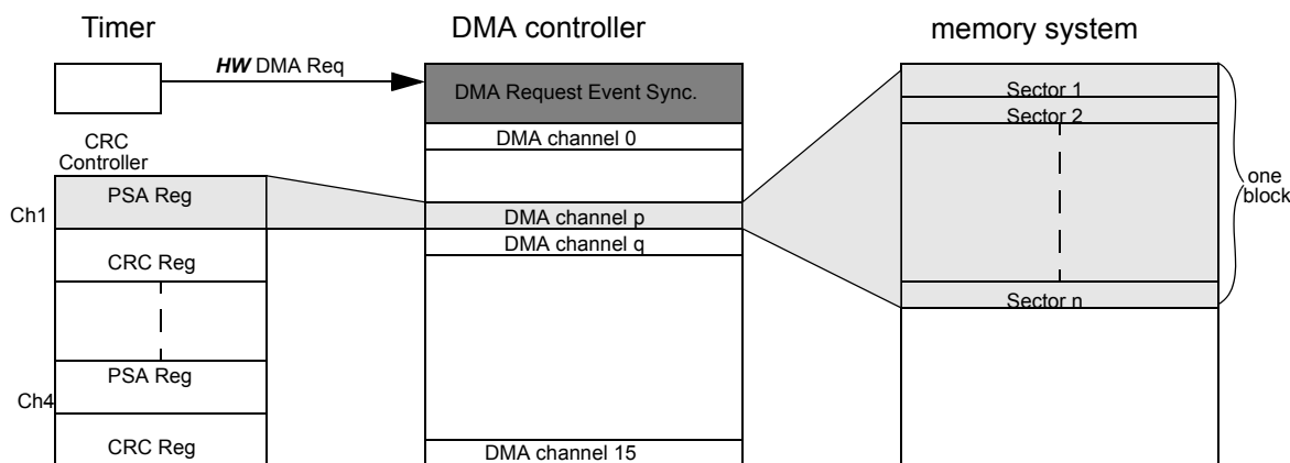
Figure 22-5. Semi-CPU Mode With Hardware Timer Trigger
