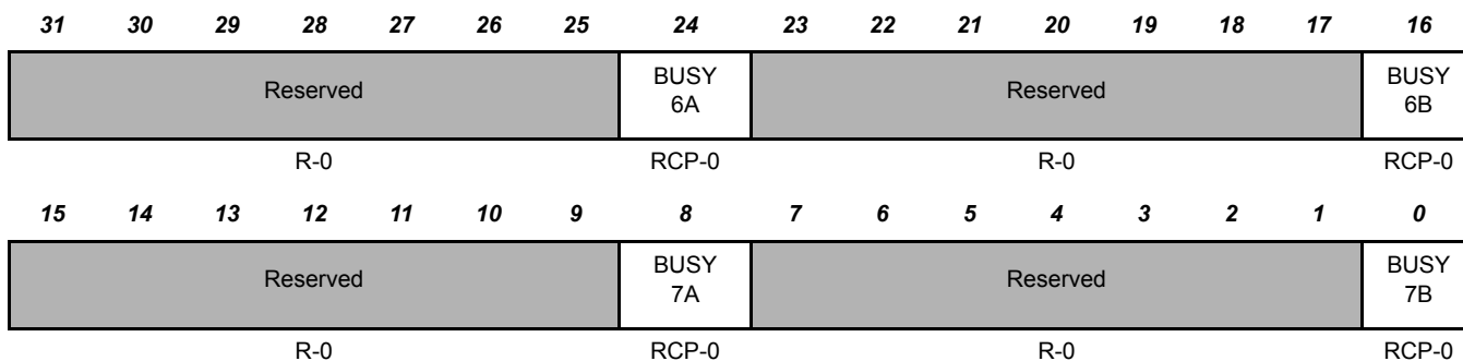
Figure 19-21. Control Packet (CP) Busy Register 3 (HTU BUSY3) [offset = 0x14]
