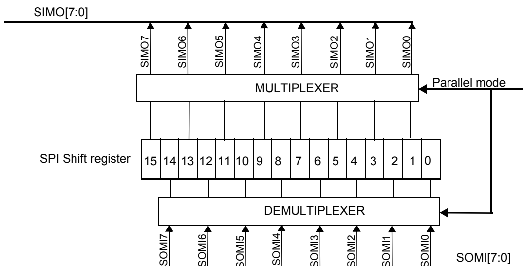
Figure 14-14. Block Diagram Shift Register, MSB First
