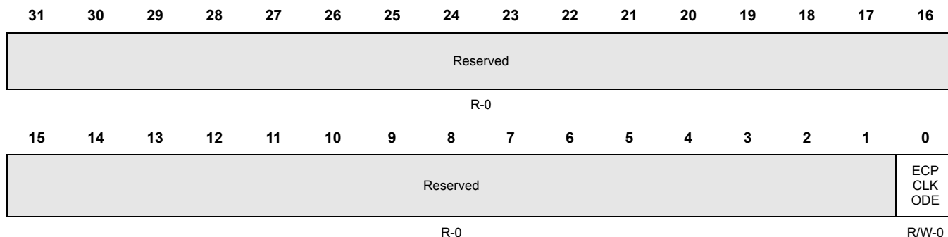
Figure 5-8. SYS Pin Control Register 7 (SYSPC7) [offset = 0x18]
