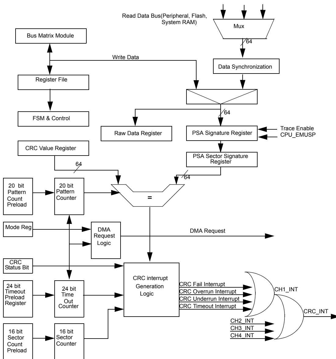
Figure 22-1. MCRC Controller Block Diagram For One Channel
