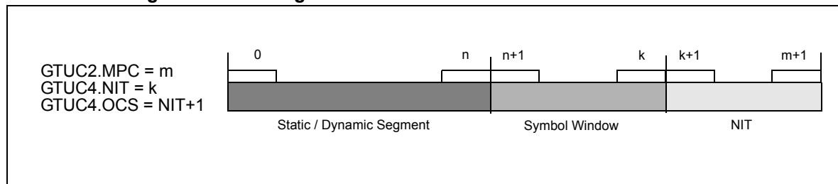
Figure 17-9. Configuration of NIT Start and Offset Correction Start
