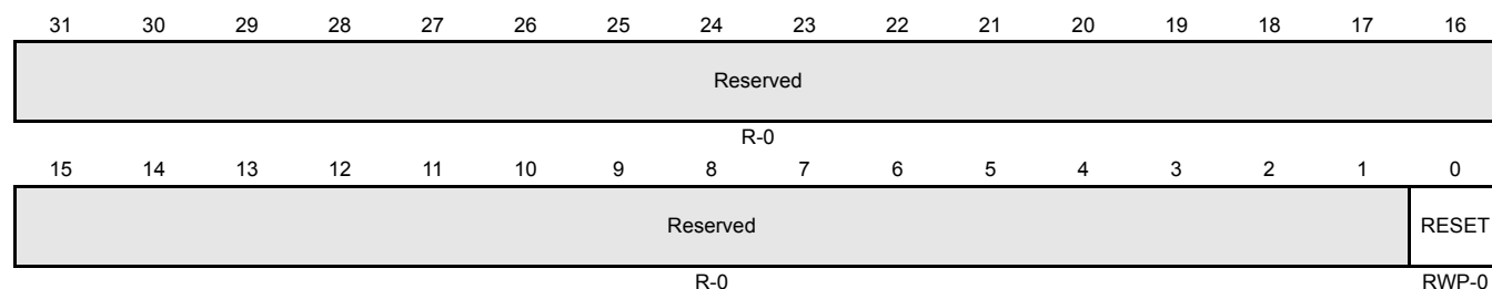
Figure 15-23. ADC Reset Control Register (ADRSTCR) [offset = 0x0]
