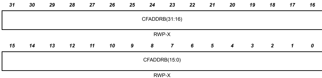
Figure 19-51. Current Full Address B Register (HTU CFADDRB)
