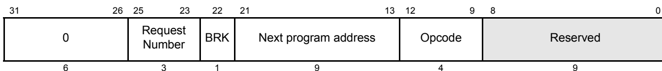
Figure 18-90. BR Control Field (C31:C0)
