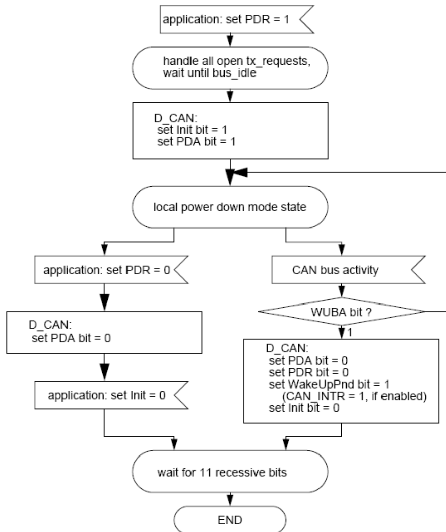
Figure 16-10. Local power down mode flow diagram
