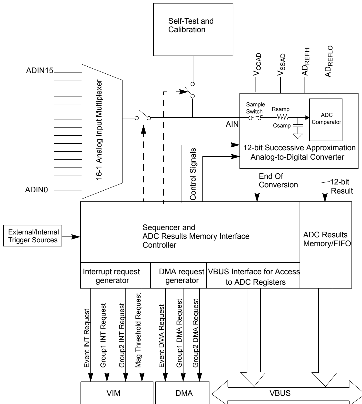
Figure 15-2. ADC Block Diagram
