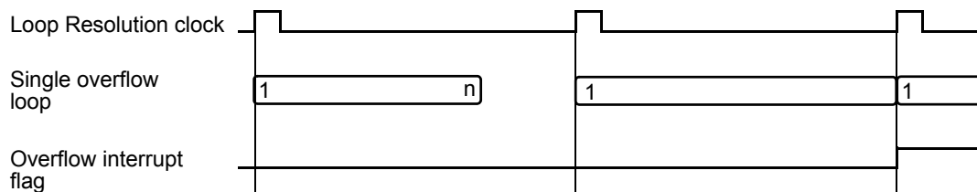
Figure 18-4. Use of the Overflow Interrupt Flag
