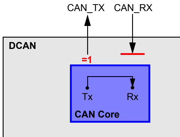
Figure 16-7. CAN Core in Loop Back combined with Silent Mode
