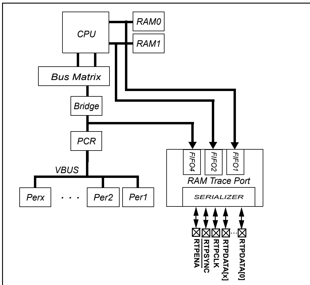
Figure 27-1. Block diagram RAM Trace Port Module
