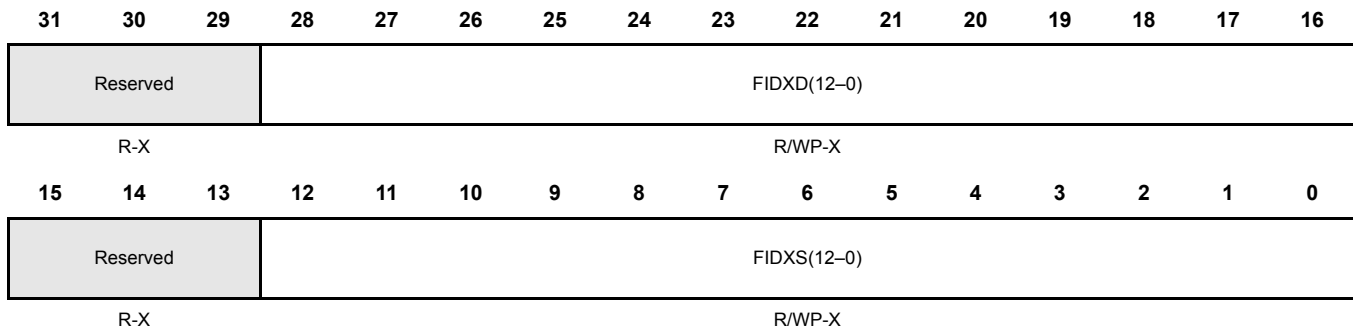
Figure 20-90. Frame Index Offset Register (FIOFF) [offset = 0x018]
