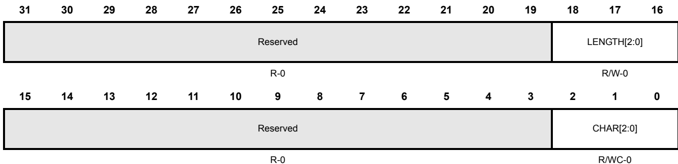
Figure 13-38. SCI Format Control Register (SCIFORMAT) [offset = 0x28]
