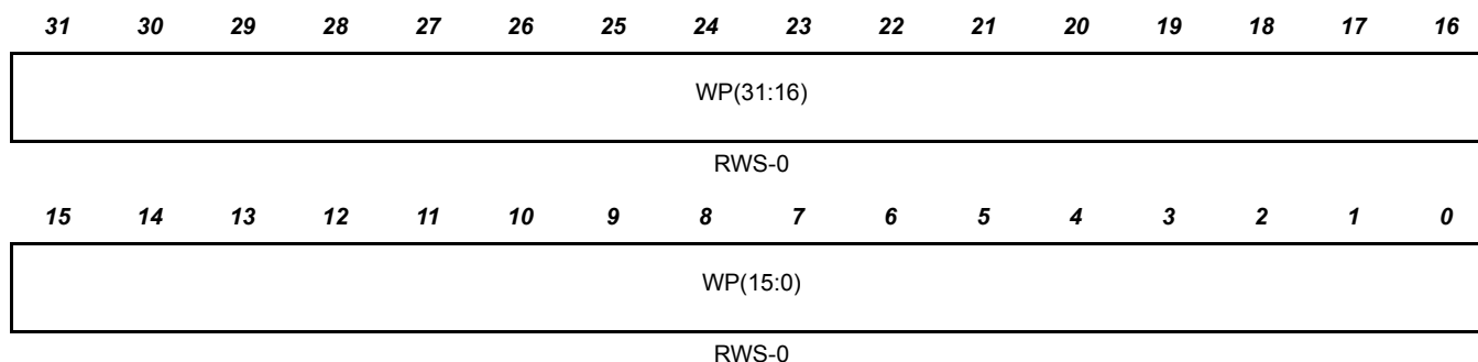
Figure 19-36. Watch Point Register (HTU WPR) [offset = 0x58]
