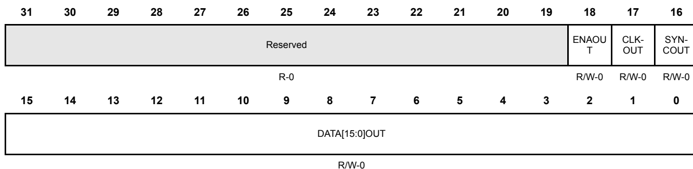
Figure 27-19. RTP Pin Control 3 Register (RTPPC3) [offset = 40h]
