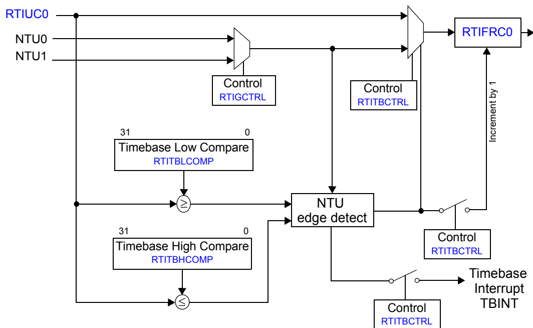
Figure 21-4. Timebase Control
