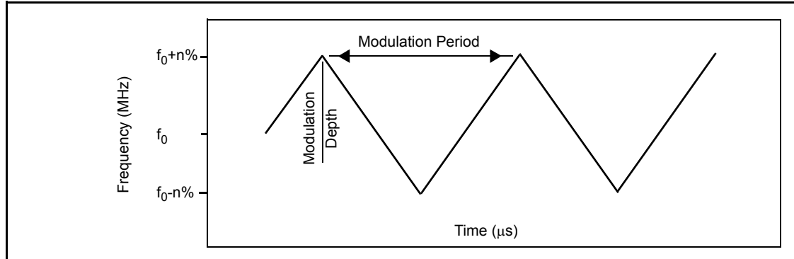
Figure 7-5. Frequency vs. Time
