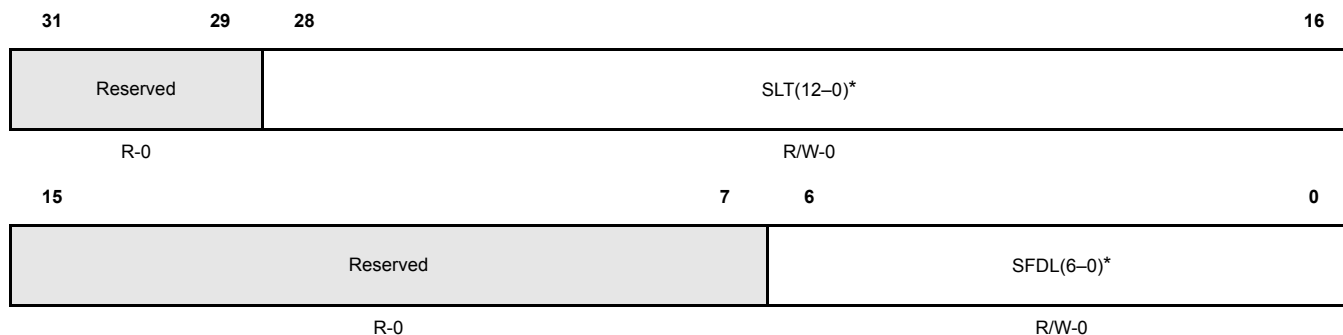
Figure 17-126. MHD Configuration Register (MHDC) [offset_CC = 0x98]
