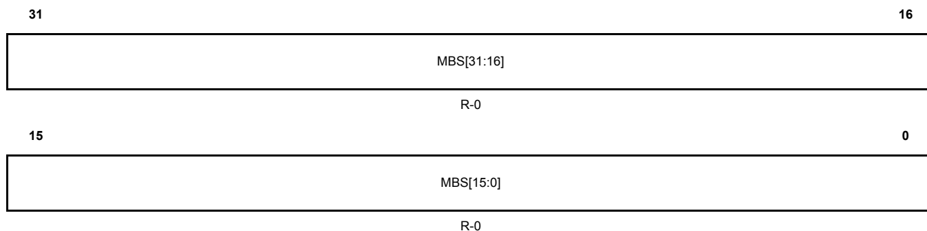
Figure 17-170. Message Buffer Status Changed Register 1 (MBSC1) [offset_CC = 0x340]
