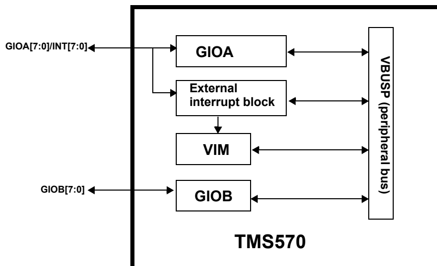
Figure 12-1. Device Level Overview
