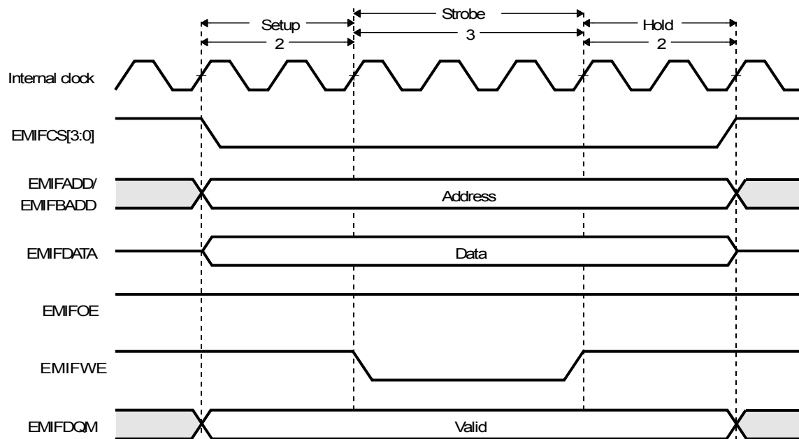
Figure 10-5. Timing Waveform of an Asynchronous Write Cycle in Normal Mode
