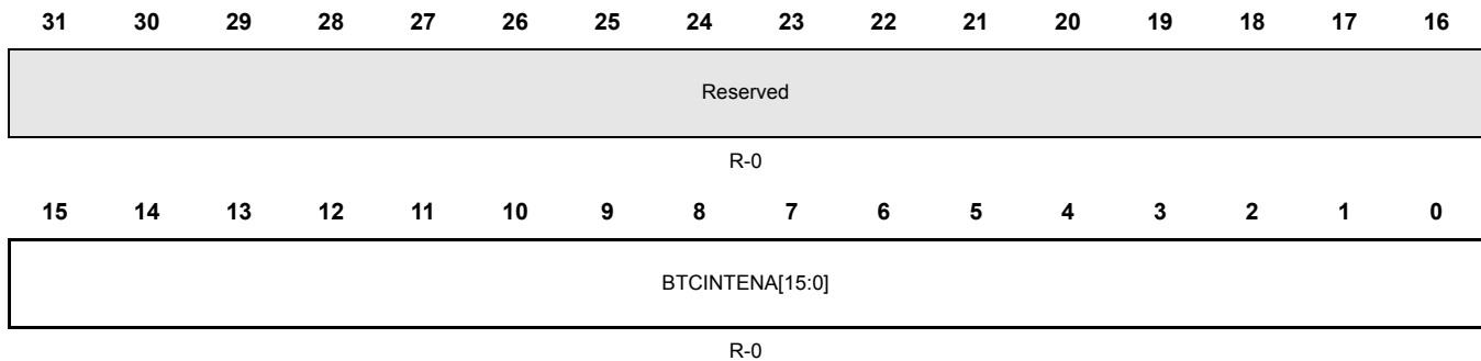
Figure 20-47. BTC Interrupt Enable Set (BTCINTENAS) [offset = 0x10C]
