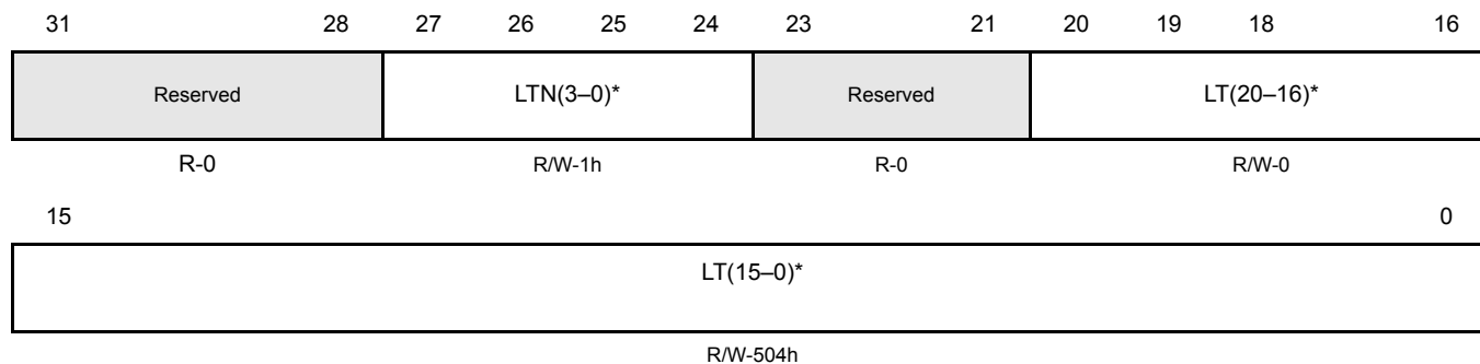
Figure 17-121. SUC Configuration Register2 (SUCC2) [offset_CC = 0x84]
