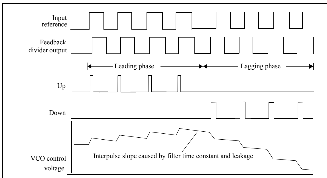
Figure 7-13. PFD Timing
