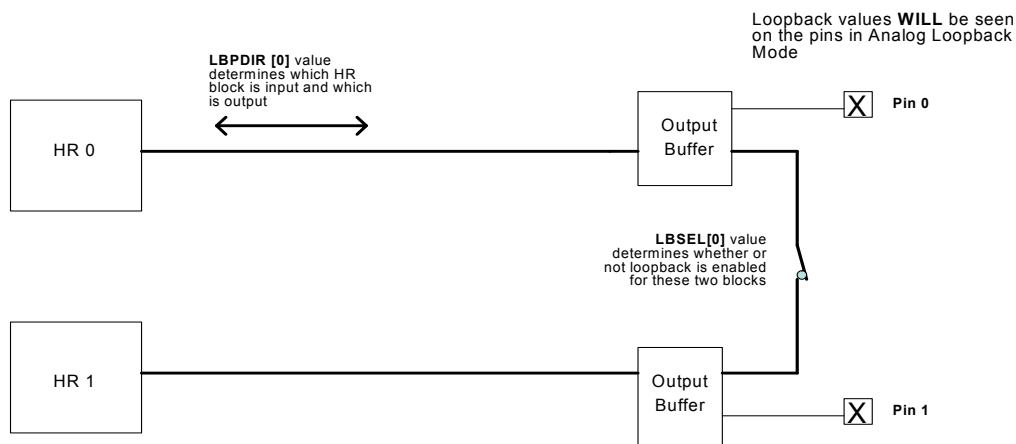
Figure 18-17. HR0 to HR1 Analog Loop Back Logic: LBTYPE[0] = '1'
