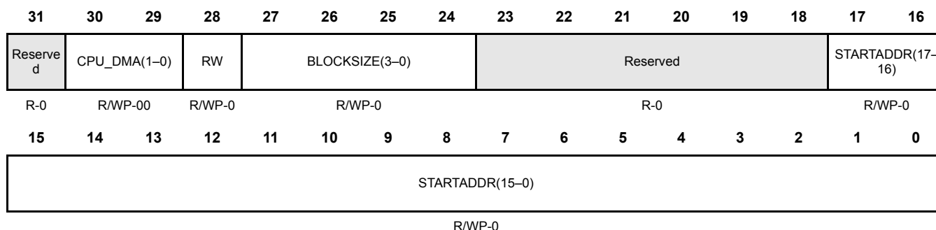
Figure 27-13. RTP RAM 2 Trace Region [1:2] Register (RTPRAM2REG[1:2]) [offset = 14h, 18h]
