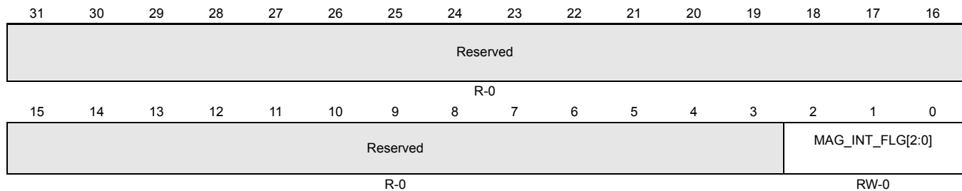
Figure 15-76. ADC Magnitude Compare Interrupt Flag (ADMAGINTFLG) [offset = 0x160]
