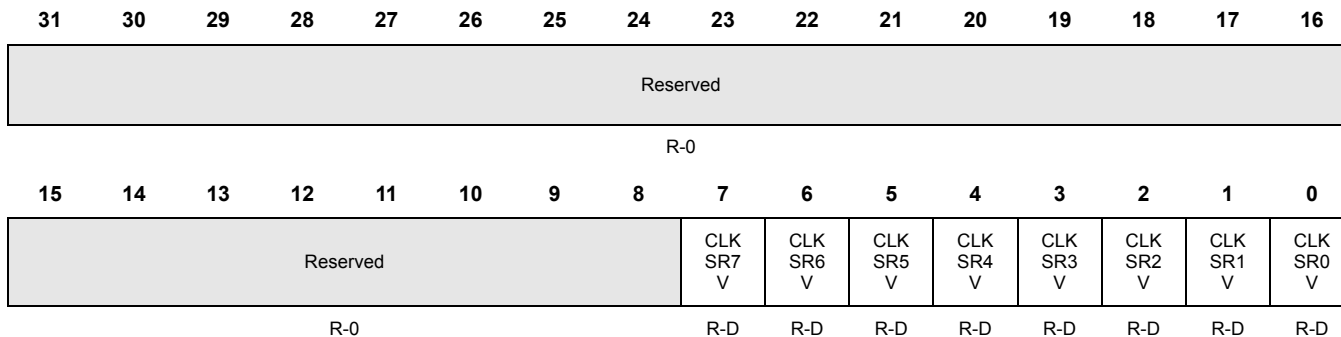
Figure 5-20. Clock Source Valid Status Register (CSVSTAT) [offset = 0x54]
