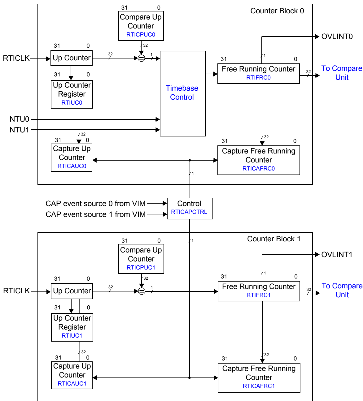
Figure 21-2. Counter Block Diagram
