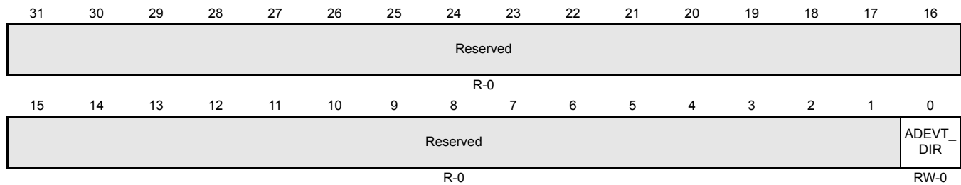
Figure 15-61. ADC ADEVT Pin Direction Control Register (ADEVTDIR) [offset = 0xFC]
