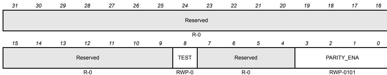
Figure 18-60. Parity Control Register (HETPCR) [0xFFF7B874]
