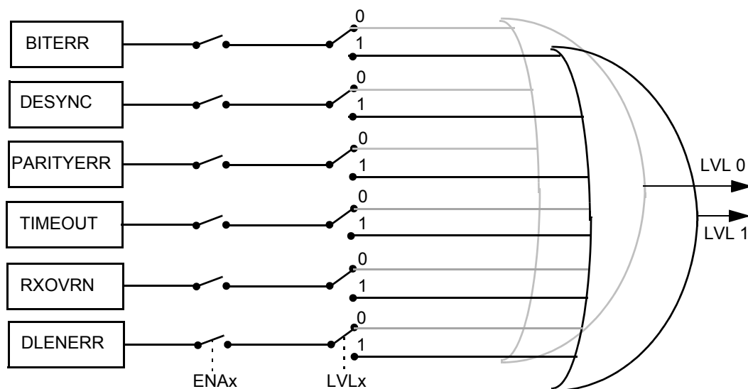
Figure 14-25. SPIFLG Interrupt Structure
