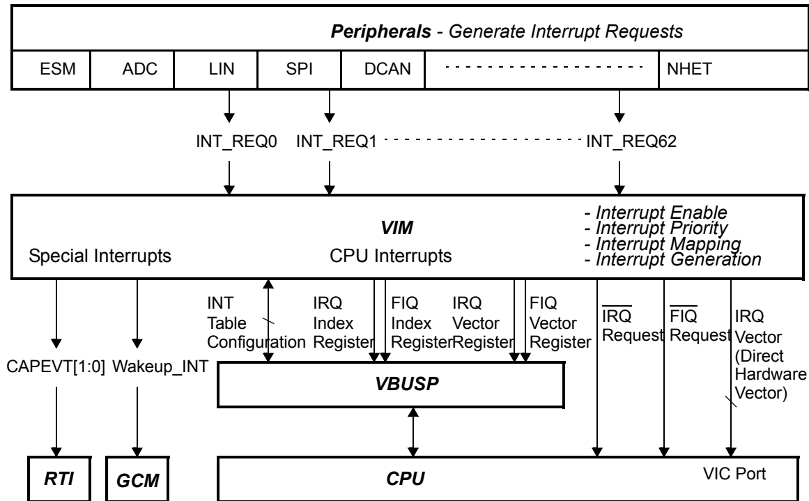
Figure 24-1. Device Level Interrupt Block Diagram
