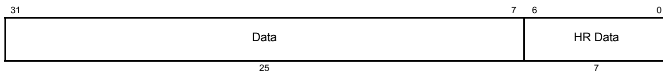
Figure 18-76. ADCNST Data Field (D31:D0)
