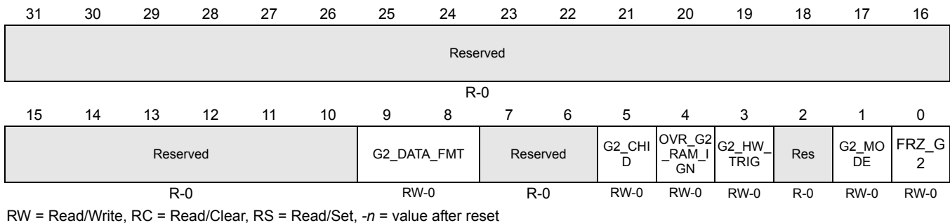
Figure 15-29. ADC Group2 Operating Mode Control Register (ADG2MODECR) [offset = 0x18]
