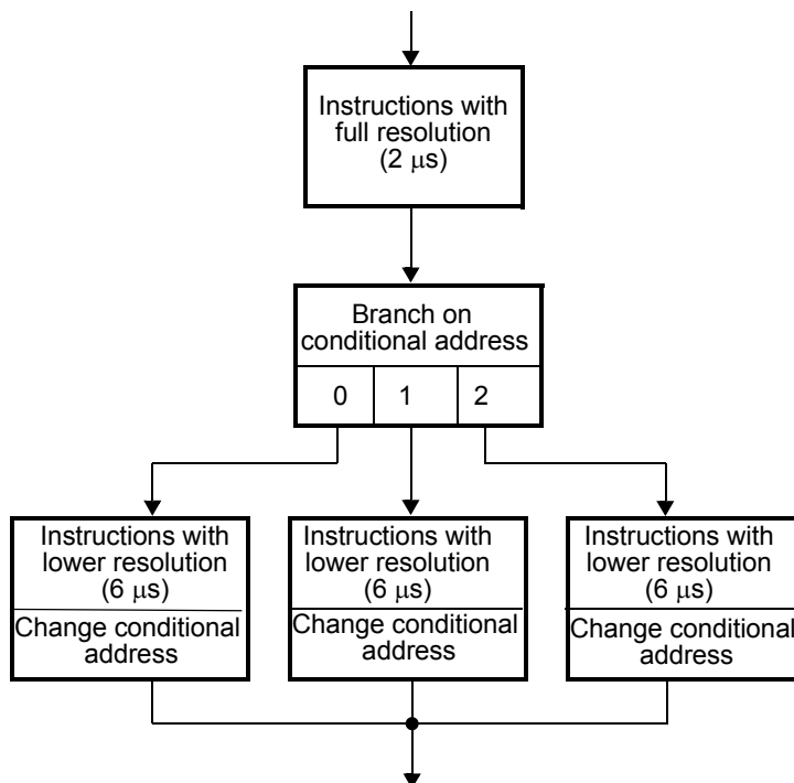
Figure 18-5. Multi-Resolution Operation Flow Example
