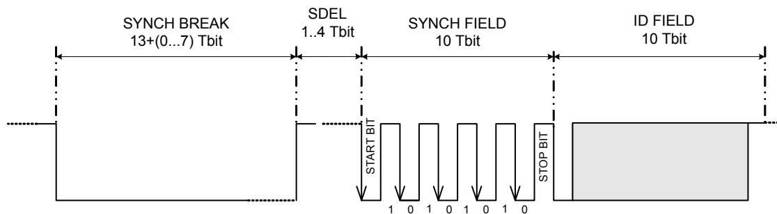
Figure 13-15. Message Header in Terms of T_{\text{bit}}
