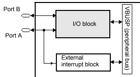
Figure 12-4. GIO Module Diagram
