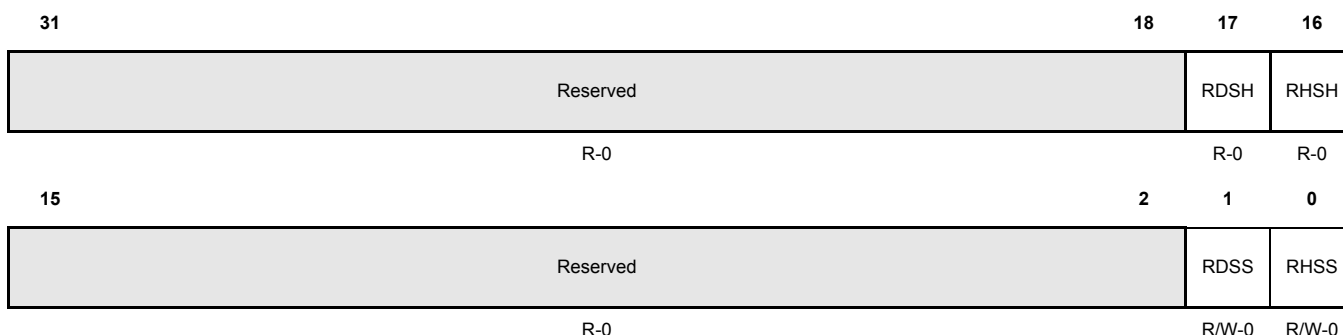
Figure 17-184. Output Buffer Command Mask Register (OBCM) [offset_CC = 0x700]
