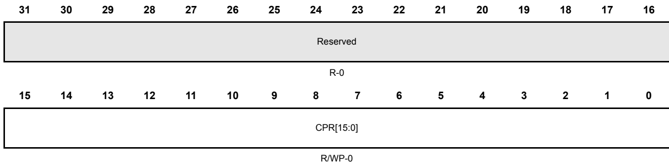
Figure 20-27. Channel Priority Reset Register (CHPRIOR) [offset = 0x3C]
