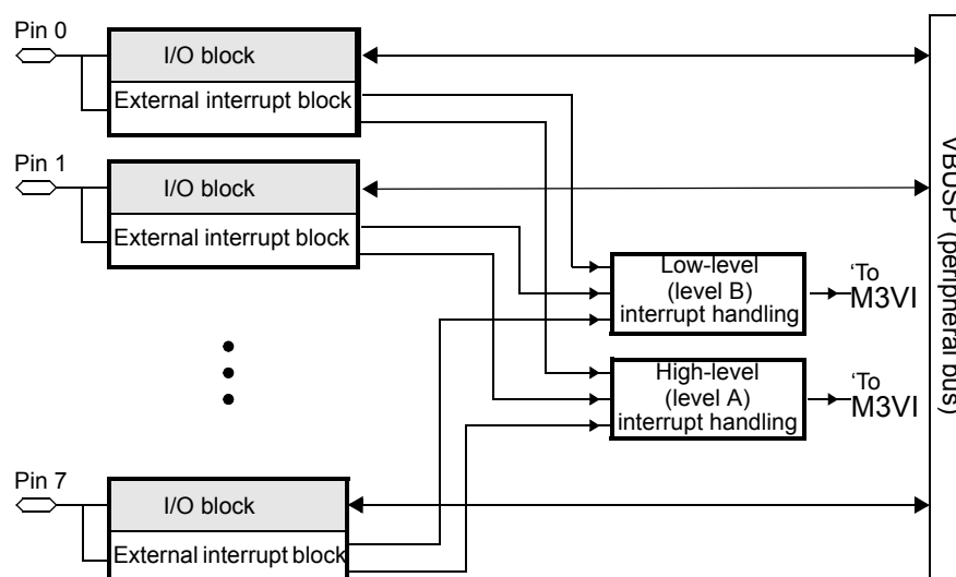
Figure 12-5. GIO Port A Module Diagram
