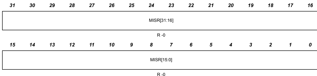
Figure 9-16. CPU2 Current MISR Register (CPU2_CURMISR3)
