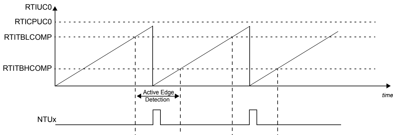
Figure 21-5. Clock detection scheme
