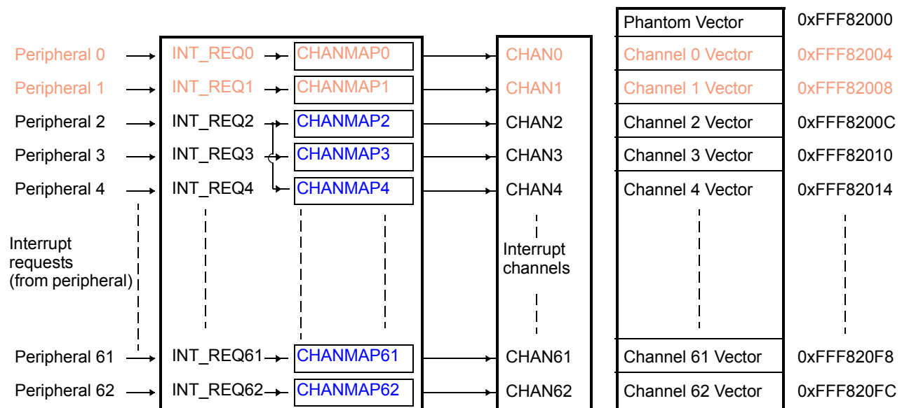
Figure 24-5. VIM in a Programmed State
