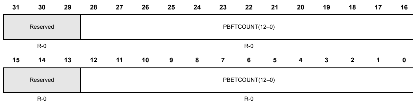
Figure 20-72. Port B Active Channel Transfer Count Register (PBACTC) [offset = 0x1A0]
