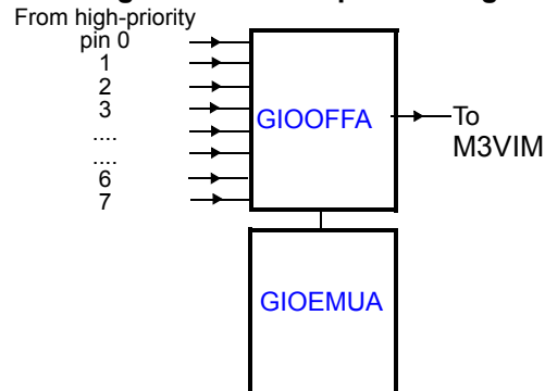
Figure 12-9. High-Level-Interrupt-Handling Block
