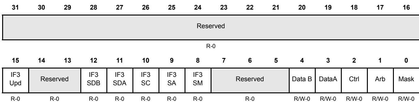
Figure 16-54. IF3 Observation Register (DCAN IF3OBS) [offset = 0x140]
