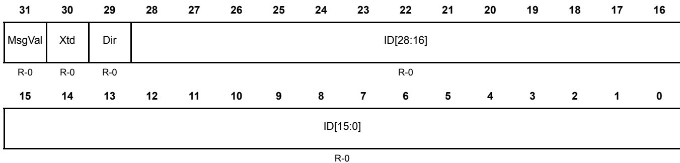
Figure 16-56. IF3 Arbitration Register (DCAN IF3ARB) [offset = 0x148]
