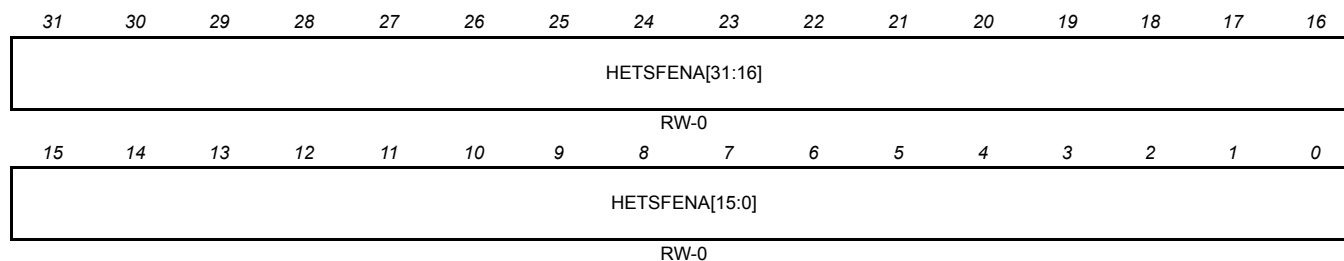
Figure 18-64. Suppression Filter Enable Register (HETSFENA) [0xFFF7B884]
