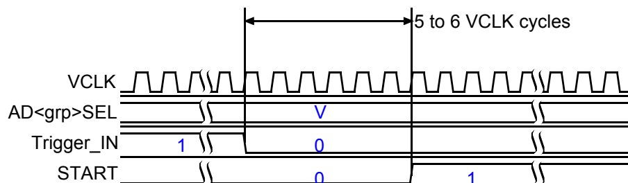
Figure 15-7. Timing Diagram of Hardware Trigger
