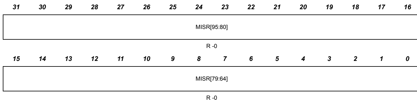
Figure 9-18. CPU2 Current MISR Register (CPU2_CURMISR1)
