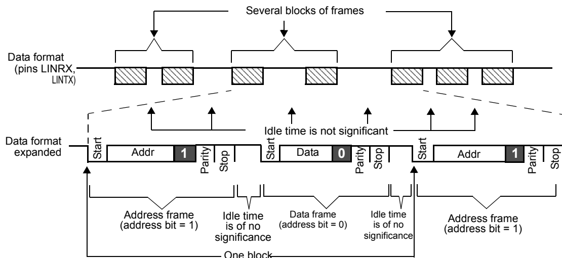
Figure 13-7. Address-Bit Multiprocessor Communication Format
