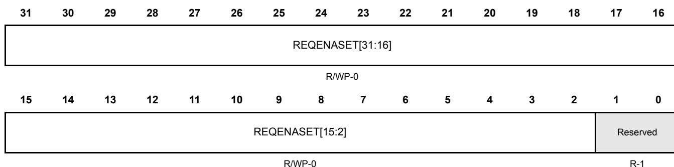
Figure 24-22. Interrupt Enable Set Register 0 (REQENASET0) [0xFFFFFE30]
