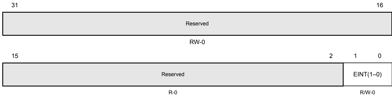
Figure 17-115. Interrupt Line Enable Register (ILE) [offset_CC = 0x40]
