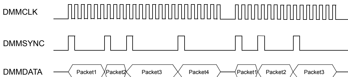
Figure 26-4. Packet Sync Signal example
