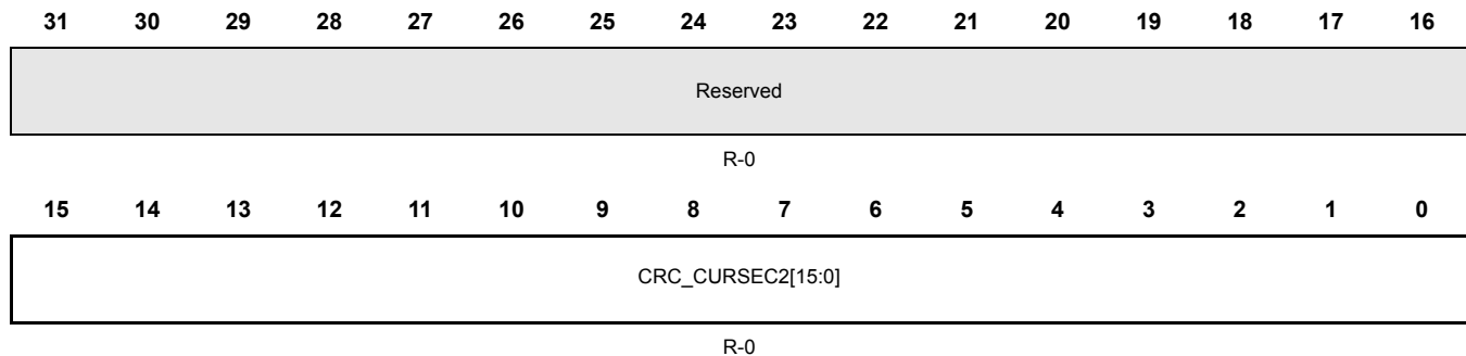
Figure 22-33. CRC Current Sector Register 2(CRC_CURSEC_REG2) [offset = 0x88]
