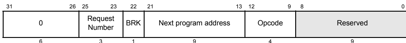
Figure 18-133. SCMP Control Field (C31:C0)
