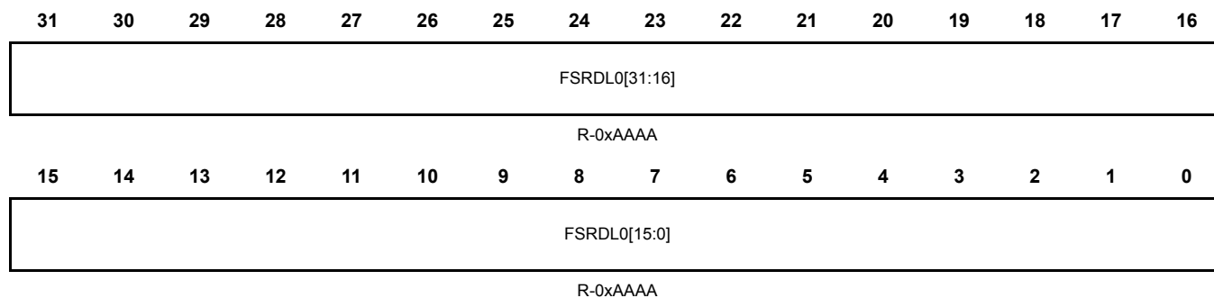
Figure 6-25. Fail Status Data Register 0 (FSRDL0) [offset = 0x01A8]
