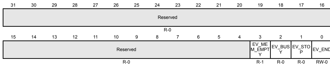
Figure 15-50. ADC Event Group Status Register (ADEVSR) [offset = 0x6C]
