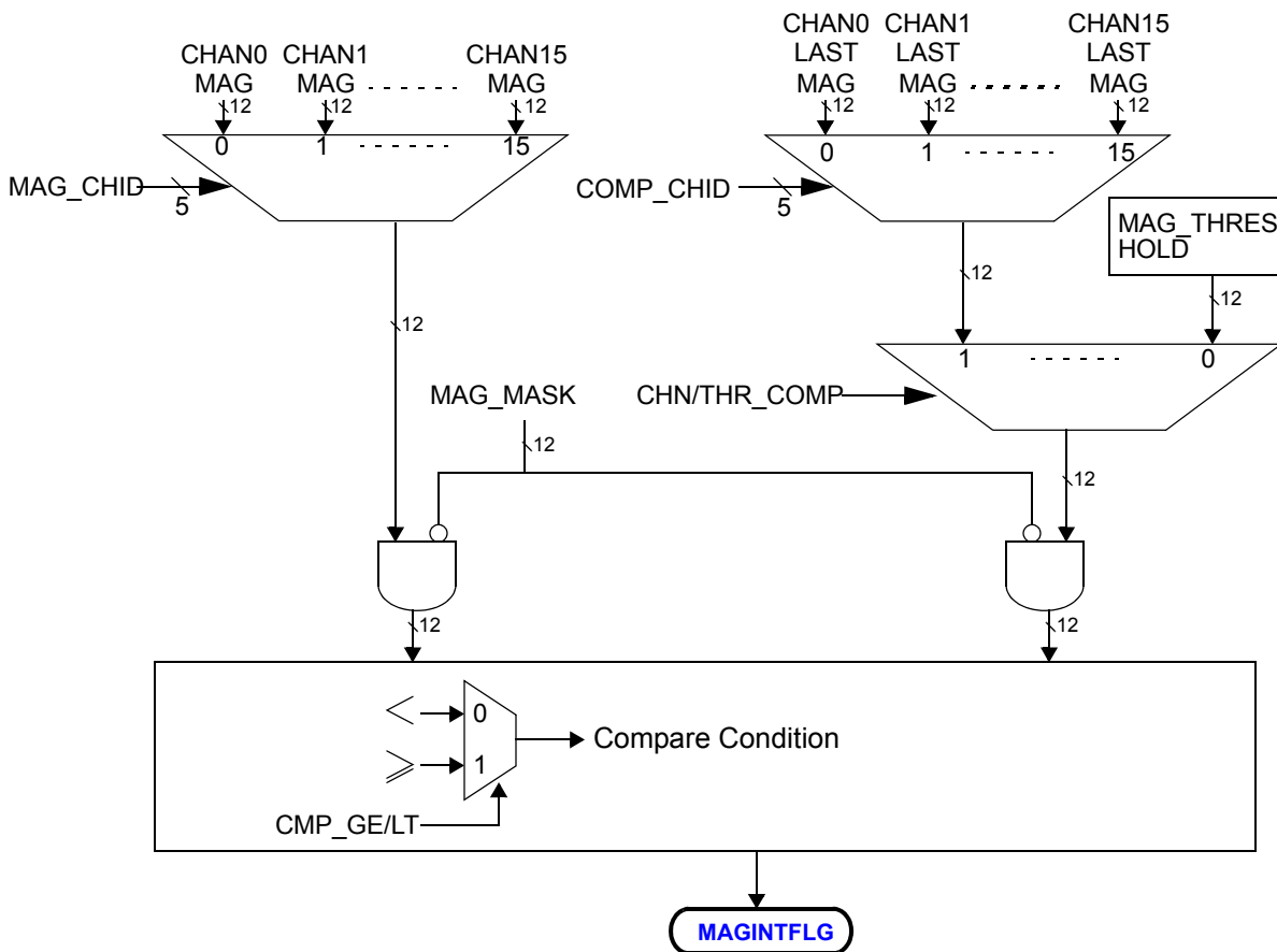
Figure 15-13. Magnitude Threshold Interrupt Configuration
