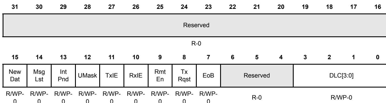
Figure 16-48. IF1 Message Control Register (DCAN IF1MCTL) [offset = 0x10C]
