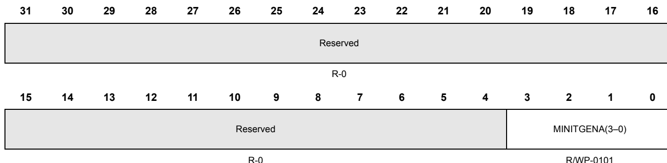
Figure 5-22. Memory Hardware Initialization Global Control Register (MINITGCR) [offset = 0x5C]
