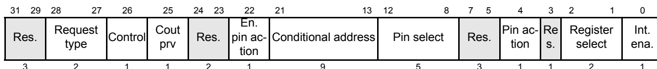
Figure 18-70. ACMP Data Field (D31:D0)
