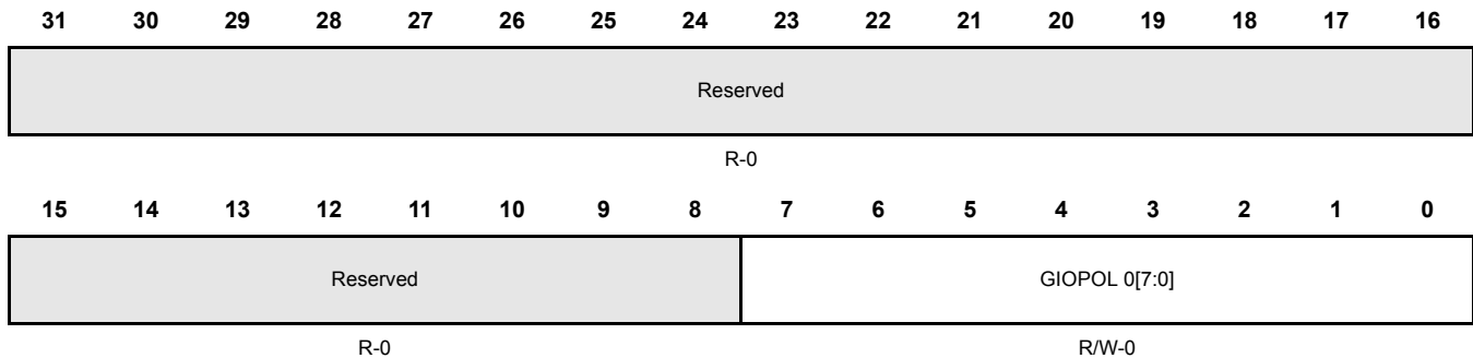
Figure 12-13. GIO Interrupt Polarity Register (GIOPOL) [0xFFF7BC0C]
