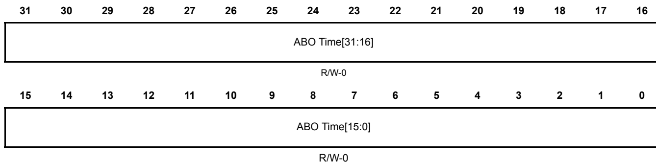
Figure 16-32. Auto-Bus-On Time Register (DCAN ABOTR) [offset = 0x80]
