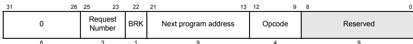
Figure 18-145. WCAPE Control Field (C31:C0)
