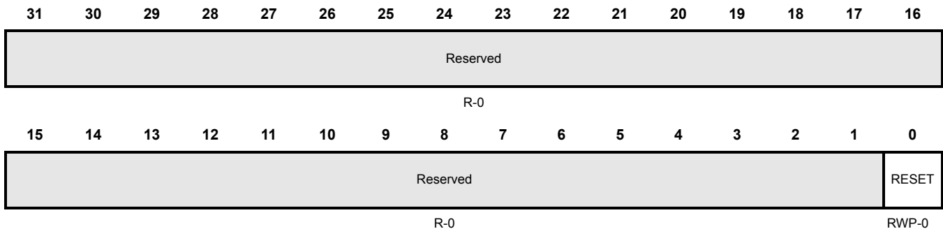
Figure 13-28. SCI Global Control Register 0 (SCIGCR0) [offset = 0x00]
