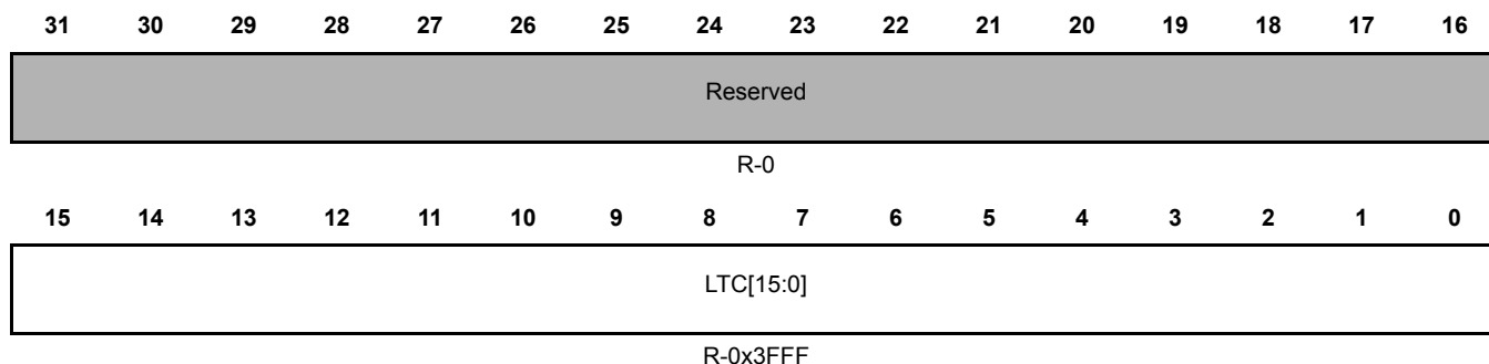
Figure 25-18. ESM Low-Time Counter Register (ESMLTCR)
