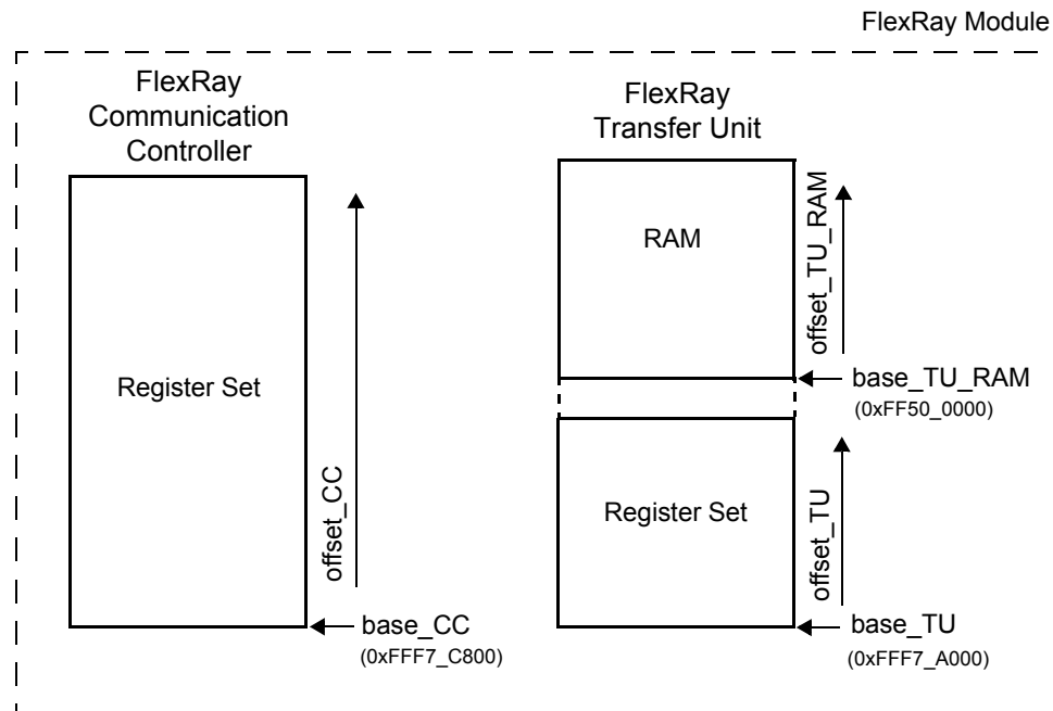
Figure 17-2. FlexRay Module Blocks
