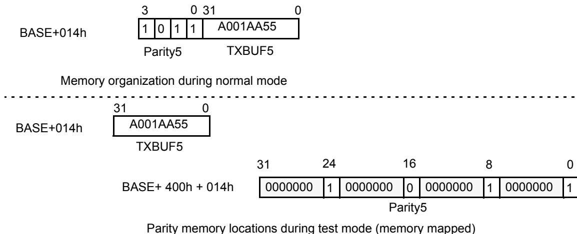
Figure 14-52. Example of Memory Mapped Parity Locations during Test Mode
