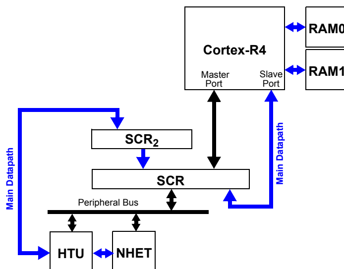
Figure 19-1. System Block Diagram
