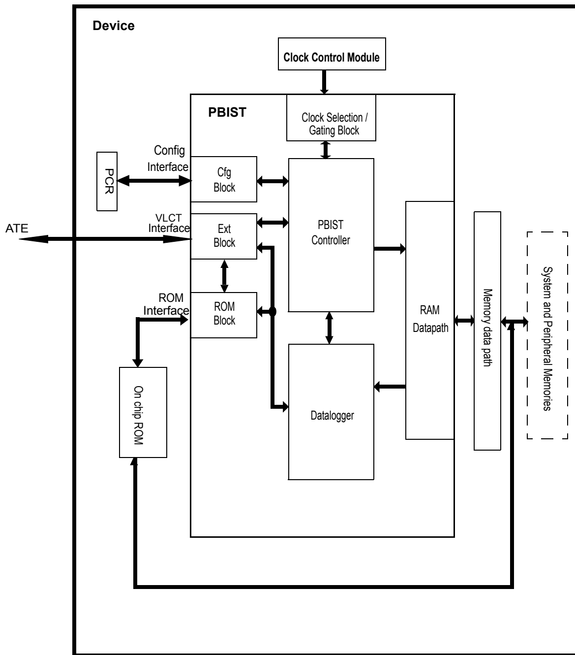
Figure 6-1. PBIST Block Diagram
