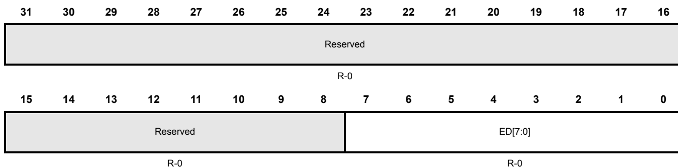
Figure 13-40. Receiver Emulation Data Buffer (SCIED) [offset = 0x30]
