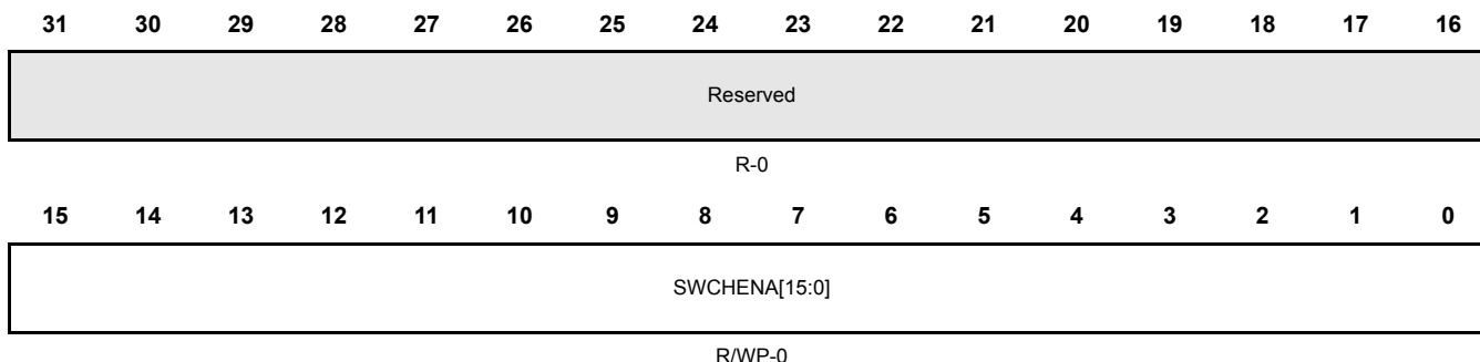
Figure 20-24. SW Channel Enable Set and Status Register (SWCHENAS) [offset = 0x24]
