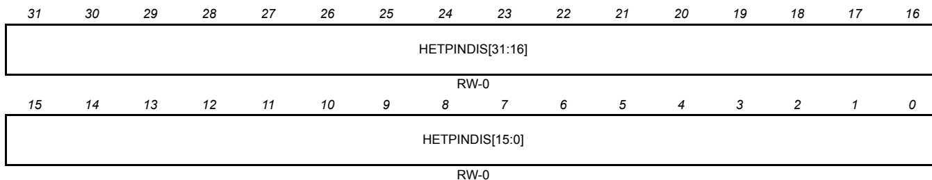
Figure 18-67. NHET Pin Disable Register (HETPINDIS) [0xFFFF7B894]
