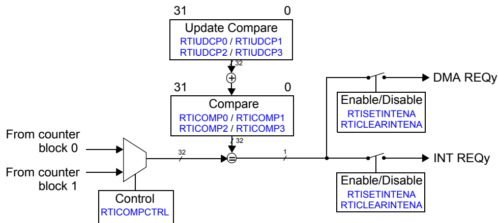
Figure 21-3. Compare Unit Block Diagram (shows only 1 of 4 blocks for simplification)
