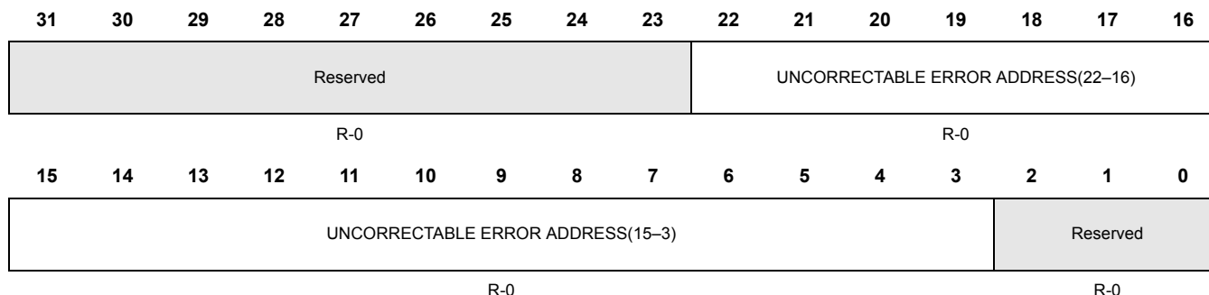
Figure 4-9. TCRAM Wrapper Uncorrectable Error Address Register (RAMUERRADDR) [offset = 0x1C]
