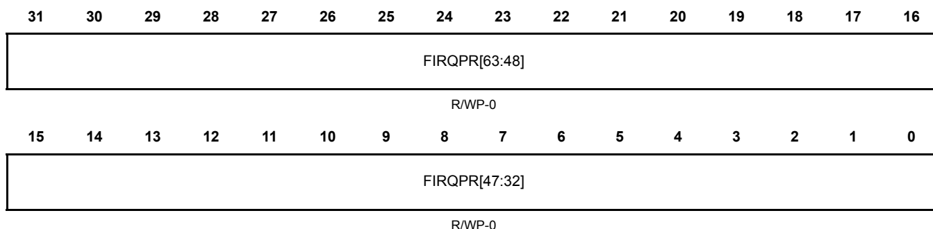
Figure 24-19. FIQ/IRQ Program Control Register 1 (FIRQPR1) [0xFFFFFE14]
