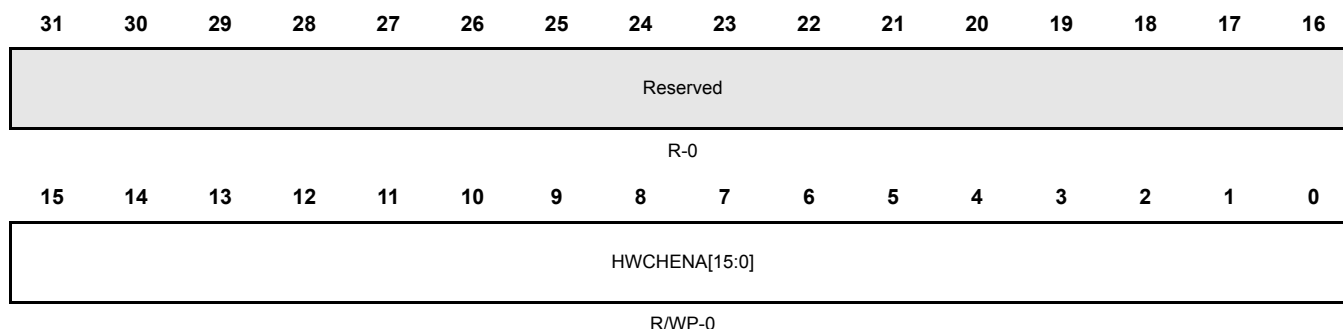
Figure 20-22. HW Channel Enable Set and Status Register (HWCHENAS) [offset = 0x14]
