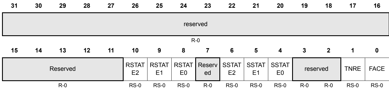
Figure 17-50. Transfer Error Interrupt Enable Set (TEIRES) [offset_TU = 0x78]
