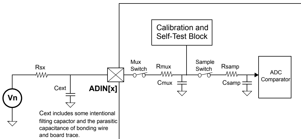
Figure 15-20. Board Level Circuit for Self-Test Mode
