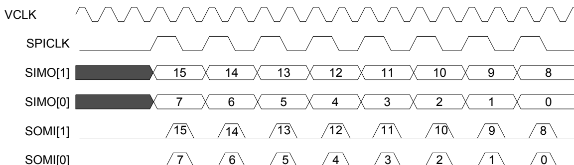
Figure 14-17. Two-Pin Parallel Mode Timing Diagram (Phase 0, Polarity 0)
