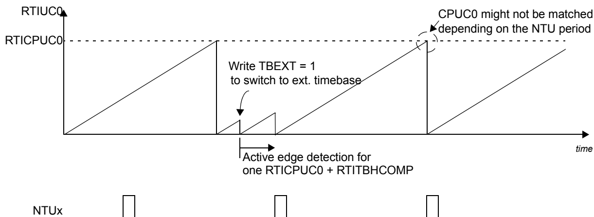
Figure 21-6. Switch to NTUx
