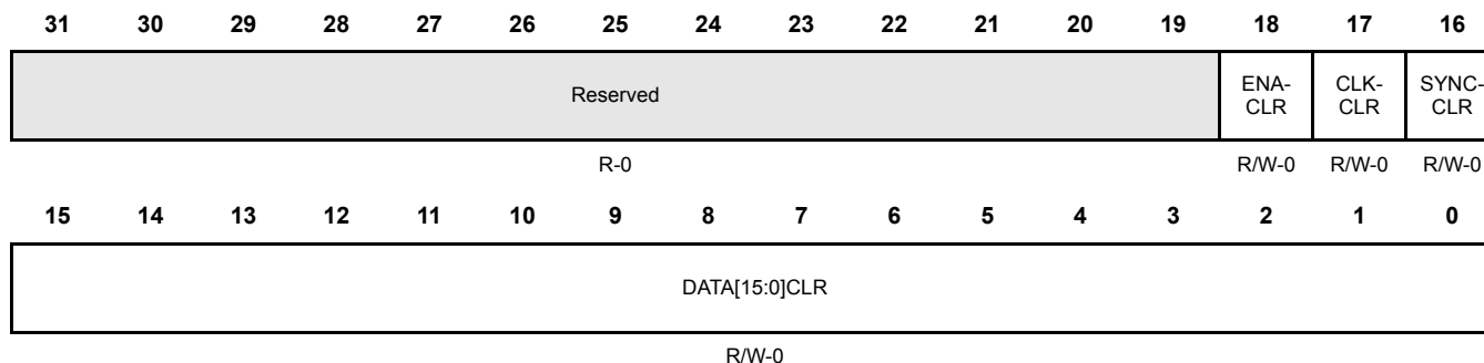
Figure 27-21. RTP Pin Control 5 Register (RTPPC5) [offset = 48h]
