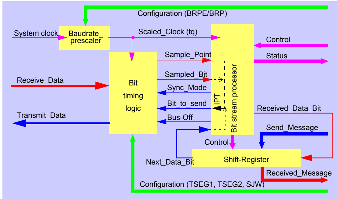
Figure 16-19. Structure of the CAN Core's CAN Protocol Controller
