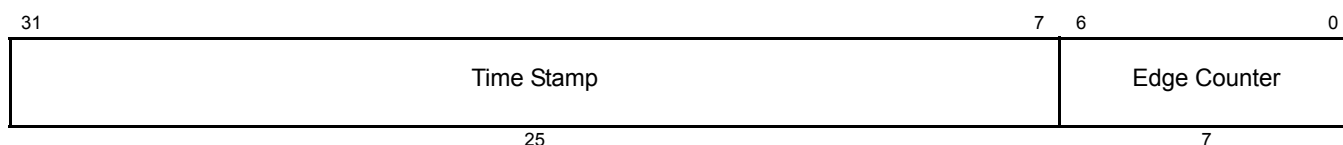
Figure 18-146. WCAPE Data Field (D31:D0)
