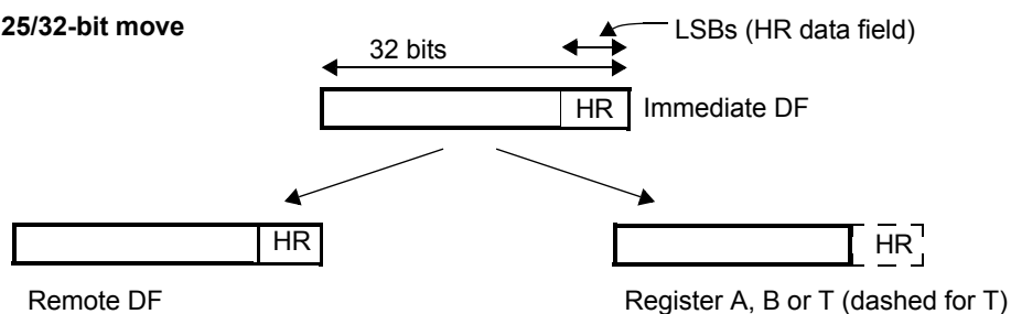
Figure 18-115. MOV32 Move Operation for IMTOREG&REM (Case 01)
