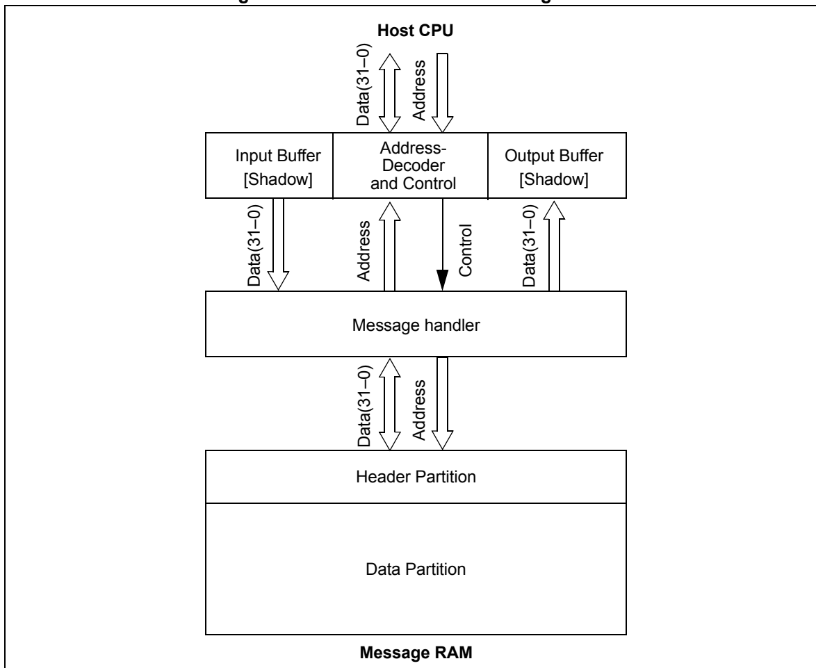
Figure 17-15. Host Access to Message RAM
