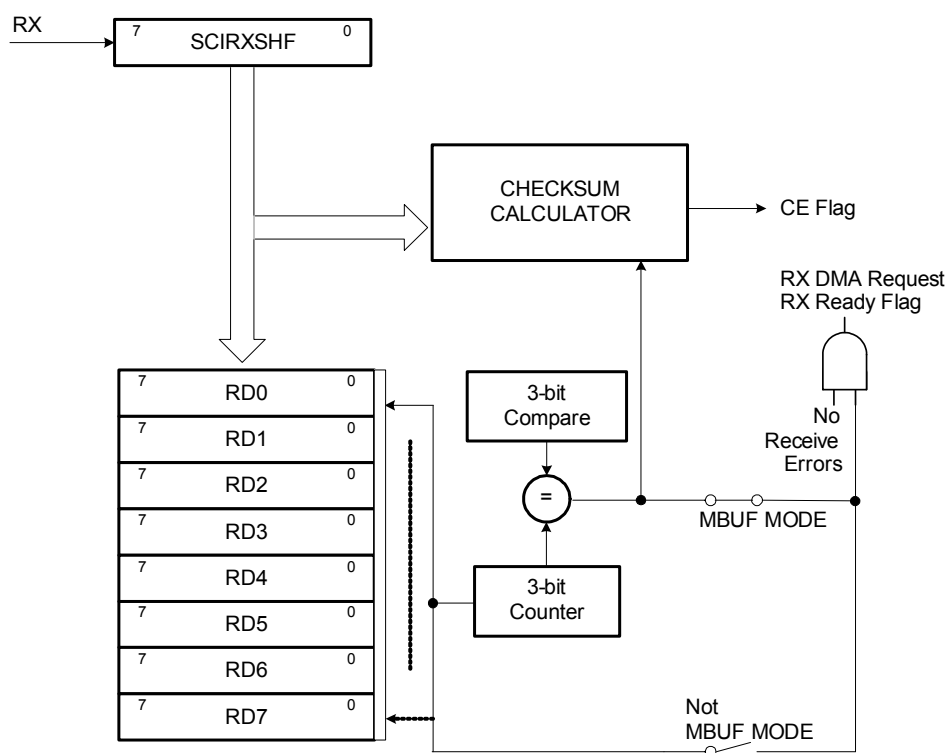
Figure 13-8. Receive Buffers
