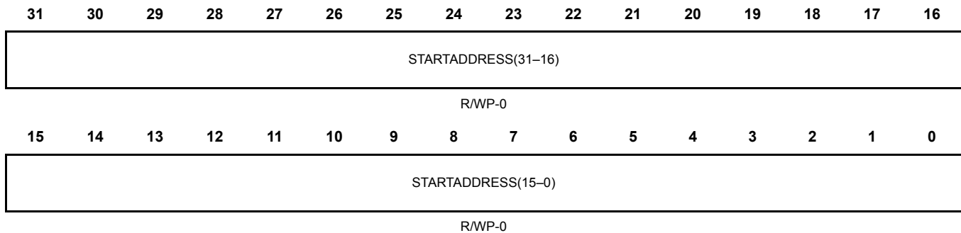
Figure 20-79. DMA Memory Protection Region 1 Start Address Register (DMAMPR1S) [offset = 0x1C0]
