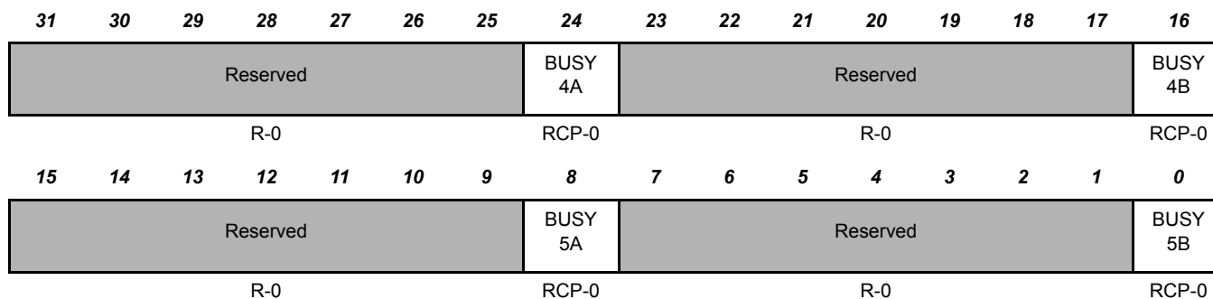
Figure 19-20. Control Packet (CP) Busy Register 2 (HTU BUSY2) [offset = 0x10]
