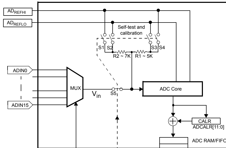
Figure 15-16. Self-Test and Calibration Logic
