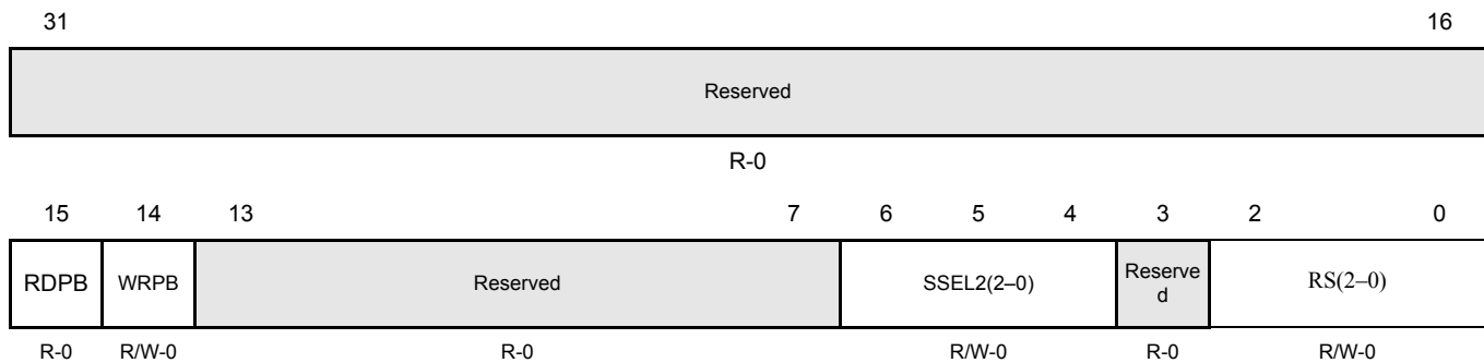
Figure 17-105. Test Register2 (TEST2) [offset_CC = 0x14]
