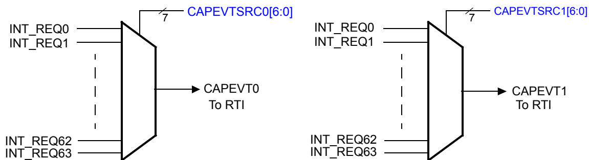
Figure 24-10. Capture Event Sources
