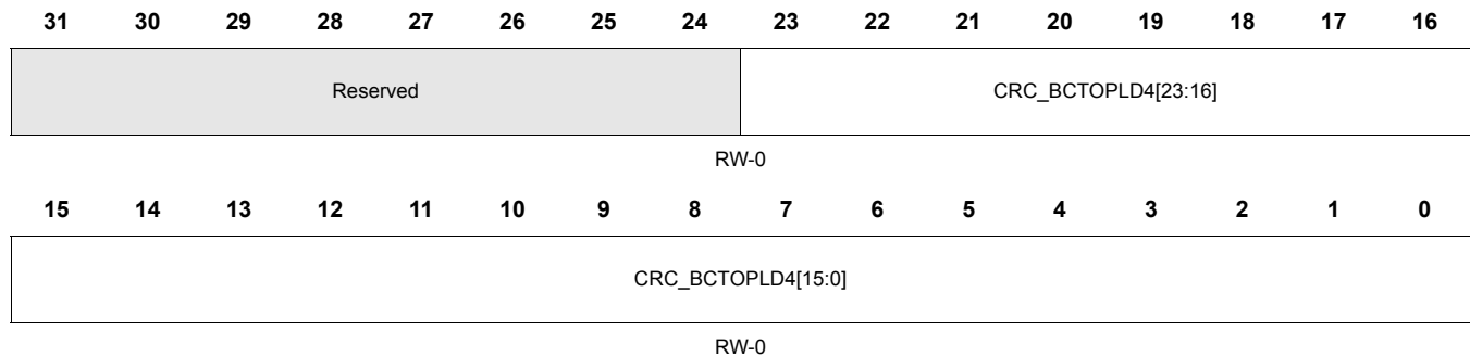
Figure 22-61. CRC Channel 4 Block Complete Timeout Preload Register B(CRC_BCTOPLD4) [offset = 0x110]
