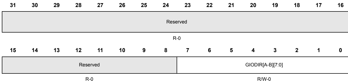
Figure 12-23. GIO Data Direction Registers [A-B][7:0] (GIODIR[A-B][7:0])[0xFFF7BC34, 0xFFF7BC54]
