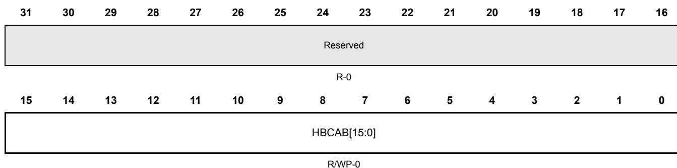
Figure 20-38. HBC Interrupt Mapping Register (HBCMAP) [offset = 0xC4]
