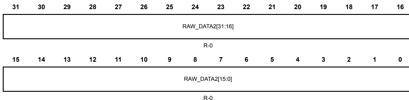
Figure 22-42. Channel 2 Raw Data Low Register(RAW_DATAREGL2) [offset = 0xB8]
