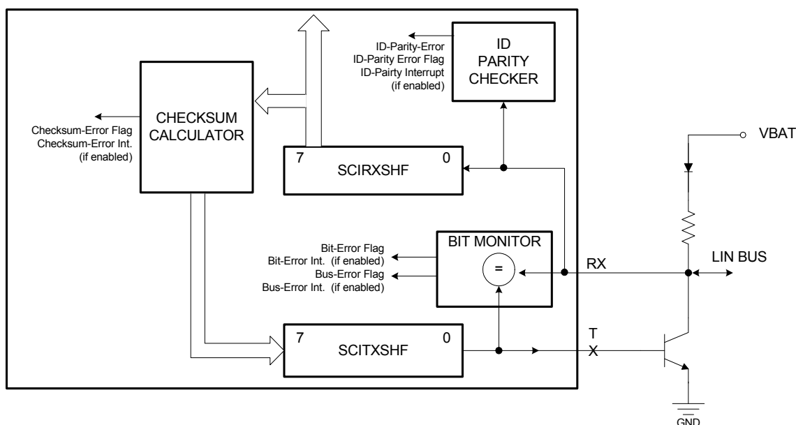
Figure 13-21. TXRX Error Detector
