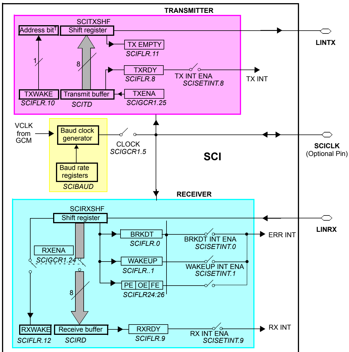
Figure 13-1. Detailed SCI Block Diagram
