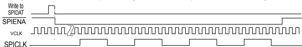
Figure 14-58. SPI/MibSPI pins during Slave mode in 4pin with \overline{\text{SPIENA}} configuration
