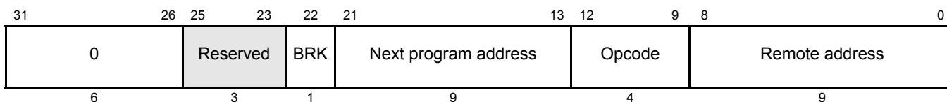
Figure 18-119. MOV64 Control Field (C31:C0)
