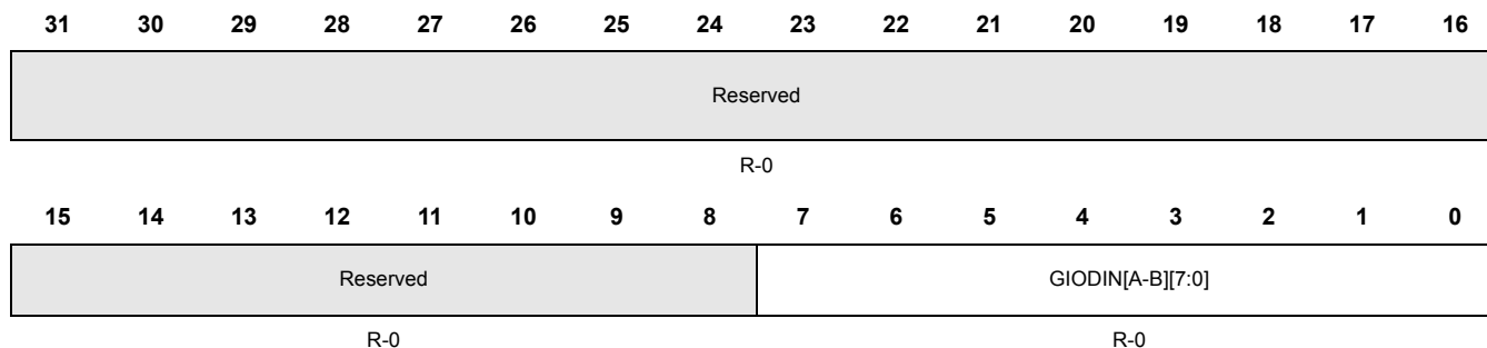
Figure 12-24. GIO Data Input Registers [A-B][7:0] (GIODIN[A-B][7:0])[0xFFF7BC38, 0xFFF7BC58]
