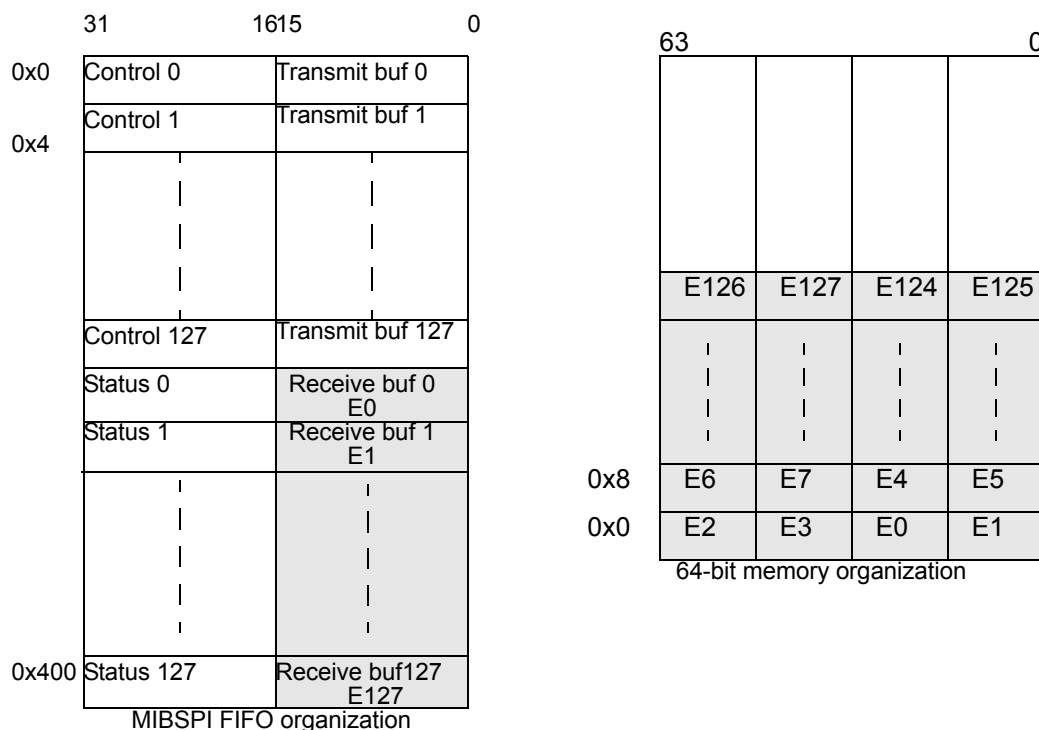
Figure 20-13. Example of DMA Data Packing
