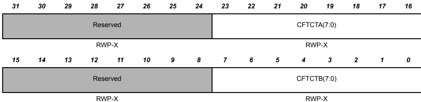
Figure 19-52. Current Frame Count Register (HTU CFCOUNT)
