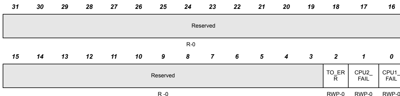
Figure 9-11. SelfTest Fail Status Register (STCFSTAT)
