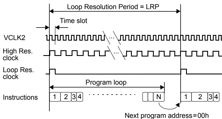
Figure 18-3. Program Flow Timings
