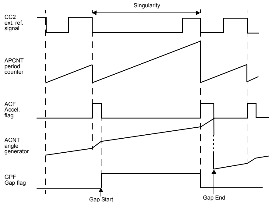
Figure 18-34. NHET Timings Associated with the Gap Flag (ACNT Acceleration)
