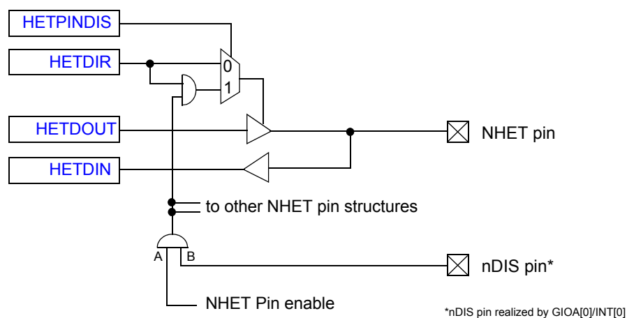
Figure 18-25. NHET Pin Disable Feature Diagram
