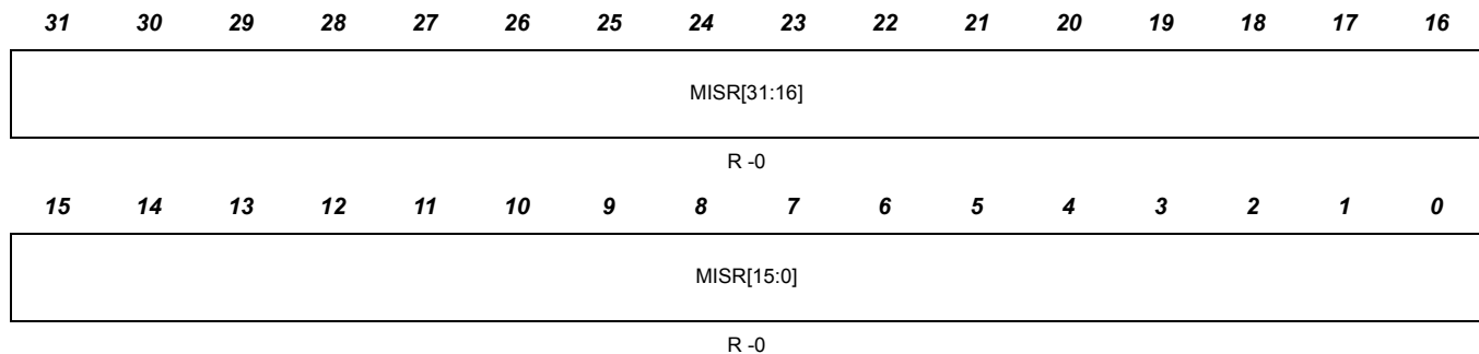
Figure 9-12. CPU1 Current MISR Register (CPU1_CURMISR3)
