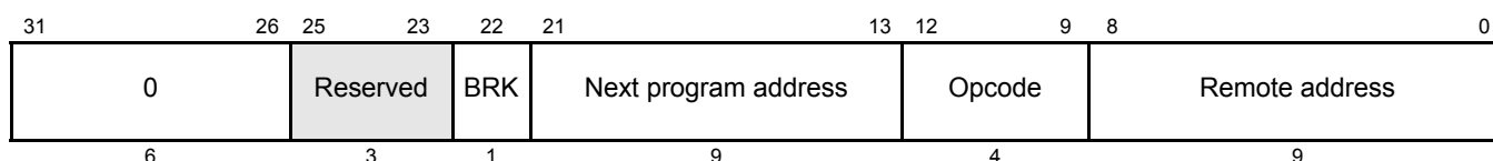
Figure 18-75. ADCNST Control Field (C31:C0)
