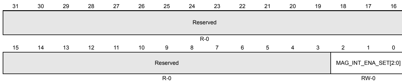
Figure 15-74. ADC Magnitude Compare Interrupt Enable Set (ADMAGINTENASET) [offset = 0x158]
