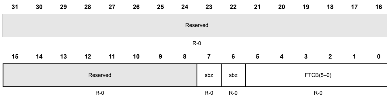
Figure 20-60. FTCB Interrupt Channel Offset Register (FTCBOFFSET) [offset = 0x160]
