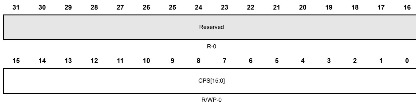
Figure 20-26. Channel Priority Set Register (CHPRIOS) [offset = 0x34]
