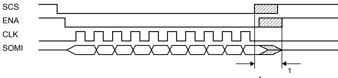
Figure 14-22. Transmit-Data-Finished-to-ENA-Inactive-Timeout
