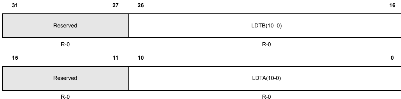
Figure 17-156. Last Dynamic Transmit Slot (LDTS) [offset_CC = 0x314]
