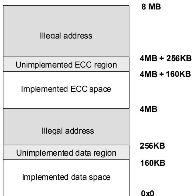
Figure 4-2. RAM Memory Map
