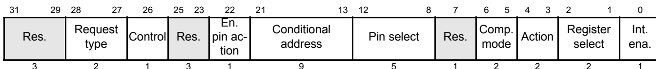
Figure 18-120. MOV64 Data Field (D31:D0)
