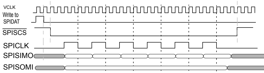
Figure 14-54. SPI/MibSPI pins during Master mode 4-pin with \overline{\text{SPISCS}} configuration.
