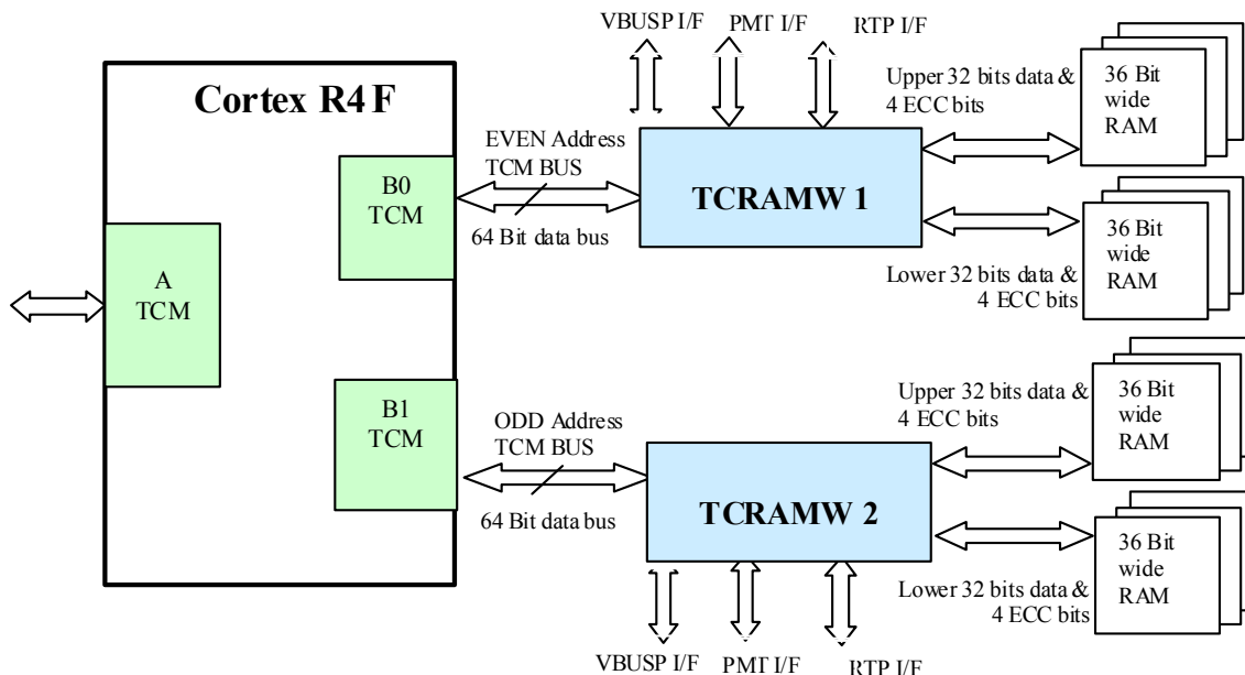
Figure 4-1. TCRAM Wrapper Connections
