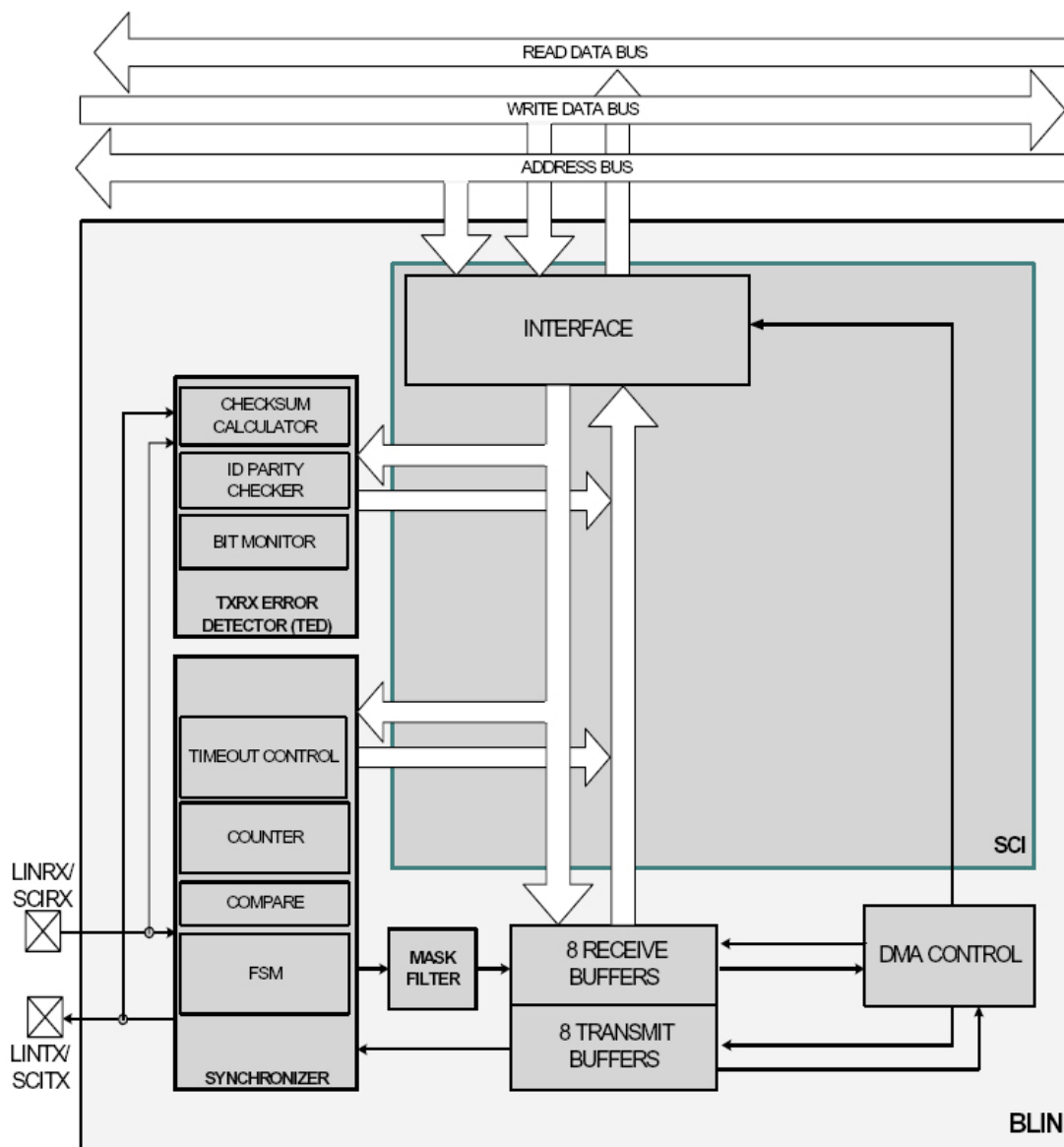
Figure 13-2. SCI/LIN Block Diagram
