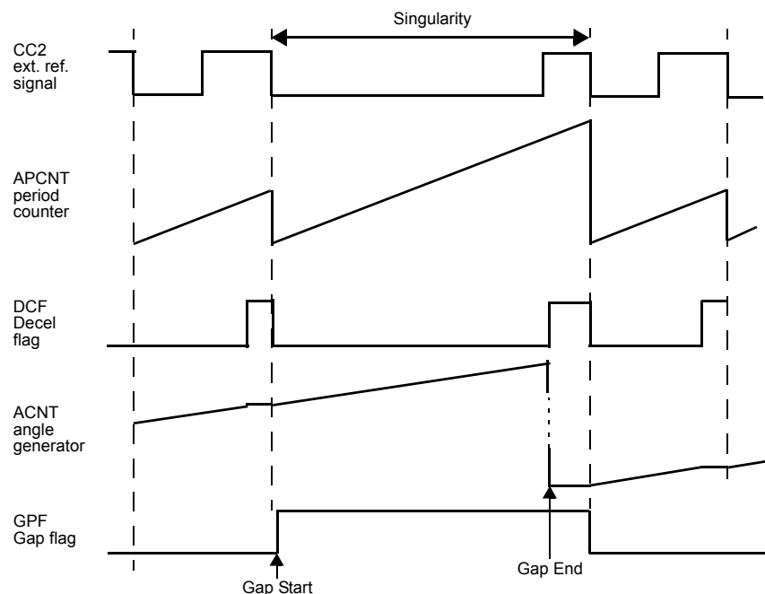
Figure 18-34. NHET Timings Associated with the Gap Flag (ACNT Acceleration)
