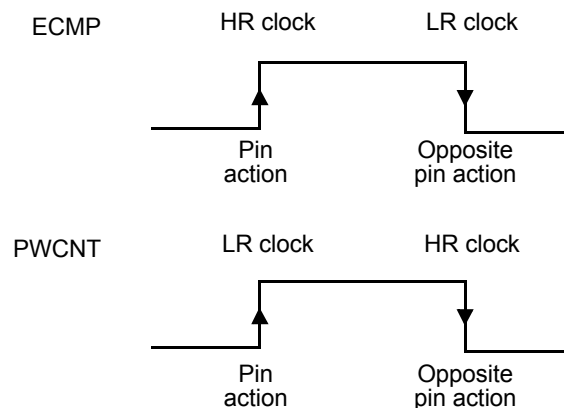
Figure 18-20. High/Low Resolution Modes for ECMP and PWCNT
