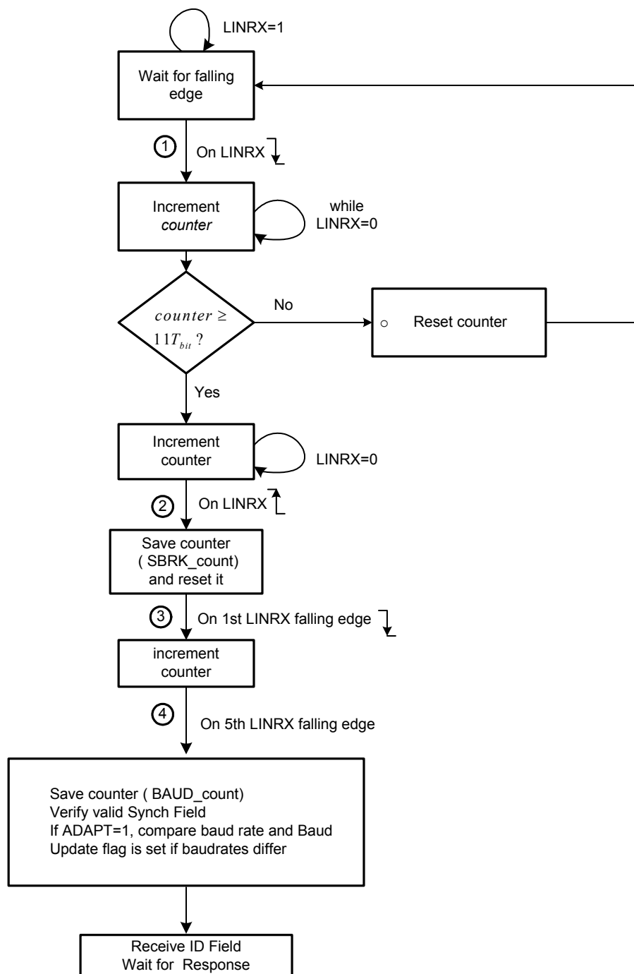
Figure 13-18. Synchronization Validation Process and Baud Rate Adjustment
