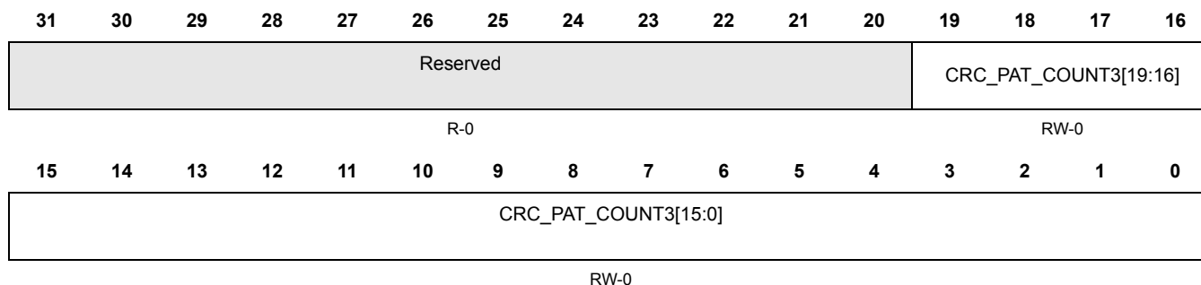
Figure 22-44. CRC Pattern Counter Preload Register3(CRC_PCOUNT_REG3) [offset = 0xC0]
