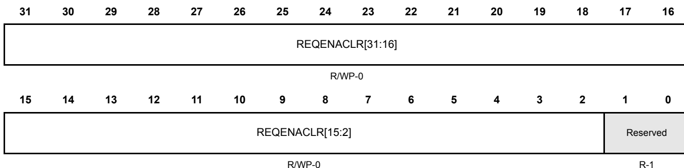
Figure 24-24. Interrupt Enable Clear Register 0 (REQENACLR0) [0xFFFFFE40]
