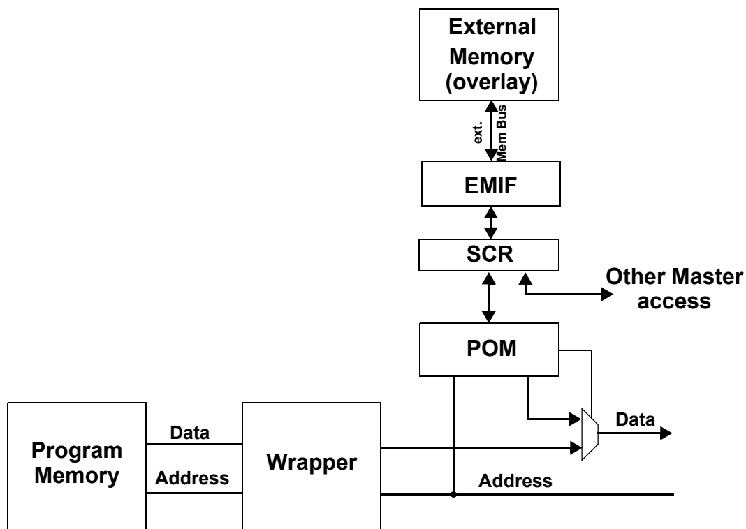
Figure 11-1. System block diagram for external memory configuration
