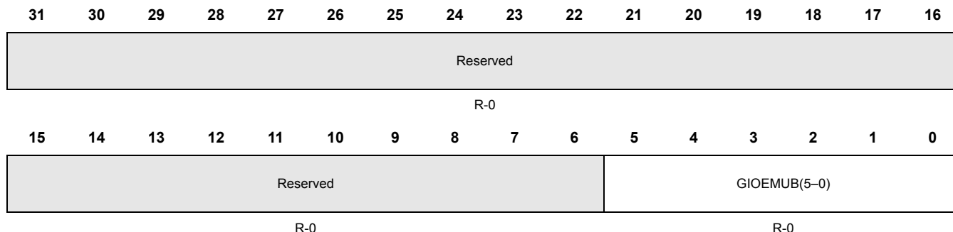
Figure 12-22. GIO Emulation B Register (GIOEMUB) [0xFFF7BC30]
