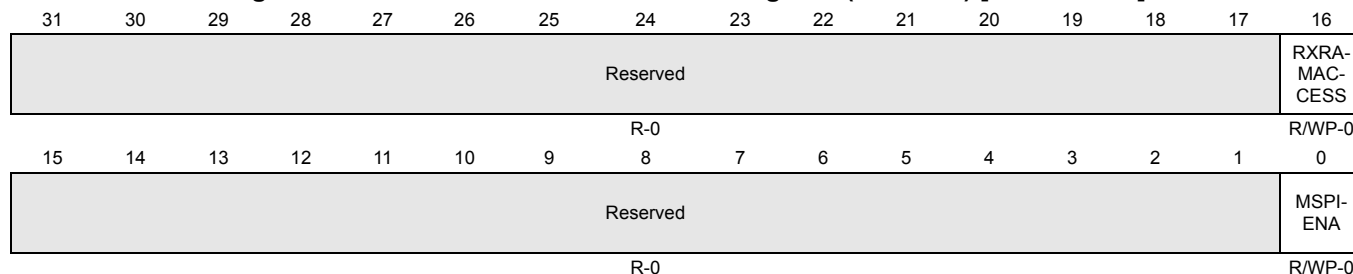
Figure 14-29. Multi-buffer Mode Enable Register (MIBSPIE) [offset = 70h]
