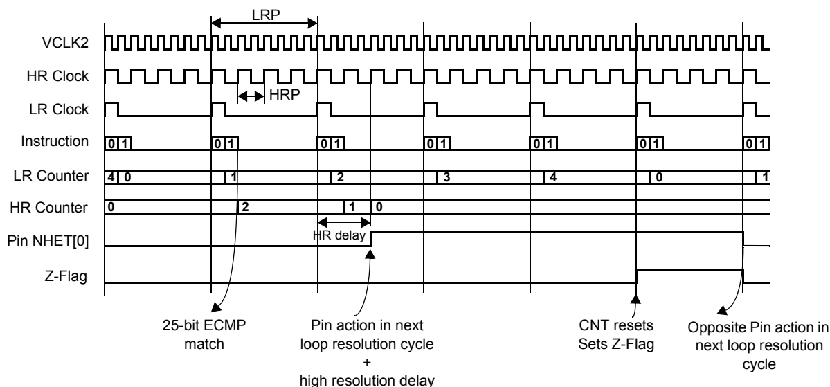
Figure 18-19. ECMP Execution Timings
