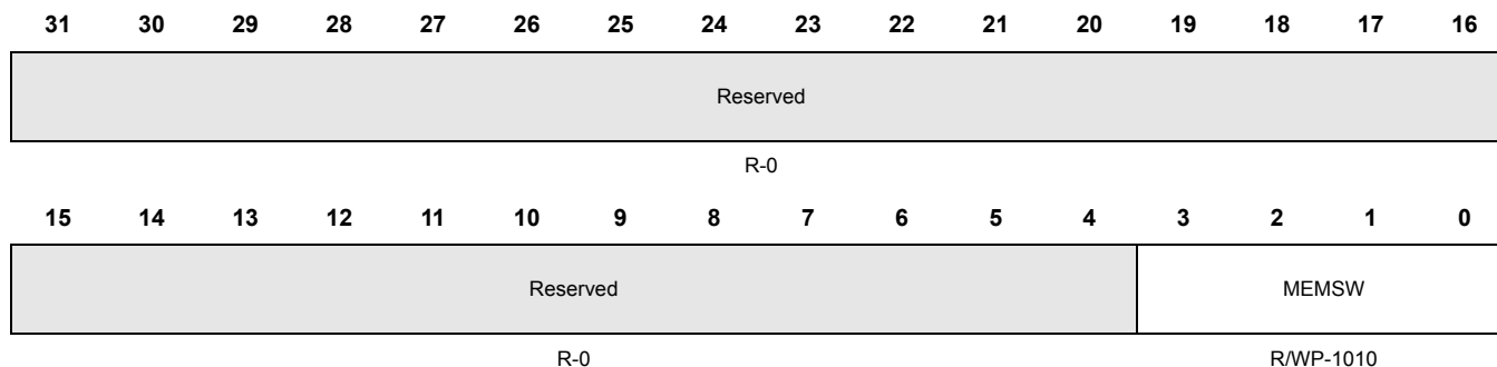
Figure 5-39. Bus Matrix Module Control Register 1 (BMMCR) [offset = 0xC4]
