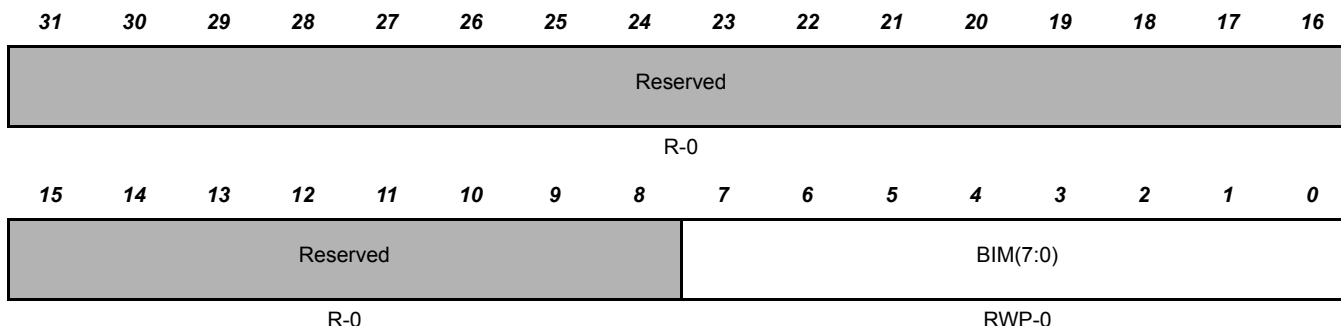
Figure 19-29. Buffer Initialization Mode Register (HTU BIM) [offset = 0x3C]
