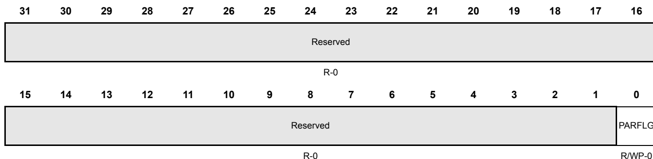
Figure 24-12. Interrupt Vector Table Parity Flag Register (PARFLG) [0xFFFFFDEC]
