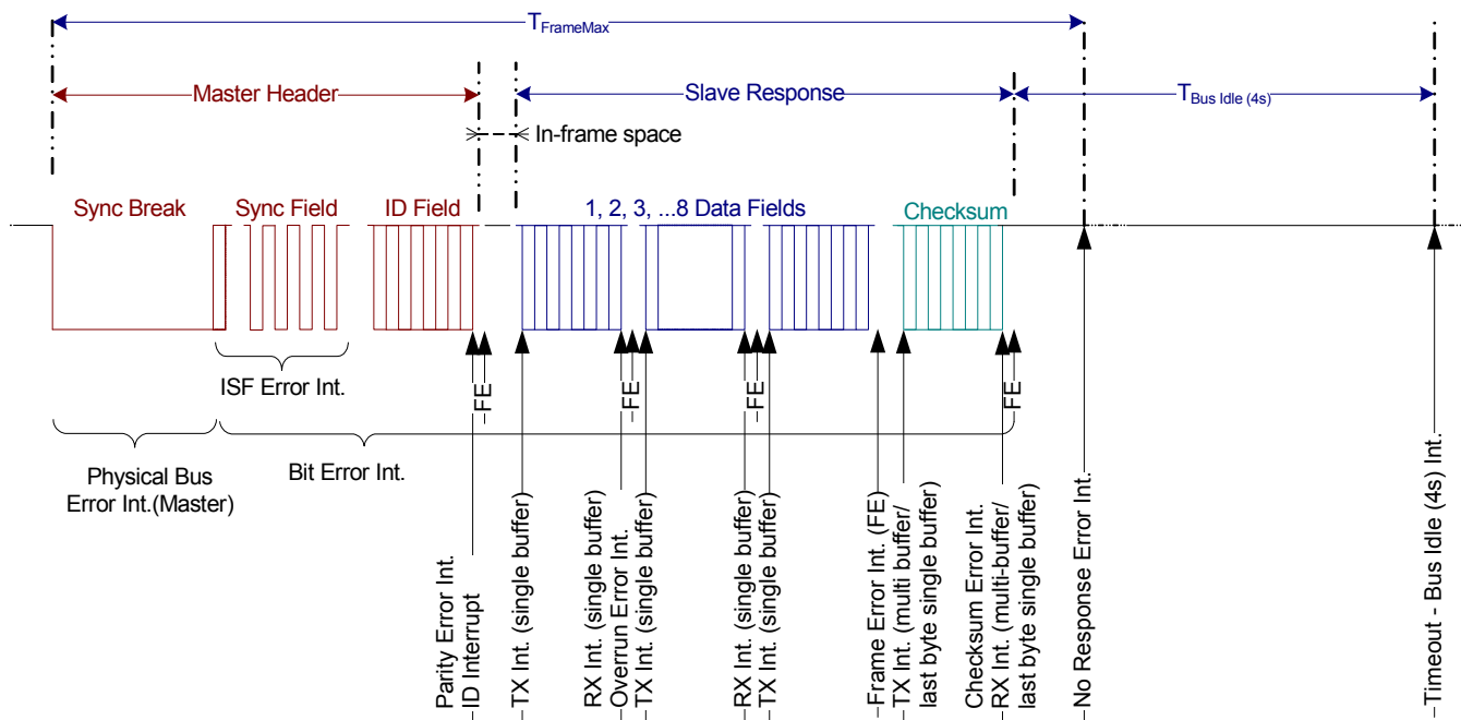
Figure 13-25. LIN Message Frame Showing LIN Interrupt Timing and Sequence
