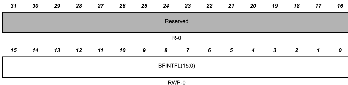
Figure 19-31. Buffer Full Interrupt Flag Register (HTU BFINTFL) [offset = 0x44]
