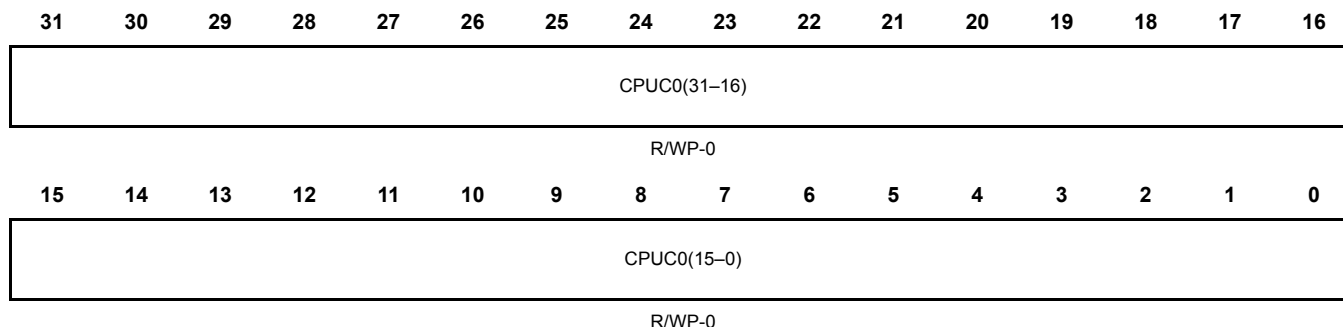
Figure 21-15. RTI Compare Up Counter 0 Register (RTICPUC0) [offset = 0x18h]
