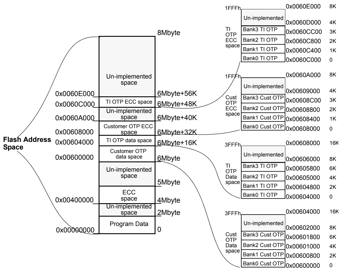
Figure 8-1. Flash Memory Map of F035 Device
