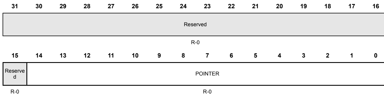
Figure 26-17. DMM Direct Data Mode Pointer Register (DMMDDMPT) [offset = 24h]
