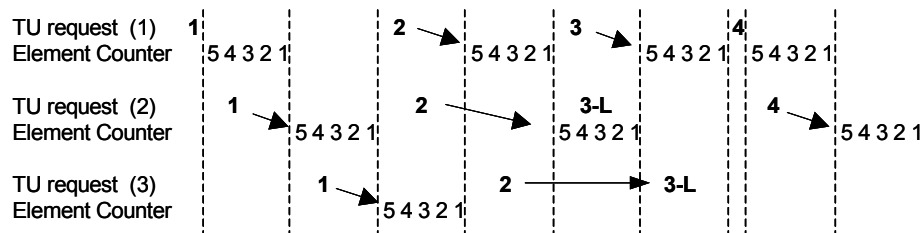
Figure 19-9. Timing Example Including Lost Requests
