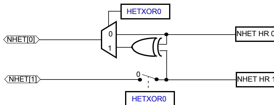
Figure 18-14. XOR-shared HR I/O
