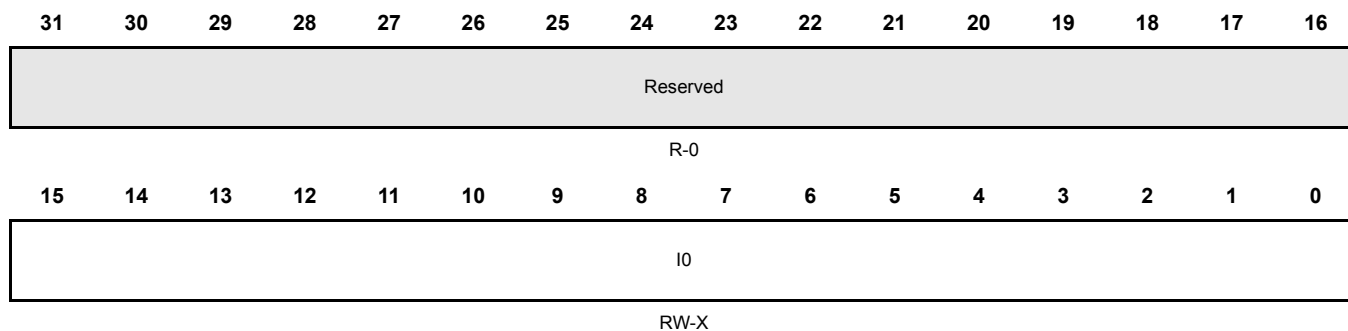
Figure 6-9. Constant Increment Register (I0, I1, I2, I3) [offset = 0x150 - 0x0154]
