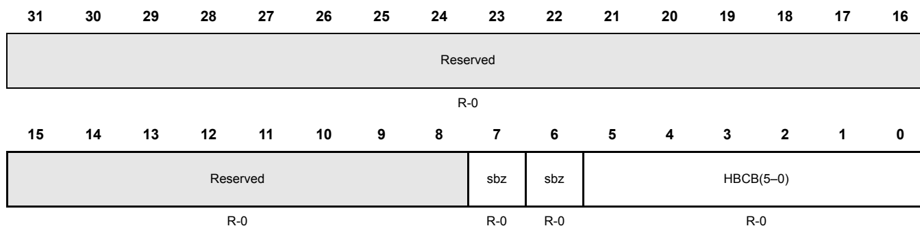
Figure 20-62. HBCB Interrupt Channel Offset Register (HBCBOFFSET) [offset = 0x168]
