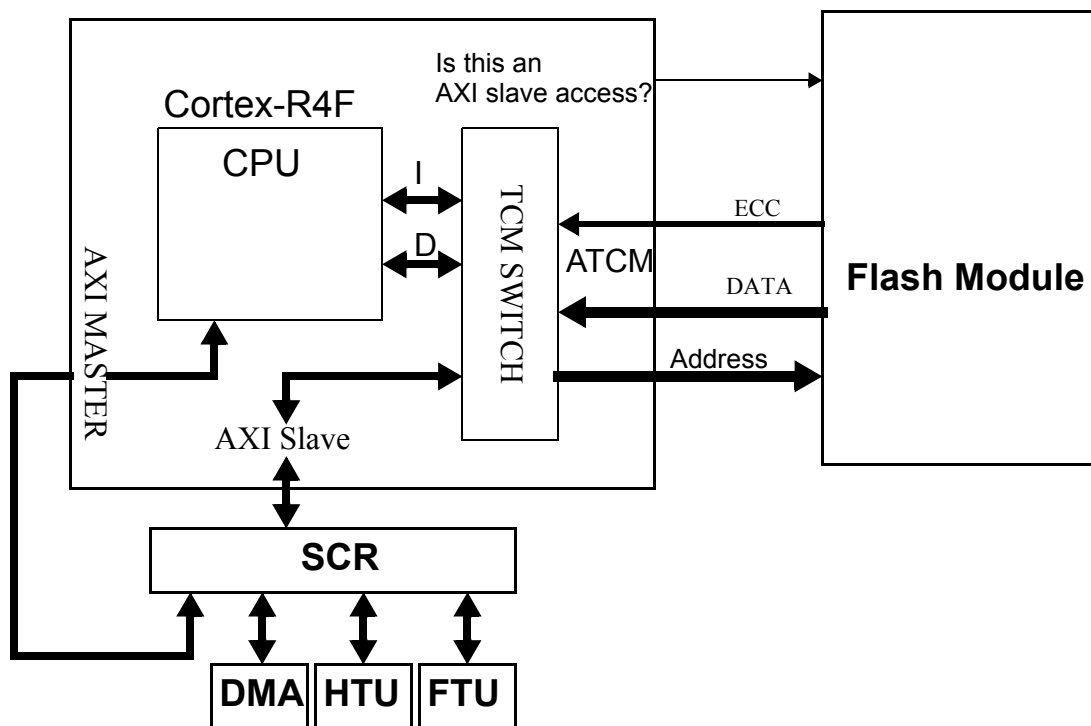
Figure 8-2. CPU ATCM Access and AXI Slave Access Diagram
