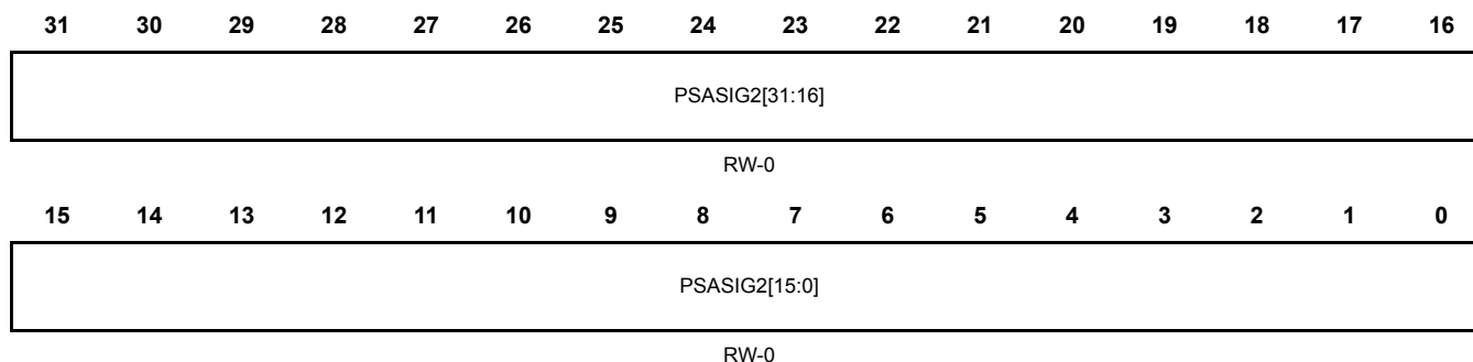
Figure 22-36. Channel 2 PSA signature low register(PSA_SIGREGL2) [offset = 0xA0]
