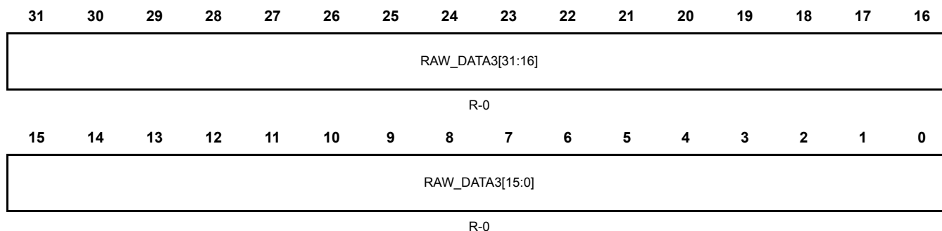
Figure 22-55. Channel 3 Raw Data Low Register(RAW_DATAREGL3) [offset = 0xF8]
