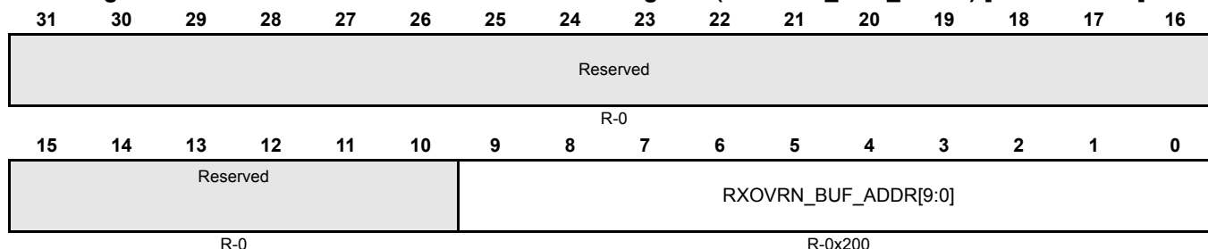
Figure 14-46. RXRAM Overrun Buffer Address Register (RXOVRN_BUF_ADDR) [offset = 130h]
