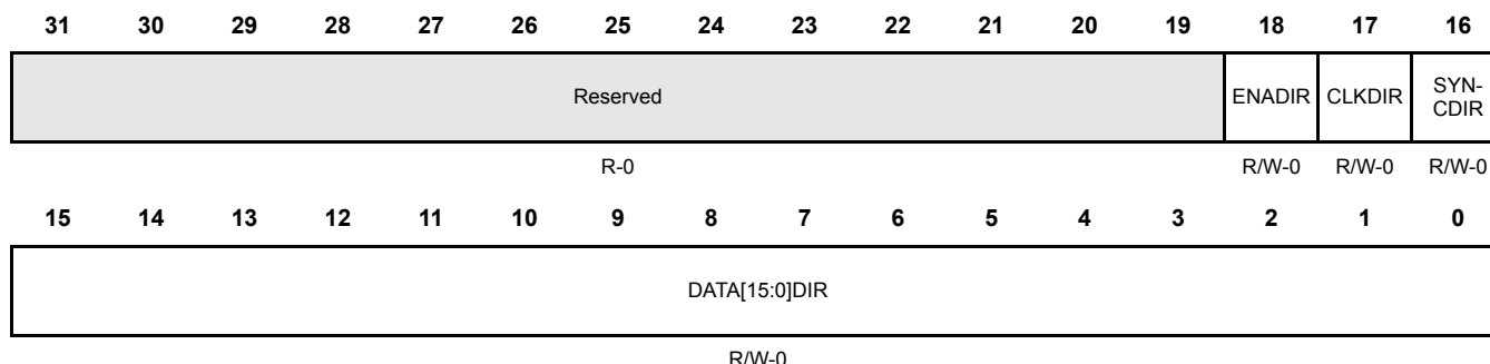
Figure 27-17. RTP Pin Control 1 Register (RTPPC1) [offset = 38h]
