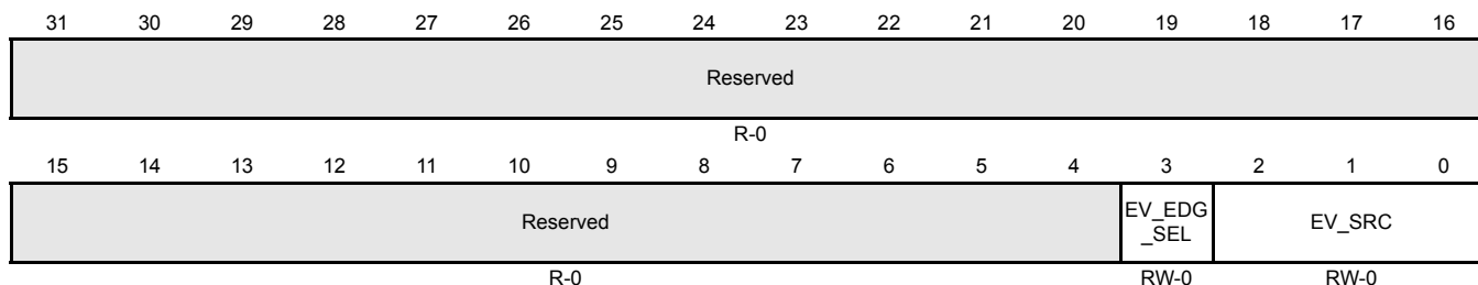
Figure 15-30. ADC Event Group Trigger Source Select Register (ADEVSR) [offset = 0x1C]
