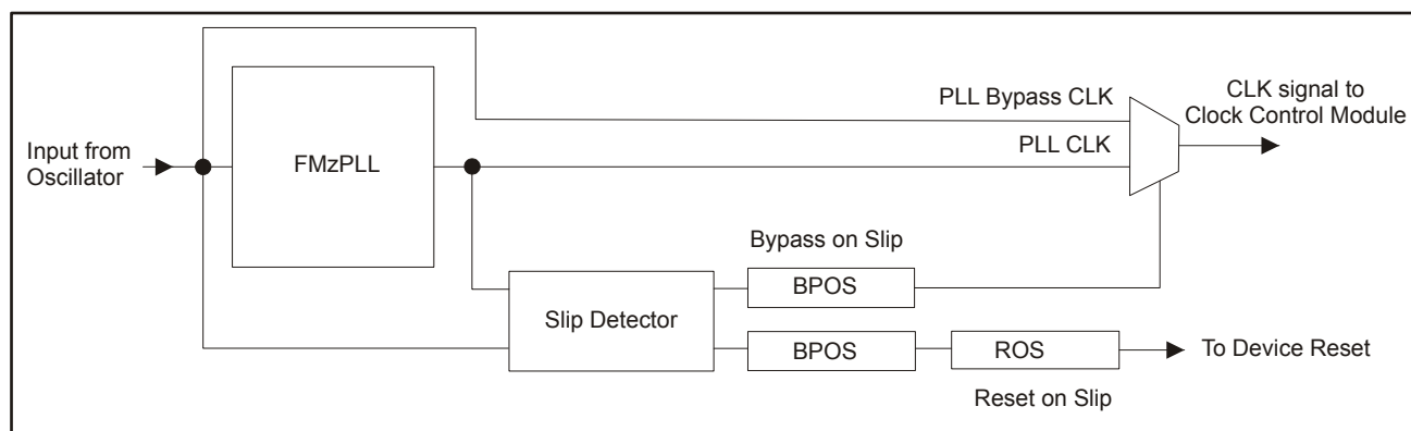
Figure 7-6. PLL Slip Detection & Reset/Bypass Block Diagram
