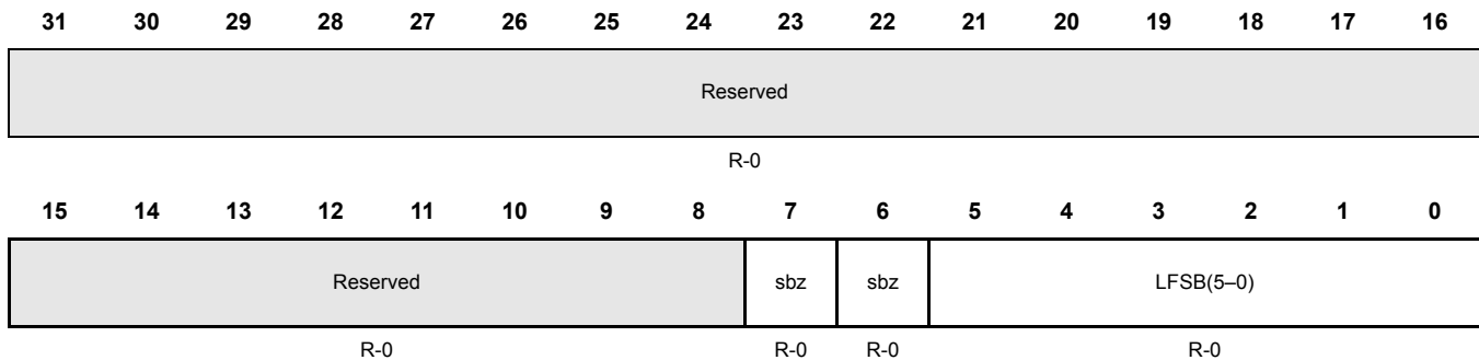
Figure 20-61. LFSB Interrupt Channel Offset Register (LFSBOFFSET) [offset = 0x164]
