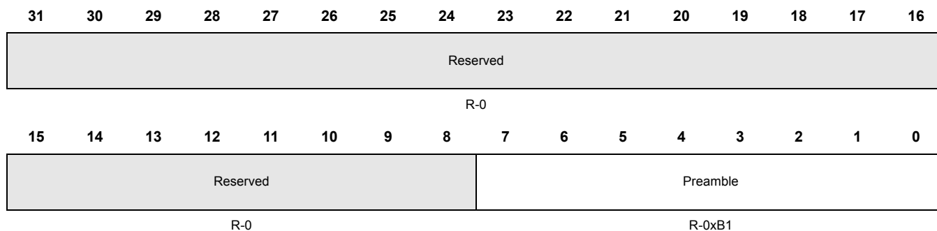
Figure 11-28. POM Component ID 3 Register (POMCPOMPONENTID3) [offset = 0xFFC]
