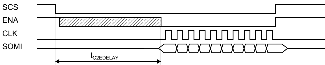
Figure 14-23. Chip-Select-Active-to-ENA-Signal-Active-Timeout
