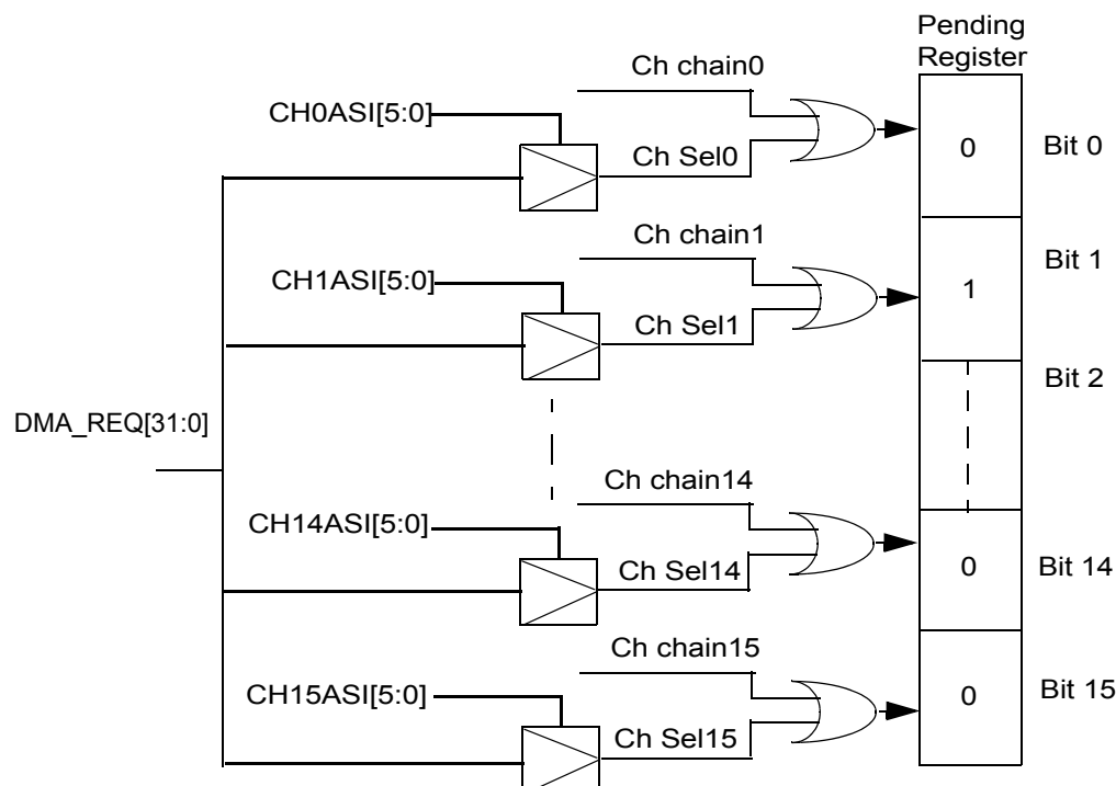
Figure 20-16. Example of Channel Chaining
