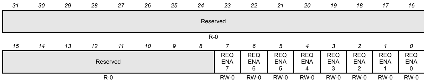
Figure 18-49. Request Enable Set Register (HETREQENS) [0xFFF7B83C]
