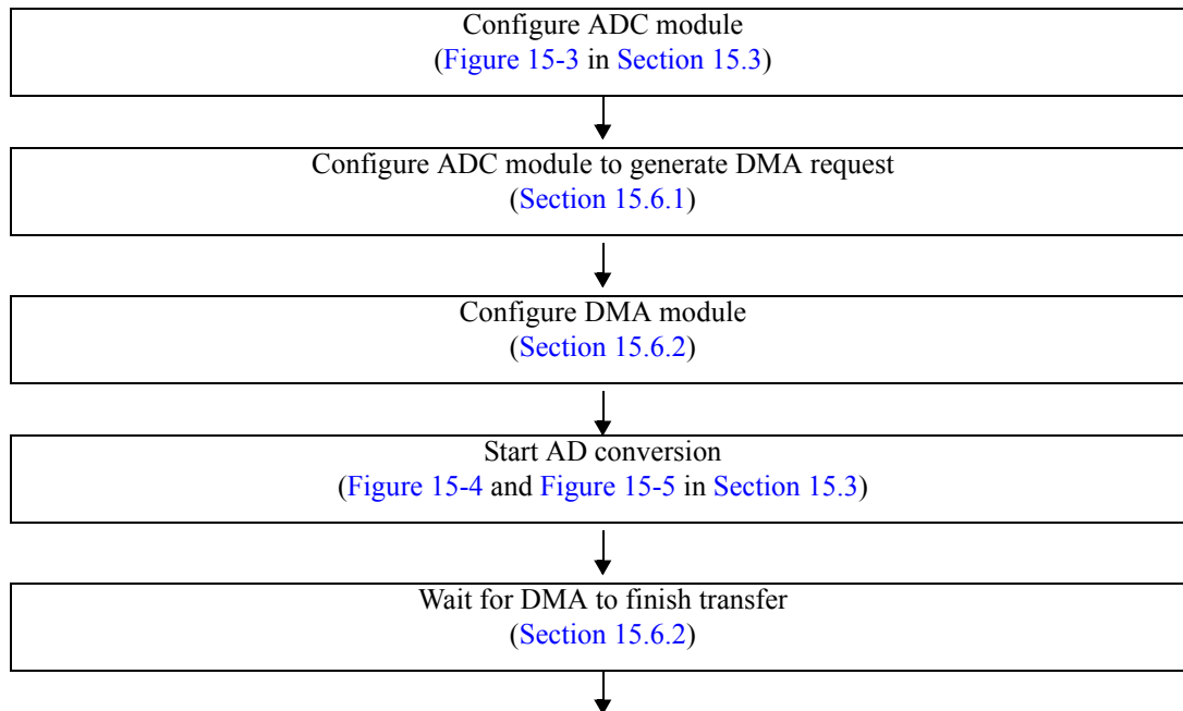
Figure 15-15. Flow Chart for Servicing the ADC by DMA
