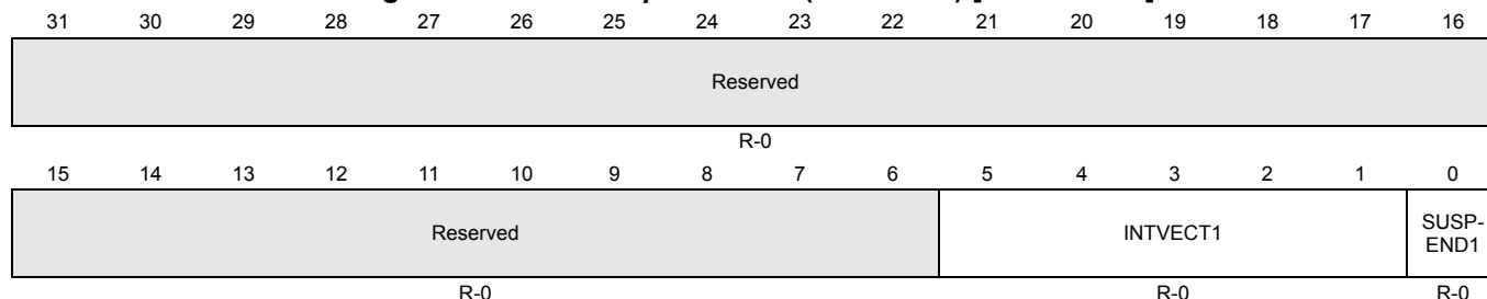
Figure 14-27. Interrupt Vector 1 (INTVECT1) [offset = 64h]
