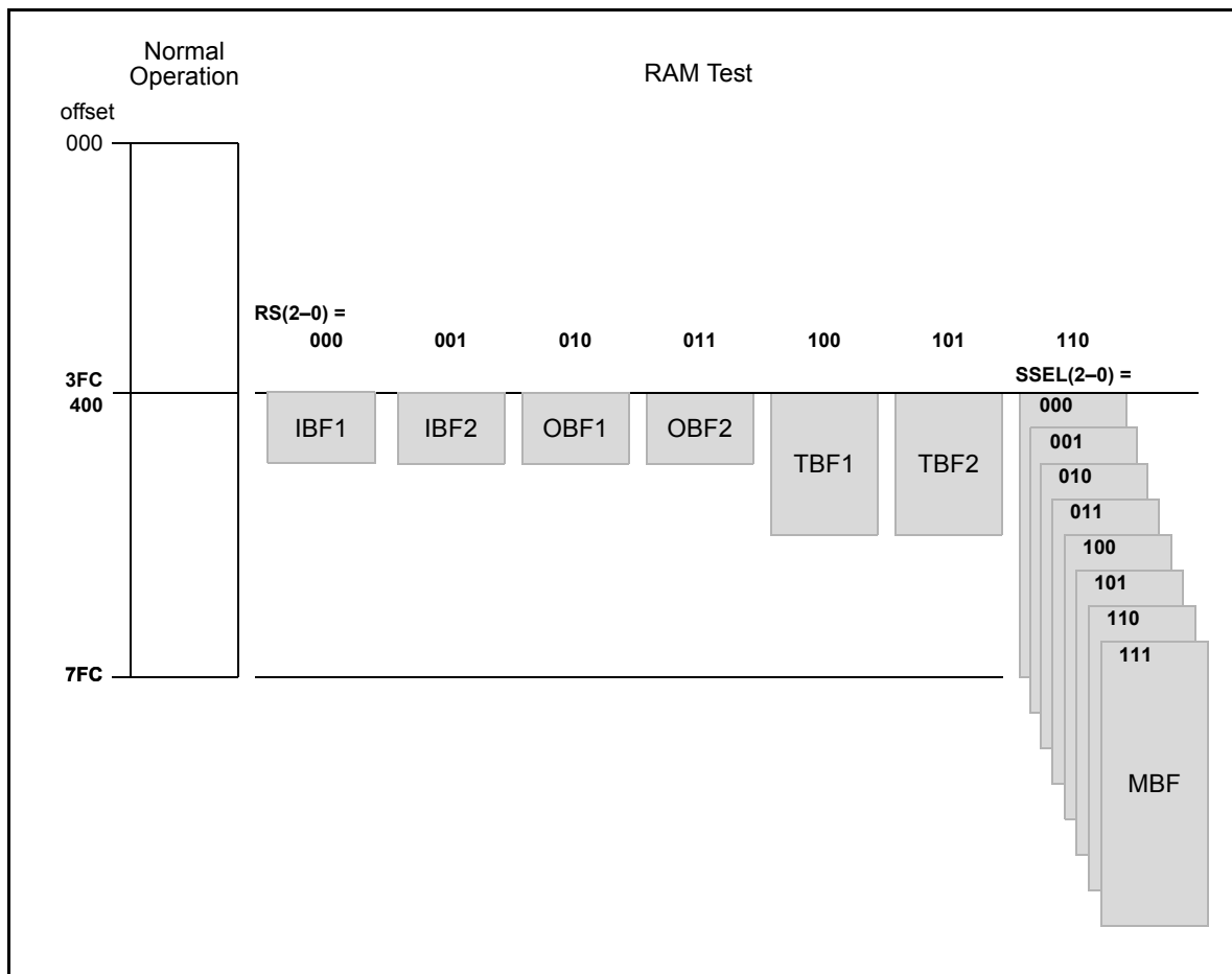
Figure 17-107. Test Mode Access to Communication Controller RAM Blocks
