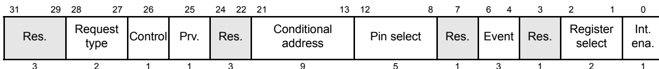
Figure 18-107. ECNT Data Field (D31:D0)
