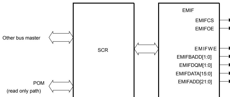
Figure 10-1. EMIF Functional Block Diagram
