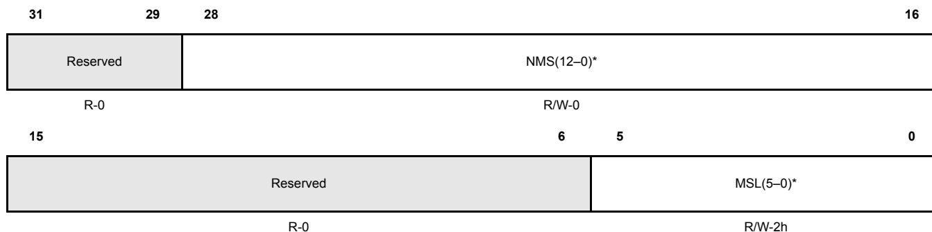
Figure 17-134. GTU Configuration Register 8 (GTUC8) [offset_CC = 0xBC]
