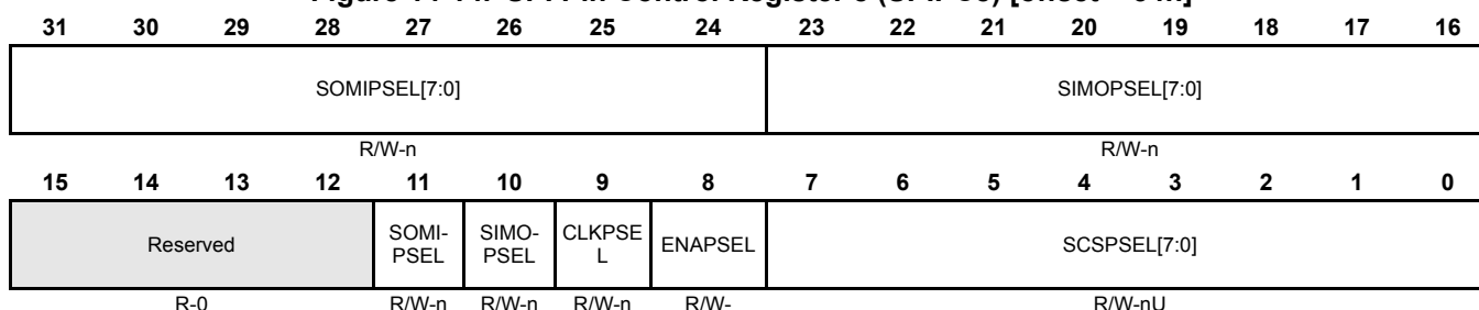
Figure 14-14. SPI Pin Control Register 8 (SPIPC8) [offset = 34h]
