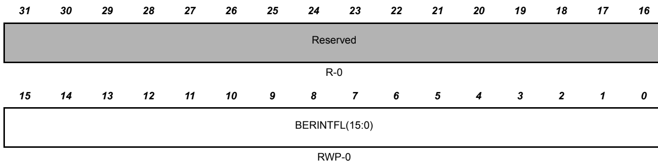
Figure 19-32. BER Interrupt Flag Register (HTU BERINTFL) [offset = 0x48]
