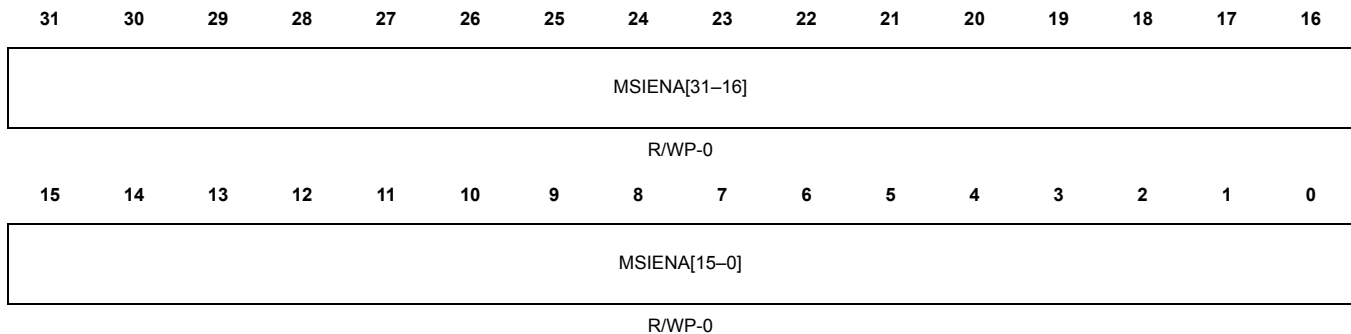
Figure 5-23. Memory Self-Test/Initialization Enable Register (MSIENA) [offset = 0x60]
