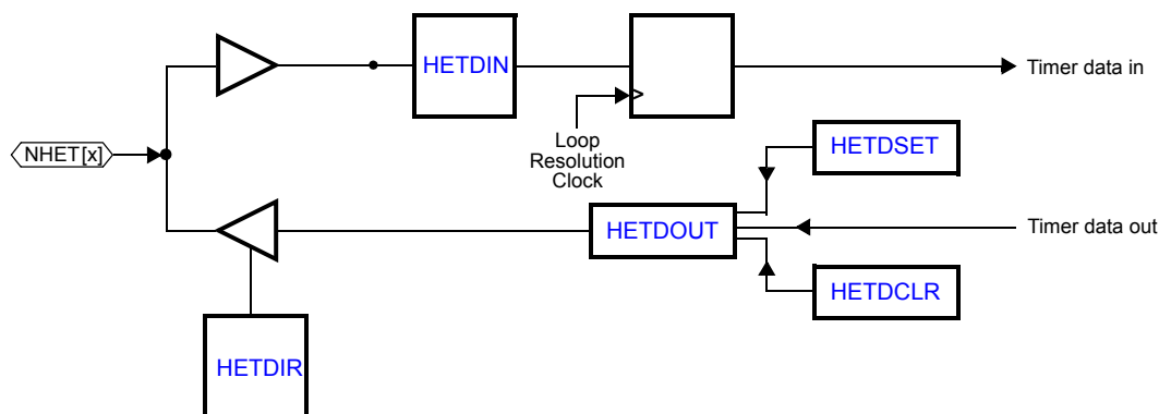
Figure 18-10. NHET Loop Resolution Structure for Each Bit
