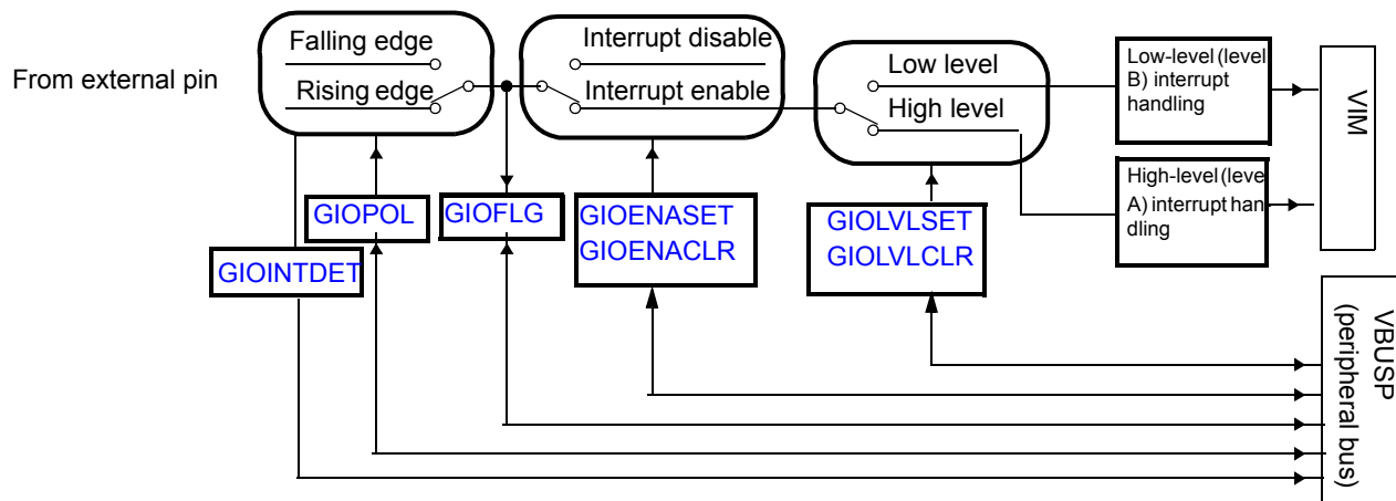
Figure 12-8. External Interrupt Block
