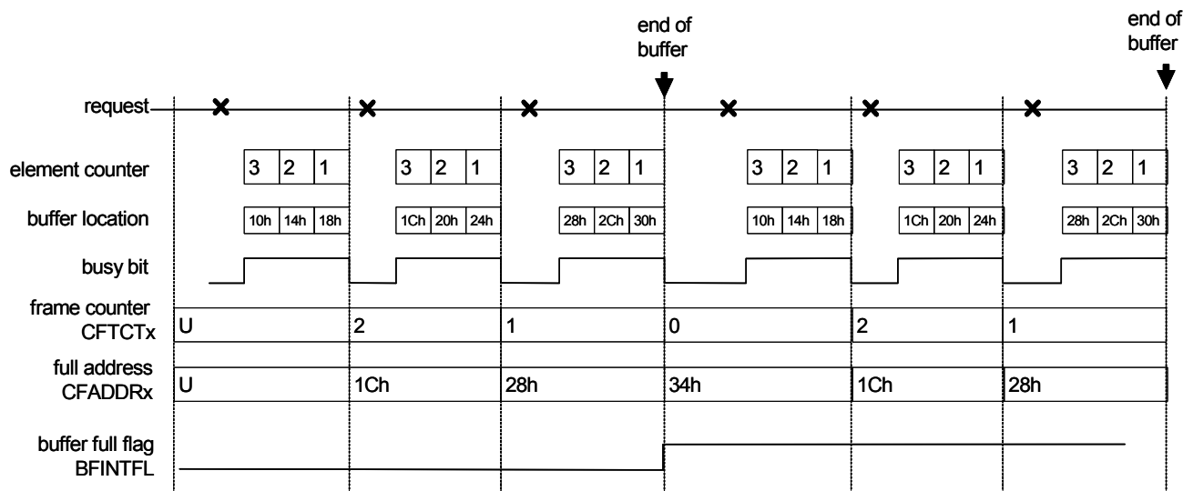
Figure 19-5. Timing Example for Circular Buffer Mode
