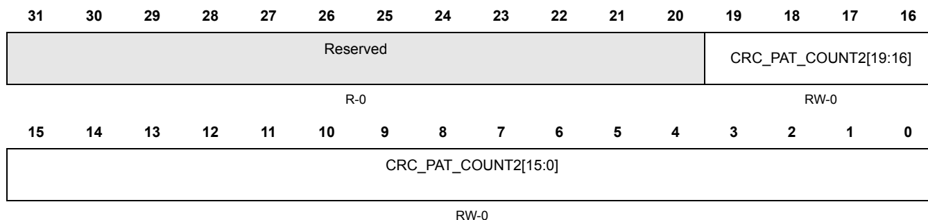
Figure 22-31. CRC Pattern Counter Preload Register2(CRC_PCOUNT_REG2) [offset = 0x80]
