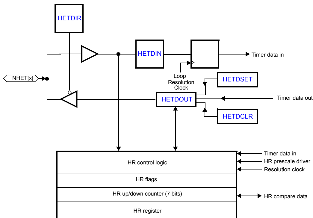
Figure 18-12. HR I/O Architecture
