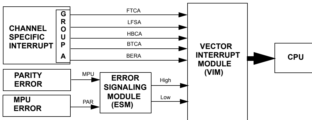
Figure 20-14. DMA Interrupts
