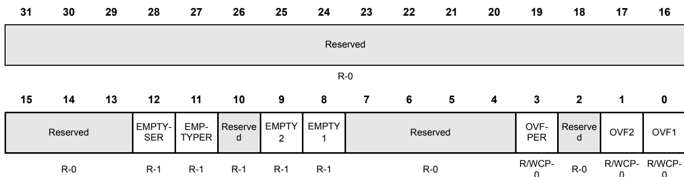
Figure 27-11. RTP Global Status Register (RTPGSR) [offset = 08h]
