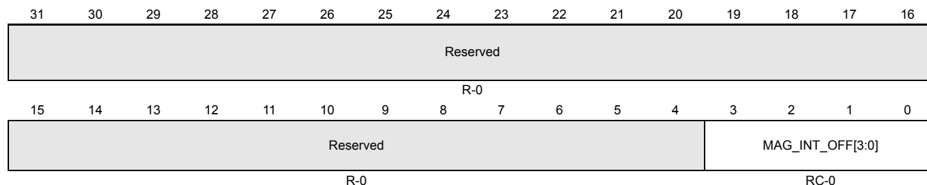
Figure 15-77. ADC Magnitude Compare Interrupt Offset (ADMAGINTOFF) [offset = 0x164]
