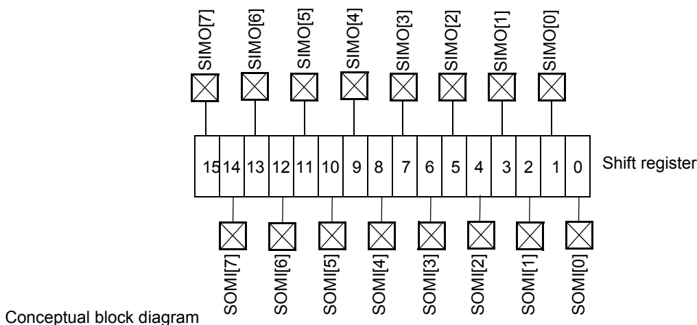
Figure 14-21. eight-data Line Mode (Phase 0, Polarity 0)
