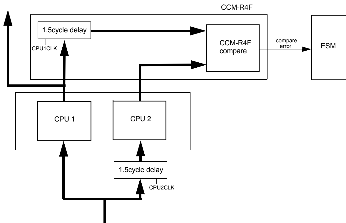
Figure 23-1. Block Diagram
