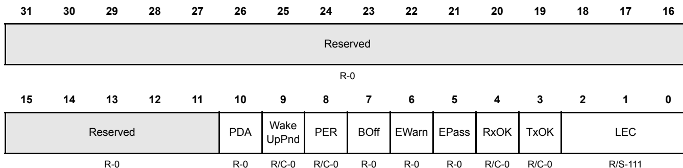
Figure 16-26. Error and Status Register (DCAN ES) [offset = 0x04]
