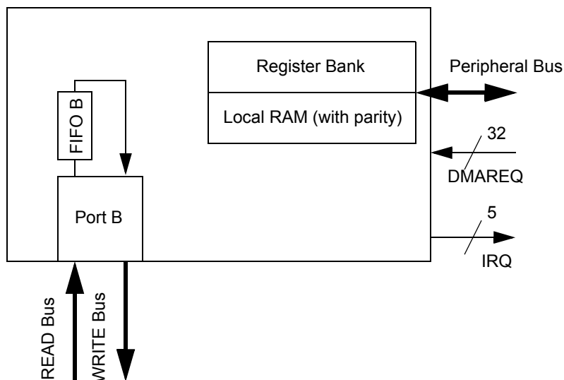
Figure 20-1. DMA Block Diagram
