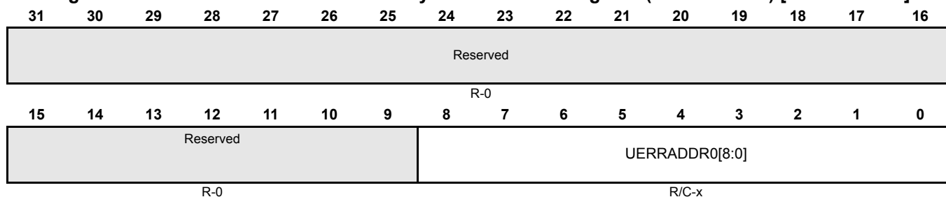
Figure 14-45. TXRAM Uncorrectable Parity Error Address Register (UERRADDR0) [offset = 12Ch]
