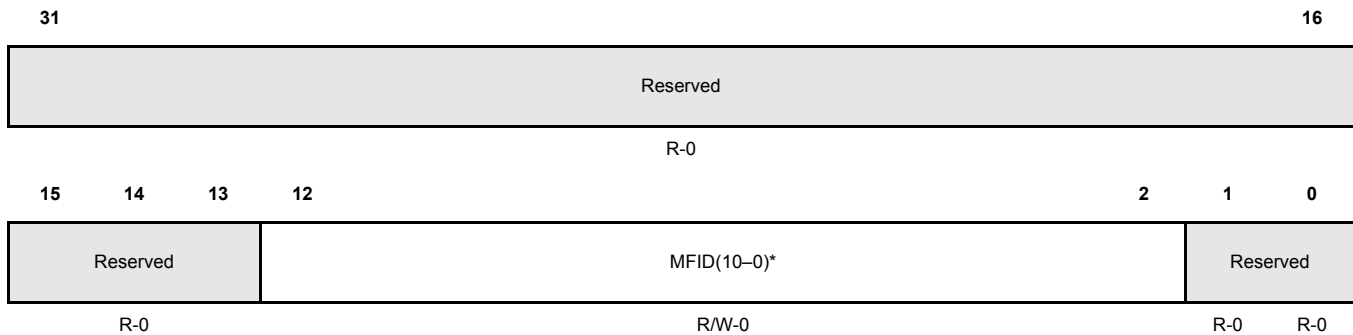
Figure 17-153. FIFO Rejection Filter Mask Register (FRFM) [offset_CC = 0x308]
