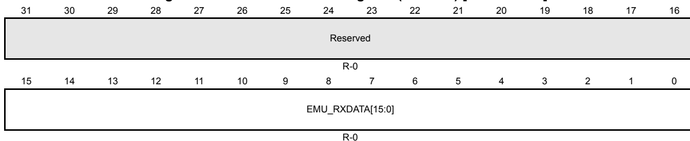
Figure 14-18. SPI Emulation Register (SPIEMU) [offset = 44h]
