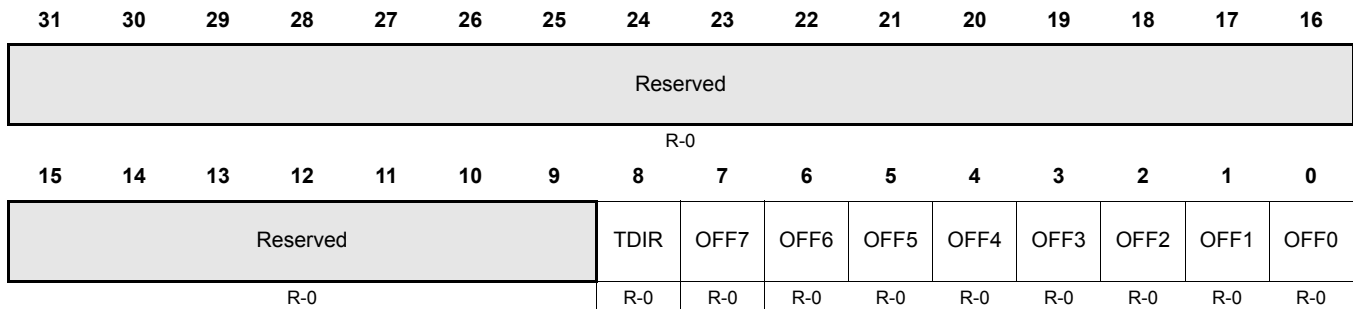
Figure 17-47. Transfer Occurred Offset (TOOFF) [offset_TU = 0x60]
