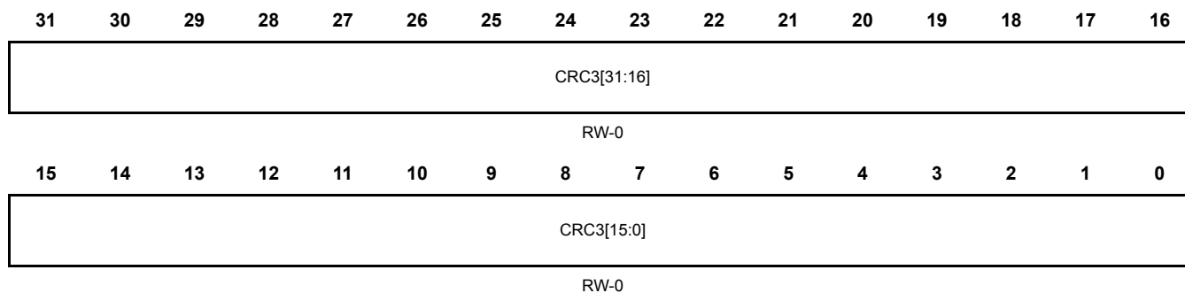
Figure 22-51. Channel 3 CRC value low register(CRC_REGL3) [offset = 0xE8]
