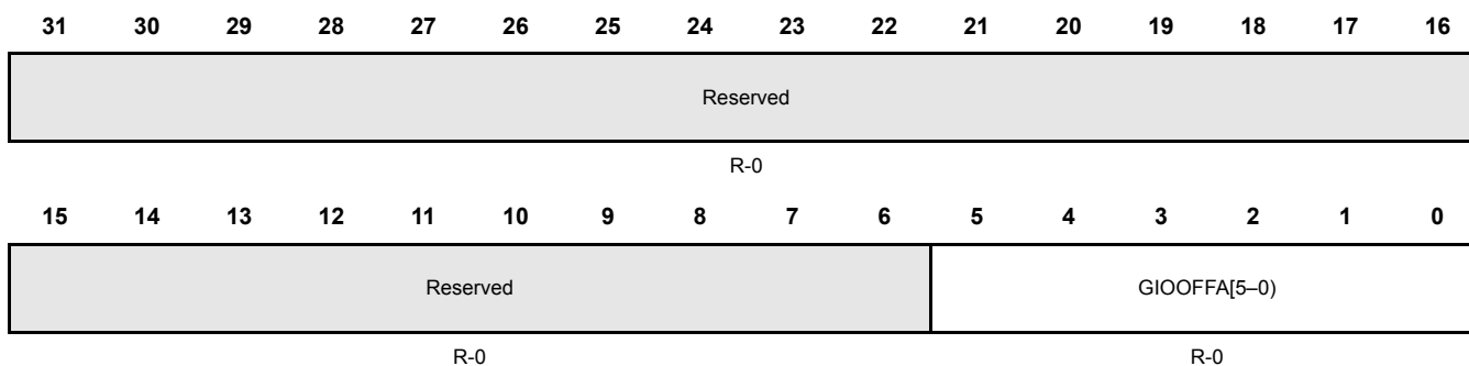
Figure 12-19. GIO Offset A Register (GIOOFFA) [0xFFF7BC24]
