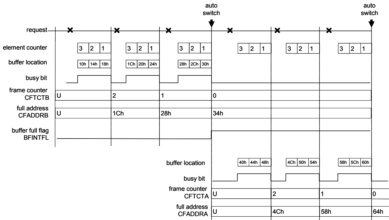
Figure 19-7. Timing Example for Auto Switch Buffer Mode
