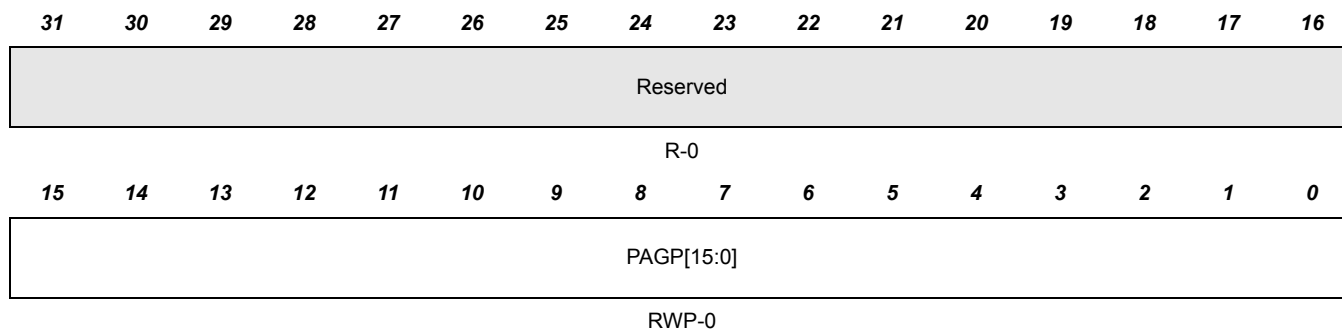
Figure 8-22. Flash Pump Access Control Register 2 (FPAC2 - 0xFFFF8704C)
