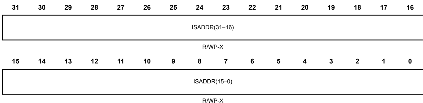
Figure 20-85. Initial Source Address (ISADDR) [offset = 0x000]
