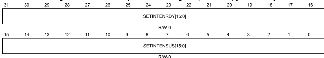
Figure 14-30. TG Interrupt Enable Set Register (TGITENST) [offset = 74h]
