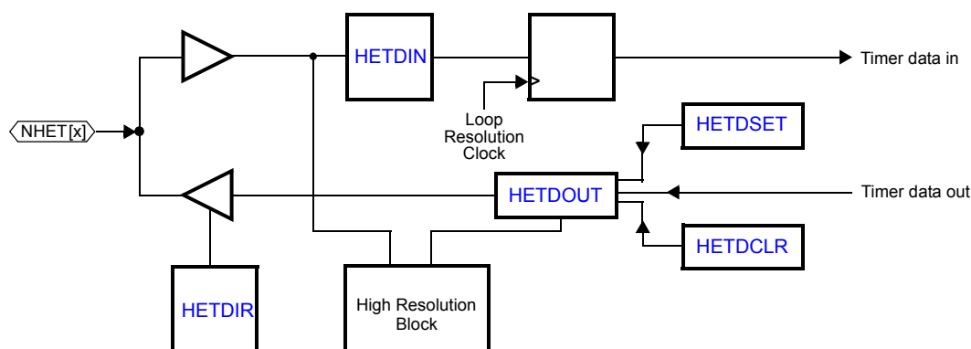
Figure 18-9. I/O Control
