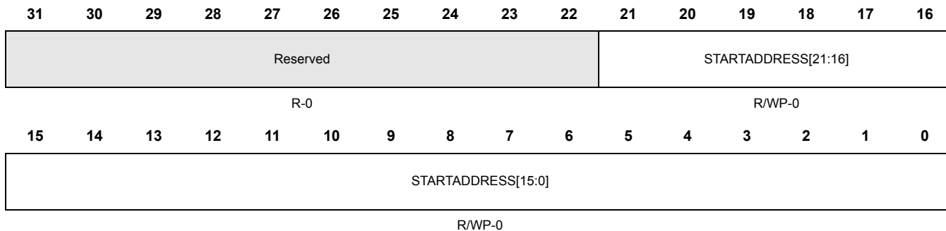
Figure 11-7. POM Overlay Region Start Register x (POMOVLSTARTx) [offset = 0x204, 0x214, ..., 0x3F4]
