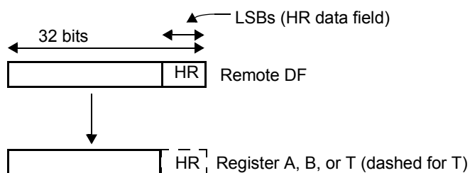
Figure 18-117. MOV32 Move Operation for REMTOREG (Case 11)
