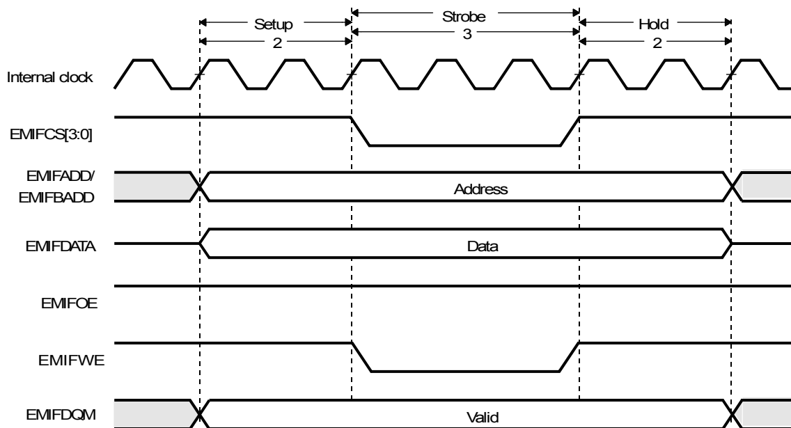
Figure 10-7. Timing Waveform of an Asynchronous Write Cycle in Select Strobe Mode
