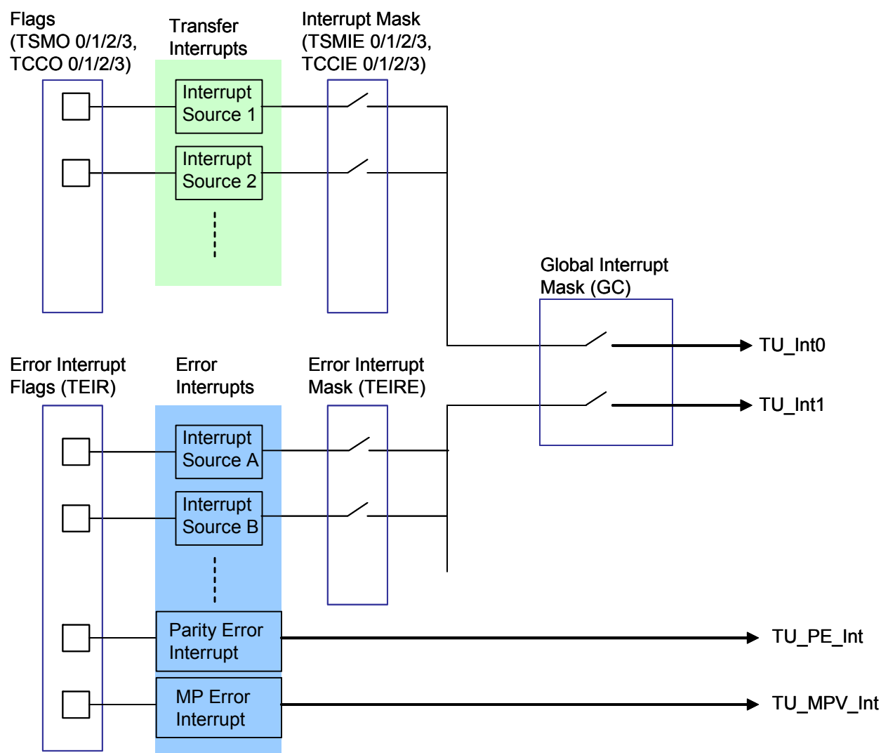
Figure 17-25. Transfer Unit Interrupt Structure
