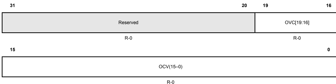
Figure 17-143. Offset Correction Value Register (OCV) [offset_CC = 0x11C]
