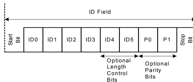
Figure 13-16. ID Field
