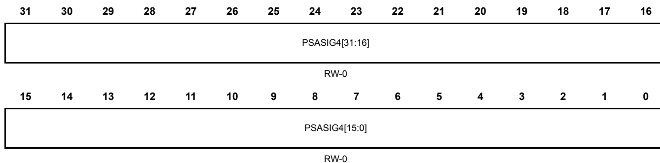
Figure 22-62. Channel 4 PSA signature low register(PSA_SIGREGL4) [offset = 0x120]
