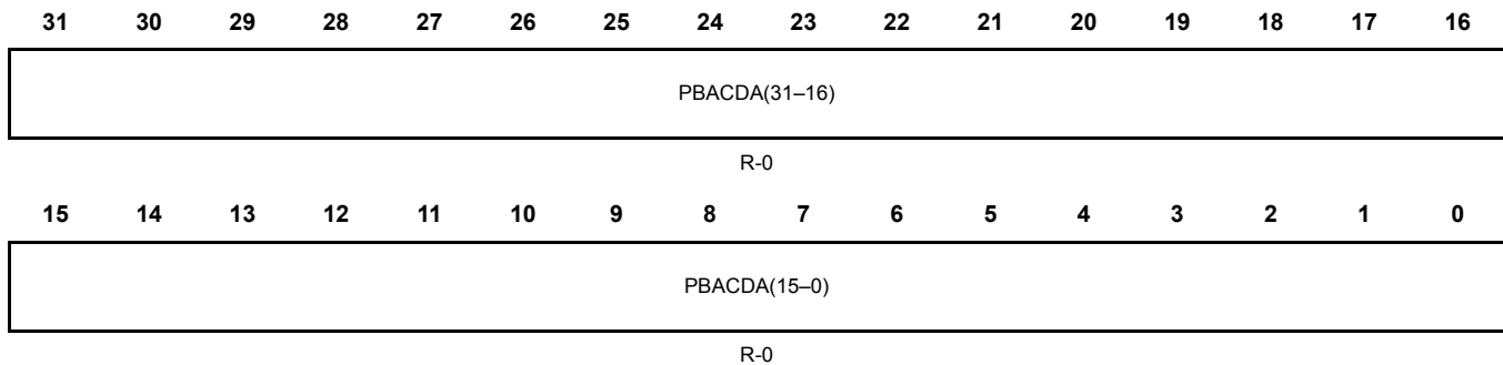
Figure 20-71. Port B Active Channel Destination Address Register (PBACDADDR) [offset = 0x19C]
