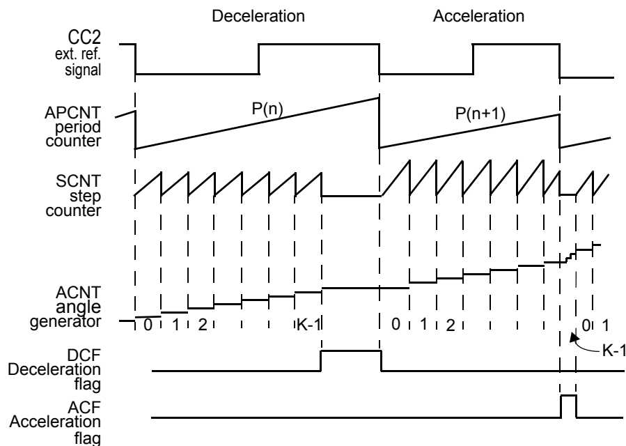
Figure 18-32. ACNT Period Variation Compensations
