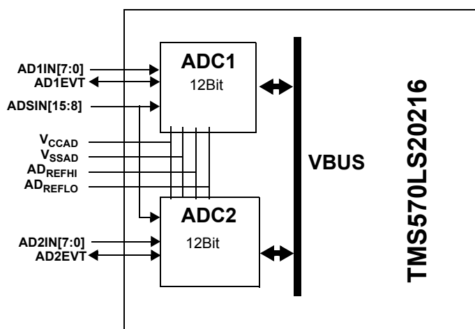
Figure 15-1. Channel Assignments of Two ADC cores
