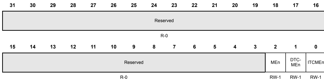
Figure 22-70. Data Bus Selection Register(MCRC_TRACE_BUS_SEL) [offset = 0x140]
