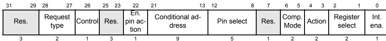
Figure 18-97. DADM64 Data Field (D31:D0)
