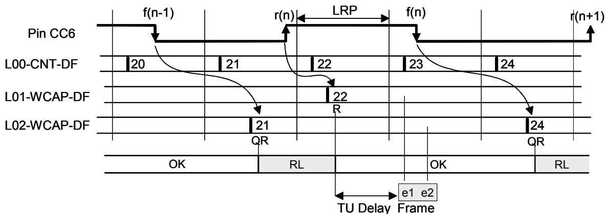
Figure 19-12. Timing Example for two WCAP Instructions
