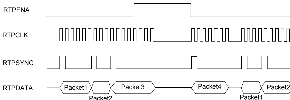
Figure 27-7. RTP Packet Transfer with Sync Signal
