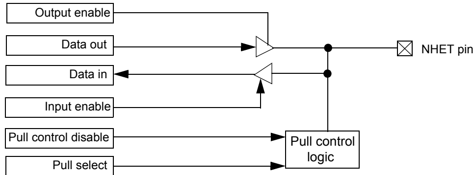
Figure 18-24. I/O Block Diagram Including Pull Control Logic
