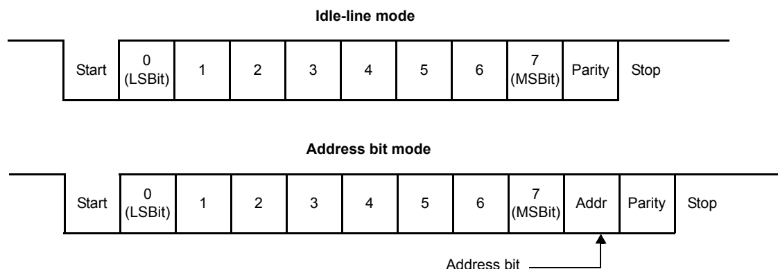
Figure 13-3. Typical SCI Data Frame Formats
