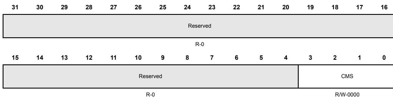
Figure 6-12. Clock-Mux Select Register (CMS) [offset = 0x0168]
