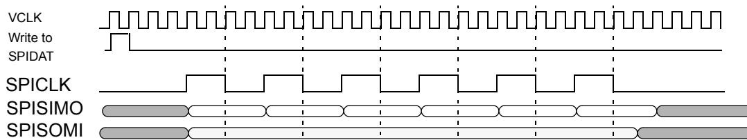
Figure 14-53. SPI/MibSPI Pins during Master mode 3-pin configuration
