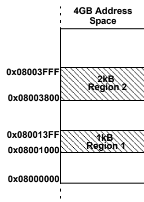
Figure 27-5. Example for Trace Region Setup
