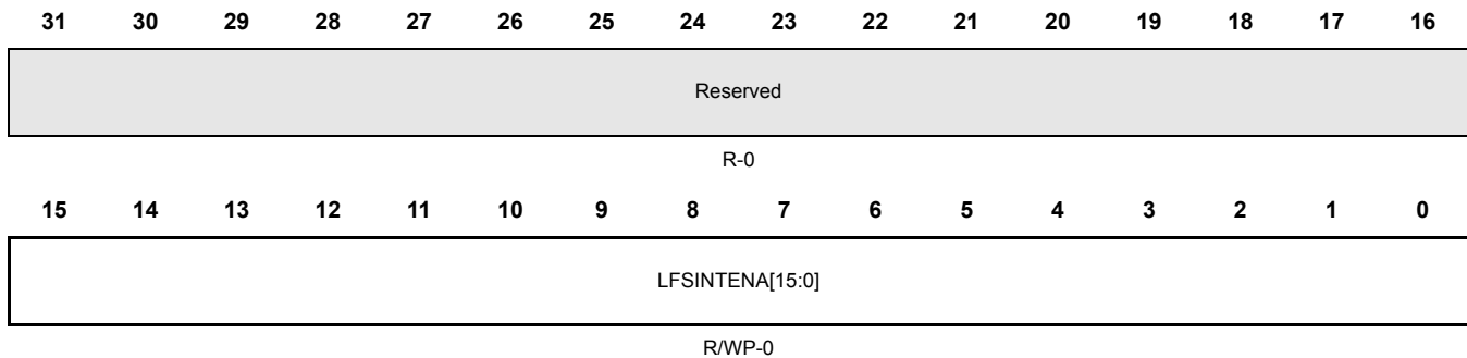
Figure 20-43. LFS Interrupt Enable Set (LFSINTENAS) [offset = 0xEC]
