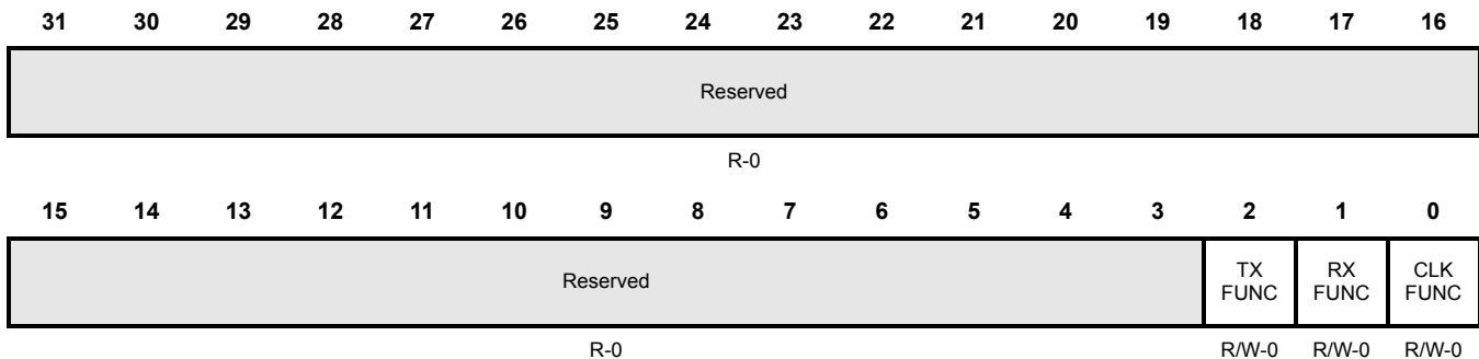
Figure 13-43. SCI Pin I/O Control Register 0 (SCIPIO0) [offset = 0x3C]
