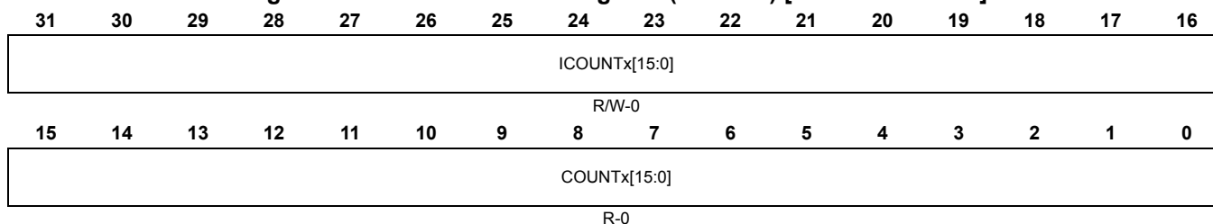
Figure 14-40. DMAxCOUNT Register (ICOUNT) [offset = F8–114h]
