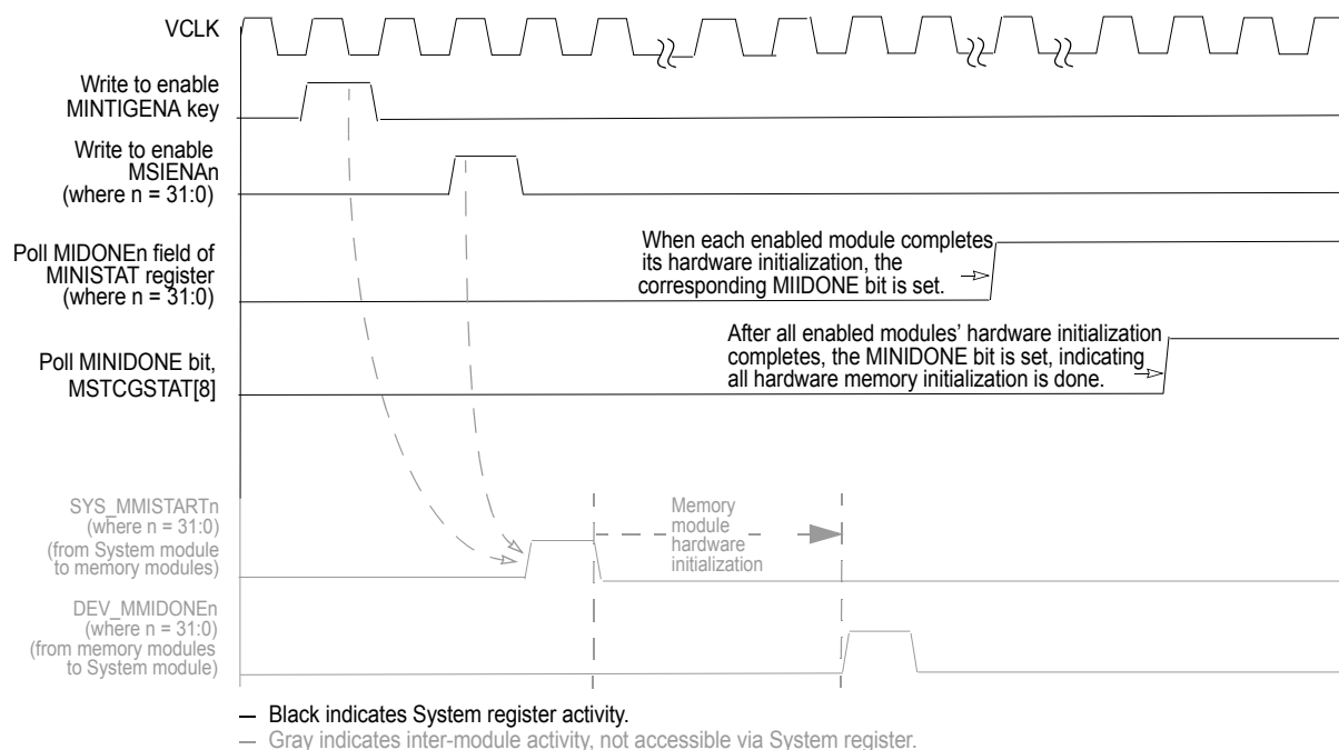
Figure 1-3. Hardware Memory Initialization Protocol
