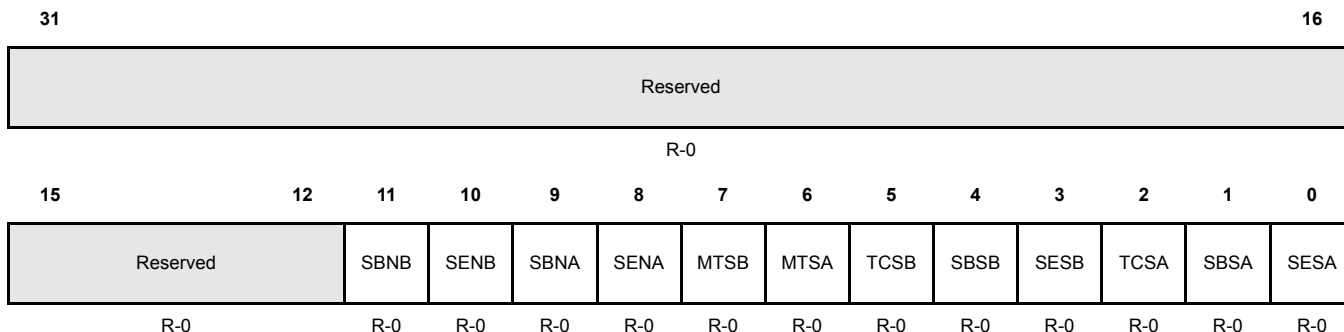
Figure 17-145. Symbol Window and NIT Status Register (SWNIT) [offset_CC = 0x124]
