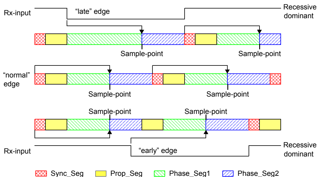
Figure 16-17. Synchronization on Late and Early Edges
