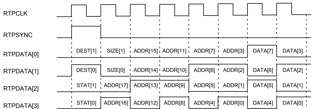
Figure 27-8. Packet Format in Trace Mode
