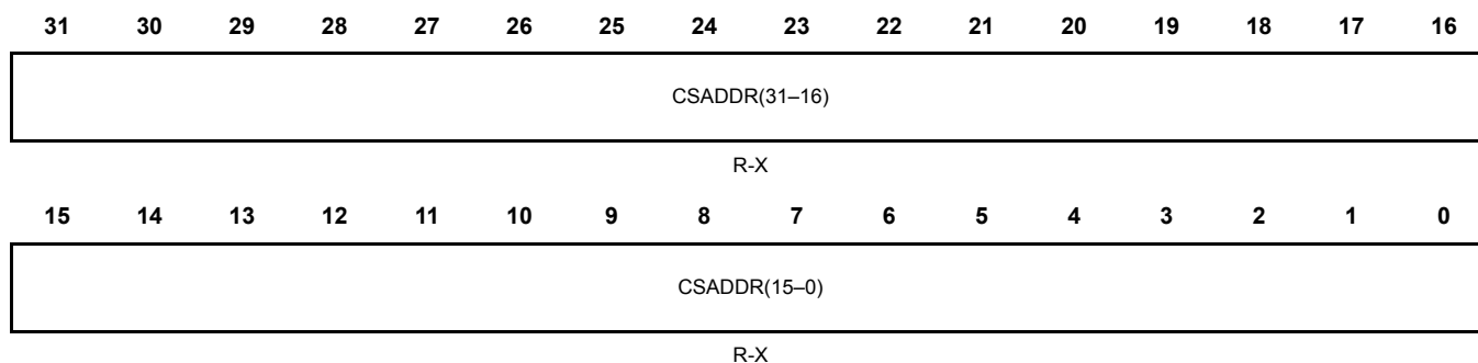
Figure 20-91. Current Source Address Register (CSADDR) [offset = 0x800]
