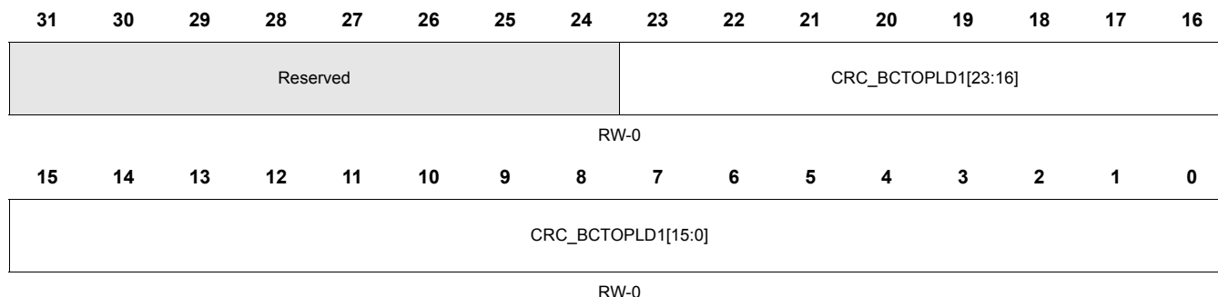
Figure 22-22. CRC Channel 1 Block Complete Timeout Preload Register B(CRC_BCTOPLD1) [offset = 0x50]
