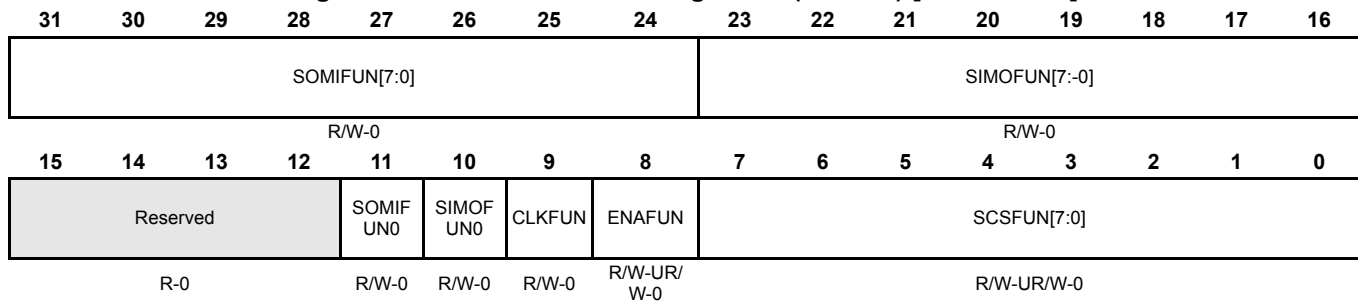
Figure 14-6. SPI Pin Control Register 0 (SPIPC0) [offset = 14h]
