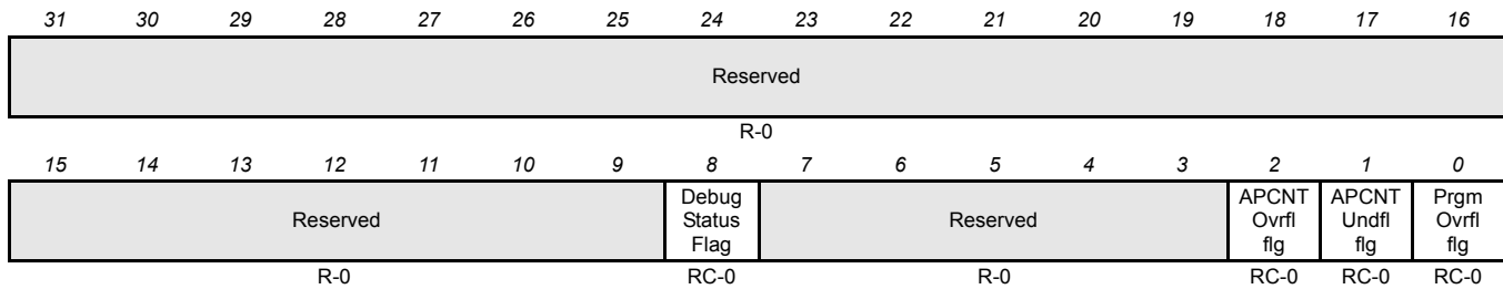
Figure 18-44. Exception Control Register 2 (HETEXC2) [0xFFF7B820]
