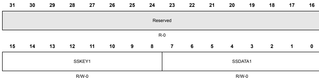
Figure 5-34. System Software Interrupt Request 1 Register (SSIR1) [offset = 0xB0]
