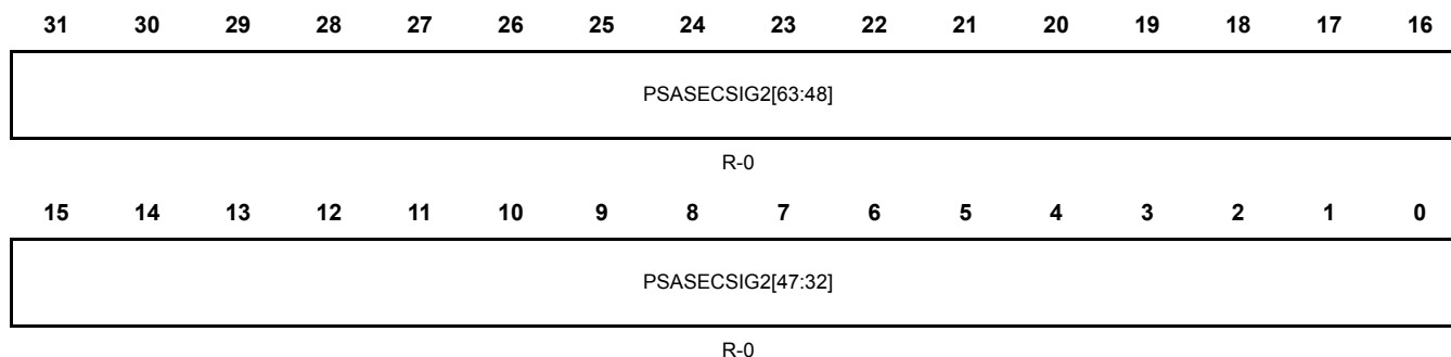
Figure 22-41. Channel 2 PSA sector signature high register(PSA_SECSIGREGH2) [offset = 0xB4]
