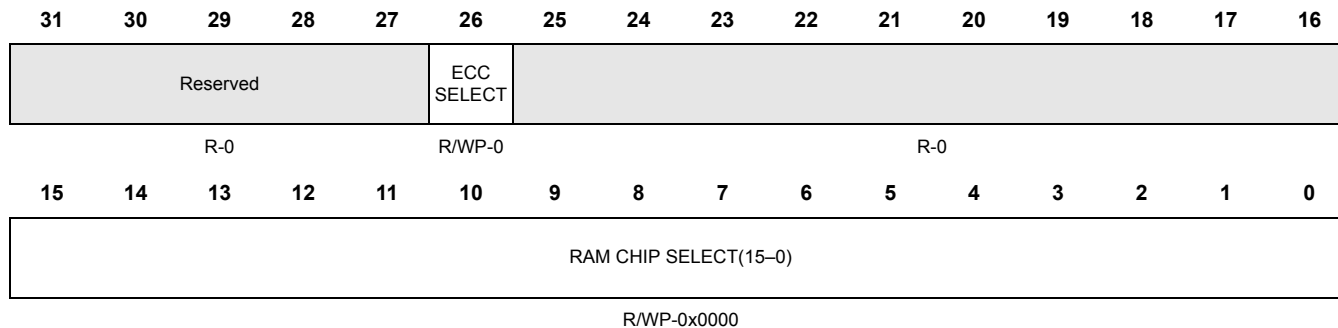
Figure 4-11. TCRAM Wrapper Test Mode Vector Register (RAMADDRDECVECT) [offset = 0x38]
