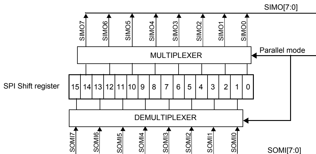
Figure 14-15. Block Diagram Shift Register, LSB First
