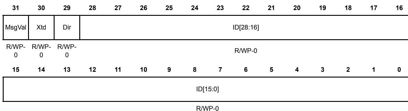
Figure 16-47. IF2 Arbitration Register (DCAN IF2ARB) [offset = 0x128]
