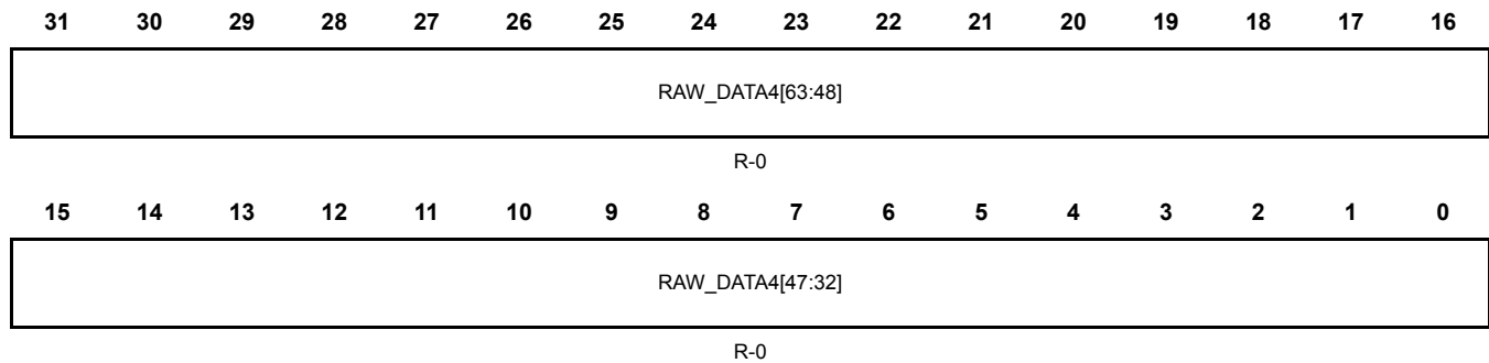
Figure 22-69. Channel 4 Raw Data High Register(RAW_DATAREGH4) [offset = 0x13C]
