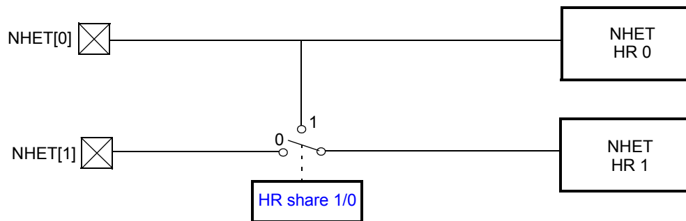
Figure 18-13. Example of HR Structure Sharing for NHET Pins 0/1
