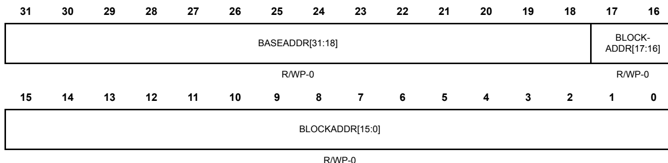
Figure 26-19. DMM Destination x Region 1 (DMMDESTxREG1) [offset = 2Ch, 3Ch, 4Ch, 5Ch]
