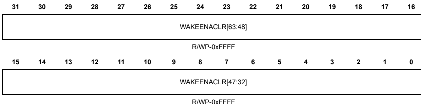
Figure 24-29. Wake-Up Enable Clear Register 1 (WAKEENACLR1) [0xFFFFFE64]
