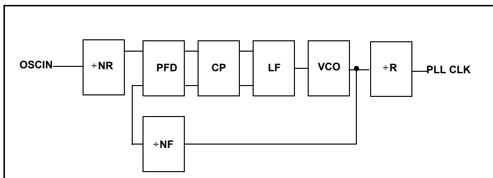
Figure 7-12. Basic PLL Circuit
