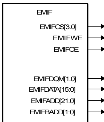
Figure 10-2. EMIF Asynchronous Interface
