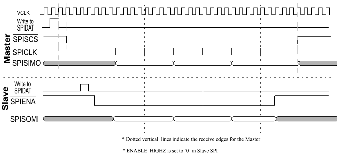
Figure 14-56. SPI/MibSPI pins during Master/Slave mode with 5-pin configuration
