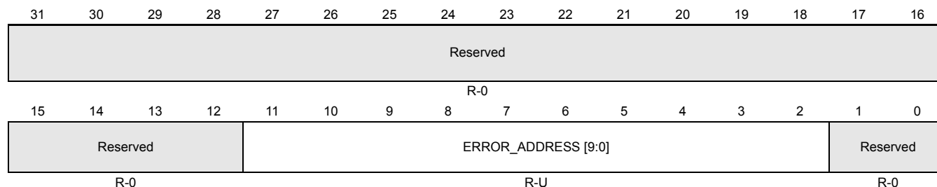
Figure 15-85. ADC Parity Error Address (ADPARADDR) [offset = 0x184]
