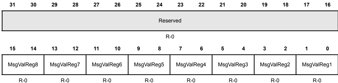
Figure 16-39. Message Valid X Register (DCAN MSGVAL X) [offset = 0xC0]
