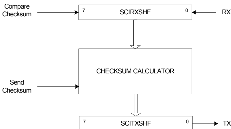
Figure 13-20. Checksum Compare and Send for Extended Frames
