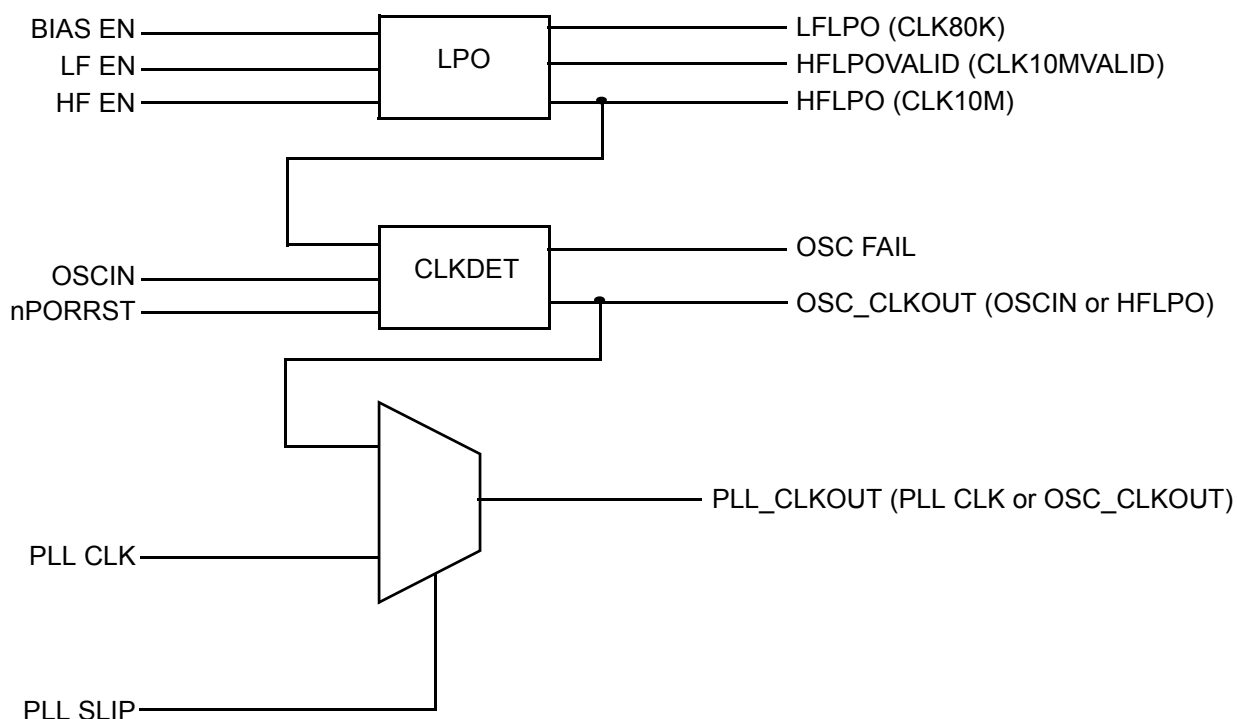
Figure 2-2. Low Power Oscillator/Clock monitor module block diagram
