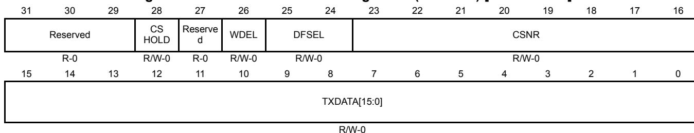
Figure 14-16. SPI Transmit Data Register 1 (SPIDAT1) [offset = 3Ch]
