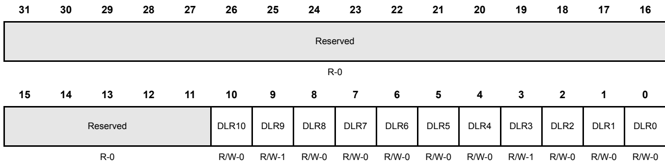
Figure 6-11. Datalogger Register (DLR) [offset = 0x0164]
