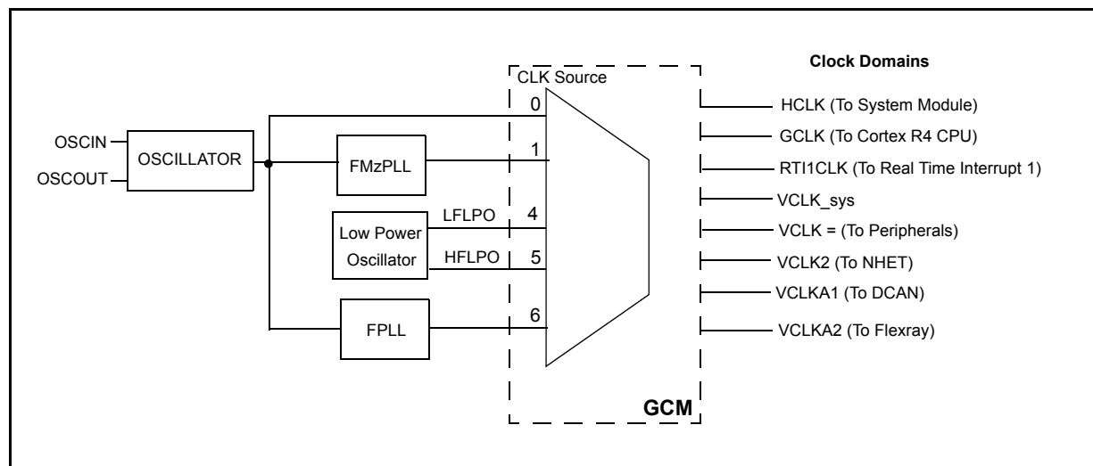
Figure 7-1. Global Clock Module Block Diagram
