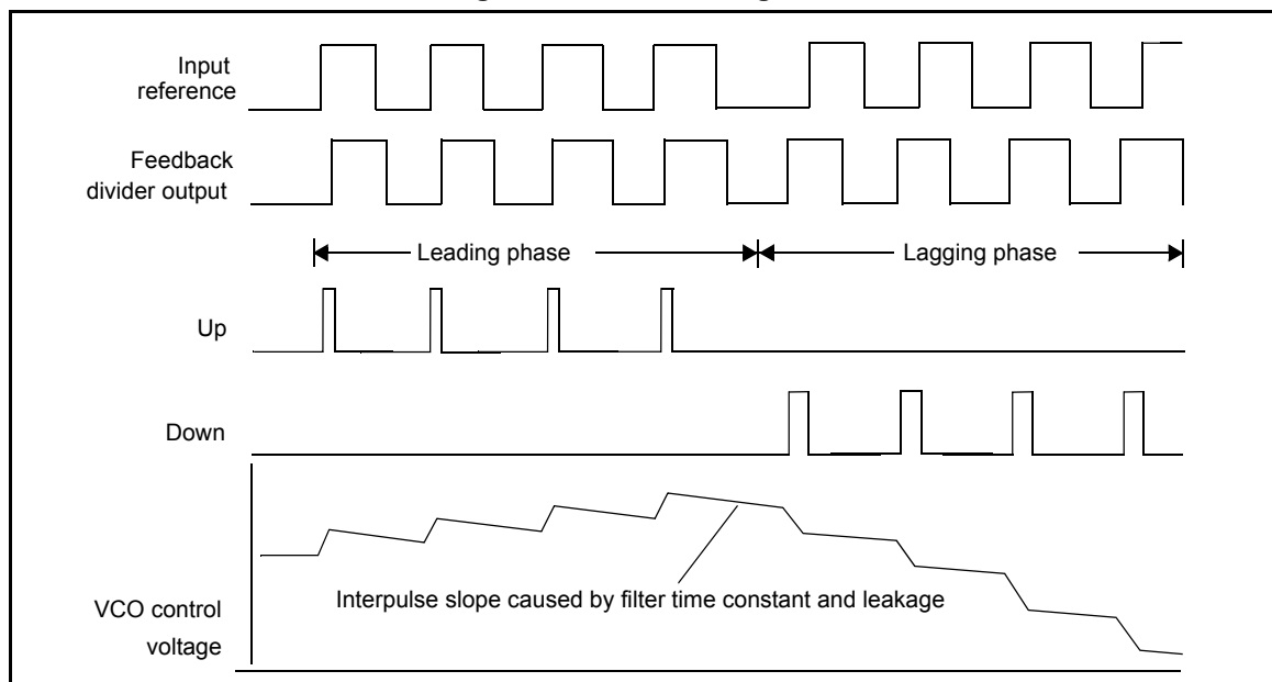
Figure 7-4. PFD Timing
