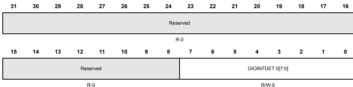
Figure 12-12. GIO Interrupt Detect Register (GIOINTDET) [0xFFF7BC08]
