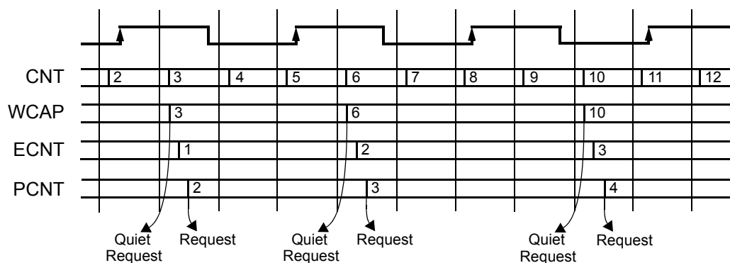
Figure 19-14. Field Addresses of the WCAP, ECNT, PCNT Example
