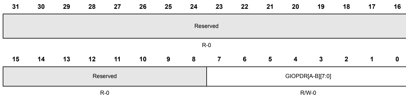
Figure 12-28. GIO Open Drain Registers [A-B][7:0] (GIOPDR[A-B][7:0])[0xFFF7BC48, 0xFFF7BC68]
