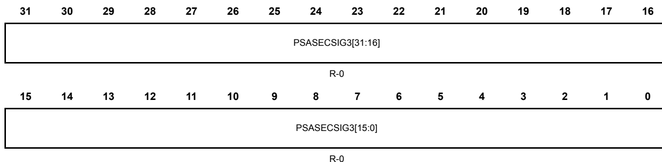
Figure 22-53. Channel 3 PSA sector signature low register(PSA_SECSIGREGL3) [offset = 0xF0]
