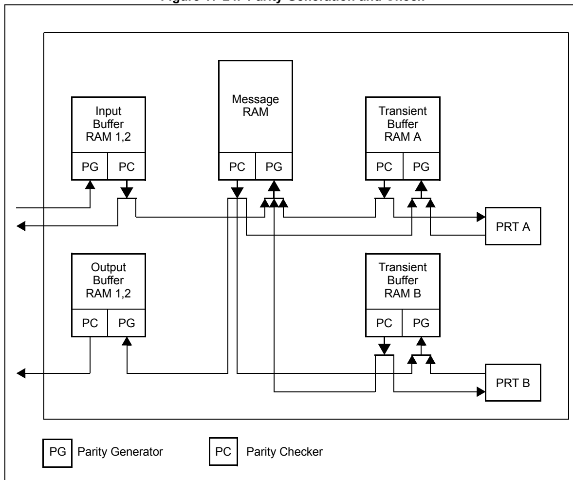
Figure 17-24. Parity Generation and Check
