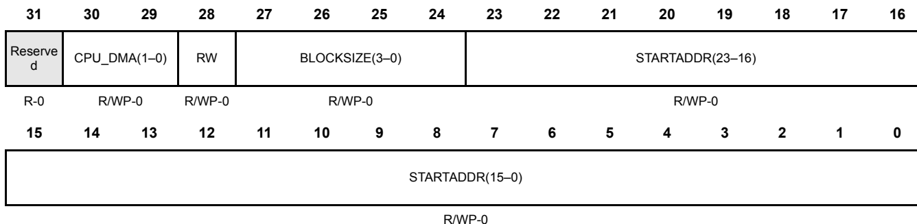
Figure 27-14. RTP Peripheral Trace Region [1:2] Register (RTPPERREG[1:2]) [offset = 24h, 28h]
