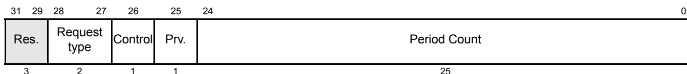
Figure 18-124. PCNT Data Field (D31:D0)
