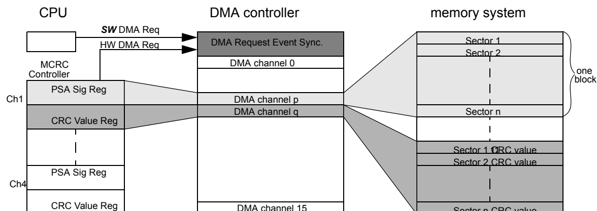
Figure 22-4. AUTO Mode With Software CPU Trigger
