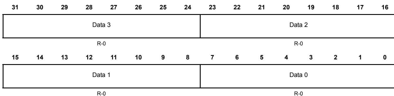
Figure 16-58. IF3 Data A Register (DCAN IF3DATA) [offset = 0x150]
