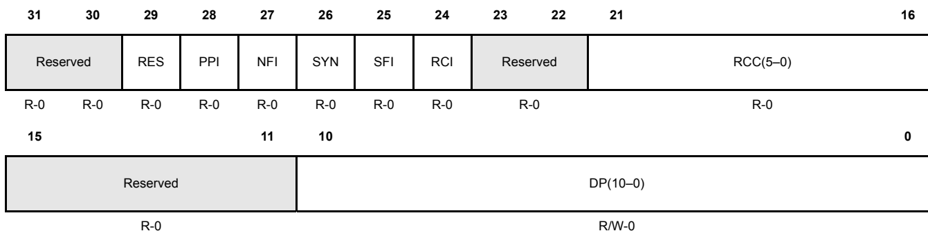
Figure 17-182. Read Header Section Register 3 (RDHS3) [offset_CC = 0x708]
