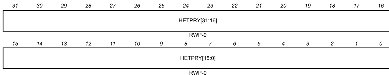
Figure 18-45. Interrupt Priority Register (HETPRY) [0xFFF7B824]
