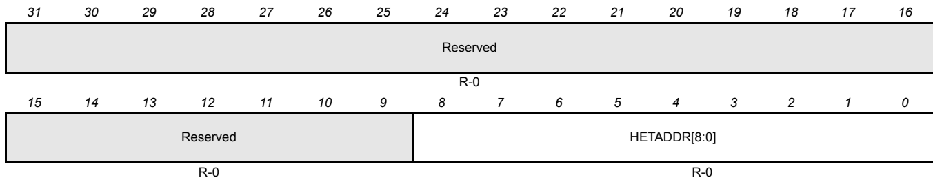
Figure 18-38. NHET Current Address (HETADDR) [0xFFF7B808]
