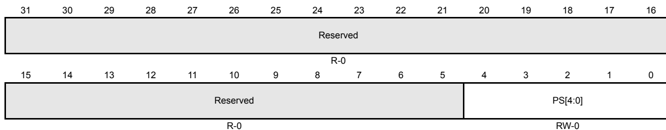
Figure 15-25. ADC Clock Control Register (ADCLOCKCR) [offset = 0x8]
