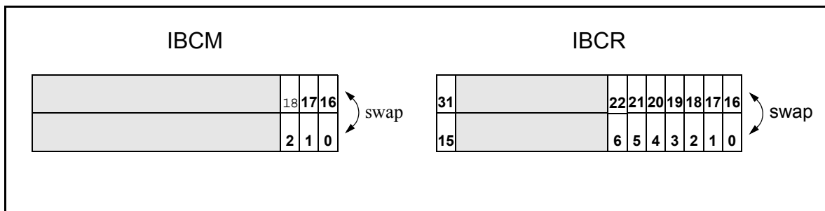
Figure 17-17. Swapping of IBCM and IBCR Bits
