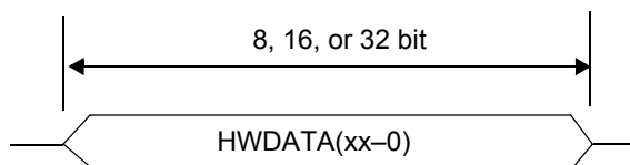
Figure 26-3. Direct Data Mode Packet Format
