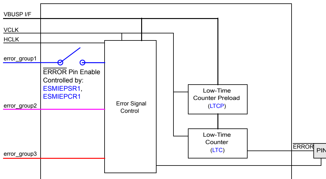
Figure 25-2. Error Signal Handling
