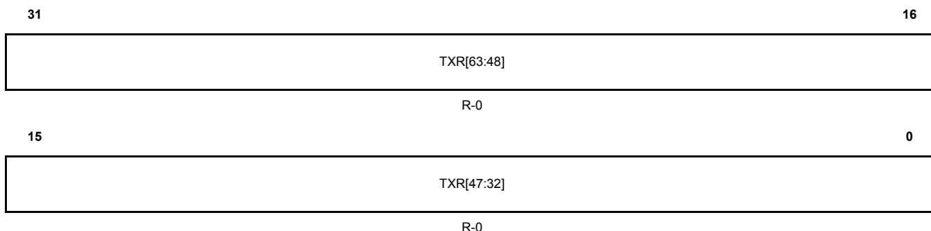
Figure 17-161. Transmission Request Register 2 (TXRQ2) [offset_CC = 0x324]
