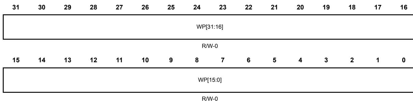
Figure 20-68. Watch Point Register (WPR) [offset = 0x184]
