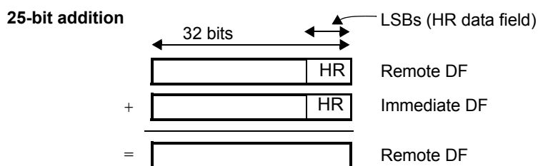
Figure 18-77. ADCNST Operation If Remote Data Field[31:7] Is Not Zero
