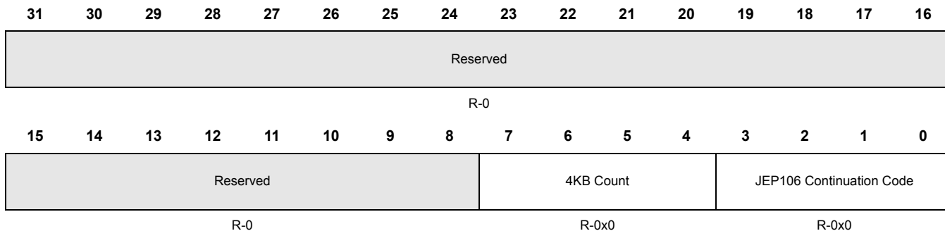
Figure 11-17. POM Peripheral ID 4 Register (POMPERIPHERALID4) [offset = 0xFD0]
