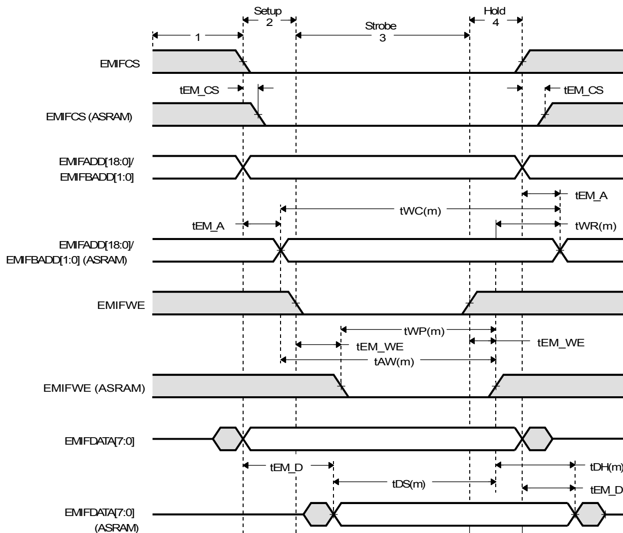
Figure 10-13. Timing Waveform of an ASRAM Read with PCB Delays
