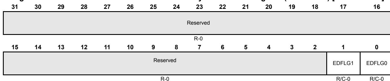
Figure 14-43. Multi-buffer RAM Uncorrectable Parity Error Status Register (UERRSTAT) [offset = 124h]
