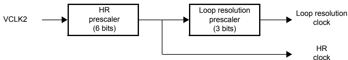
Figure 18-8. Prescaler Configuration
