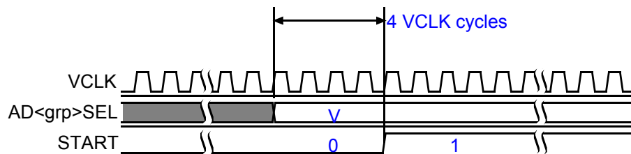
Figure 15-6. Timing Diagram of Software Trigger
