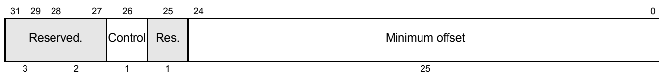
Figure 18-76. ADCNST Data Field (D31:D0)
