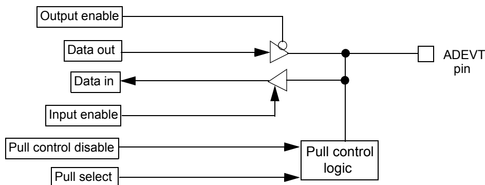
Figure 15-22. GPIO Functionality
