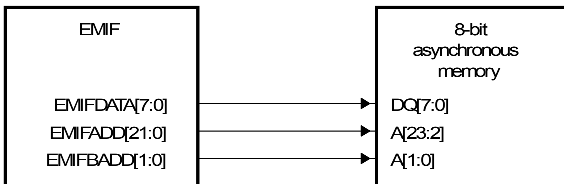
Figure 10-3. EMIF to 8-Bit Memory Interface
