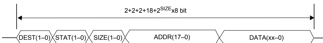
Figure 26-2. Trace Mode Packet Format
