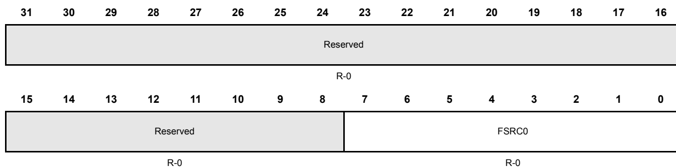
Figure 6-21. Fail Status Count 0 Register (FSRC0) [offset = 0x0198]
