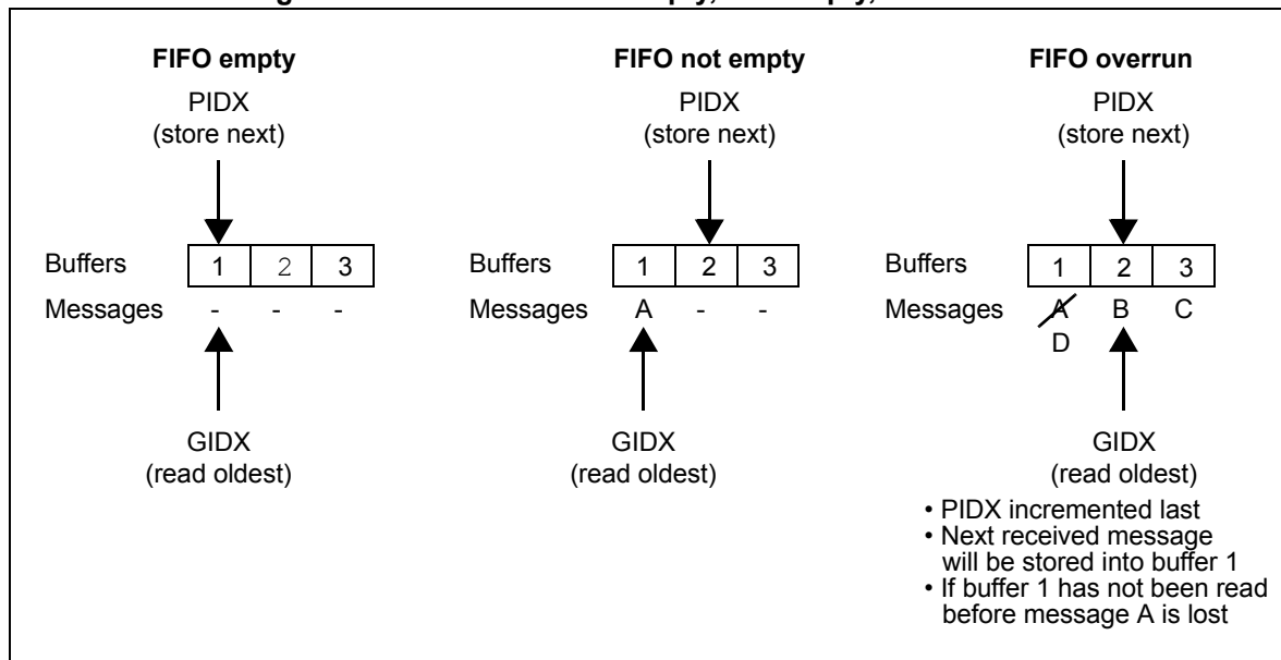
Figure 17-14. FIFO Status: Empty, Not Empty, and Overrun
