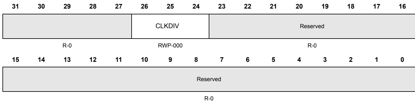
Figure 5-53. CPU Logic BIST Clock Prescaler (STCCLKDIV) [offset = 0x08]
