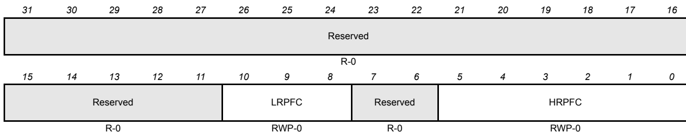
Figure 18-37. Prescale Factor Register (HETPFR) [0xFFFF7B804]
