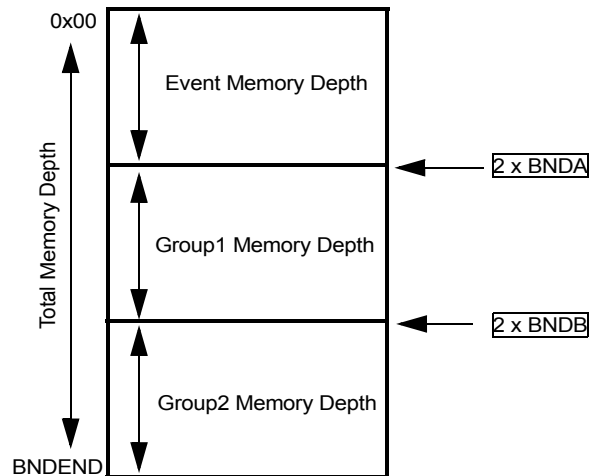
Figure 15-8. FIFO Memory Partitioning between Conversion Groups
