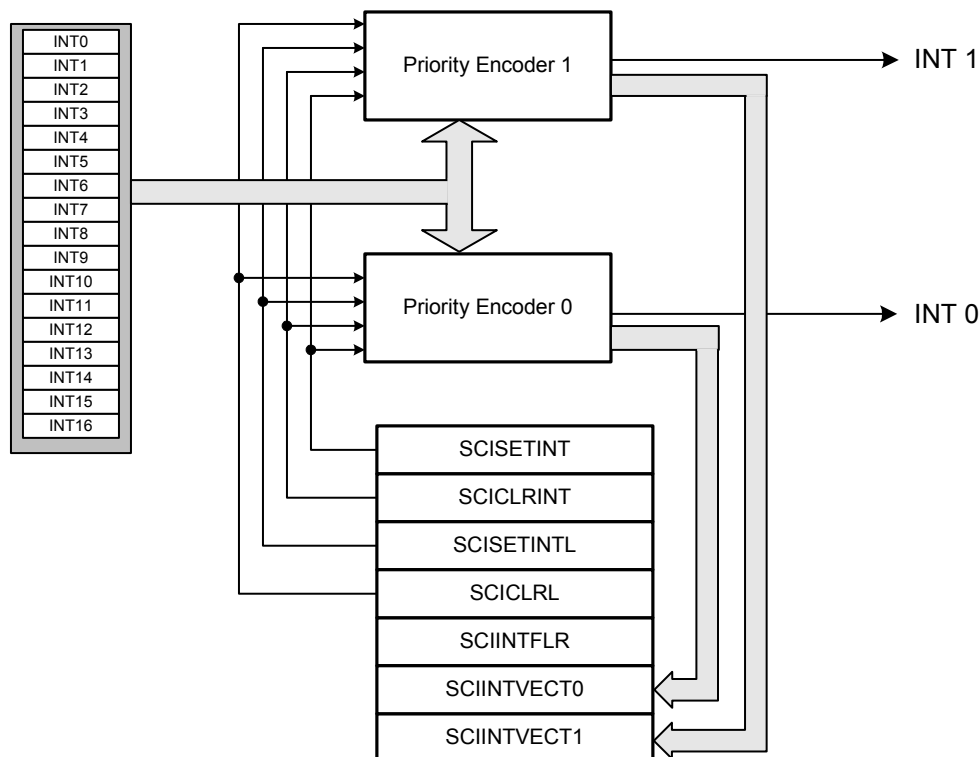
Figure 13-10. General Interrupt Scheme
