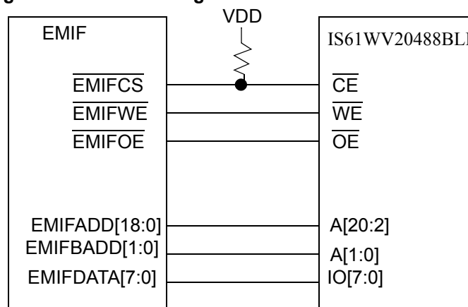
Figure 10-8. Connecting the EMIF to the IS61WV20488BLL
