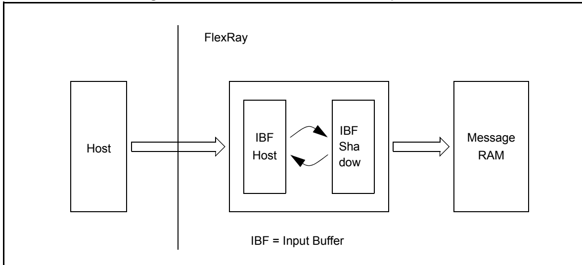
Figure 17-16. Double Buffer Structure Input Buffer
