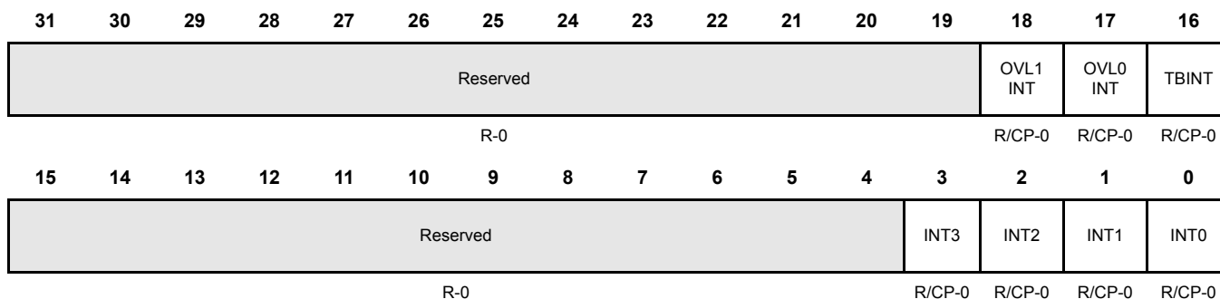
Figure 21-35. RTI Interrupt Flag Register (RTIINTFLAG) [offset = 0x88h]
