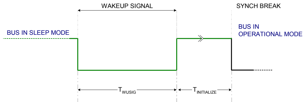
Figure 13-26. Wakeup Signal Generation
