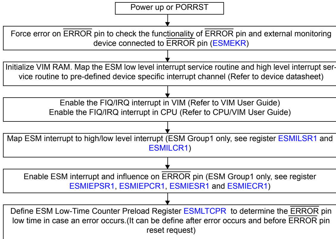
Figure 25-5. ESM Initialization
