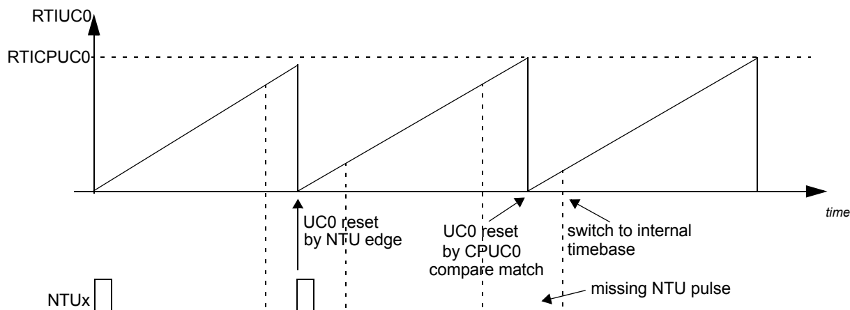
Figure 21-7. Missing NTUx Signal Example
