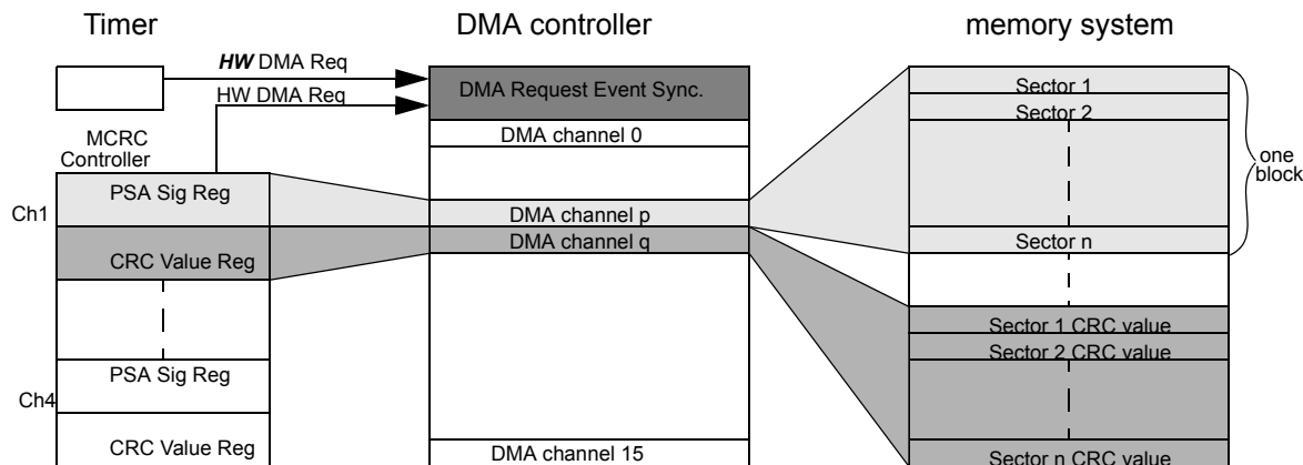
Figure 22-3. AUTO Mode Using Hardware Timer Trigger
