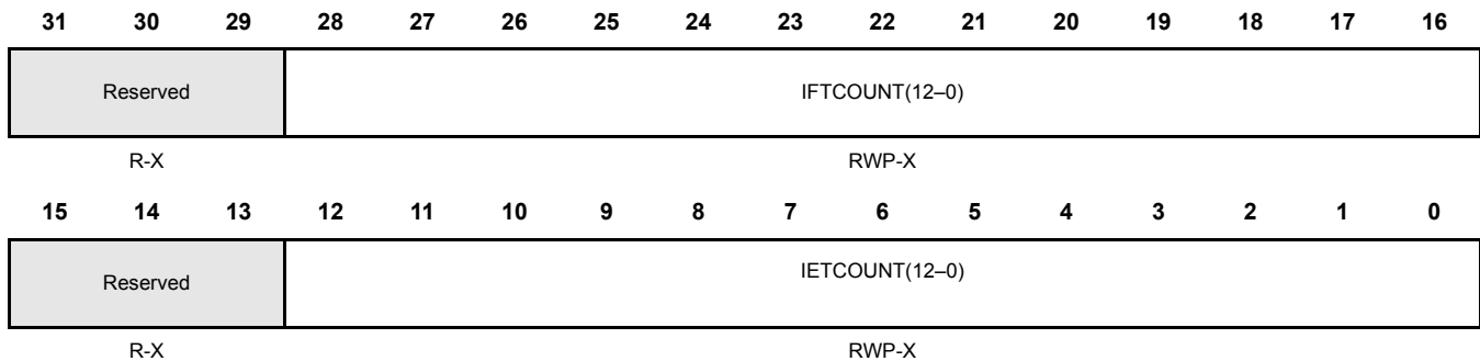
Figure 20-87. Initial Transfer Count Register (ITCOUNT) [offset = 0x008]
