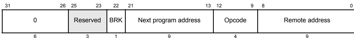
Figure 18-112. MOV32 Control Field (C31:C0)
