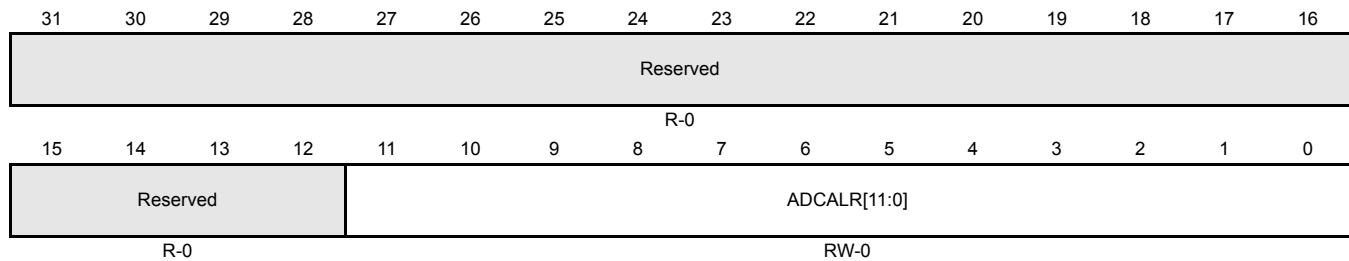
Figure 15-56. ADC Calibration and Error Offset Correction Register (ADCALR) [offset = 0x84]
