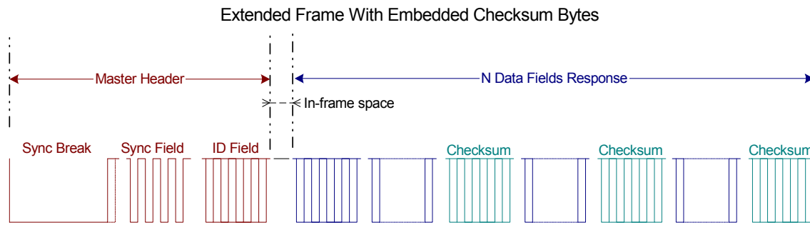
Figure 13-19. Optional Embedded Checksum in Response for Extended Frames
