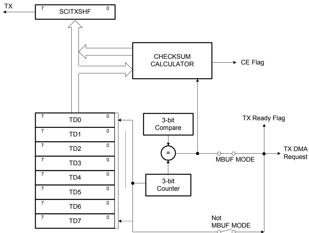
Figure 13-9. Transmit Buffers
