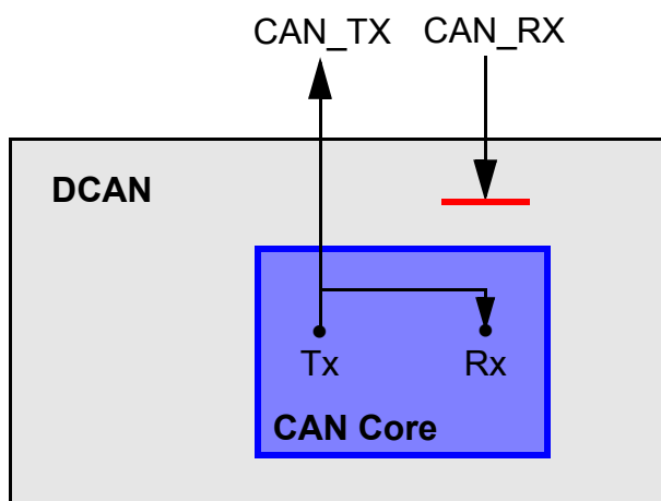
Figure 16-5. CAN Core in Loop Back Mode
