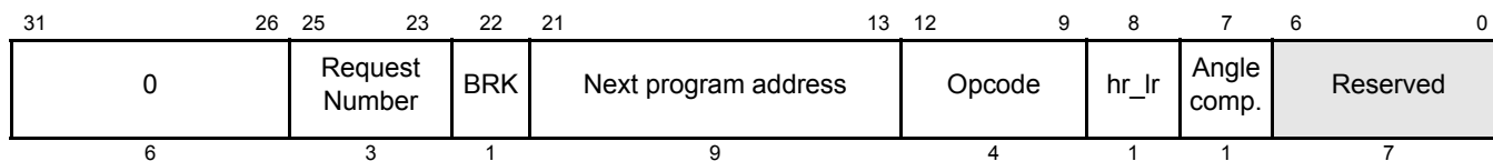
Figure 18-103. ECMP Control Field (P31:P0)
