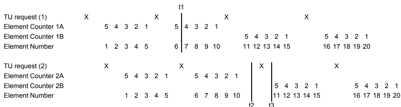
Figure 19-6. Dual Buffer Timing
