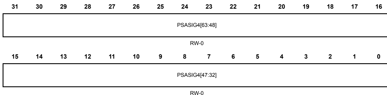
Figure 22-63. Channel 4 PSA signature high register(PSA_SIGREGH4) [offset = 0x124]
