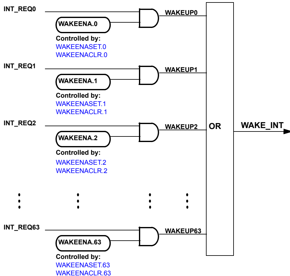
Figure 24-9. Detail of the IRQ Input
