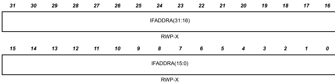
Figure 19-46. Initial Full Address A Register (HTU IFADDRA)
