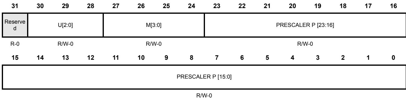
Figure 13-39. Baud Rate Selection Register (BRS) [offset = 0x2C]
