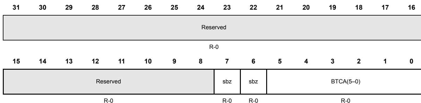
Figure 20-58. BTCA Interrupt Channel Offset Register (BTCAOFFSET) [offset = 0x158]
