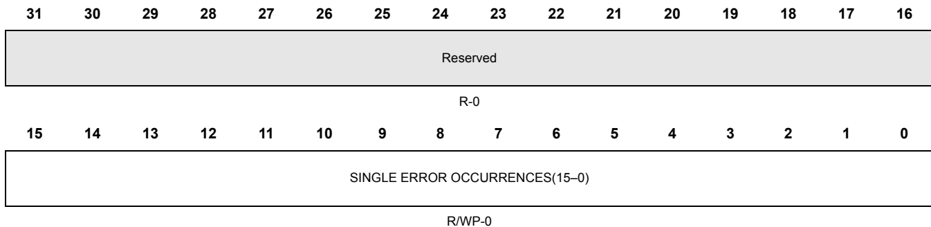
Figure 4-5. TCRAM Wrapper Single-Bit Error Occurrences Counter Register (RAMOCCUR) [offset = 0x08]
