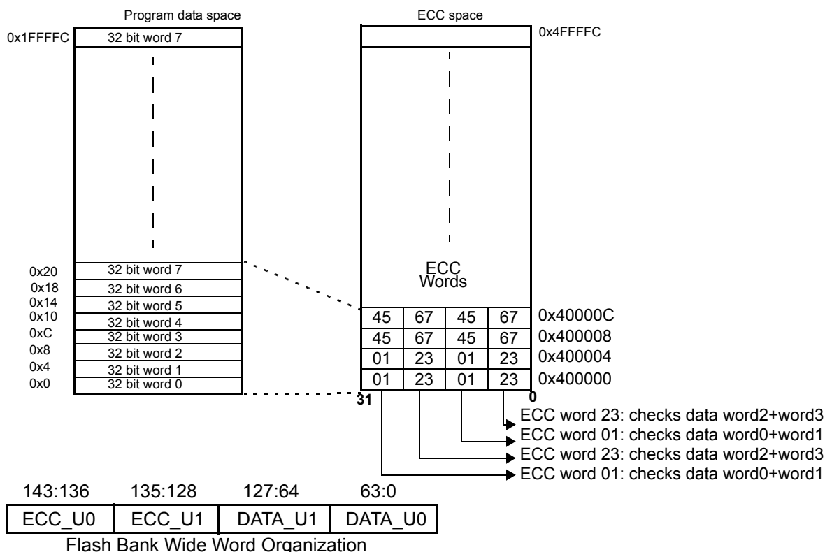
Figure 8-4. ECC Word Memory Mapping in CPU Address Space
