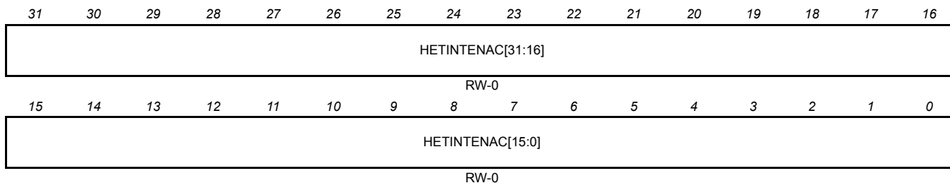
Figure 18-42. NHET Interrupt Enable Clear (HETINTENAC) [0xFFF7B818]
