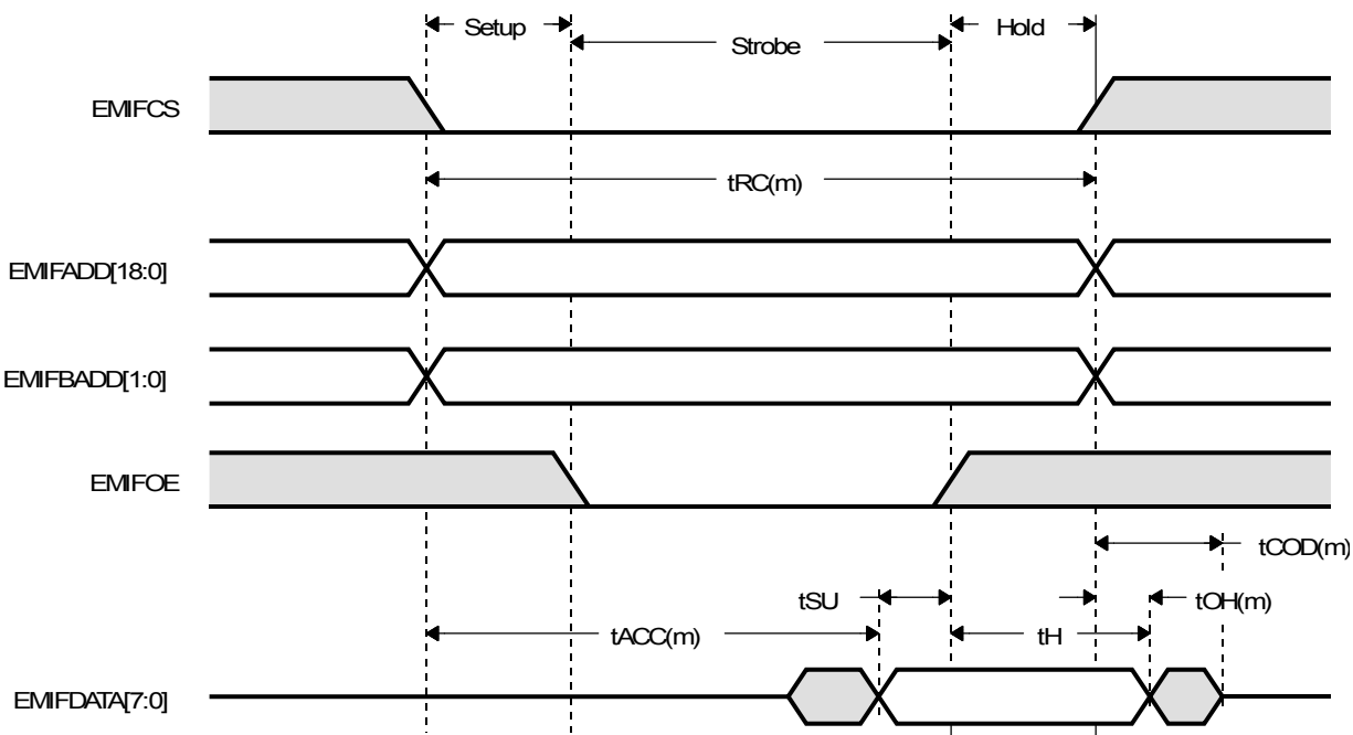
Figure 10-11. Timing Waveform of an ASRAM Write
