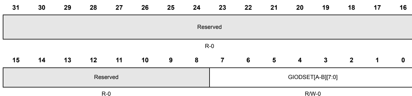
Figure 12-26. GIO Data Set Registers [A-B][7:0] (GIODSET[A-B][7:0])[0xFFF7BC40, 0xFFF7BC60]
