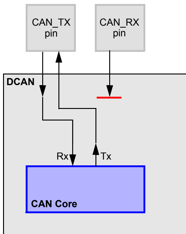
Figure 16-6. CAN Core in External Loop Back Mode
