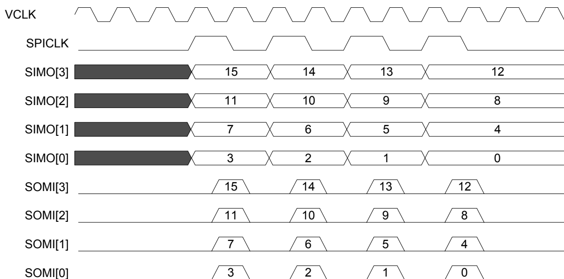
Figure 14-20. 4 Pins Parallel Mode Timing Diagram (Phase 0, Polarity 0)
