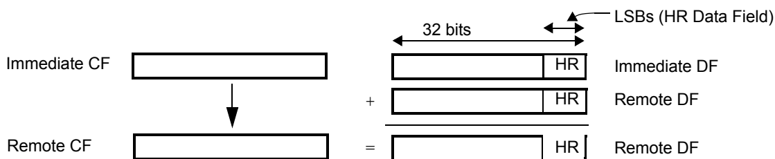
Figure 18-98. DADM64 Add and Move Operation
