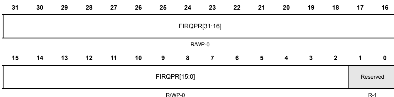
Figure 24-18. FIQ/IRQ Program Control Register 0 (FIRQPR0) [0xFFFFFE10]
