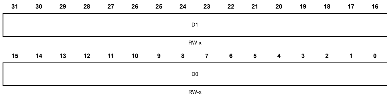
Figure 6-5. DD0 Data Register (DD0) [offset = 0x0120]
