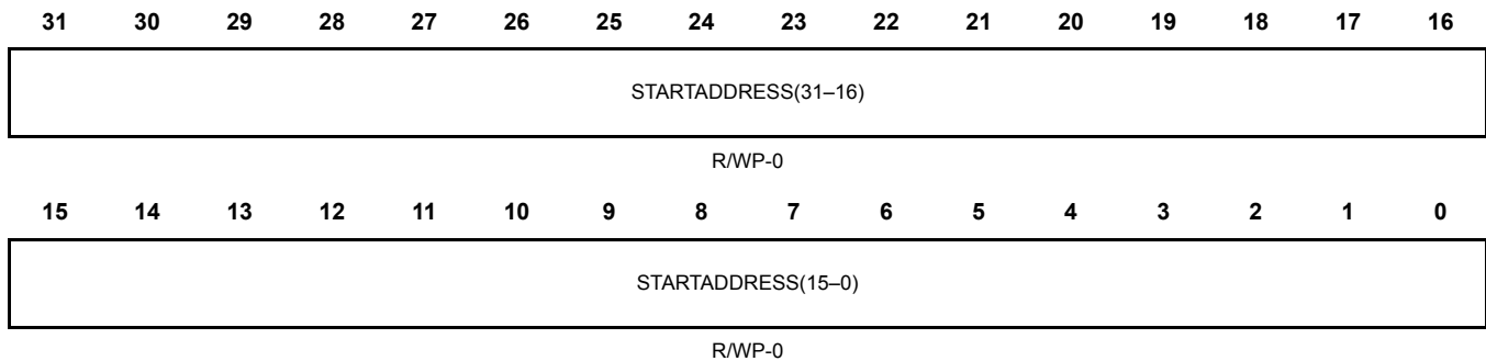
Figure 20-77. DMA Memory Protection Region 0 Start Address Register (DMAMPR0S) [offset = 0x1B8]
