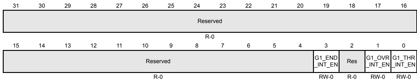
Figure 15-34. ADC Group1 Interrupt Enable Control Register (ADG1INTENA) [offset = 0x2C]
