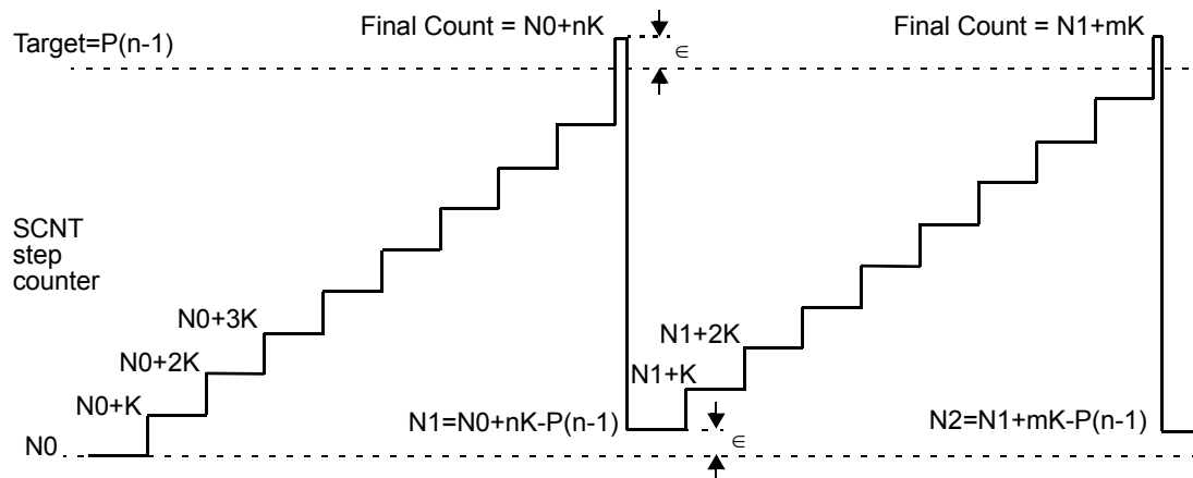
Figure 18-31. SCNT Count Operation
