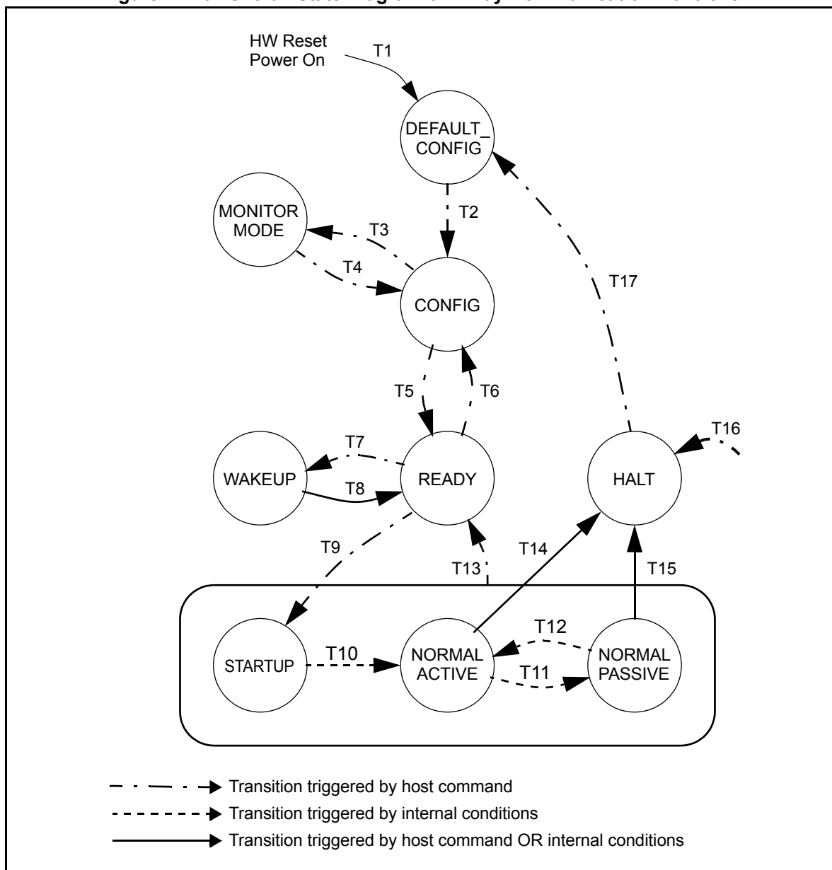
Figure 17-10. Overall State Diagram of E-Ray Communication Controller
