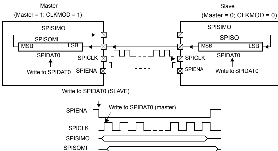
Figure 14-4. Operation with SPIENA
