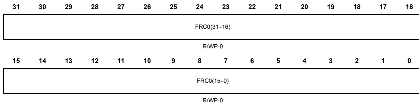
Figure 21-13. RTI Free Running Counter 0 Register (RTIFRC0) [offset = 0x10h]
