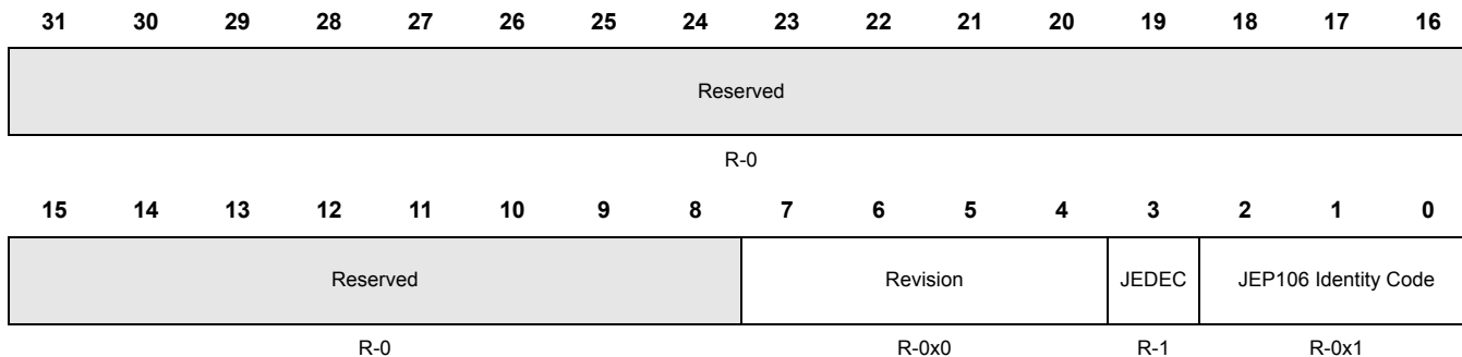
Figure 11-23. POM Peripheral ID 2 Register (POMPERIPHERALID2) [offset = 0xFE8]
