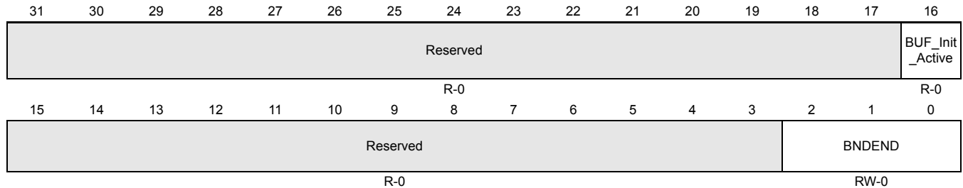
Figure 15-46. ADC Results Memory Size Configuration Register (ADBNDEND) [offset = 0x5C]
