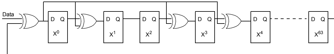
Figure 22-2. LFSR
