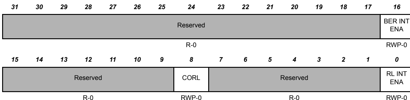
Figure 19-23. Request Lost and Bus Error Control Register (HTU RLBECTRL) [offset = 0x20]
