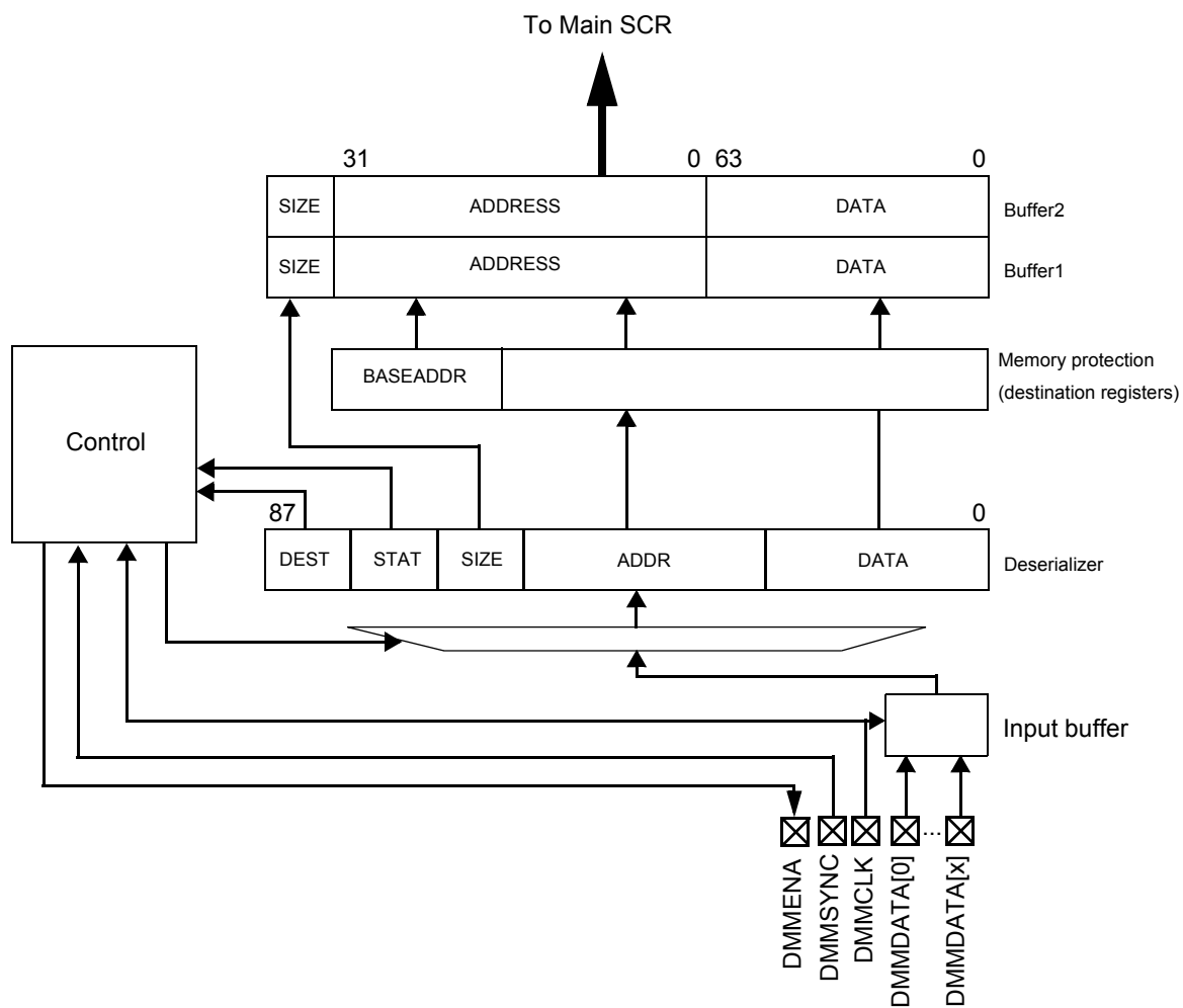
Figure 26-1. DMM Block Diagram
