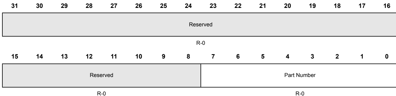
Figure 11-21. POM Peripheral ID 0 Register (POMPERIPHERALID0) [offset = 0xFE0]
