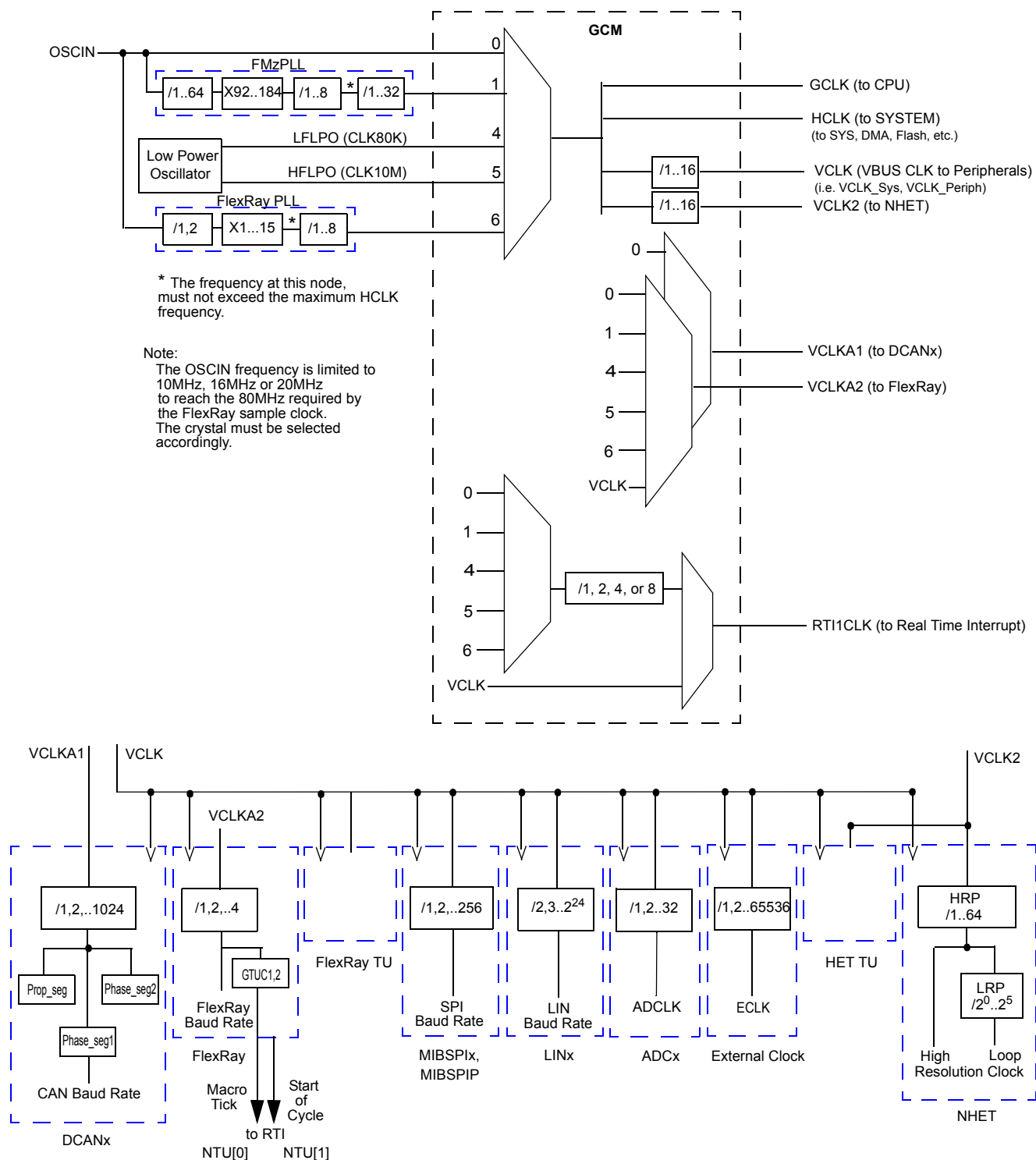
Figure 2-1. TMS570LS20x/10x Safety MCUs Device Clocks
