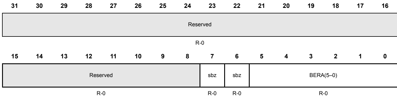
Figure 20-59. BERA Interrupt Channel Offset Register (BERAOFFSET) [offset = 0x15C]
