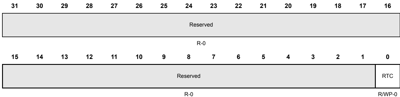
Figure 20-66. RAM Test Control (RTCTRL) [offset = 0x17C]
