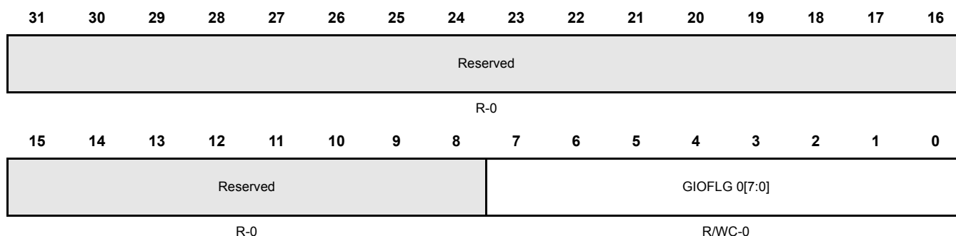
Figure 12-18. GIO Interrupt Flag Register (GIOFLG) [0xFFF7BC20]
