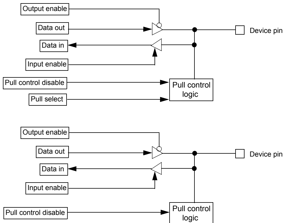
Figure 13-61. GPIO Functionality
