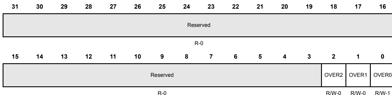
Figure 6-18. Override Register (OVER) [offset = 0x0188]
