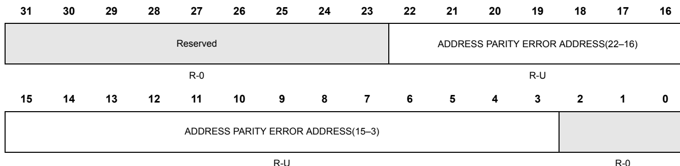
Figure 4-12. TCRAM Wrapper Parity Error Address Register (RAMPERRADDR) [offset = 0x3C]
