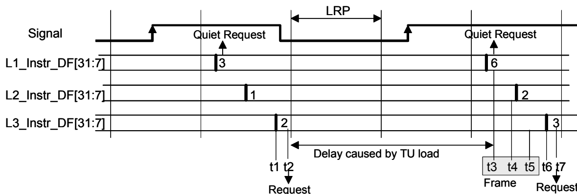
Figure 19-11. Timing, which generates a request lost error
