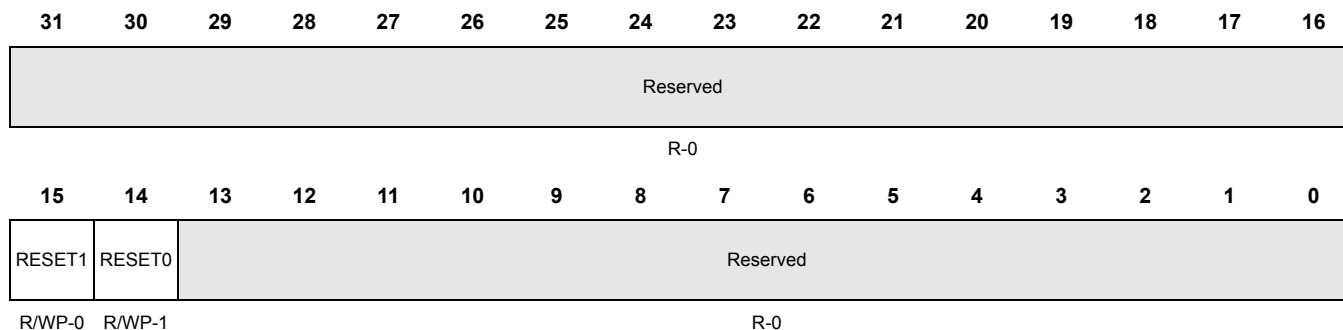
Figure 5-45. System Exception Control Register (SYSECR) [offset = 0xE0]
