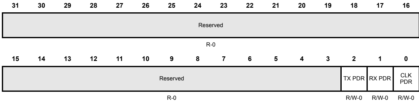
Figure 13-49. SCI Pin I/O Control Register 6 (SCIPIO6) [offset = 0x54]
