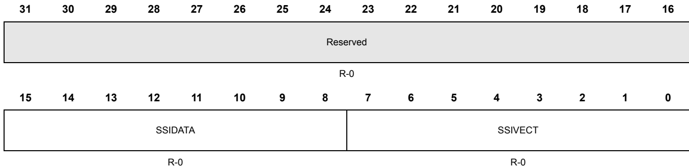
Figure 5-49. Software Interrupt Vector Register (SSIVEC) [offset = 0xF4]
