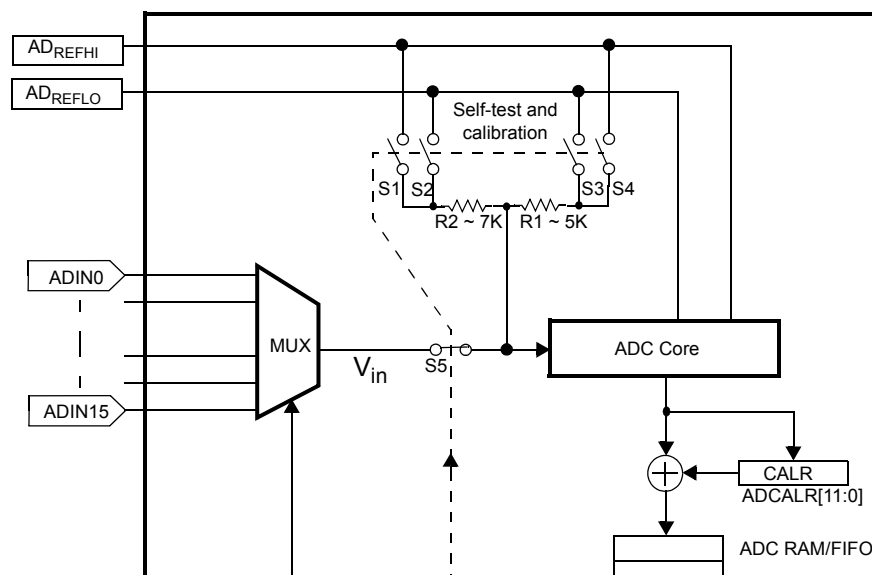
Figure 15-19. Self-Test and Calibration Logic
