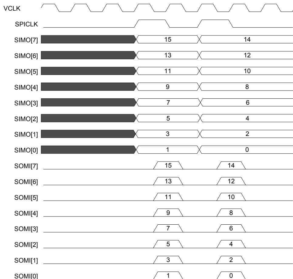
Figure 14-22. 8 Pins Parallel Mode Timing Diagram (Phase 0, Polarity 0)
