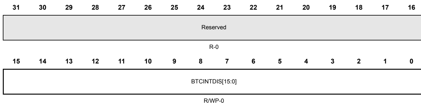
Figure 20-48. BTC Interrupt Enable Reset (BTCINTENAR) [offset = 0x114]
