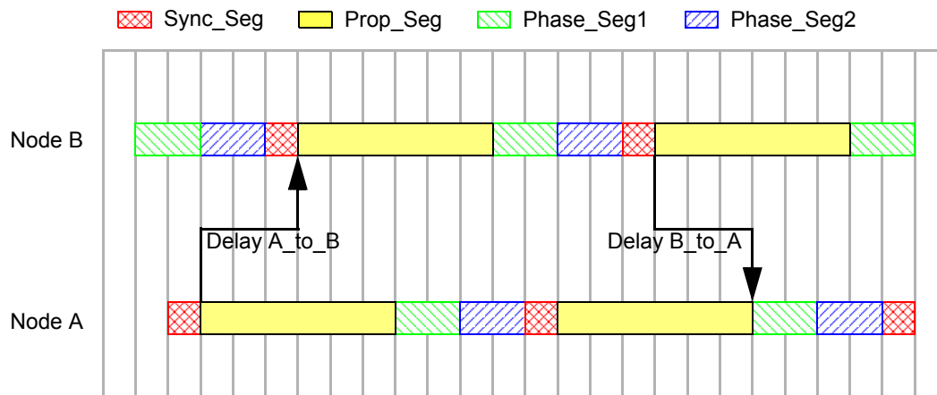
Figure 16-16. The Propagation Time Segment
