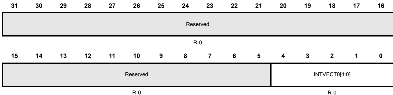
Figure 13-36. SCI Interrupt Vector Offset 0 (SCIINTVECT0) [offset = 0x20]
