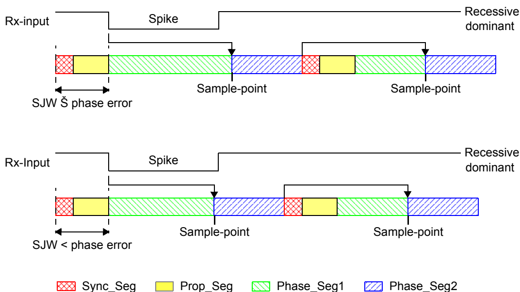
Figure 16-18. Filtering of Short Dominant Spikes
