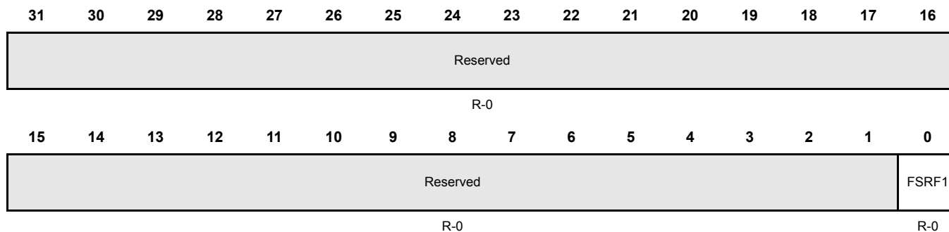
Figure 6-20. Fail Status Fail Register 1 (FSRF1) [offset = 0x0194]
