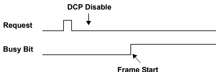
Figure 19-8. Timing for disabling Control Packets
