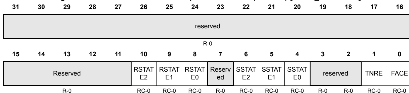
Figure 17-51. Transfer Error Interrupt Enable Reset (TEIRER) [offset_TU = 0x7C]
