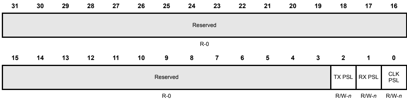
Figure 13-51. SCI Pin I/O Control Register 8 (SCIPIO8) [offset = 0x5C]
