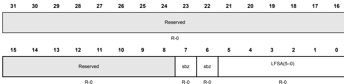
Figure 20-56. LFSA Interrupt Channel Offset Register (LFSAOFFSET) [offset = 0x150]
