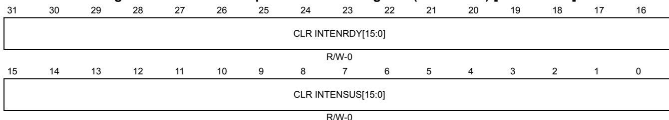
Figure 14-31. TG Interrupt Enable Clear Register (TGITENCR) [offset = 78h]
