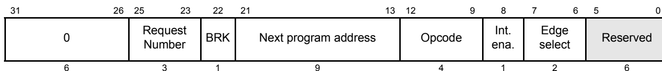
Figure 18-87. APCNT Control Field (C31:C0)
