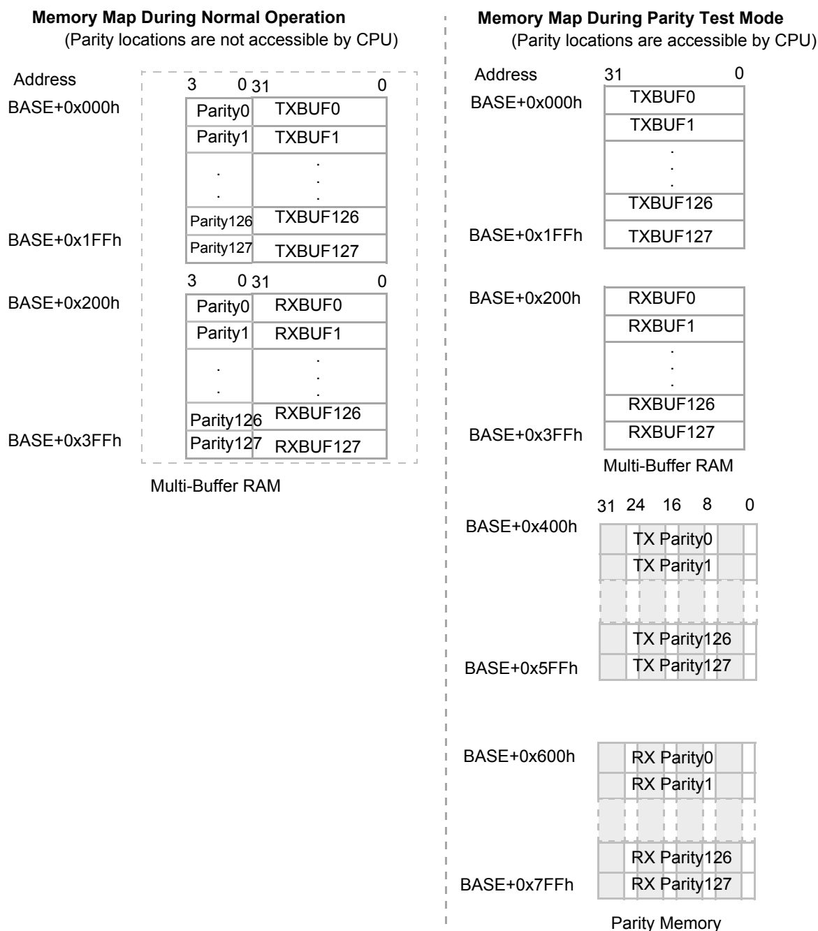
Figure 14-51. Memory Map for Parity Locations during Normal and Test Mode
