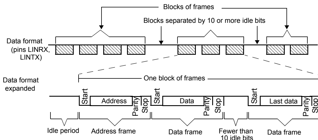
Figure 13-6. Idle-Line Multiprocessor Communication Format
