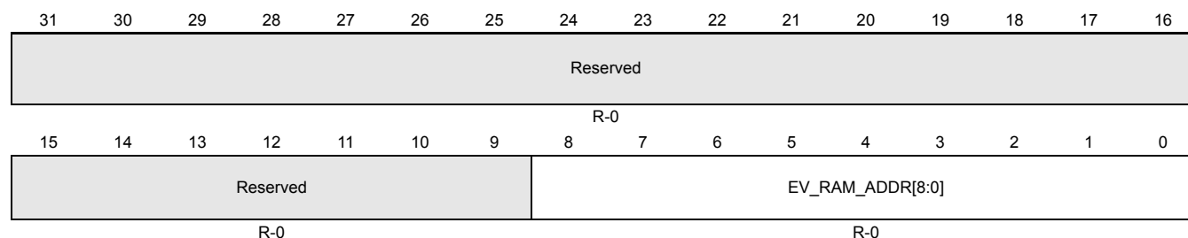
Figure 15-81. ADC Event Group RAM Write Address (ADEVAMWRADDR) [offset = 0x174]
