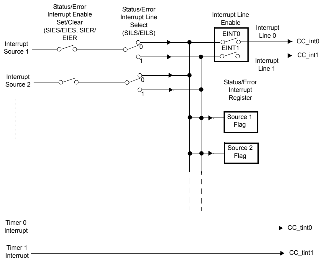
Figure 17-26. Interrupt Structure
