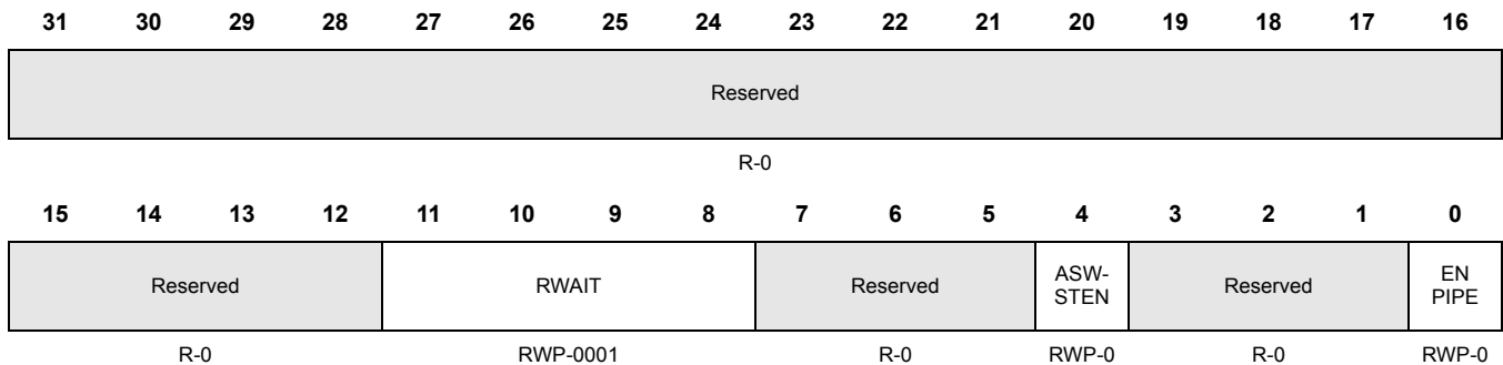
Figure 8-7. Flash Option Control Register (FRDCNTL) [0xFFFF87000]
