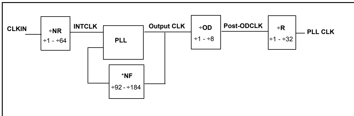
Figure 7-2. FMzPLL Block Diagram
