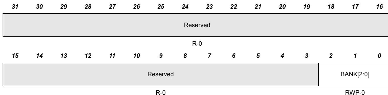
Figure 8-23. Flash Module Access Control Register (FMAC - 0xFFFF87050)
