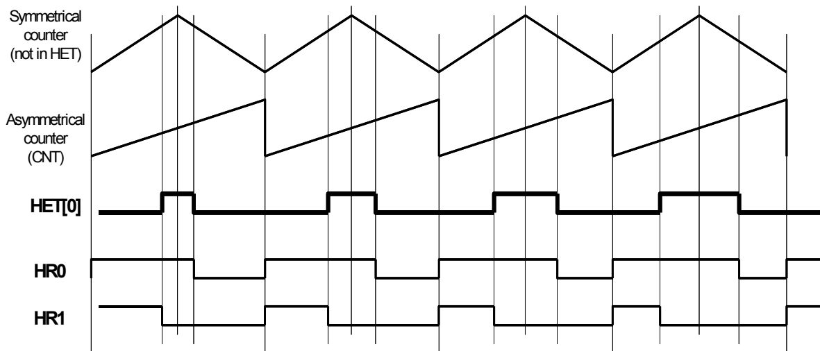
Figure 18-15. Symmetrical PWM with XOR-sharing Output
