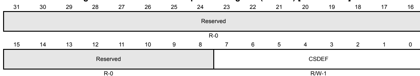
Figure 14-24. SPI Default Chip Select Register (SPIDEF) [offset = 4Ch]
