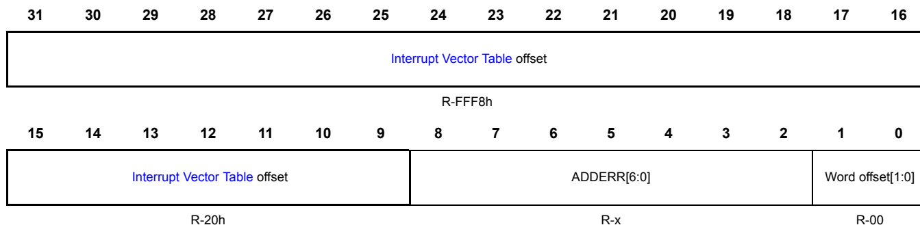
Figure 24-14. Address Parity Error Register (ADDERR) [0xFFFFDF4]
