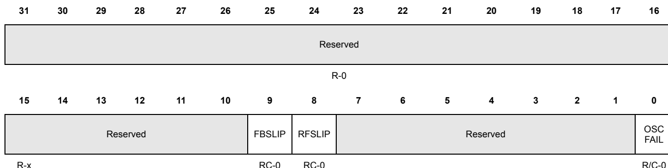
Figure 5-47. Global Status Register (GLBSTAT) [offset = 0xEC]
