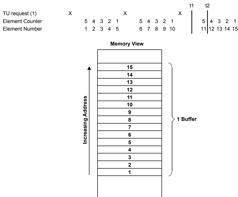
Figure 19-4. Single Buffer Timing and Memory Representation
