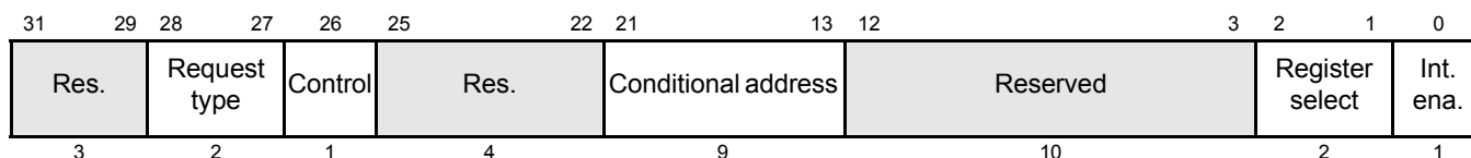
Figure 18-101. DJZ Data Field (D31:D0)
