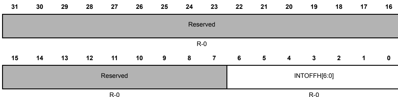
Figure 25-16. ESM Interrupt Offset High Register (ESMIOFFHR)
