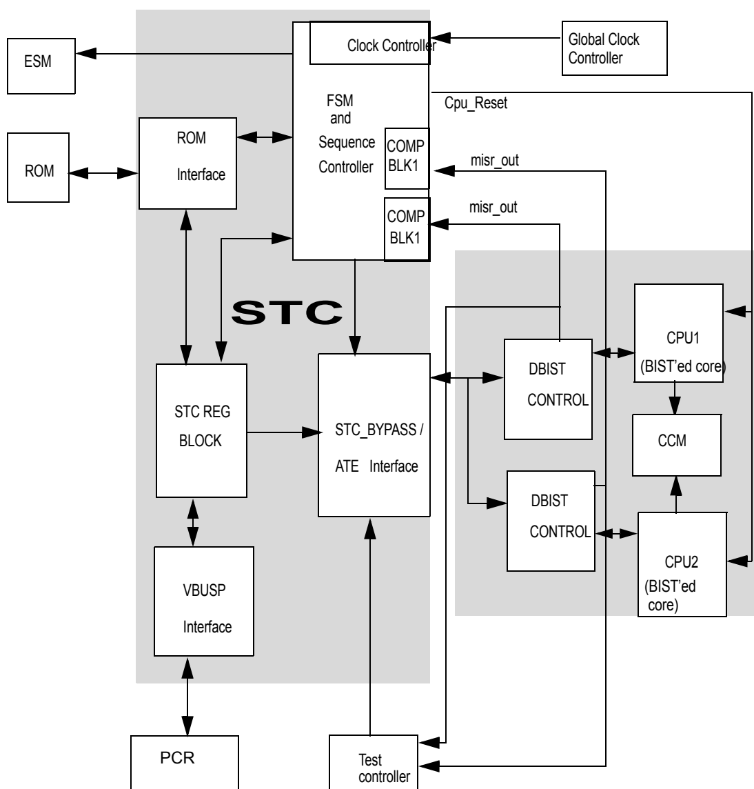
Figure 9-2. Block diagram for Dual CPU architecture with CCM
