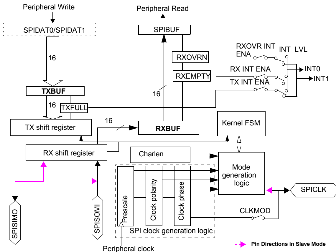
Figure 14-1. SPI Functional Logic Diagram
