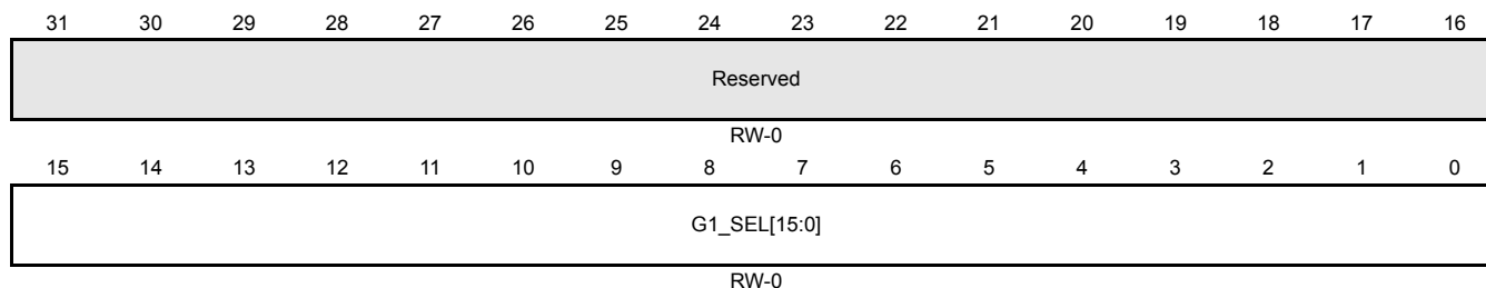
Figure 15-54. ADC Group1 Channel Select Register (ADG1SEL) [offset = 0x7C]
