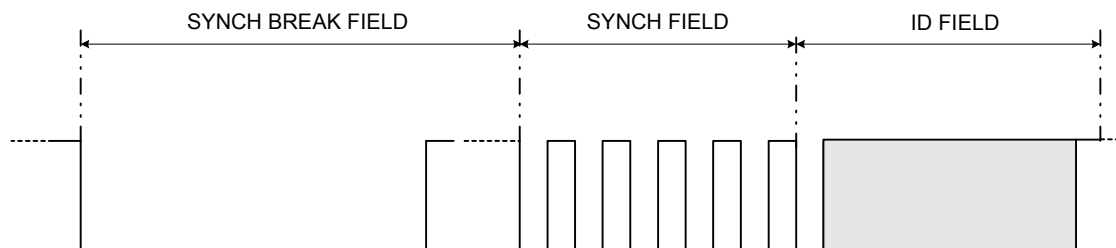
Figure 13-13. Header 3 fields: Synch Break, Synch, and ID
