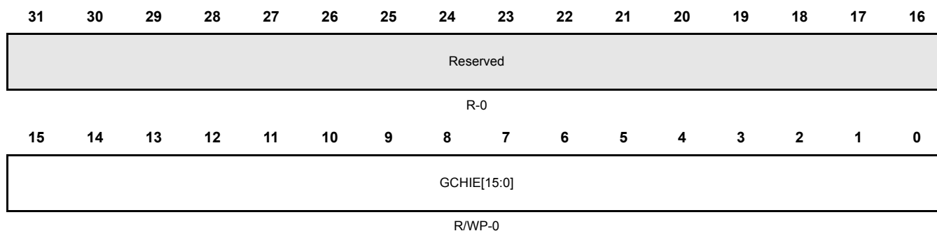
Figure 20-28. Global Channel Interrupt Enable Set Register (GCHIENAS) [offset = 0x44]
