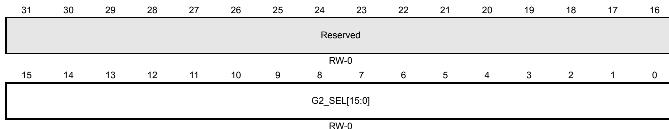
Figure 15-55. ADC Group2 Channel Select Register (ADG2SEL) [offset = 0x80]
