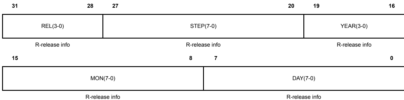
Figure 17-171. Core Release Register (CREL) [offset_CC = 0x3F0]
