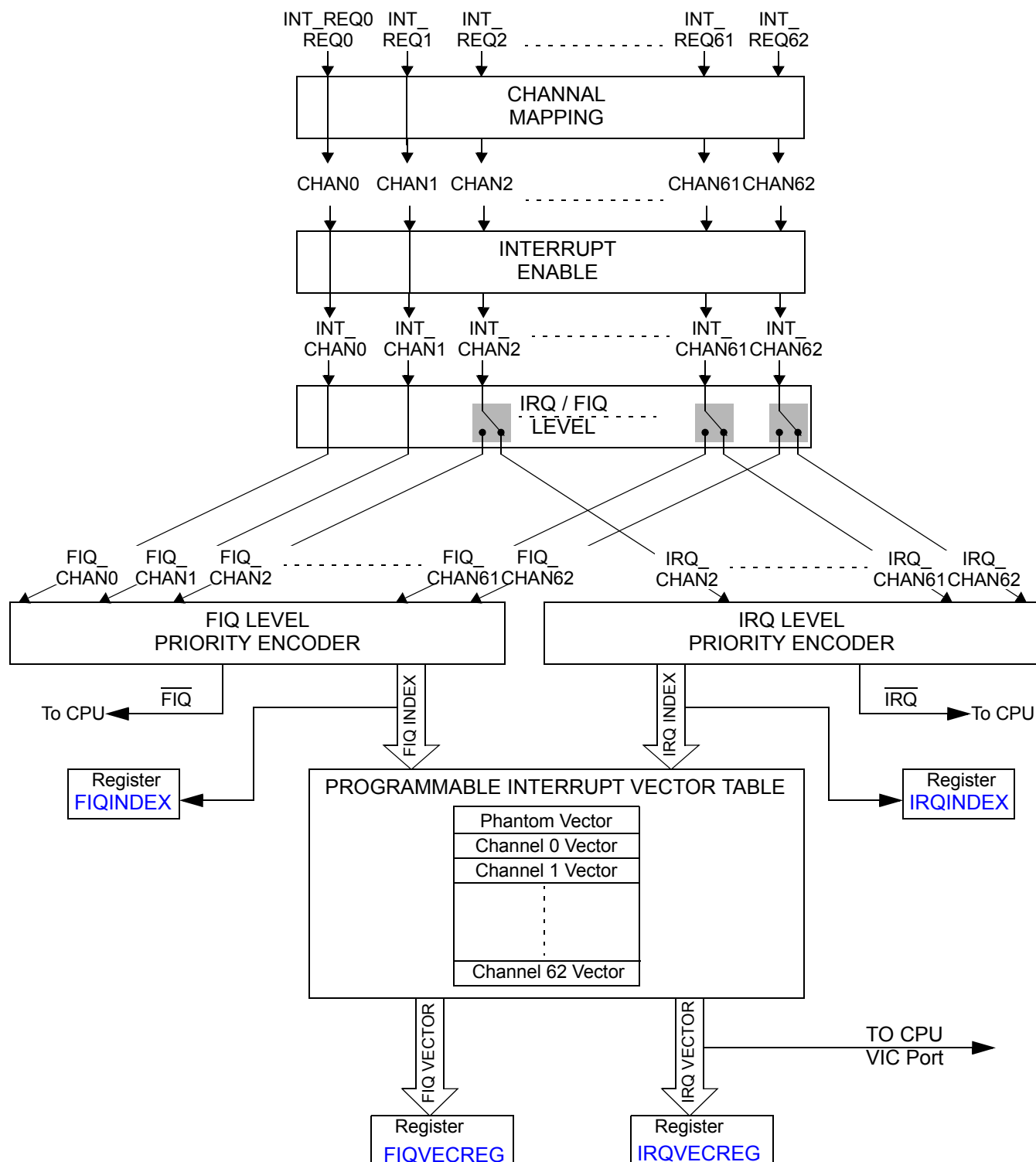
Figure 24-2. VIM Interrupt Handling Block Diagram
