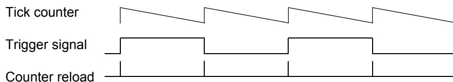
Figure 14-35. Tick Counter Operation
