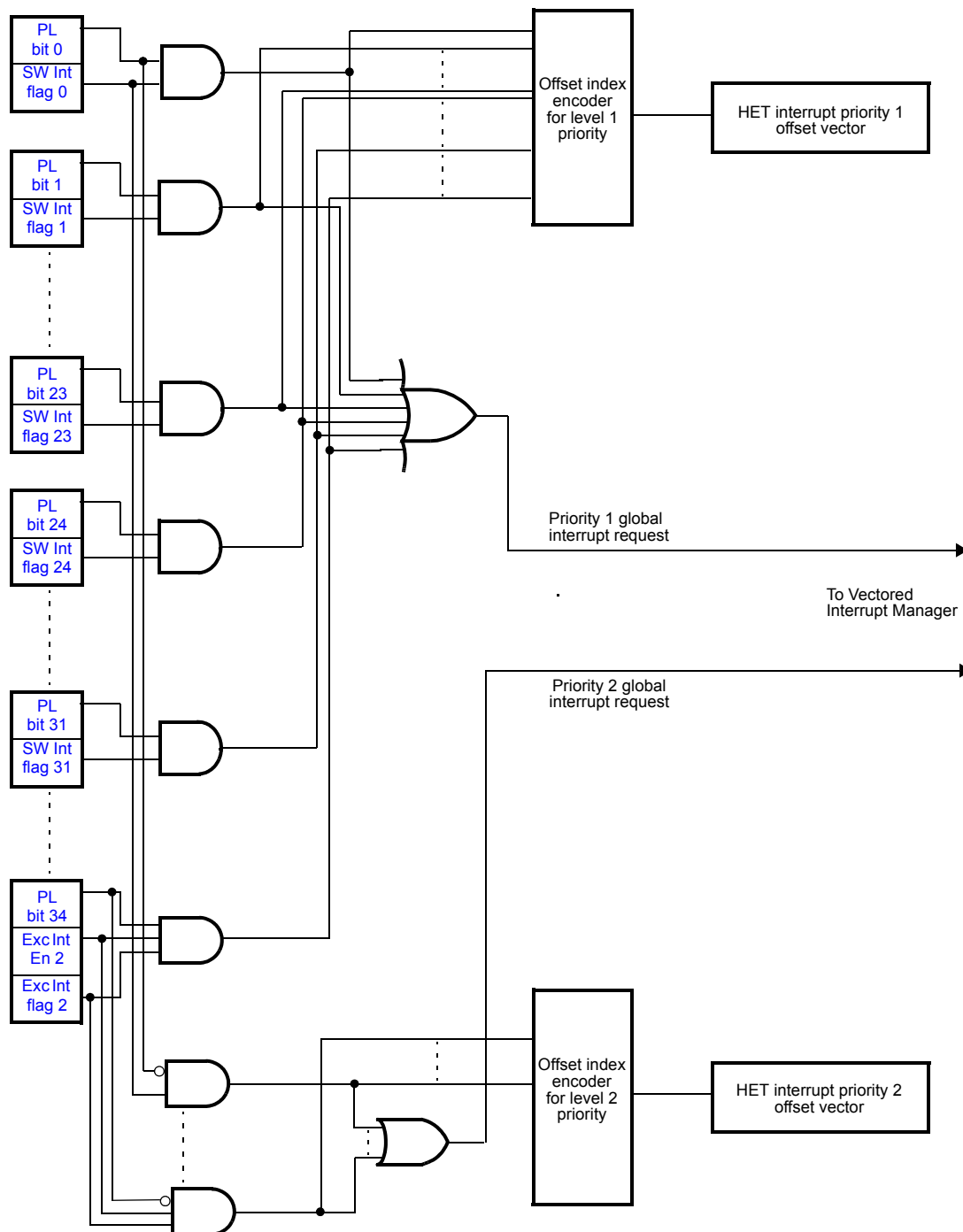
Figure 18-28. Interrupt Flag/Priority Level Architecture
