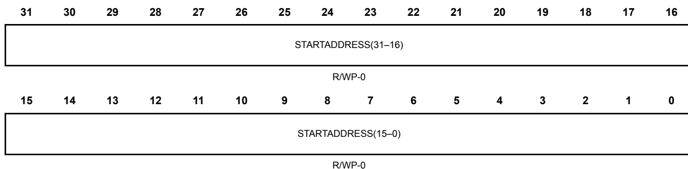
Figure 20-81. DMA Memory Protection Region 2 Start Address Register (DMAMPR2S) [offset = 0x1C8]
