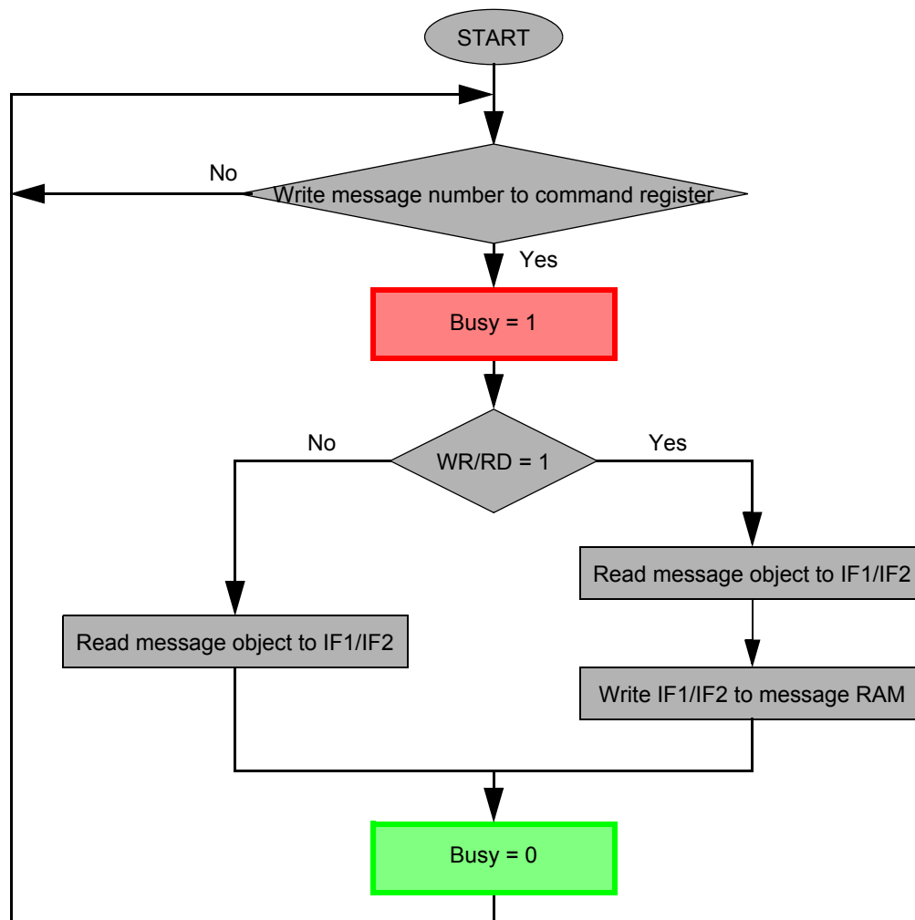
Figure 16-20. Data Transfer Between IF1 / IF2 Registers and Message RAM
