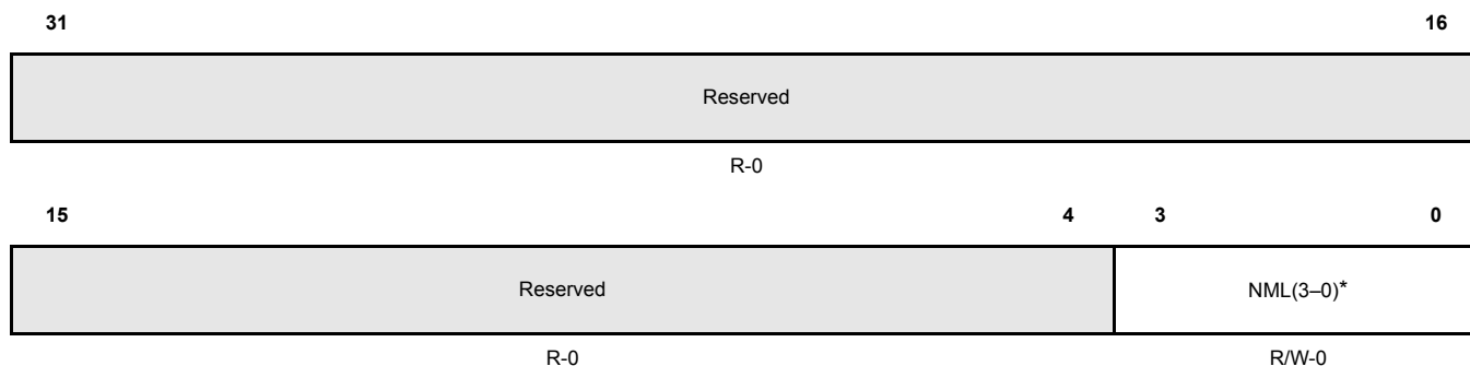
Figure 17-123. NEM Configuration Register (NEMC) [offset_CC = 0x8C]
