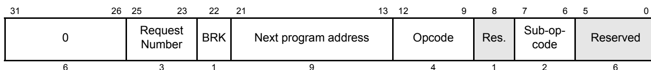
Figure 18-100. DJZ Control Field (C31:C0)
