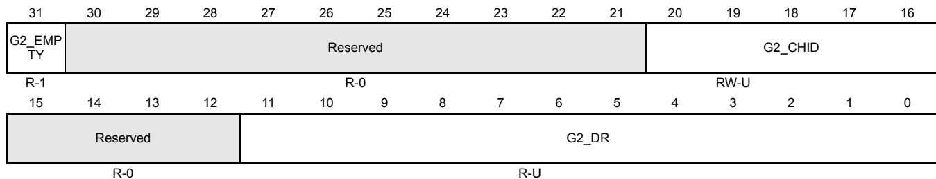
Figure 15-60. ADC Group2 Results FIFO (ADG2BUFFER) [offset = 0xD0 - 0xEF]
