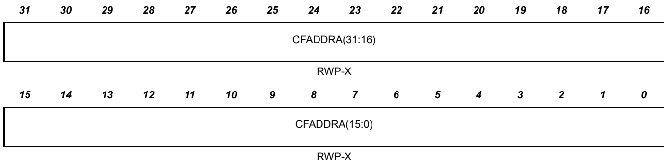
Figure 19-50. Current Full Address A Register (HTU CFADDRA)
