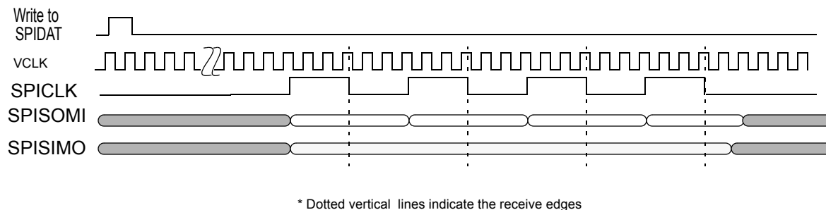
Figure 14-57. SPI/MibSPI pins during Slave mode 3-pin configuration
