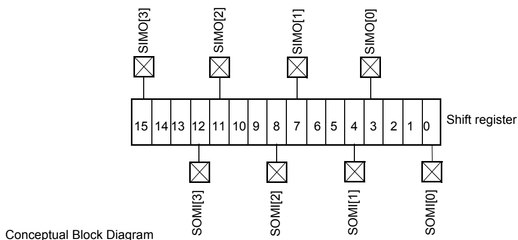
Figure 14-19. 4-Data Line Mode (Phase 0, Polarity 0)
