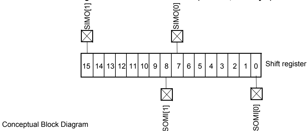
Figure 14-16. 2-data Line Mode (Phase 0, Polarity 0)
