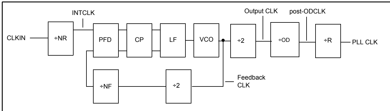
Figure 7-3. Basic PLL Circuit
