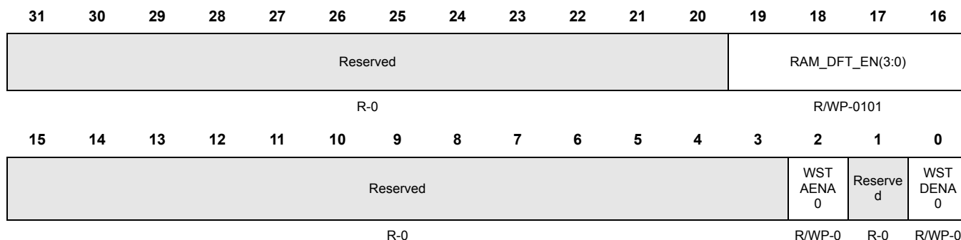
Figure 5-38. RAM Control Register (RAMGCR) [offset = 0xC0]
