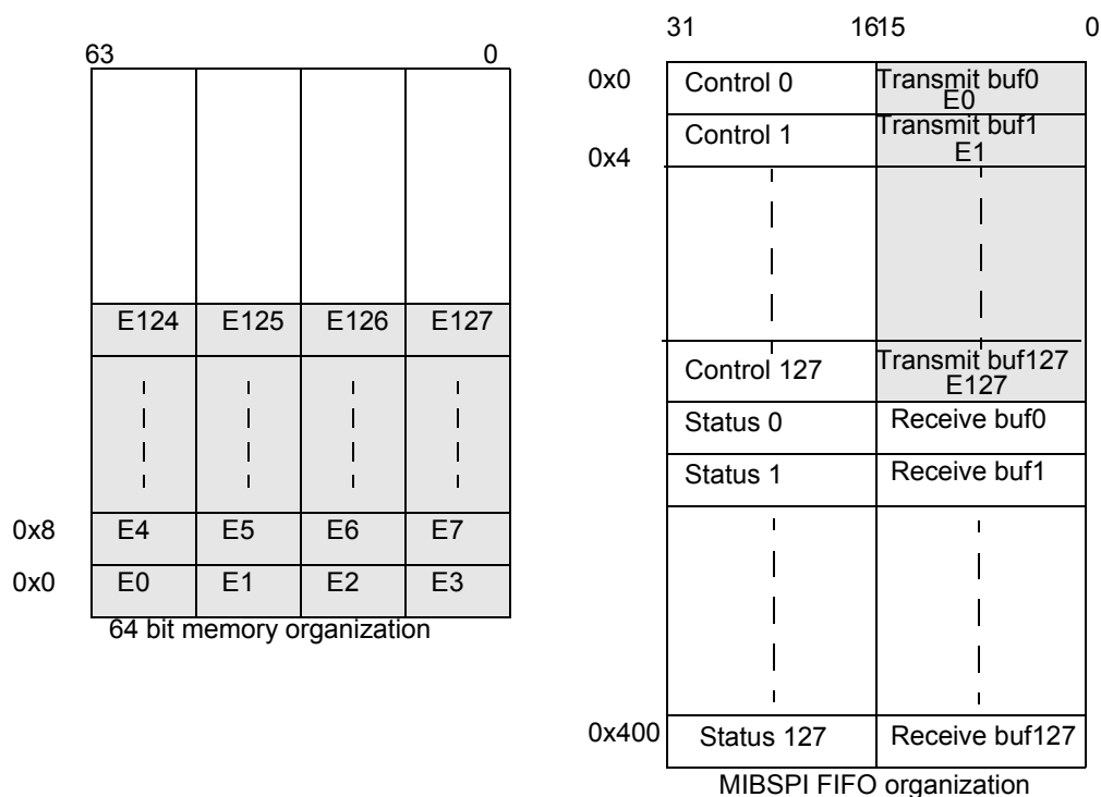
Figure 20-12. Example of DMA Data Unpacking
