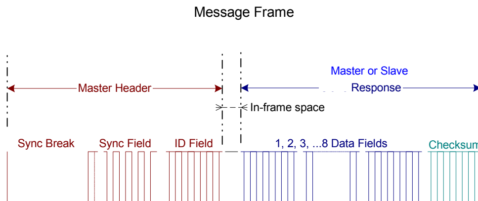
Figure 13-12. LIN Protocol Message Frame Format: Master Header and Slave Response
