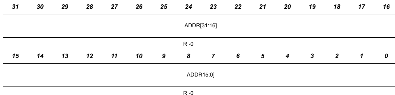
Figure 9-8. STC Current ROM Address Register (STC_CADDR)
