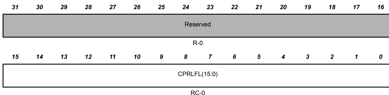
Figure 19-30. Request Lost Flag Register (HTU RLOSTFL) [offset = 0x40]
