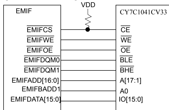
Figure 10-9. Connecting the EMIF to the CY7C1041CV33
