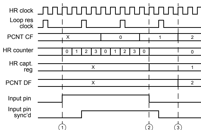
Figure 18-21. PCNT Instruction Timing (With Capture Edge After HR Counter Overflow)
