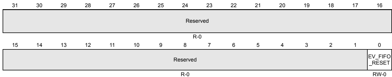
Figure 15-78. ADC Event Group FIFO Reset Control Register (ADEVFIFORESETCR) [offset = 0x168]
