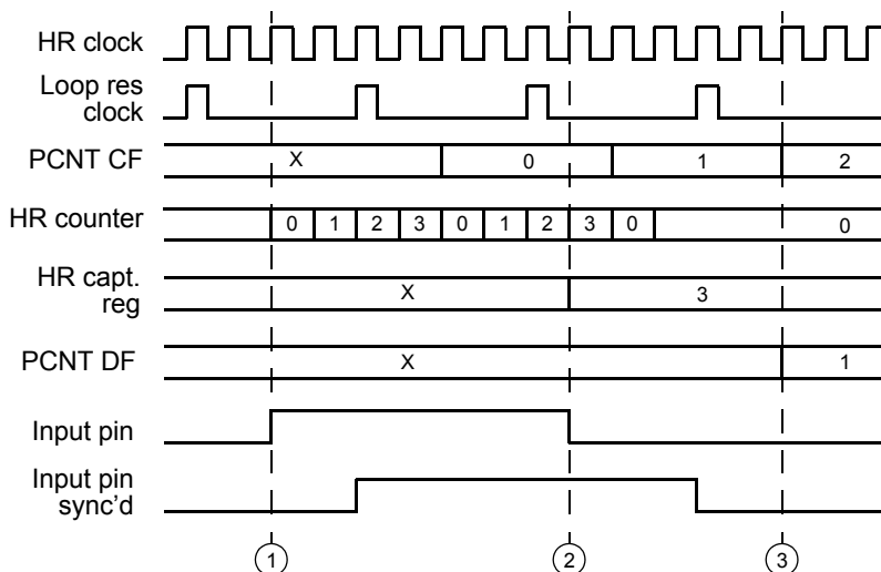
Figure 18-22. PCNT Instruction Timing (With Capture Edge Before HR Counter Overflow)
