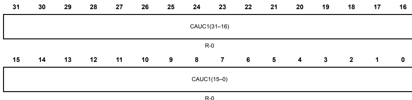
Figure 21-22. RTI Capture Up Counter 1 Register (RTICAUC1) [offset = 0x44h]
