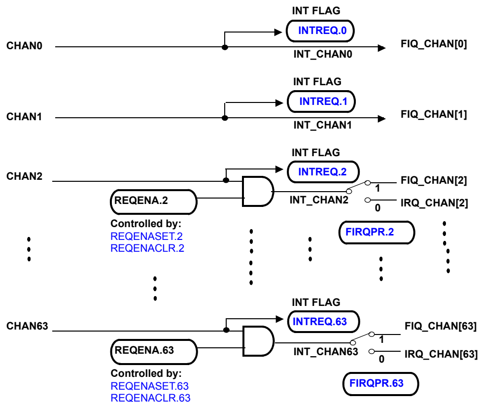
Figure 24-6. Interrupt Channel Management
