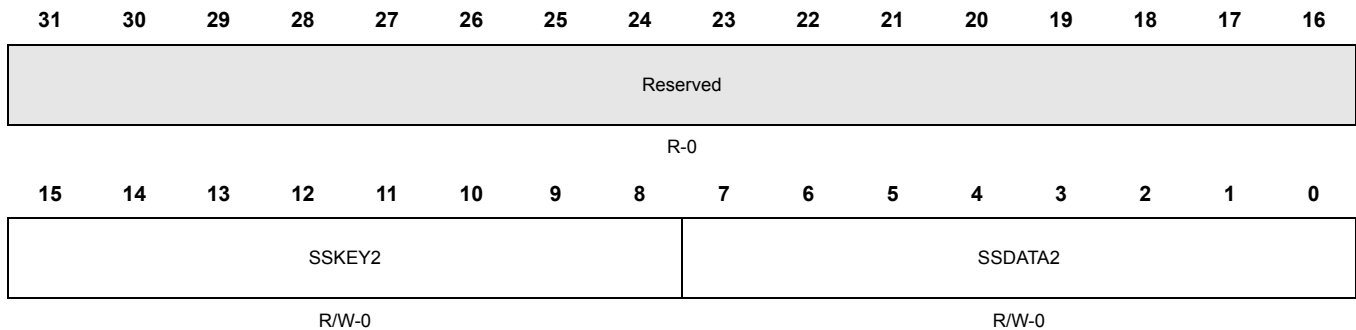
Figure 5-35. System Software Interrupt Request 2 Register (SSIR2) [offset = 0xB4]
