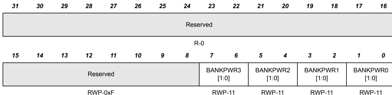
Figure 8-19. Flash Bank Fallback Power Register (FBFALLBACK - 0xFFFF87040)
