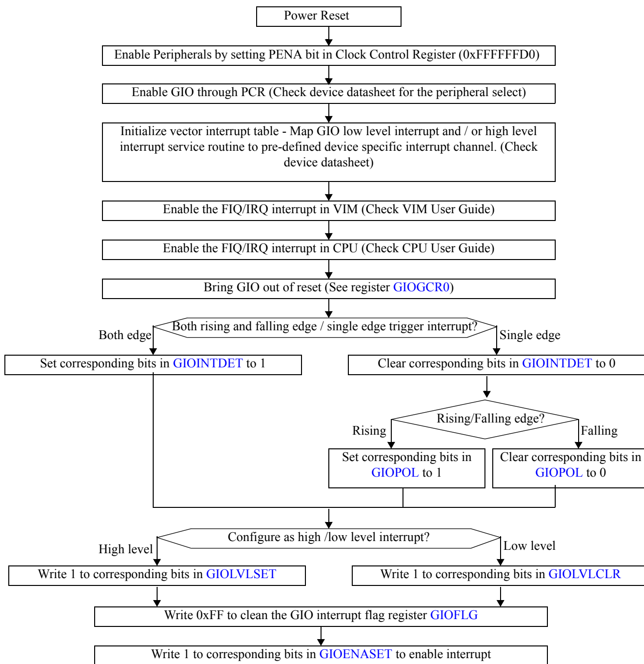
Figure 12-3. External Interrupt Function Quick Start Flow Chart
