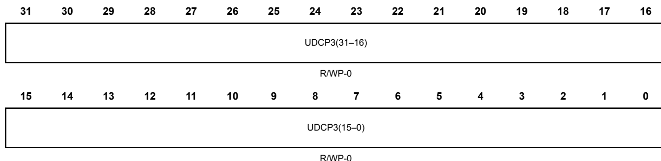
Figure 21-30. RTI Update Compare 3 Register (RTIUDCP3) [offset = 0x6Ch]
