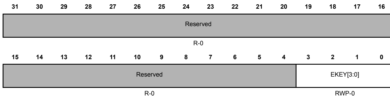
Figure 25-20. ESM Error Key Register (ESMEKR)
