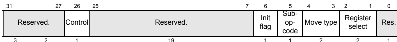
Figure 18-81. ADM32 Data Field (D31:D0)
