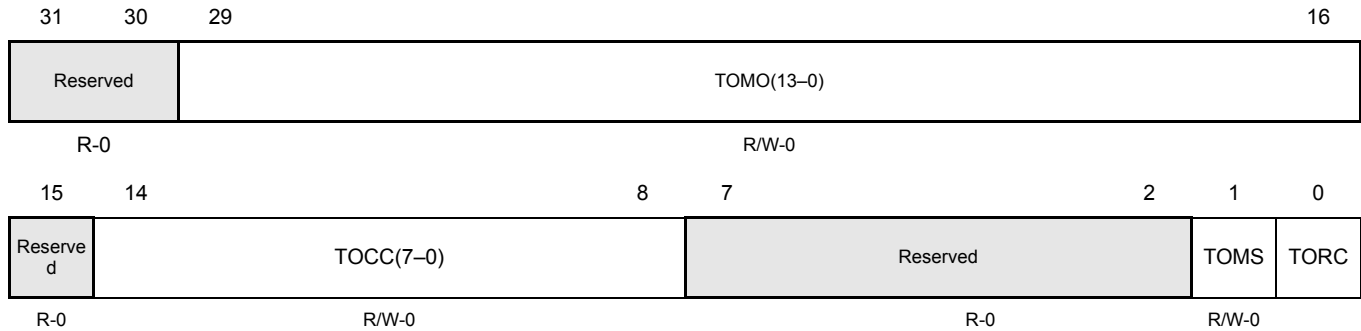
Figure 17-116. Timer 0 Configuration Register (T0C) [offset_CC = 0x44]
