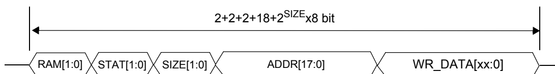
Figure 27-2. Packet Format Trace Mode for RAM Locations
