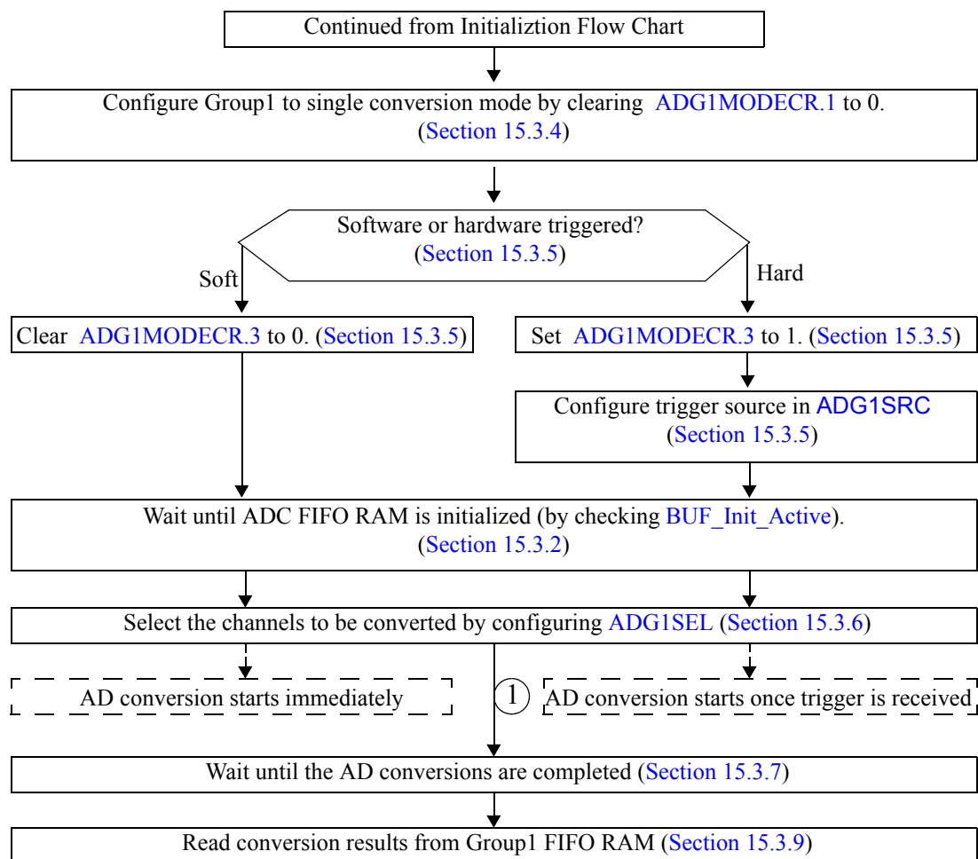
Figure 15-4. Flow Chart for Single Conversion
