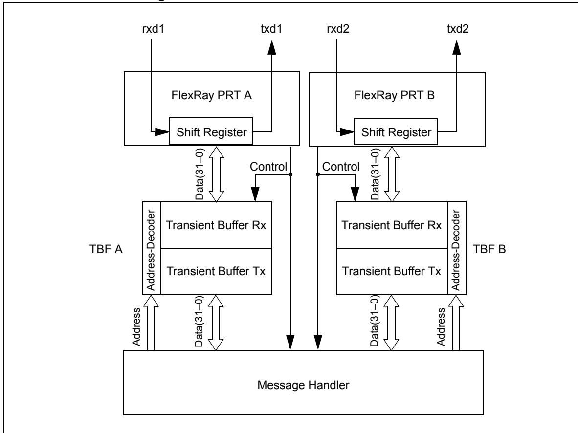
Figure 17-20. Access to Transient Buffer RAMs
