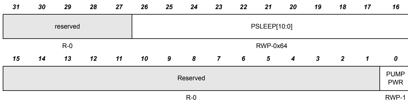
Figure 8-21. Flash Pump Access Control Register 1 (FPAC1 - 0xFFFF87048)
