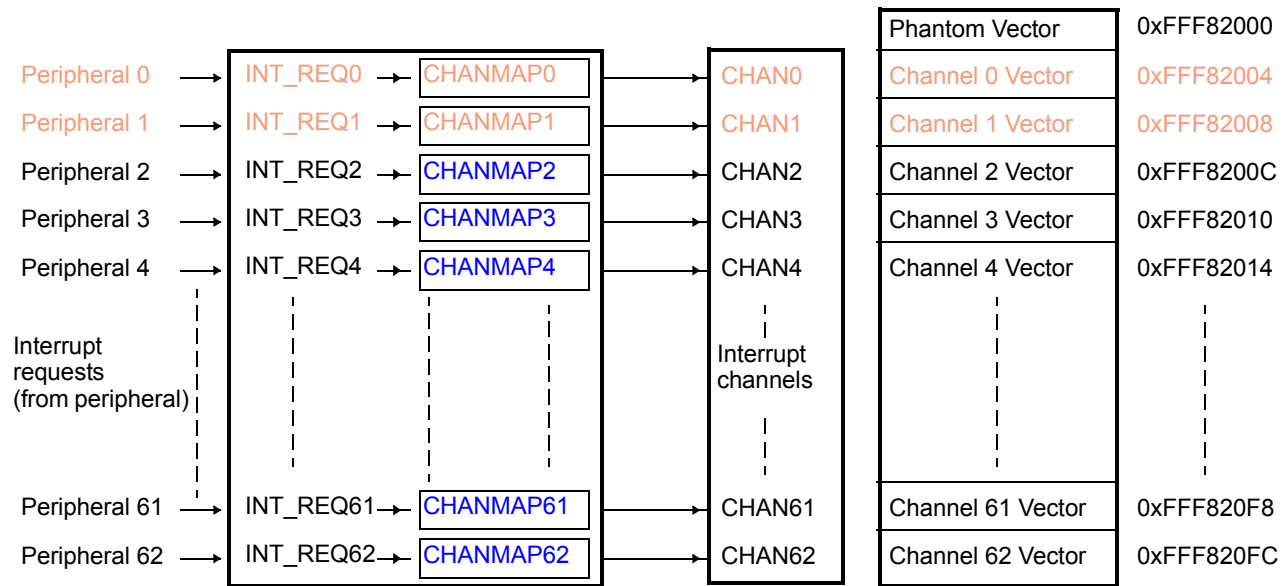
Figure 24-4. VIM in Default State
