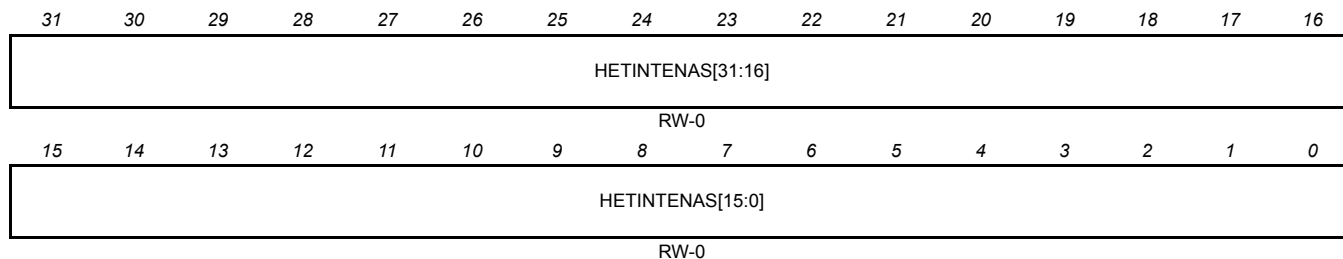
Figure 18-41. NHET Interrupt Enable Set (HETINTENAS) [0xFFF7B814]
