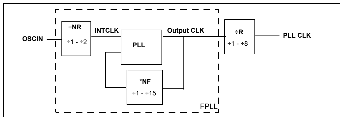
Figure 7-11. FPLL Block Diagram
