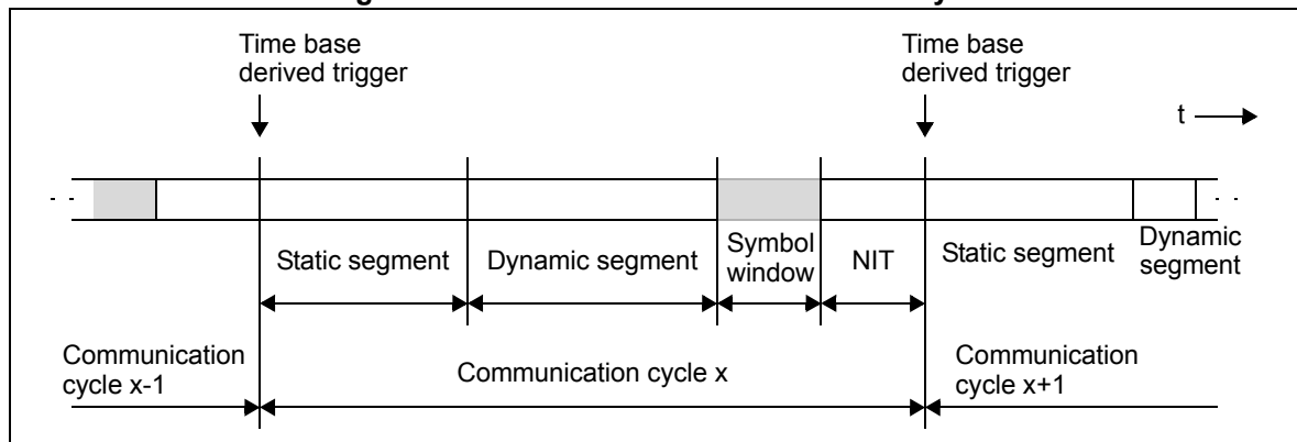
Figure 17-8. Structure of Communication Cycle
