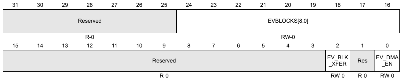
Figure 15-42. ADC Event Group DMA Control Register (ADEVDMACR) [offset = 0x4C]
