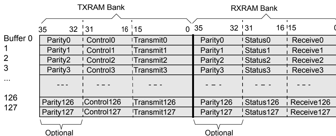
Figure 14-48. Multi-Buffer RAM Configuration
