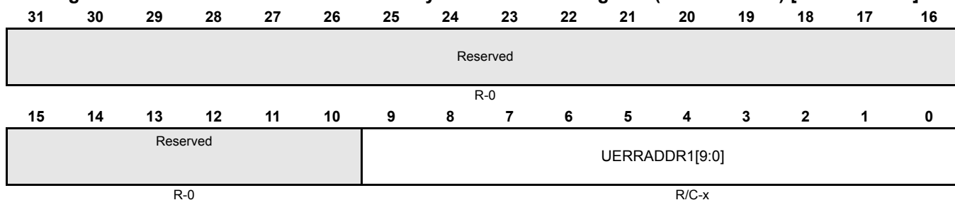
Figure 14-44. RXRAM Uncorrectable Parity Error Address Register (UERRADDR1) [offset = 128h]
