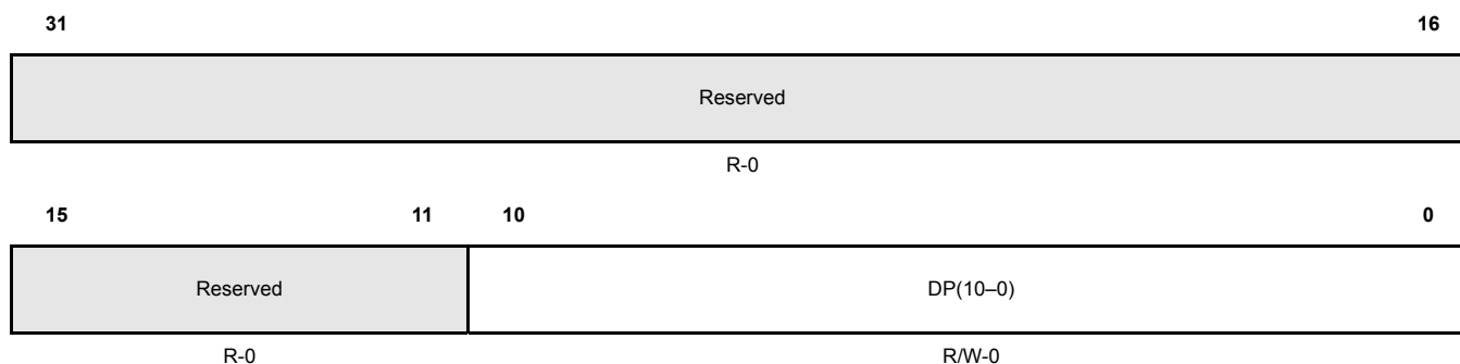
Figure 17-176. Write Header Section Register 3 (WRHS3) [offset_CC = 0x508]
