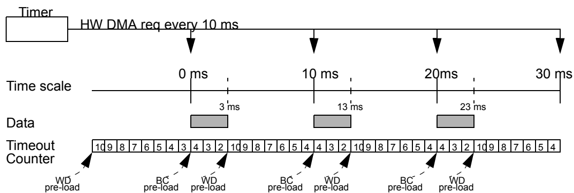
Figure 22-6. Timeout Example 1
