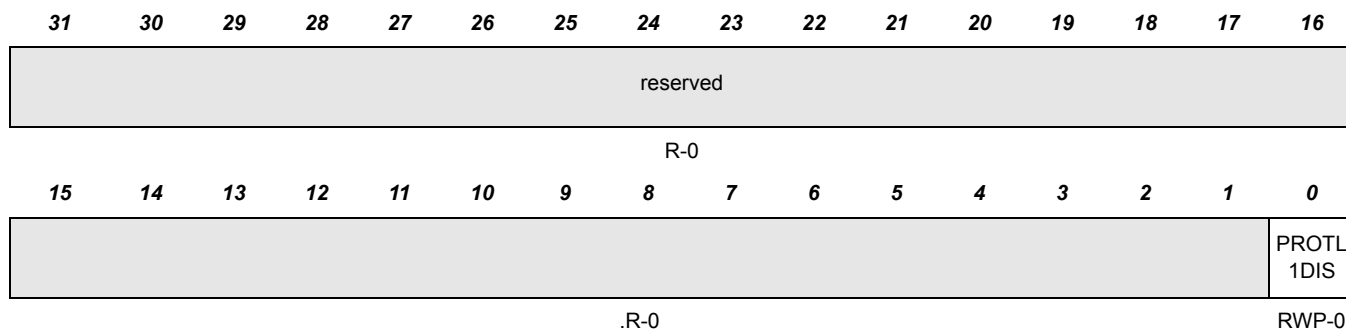
Figure 8-16. Flash Bank Protection Register (FBPROT - 0xFFFF87030)
