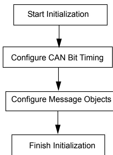
Figure 16-2. CAN module general initialization flow
