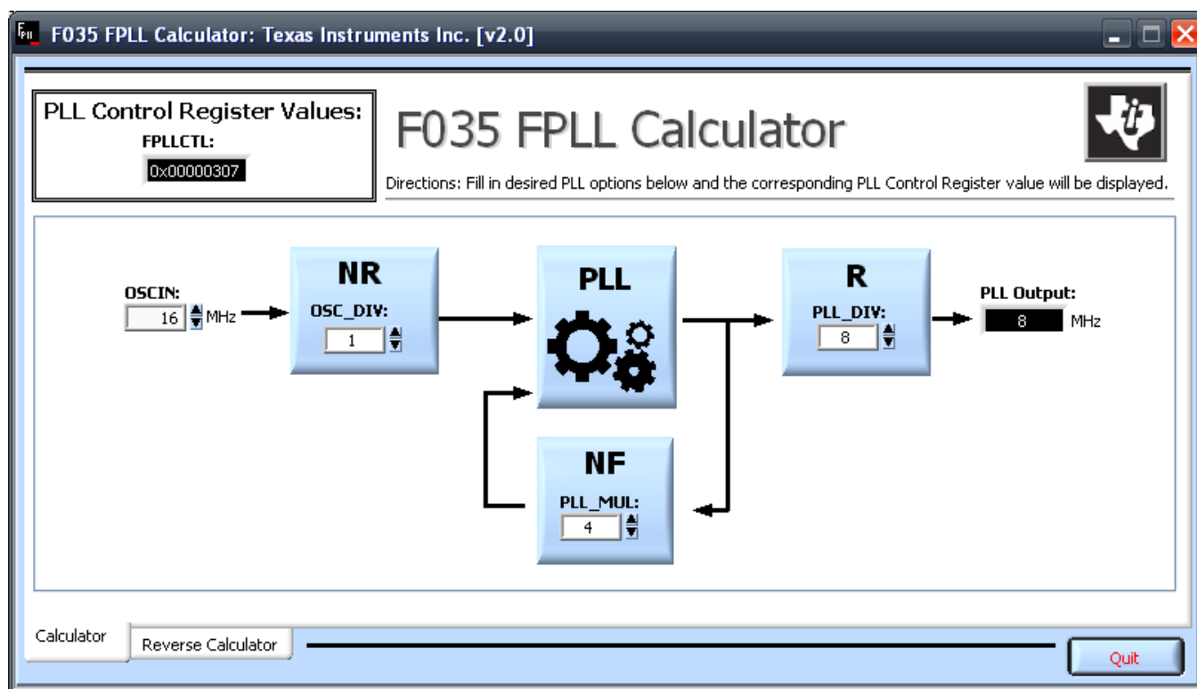
Figure 7-15. F035 FPLL Calculator
