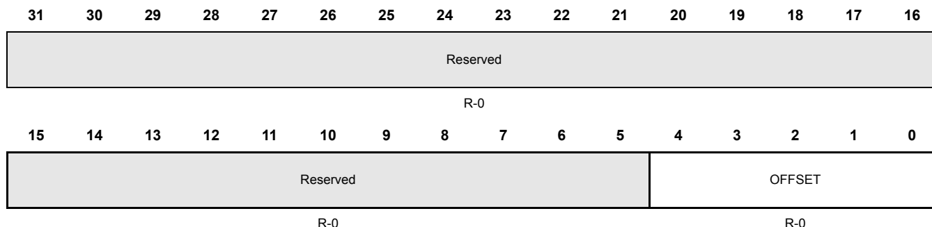
Figure 26-13. DMM Interrupt Offset 1 Register (DMMOFF1) [offset = 14h]
