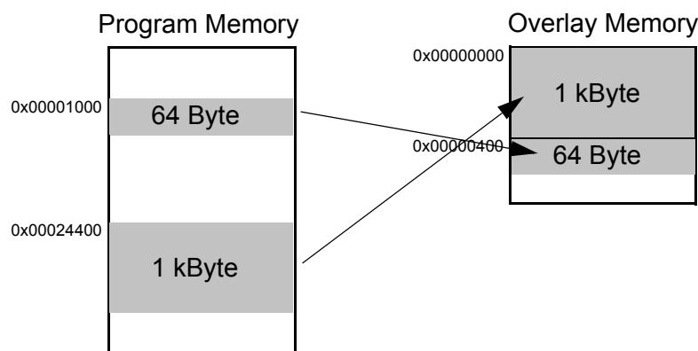
Figure 11-2. Region definition example
