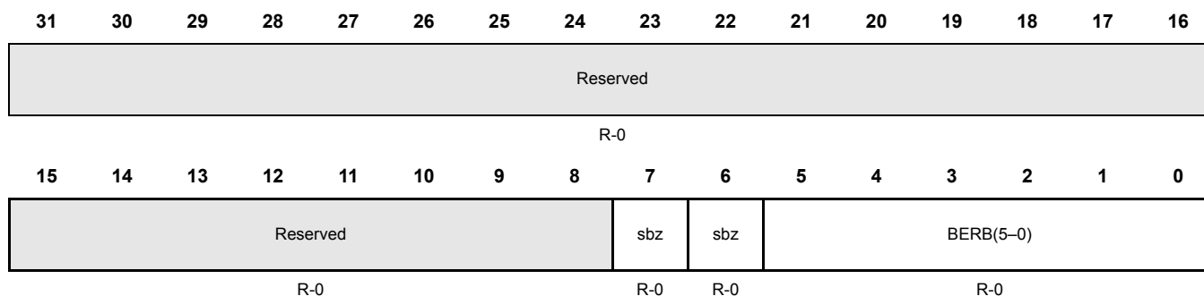
Figure 20-64. BERB Interrupt Channel Offset Register (BERBOFFSET) [offset = 0x170]
