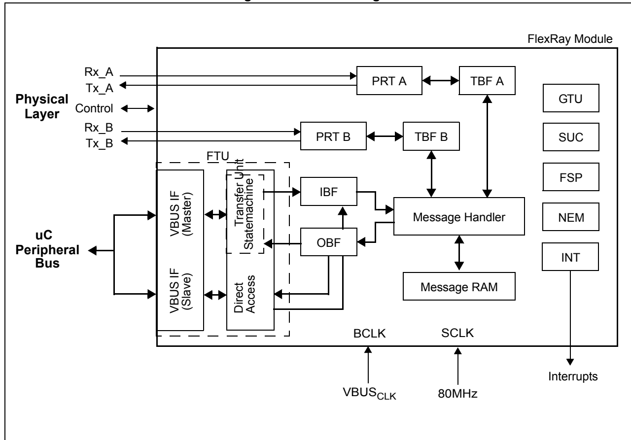
Figure 17-1. Block Diagram
