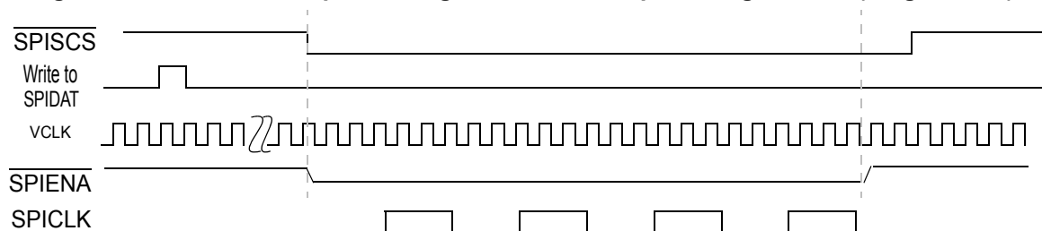
Figure 14-59. SPI/MibSPI pins during Slave mode in 5pin configuration - (Single Slave).
