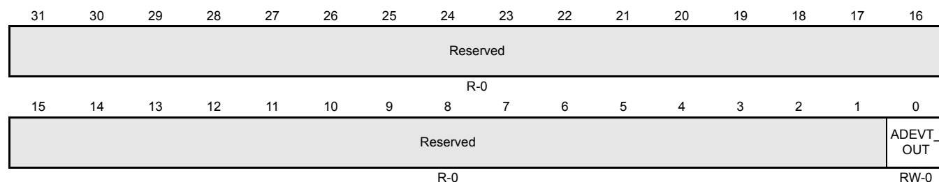
Figure 15-62. ADC ADEVT Pin Output Value Control Register (ADEVTOUT) [offset = 0x100]
