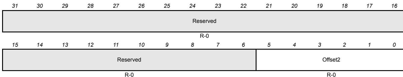
Figure 18-40. Offset Index Priority Level 2 Register (HETOFF2) [0xFFF7B810]
