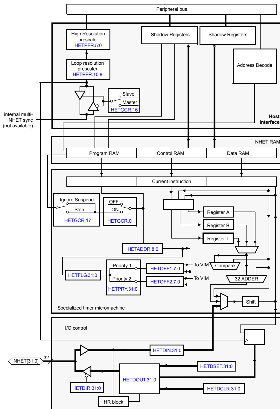
Figure 18-1. NHET Block Diagram
