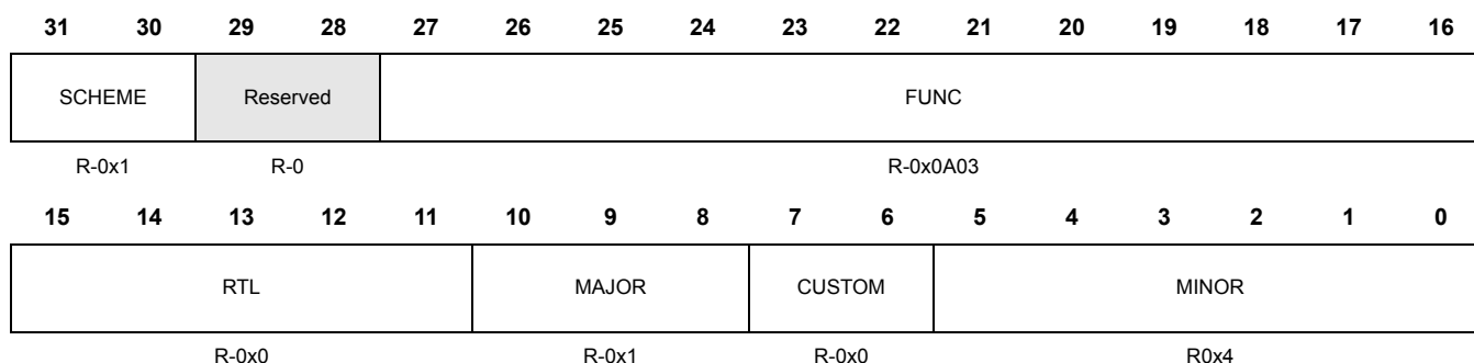
Figure 11-4. POM Revision ID (POMREV) [offset = 0x04h]
