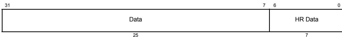
Figure 18-143. WCAP Data Field (D31:D0)
