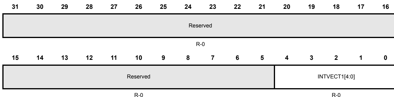
Figure 13-37. SCI Interrupt Vector Offset 1 (SCIINTVECT1) [offset = 0x24
