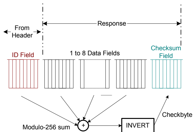
Figure 13-23. LIN 2.0-Compliant Checksum Generation at Transmitting Node
