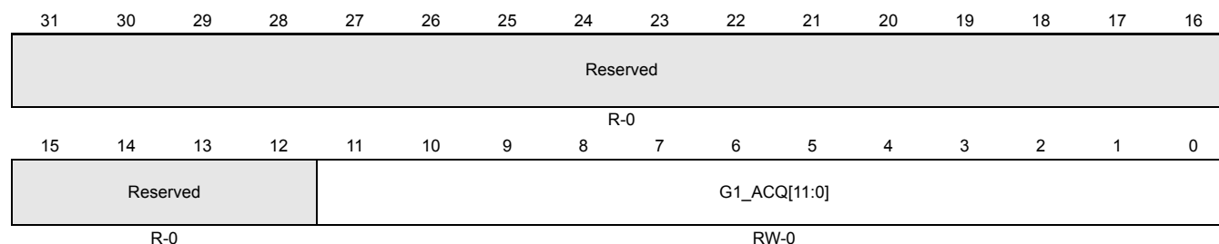
Figure 15-48. ADC Group1 Sampling Time Configuration Register (ADG1SAMP) [offset = 0x64]
