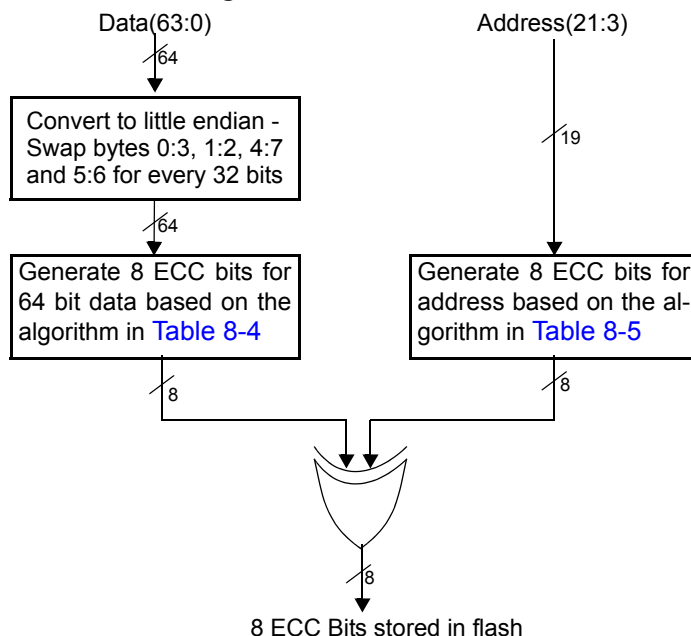
Figure 8-5. Flash ECC Calculation
