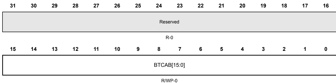
Figure 20-39. BTC Interrupt Mapping Register (BTCMAP) [offset = 0xCC]
