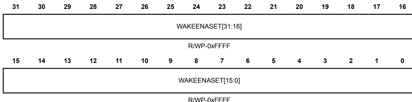
Figure 24-26. Wake-Up Enable Set Register 0 (WAKEENASET0) [0xFFFFFE50]
