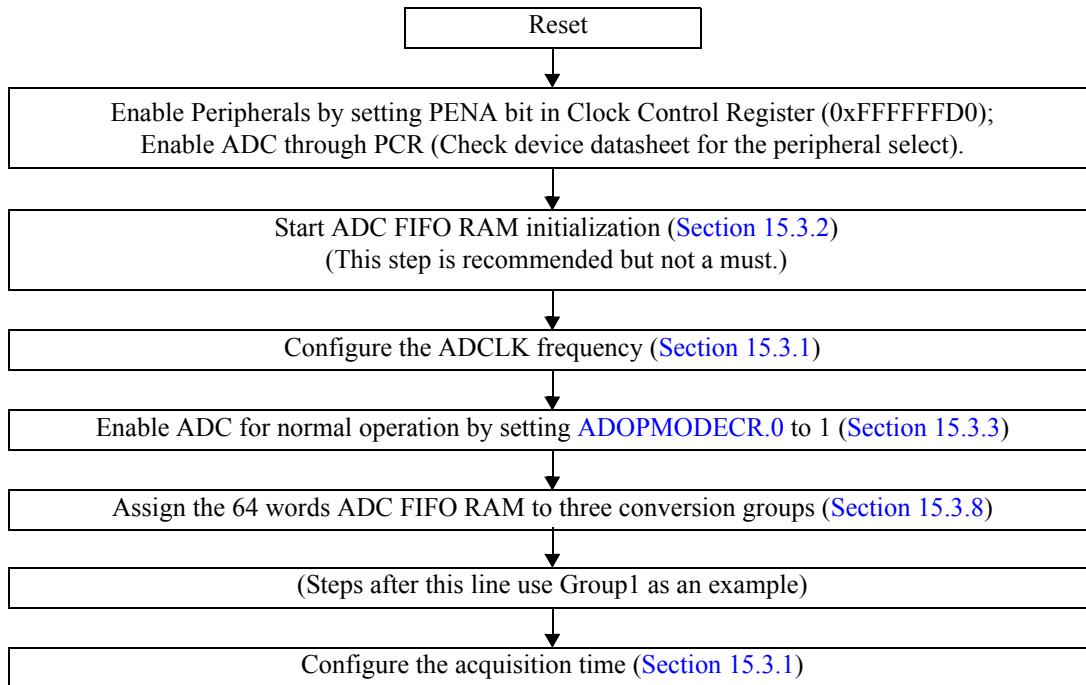
Figure 15-3. ADC Initialization Flow Chart
