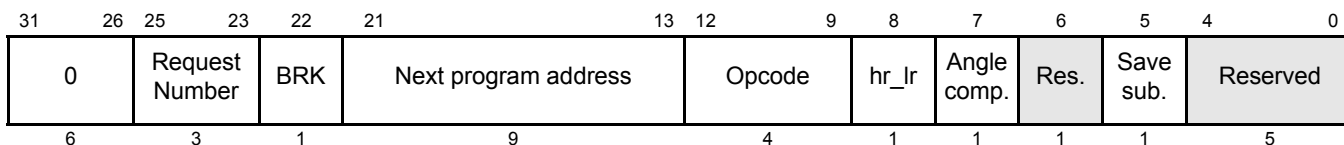
Figure 18-109. MCMP Control Field (C31:C0)
