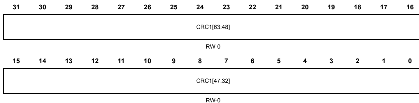
Figure 22-26. Channel 1 CRC value high register(CRC_REGH1) [offset = 0x6C]
