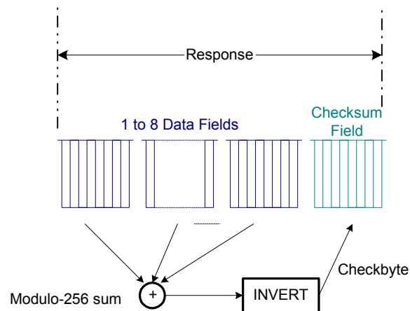
Figure 13-23. LIN 2.0-Compliant Checksum Generation at Transmitting Node
