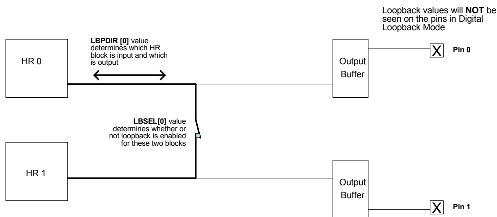
Figure 18-16. HR0 to HR1 Digital Loopback Logic: LBTYPE[0] = '0'
