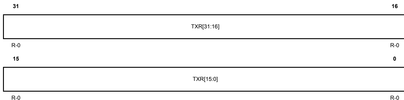
Figure 17-162. Transmission Request Register 1 (TXRQ1) [offset_CC = 0x320]
