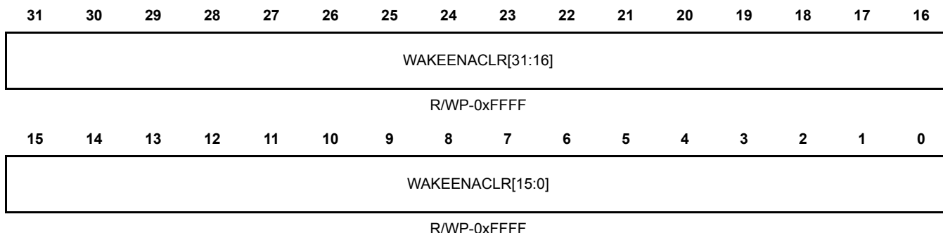
Figure 24-28. Wake-Up Enable Clear Register 0 (WAKEENACLR0) [0xFFFFFE60]
