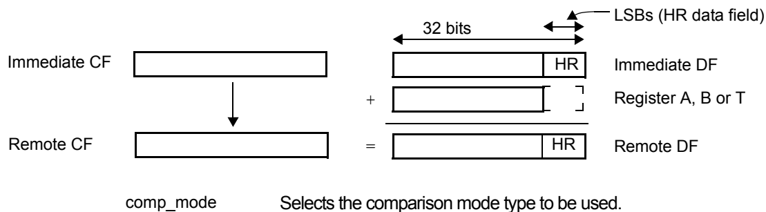
Figure 18-131. RADM64 Add and Move Operation
