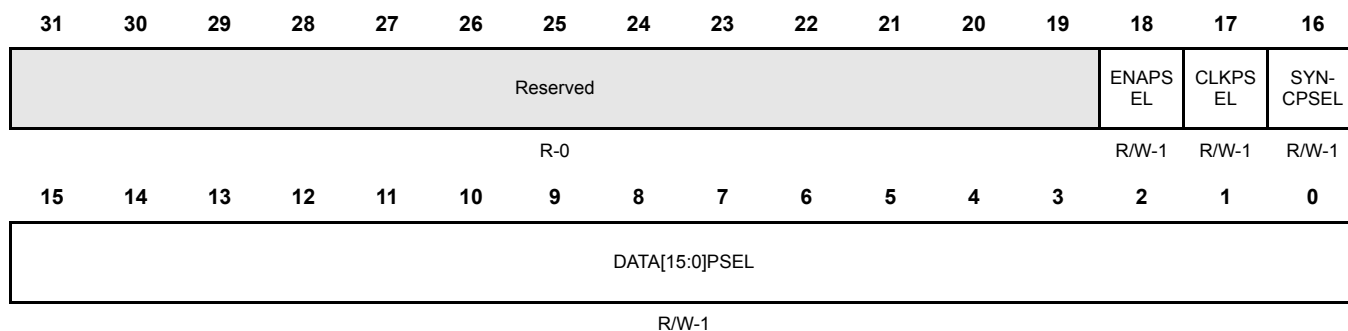
Figure 27-24. RTP Pin Control 8 Register (RTPPC8) [offset = 54h]
