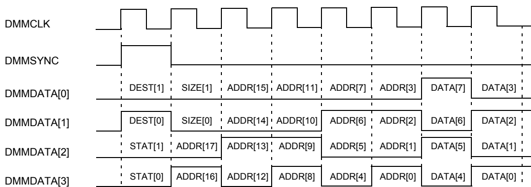
Figure 26-5. Example Single Packet Transmission
