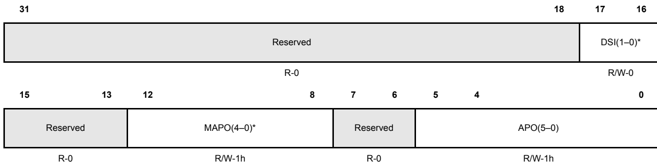
Figure 17-135. GTU Configuration Register 9 (GTUC9) [offset_CC = 0xC0]
