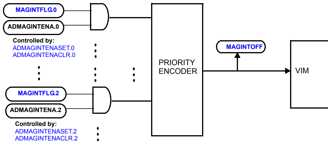
Figure 15-14. Magnitude Threshold Interrupt Generation
