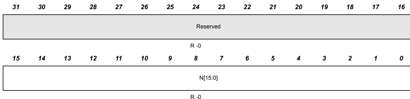
Figure 9-9. STC Current Interval Count Register (STCCICR)
