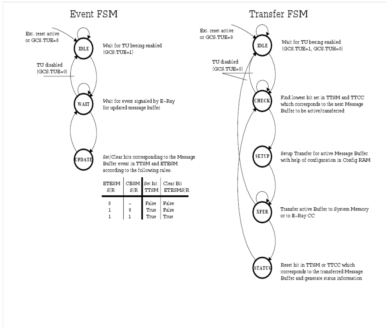
Figure 17-4. FlexRay Transfer Unit Operation Principle (simplified)
