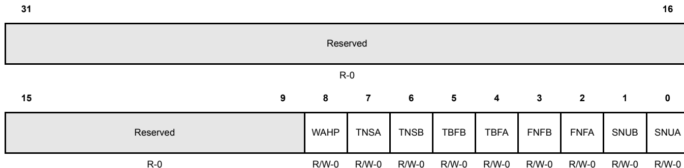
Figure 17-158. Message Handler Constraints Flags (MHDF) [offset_CC = 0x31C]
