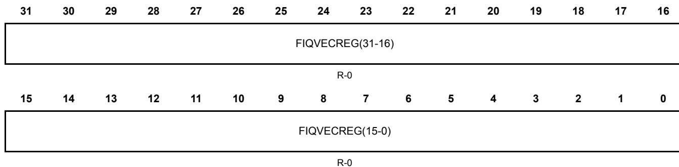
Figure 24-31. IRQ Interrupt Vector Register (FIQVECREG) [0xFFFFFE74]
