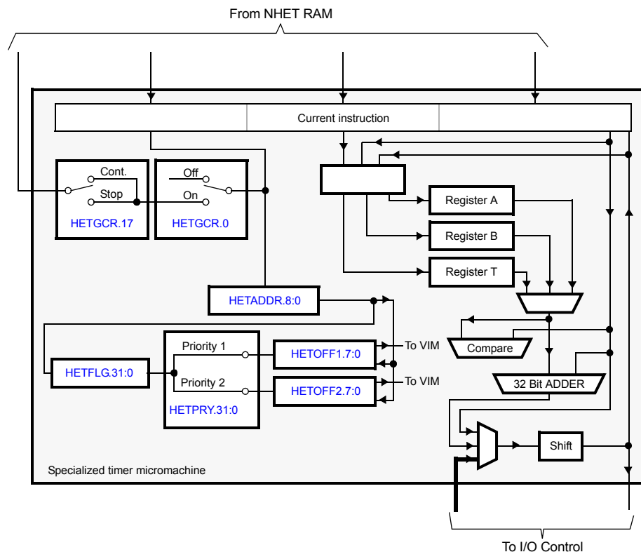
Figure 18-2. Specialized Timer Micromachine
