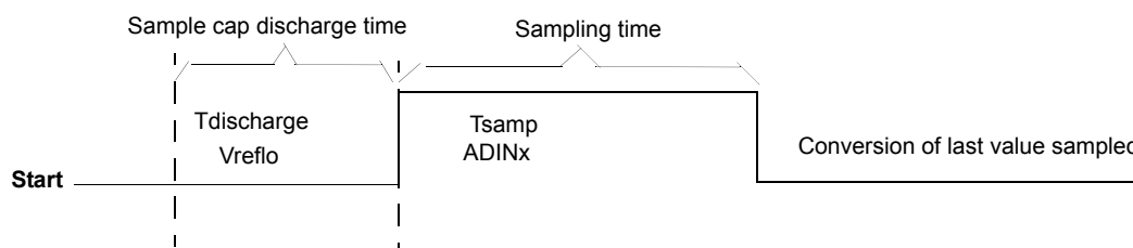
Figure 15-21. Timing for Sample Capacitor Discharge Mode
