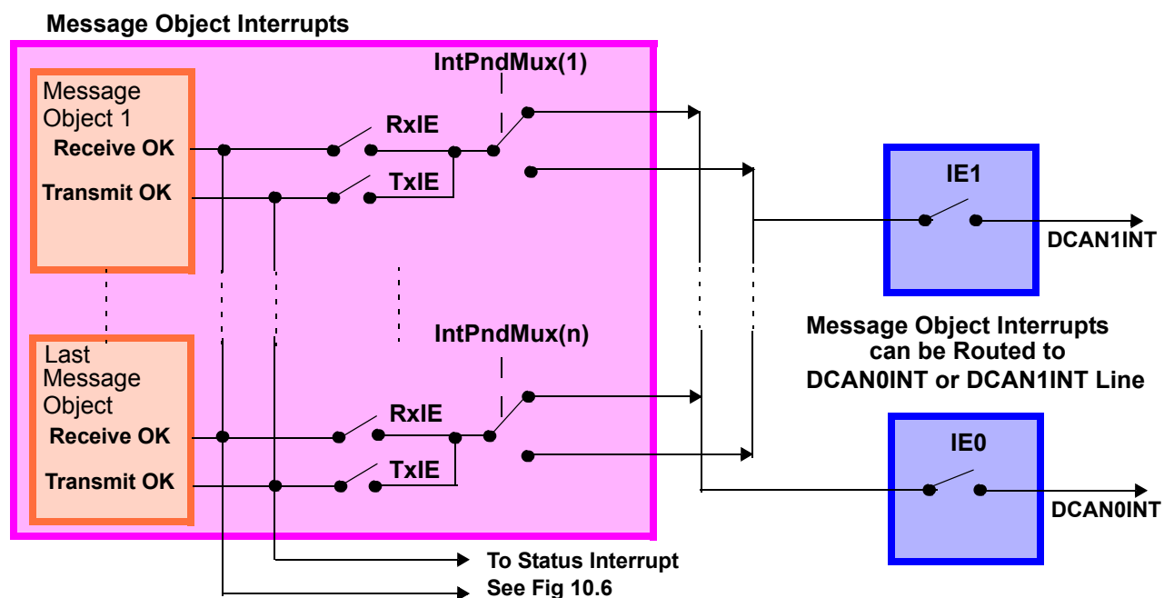
Figure 16-9. CAN Interrupt Topology 2
