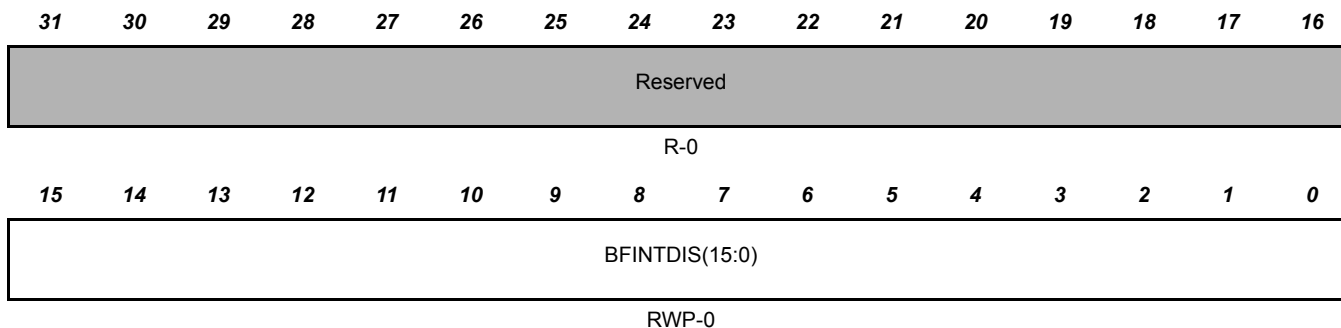
Figure 19-25. Buffer Full Interrupt Enable Clear Register (HTU BFINTC) [offset = 0x28]
