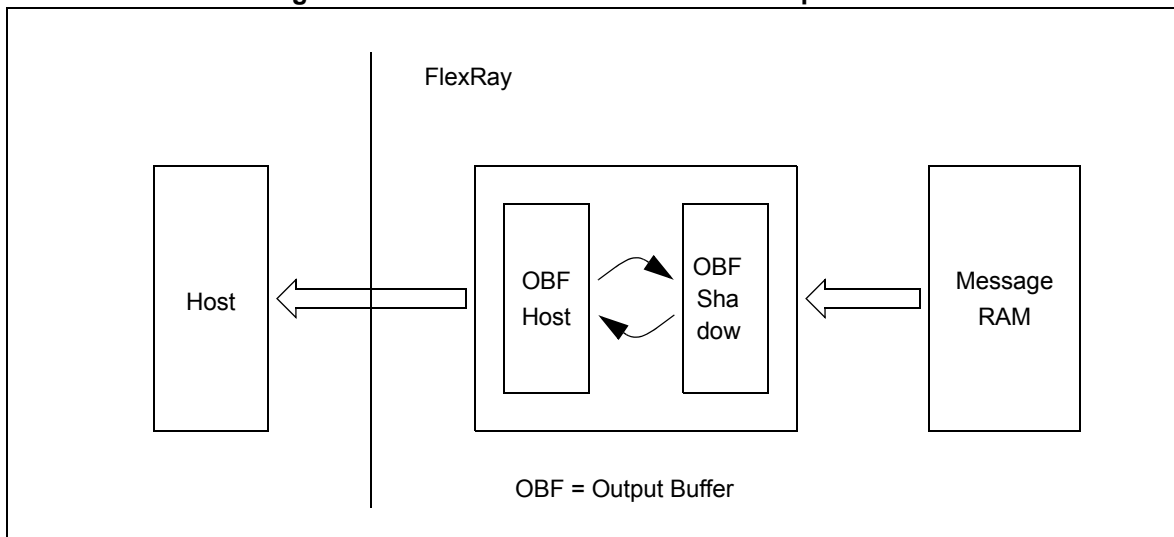
Figure 17-18. Double Buffer Structure Output Buffer
