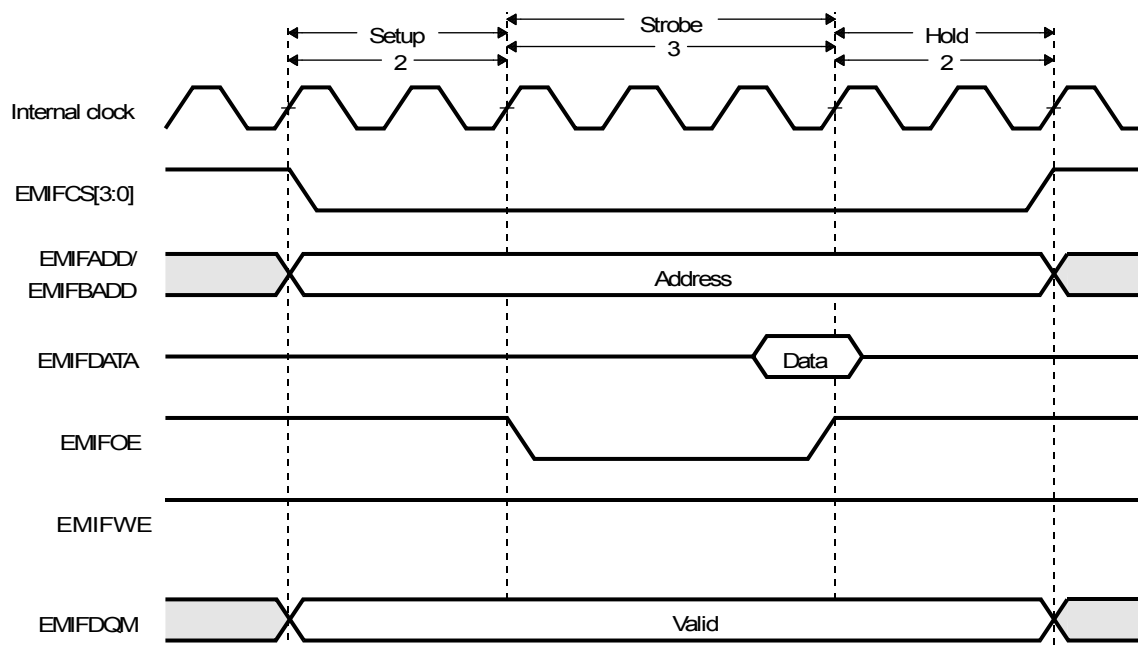
Figure 10-4. Timing Waveform of an Asynchronous Read Cycle in Normal Mode
