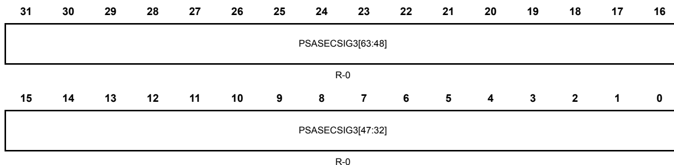
Figure 22-54. Channel 3 PSA sector signature high register(PSA_SECSIGREGH3) [offset = 0xF4]
