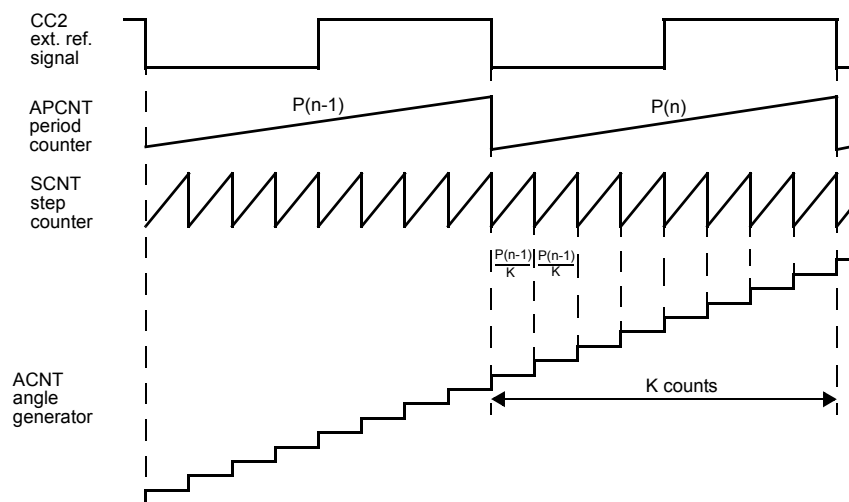
Figure 18-30. Operation of NHET Count Instructions
