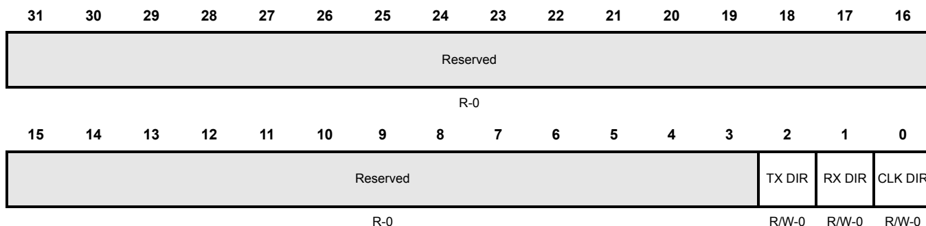
Figure 13-44. SCI Pin I/O Control Register 1 (SCIPIO1) [offset = 0x40]
