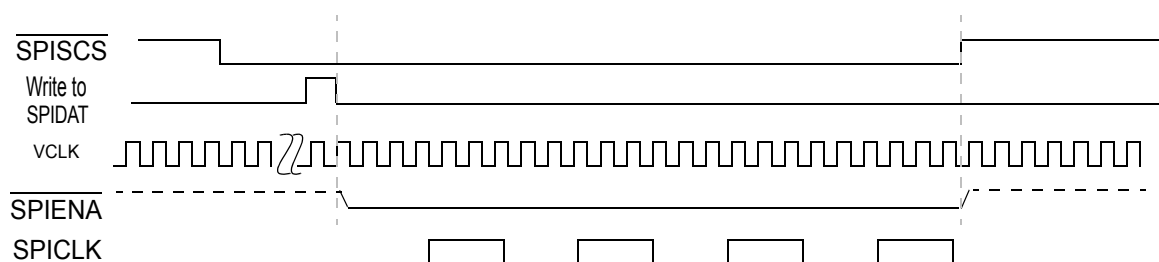
Figure 14-60. SPI/MibSPI pins during Slave mode in 5pin configuration - (Single/Multi Slave).
