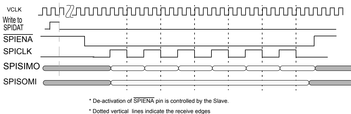
Figure 14-55. SPI/MibSPI pins during Master mode in 4pin with \overline{\text{SPIENA}} configuration
