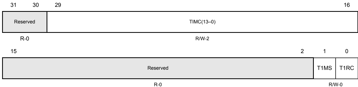
Figure 17-117. Timer 1 Configuration Register (T1C) [offset_CC = 0x48]
