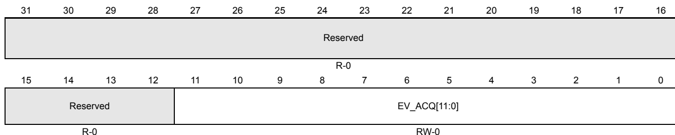
Figure 15-47. ADC Event Group Sampling Time Configuration Register (ADEVSAMP) [offset = 0x60]
