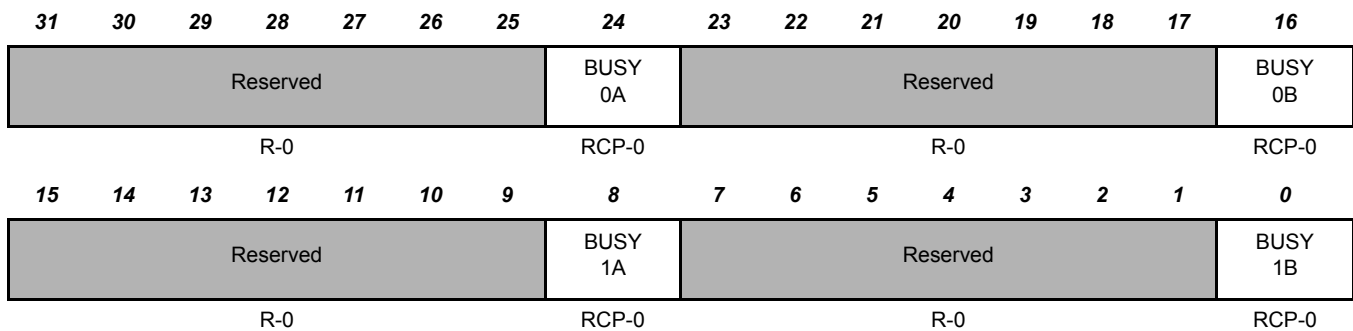
Figure 19-18. Control Packet (CP) Busy Register 0 (HTU BUSY0) [offset = 0x08]
