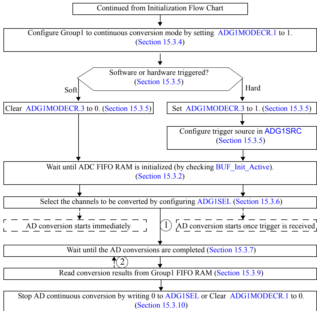
Figure 15-5. Flow Chart for Continuous Conversion
