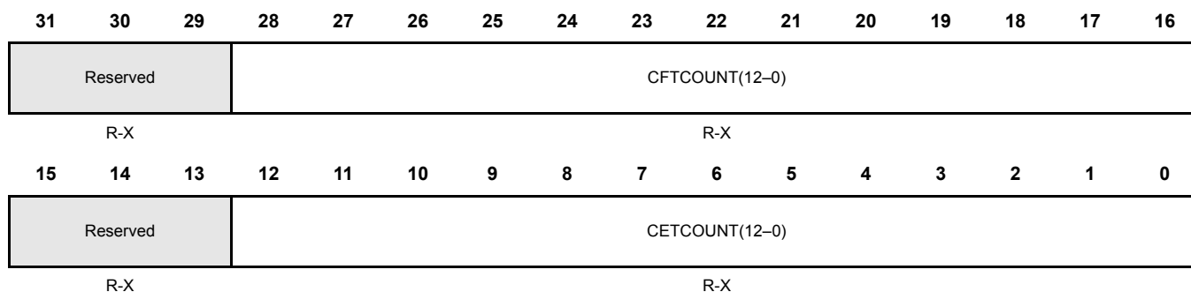
Figure 20-93. Current Transfer Count Register (CTCOUNT) [offset = 0x808]
