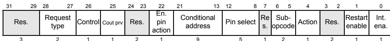
Figure 18-134. SCMP Data Field (D31:D0)
