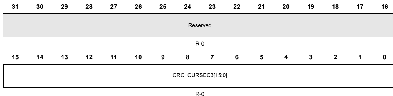
Figure 22-46. CRC Current Sector Register 3(CRC_CURSEC_REG3) [offset = 0xC8]
