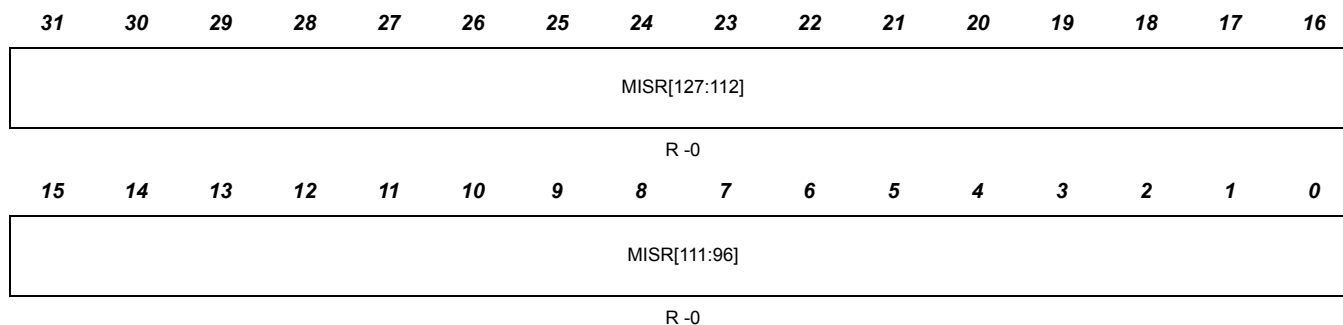
Figure 9-15. CPU1 Current MISR Register (CPU1_CURMISR0)
