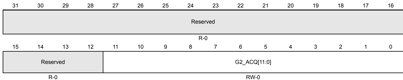
Figure 15-49. ADC Group2 Sampling Time Configuration Register (ADG2SAMP) [offset = 0x68]
