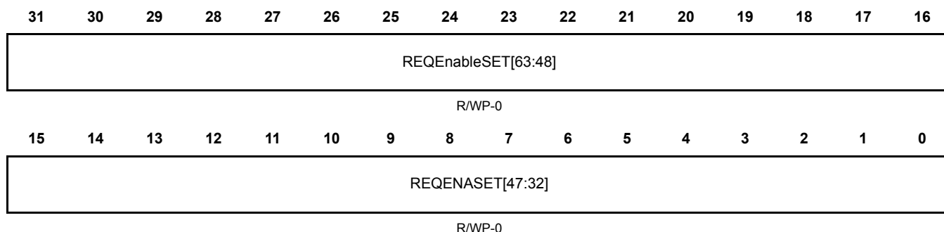
Figure 24-23. Interrupt Enable Set Register 1 (REQENASET1) [0xFFFFFE34]
