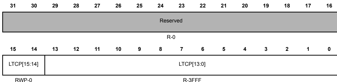
Figure 25-19. ESM Low-Time Counter Preload Register (ESMLTCPR)
