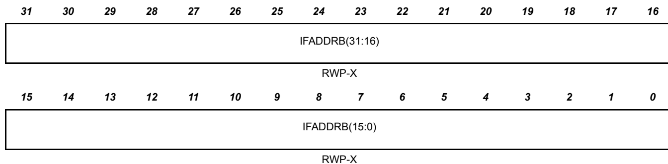
Figure 19-47. Initial Full Address B Register (HTU IFADDRB)
