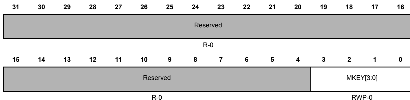
Figure 23-4. CCM-R4F Key Register (CCMKEYR)
