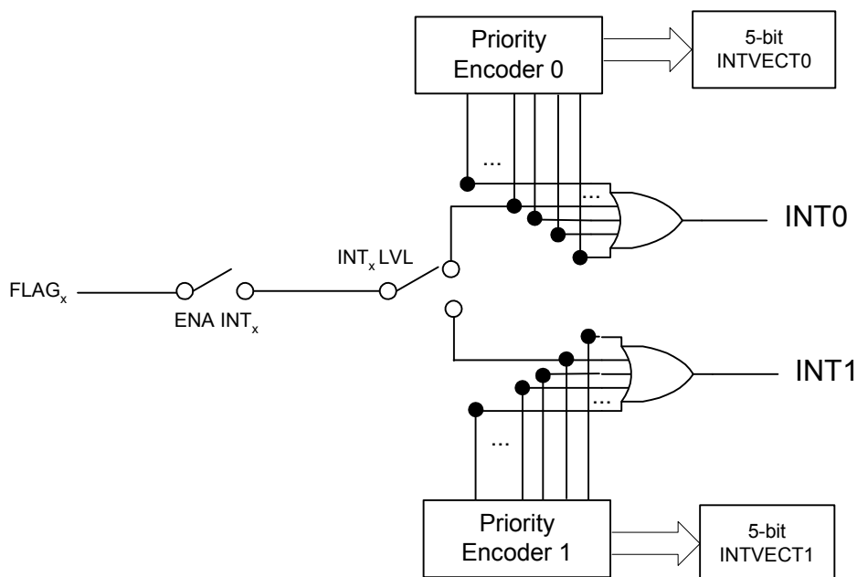
Figure 13-11. Interrupt Generation for Given Flags
