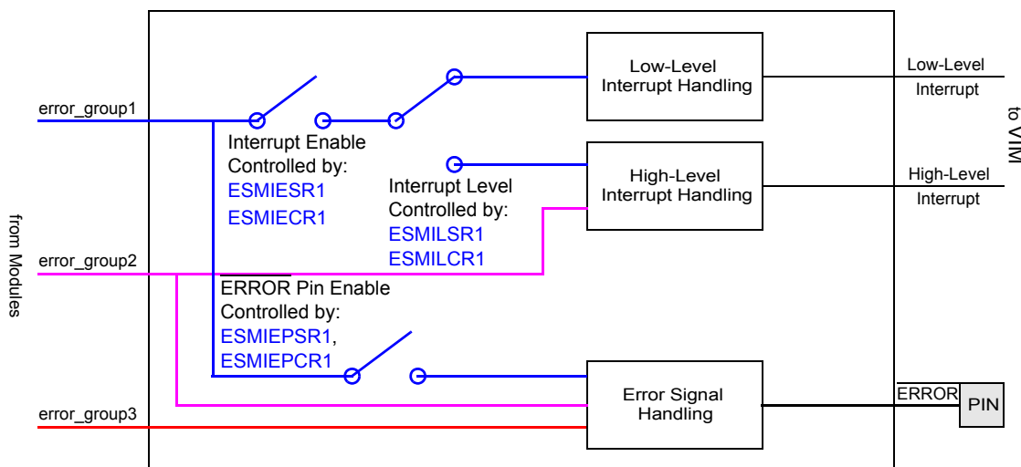
Figure 25-1. Block Diagram
