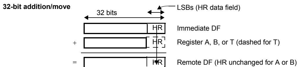
Figure 18-85. ADM32 Add and Move Operation for IM&REGTOREM (Case 11)
