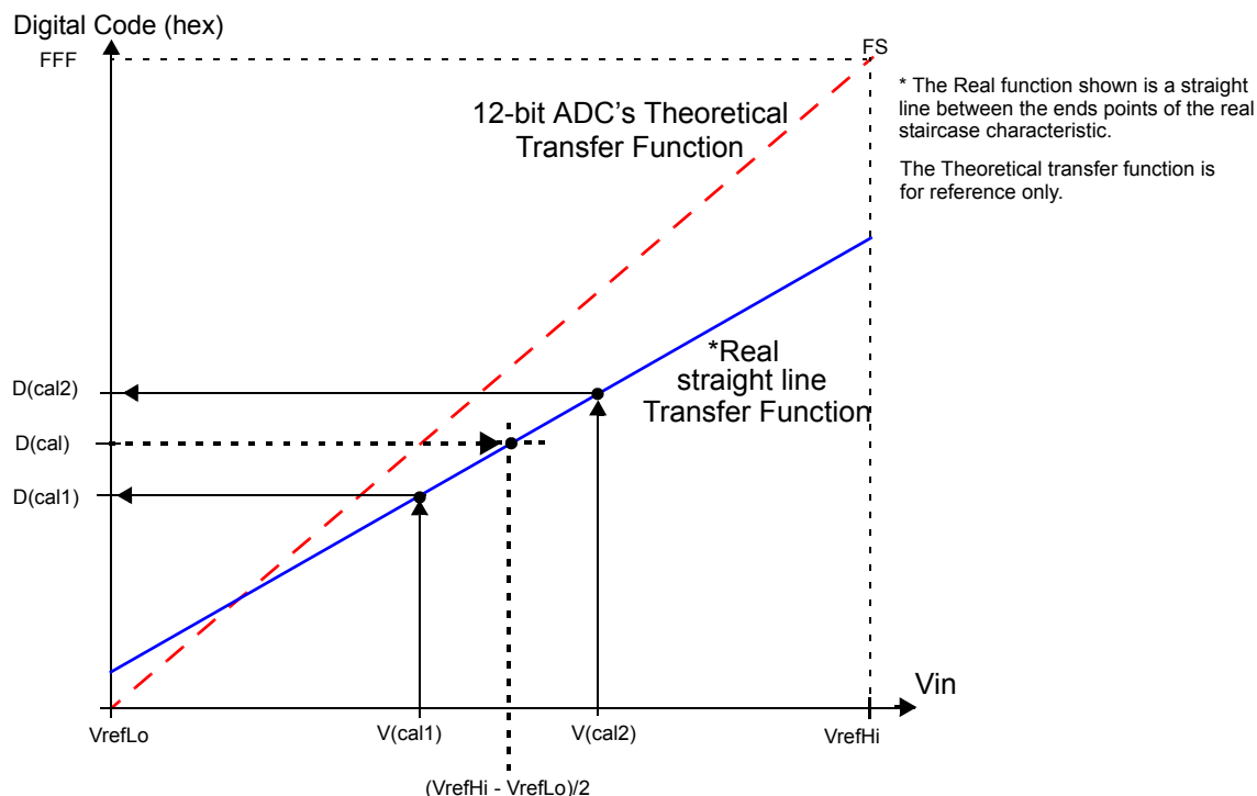
Figure 15-17. Mid-point value calculation
