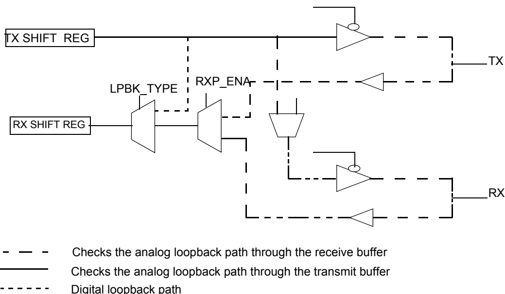
Figure 14-23. I/O Paths during I/O Loopback Modes
