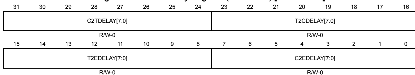
Figure 14-19. SPI Delay Register (SPIDELAY) [offset = 48h]
