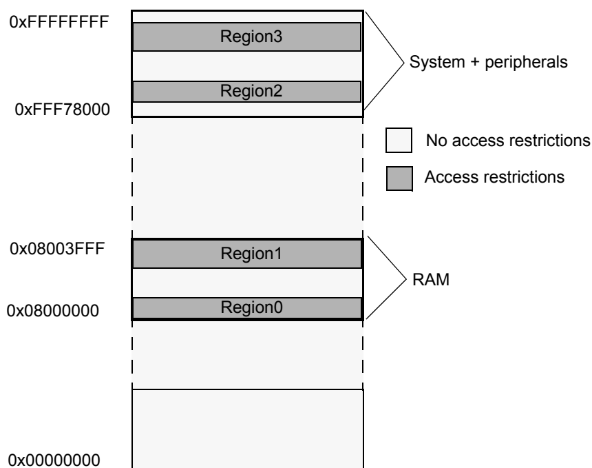
Figure 20-17. Example of Protection Mechanism
