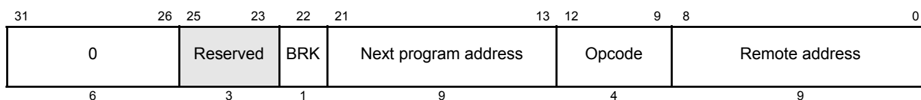
Figure 18-80. ADM32 Control Field (C31:C0)
