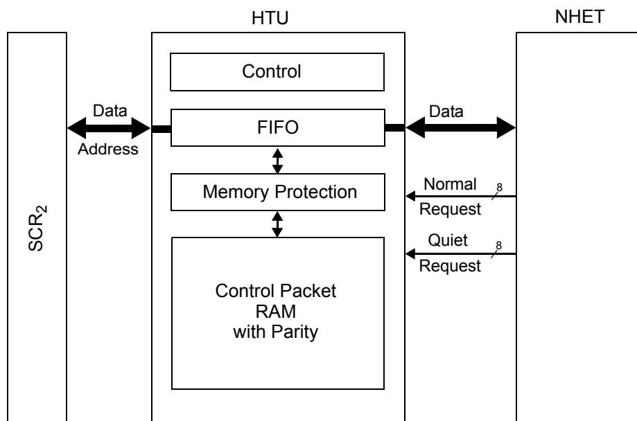
Figure 19-2. HTU Block Diagram
