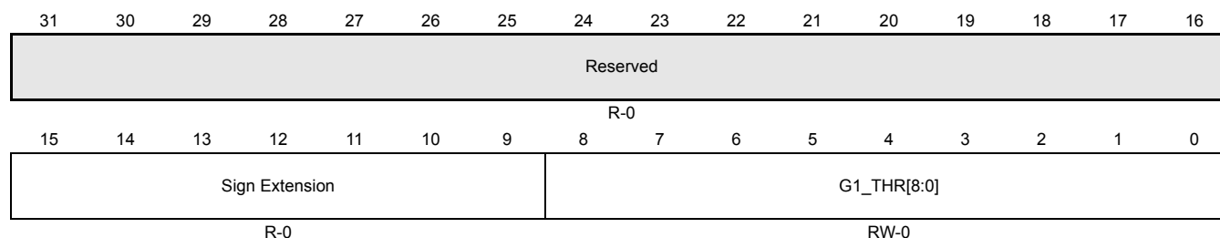
Figure 15-40. ADC Group1 Threshold Interrupt Control Register (ADG1THRINTCR) [offset = 0x44]
