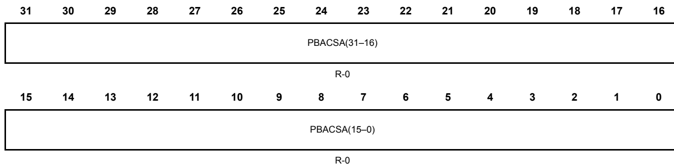
Figure 20-70. Port B Active Channel Source Address Register (PBACSADDR) [offset = 0x198]
