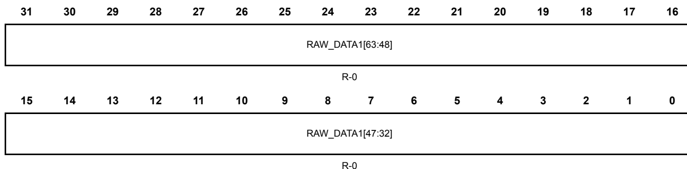
Figure 22-30. Channel 1 Raw Data High Register(RAW_DATAREGH1) [offset = 0x7C]
