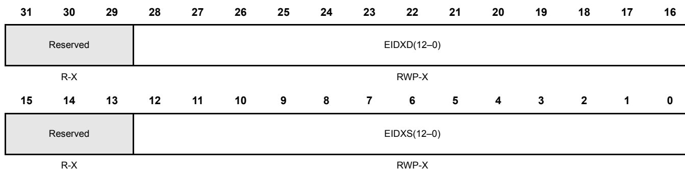
Figure 20-89. Element Index Offset Register (EIOFF) [offset = 0x014]
