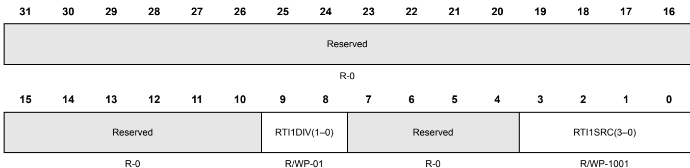
Figure 5-19. RTI Clock Source Register (RCLKSRC) [offset = 0x50]
