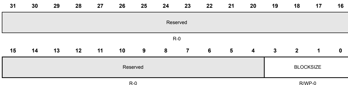
Figure 26-16. DMM Direct Data Mode Blocksize Register (DMMDDMBL) [offset = 20h]
