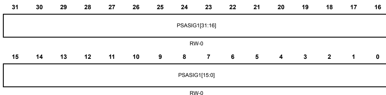
Figure 22-23. Channel 1 PSA signature low register(PSA_SIGREGL1) [offset = 0x60]
