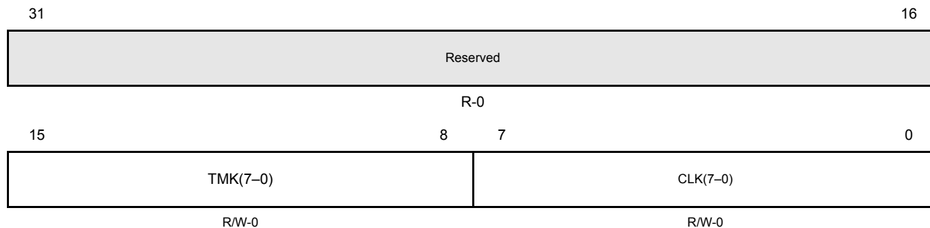
Figure 17-108. Lock Register (LCK) [offset_CC = 0x1C]
