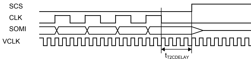
Figure 14-21. Example: t_{T2CDELAY} = 4 VCLK Cycles
