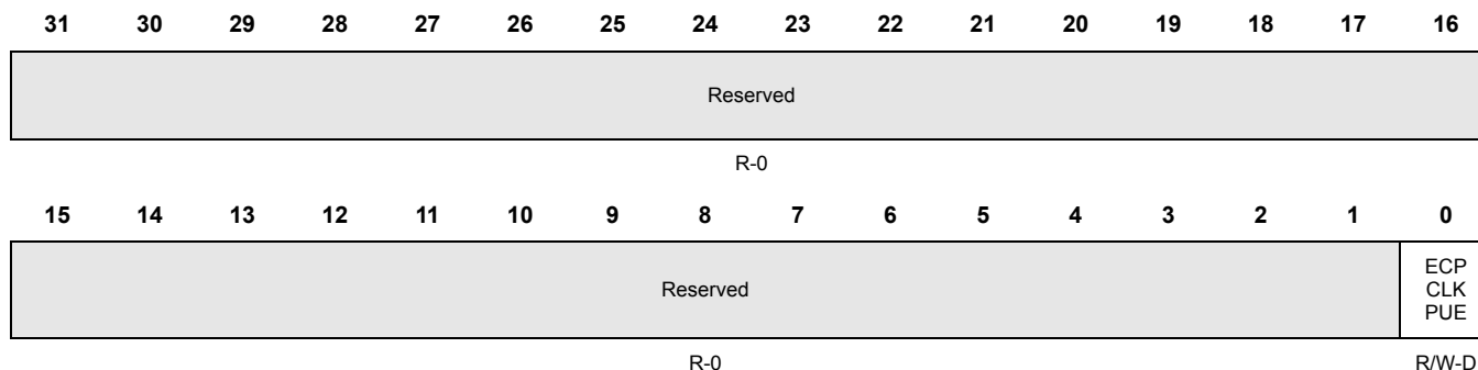
Figure 5-9. SYS Pin Control Register 8 (SYSPC8) [offset = 0x1C]
