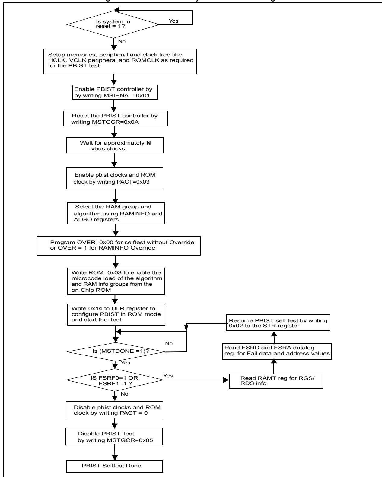
Figure 6-2. PBIST Memory Self Test Flow Diagram
