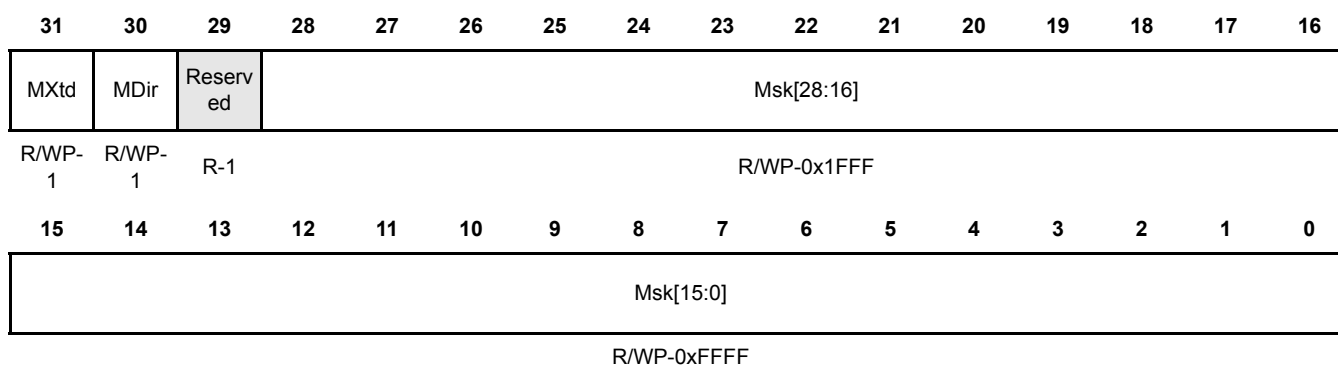
Figure 16-45. IF2 Mask Register (DCAN IF2MSK) [offset = 0x124]
