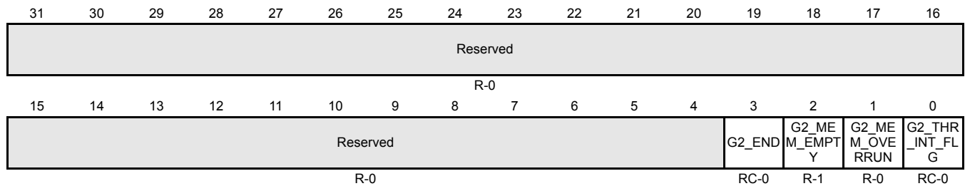
Figure 15-38. ADC Group2 Interrupt Flag Register (ADG2INTFLG) [offset = 0x3C]
