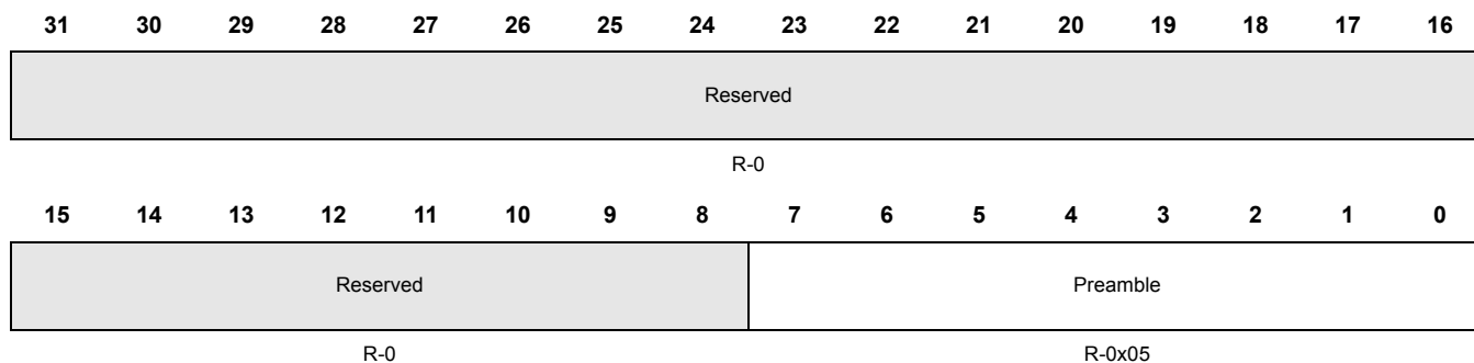
Figure 11-27. POM Component ID 2 Register (POMCPOMPONENTID2) [offset = 0xFF8]
