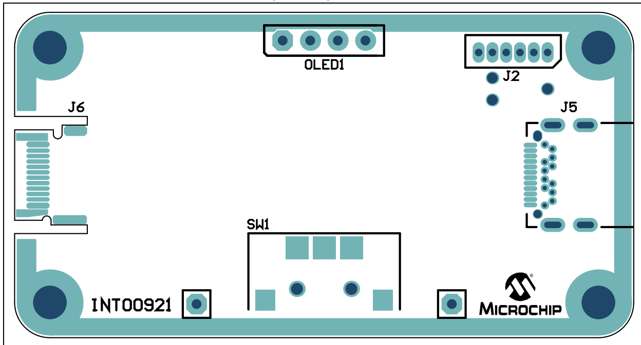
A.14 BOARD – TOP SILK LAYER (USB C)
