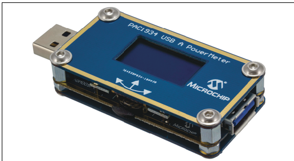
FIGURE 1-1: PAC1934 Power Meter.
