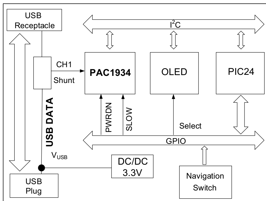
FIGURE 3-1: Block Diagram PAC1934 USB-A.
