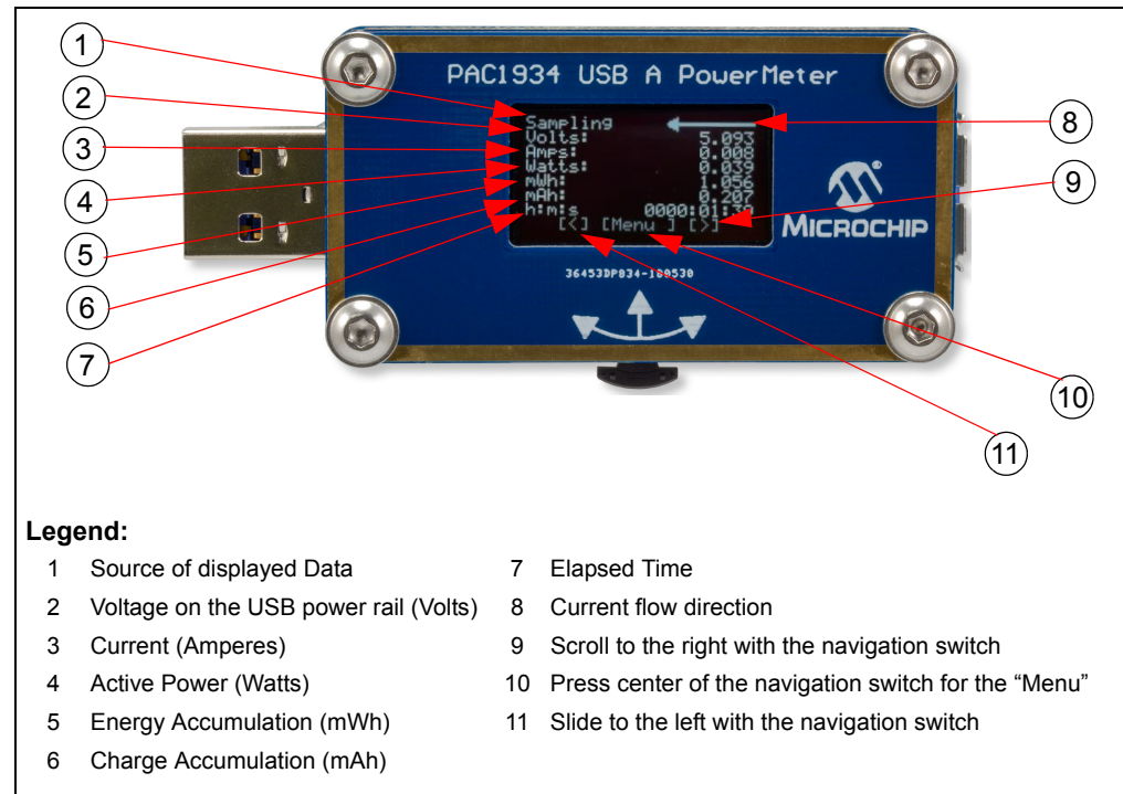
FIGURE 2-3: Main Display.
