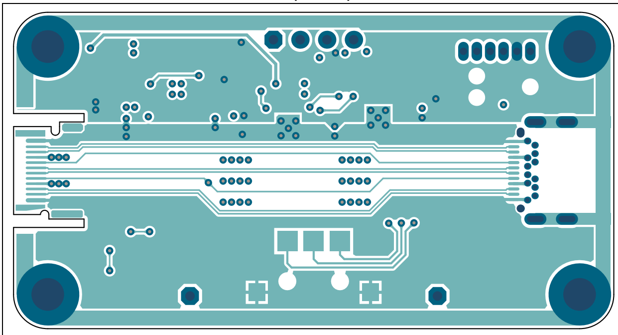
A.16 BOARD – TOP COPPER LAYER (USB C)
