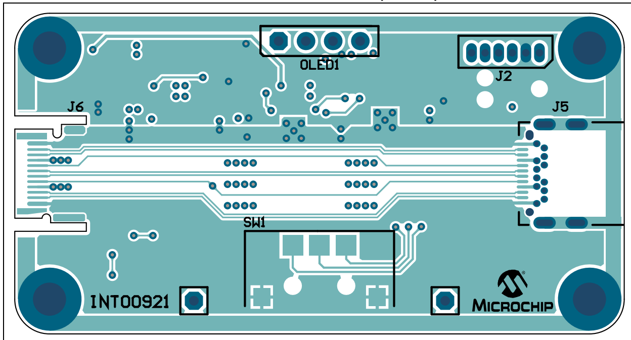
A.15 BOARD – TOP COPPER AND SILK LAYER (USB C)
