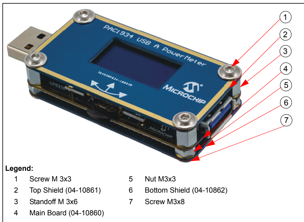
FIGURE 4-1: PAC1934 Power Meter Assembly.
