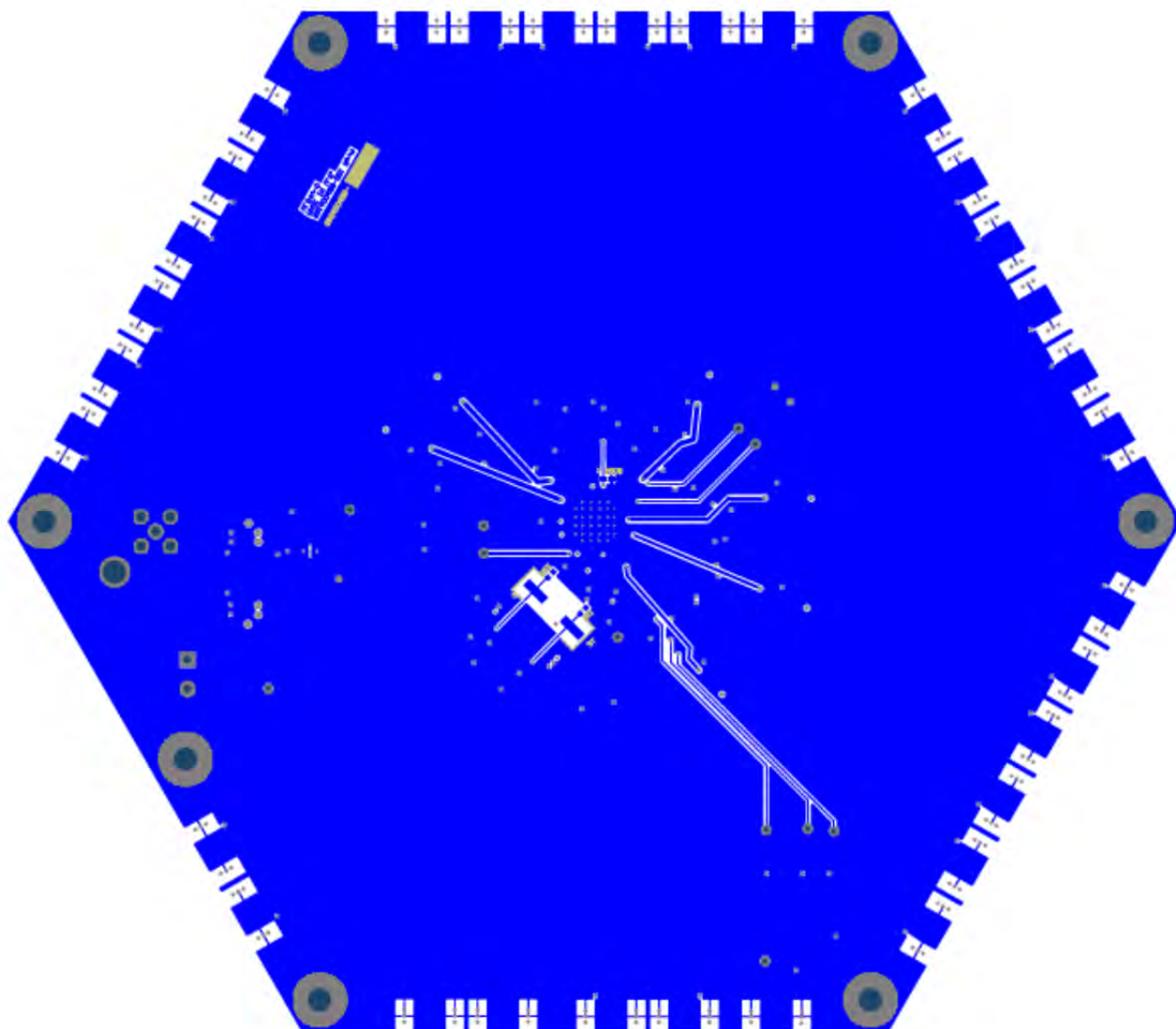
Figure 25: Layer 4 - Bottom
