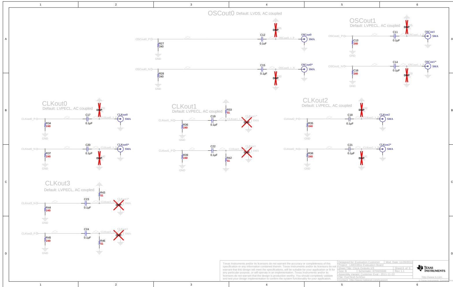
Figure 18 - Outputs, (OSCont, CLKout0/1/2/3) Schematics
