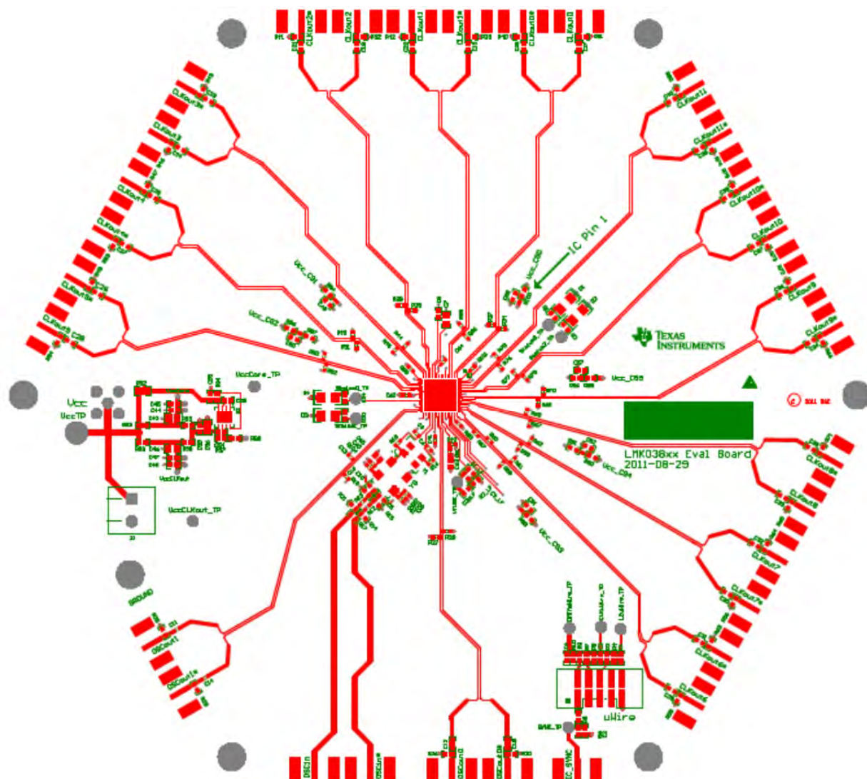
Figure 22: Layer 1 - Top
