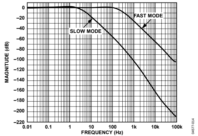
Figure 34. Frequency Response of the Digital Servo Loop; f_{S\_IN} is the X-Axis, f_{S\_OUT} = 192 kHz, Master Clock is 30 MHz
