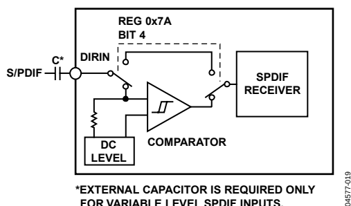
Figure 39. DIRIN Block
