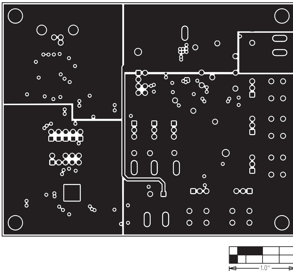
Figure 11. MAX6948 EV Kit PCB Layout—Layer 3
