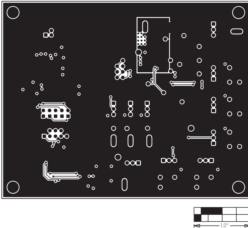
Figure 12. MAX6948 EV Kit PCB Layout—Solder Side
