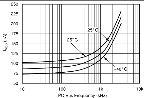
Figure 3. Supply Current vs I²C Bus Frequency
