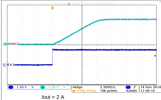
Figure 46. BUCK3, Soft-Start
