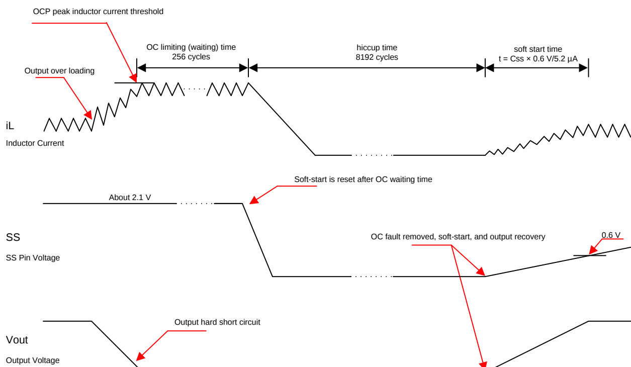
Figure 31. Overcurrent Protection
