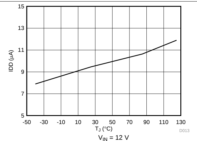
Figure 12. Shutdown Quiescent Current vs Temperature
