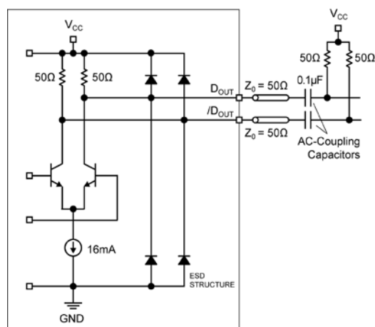
Figure 3. Output Structure
