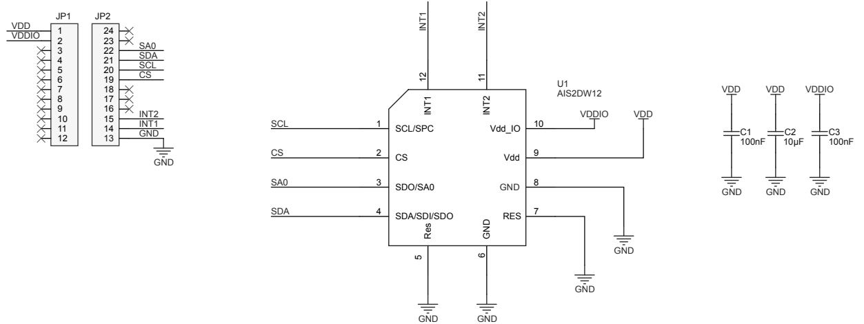
Figure 1. STEVAL-MKI206V1 circuit schematic
