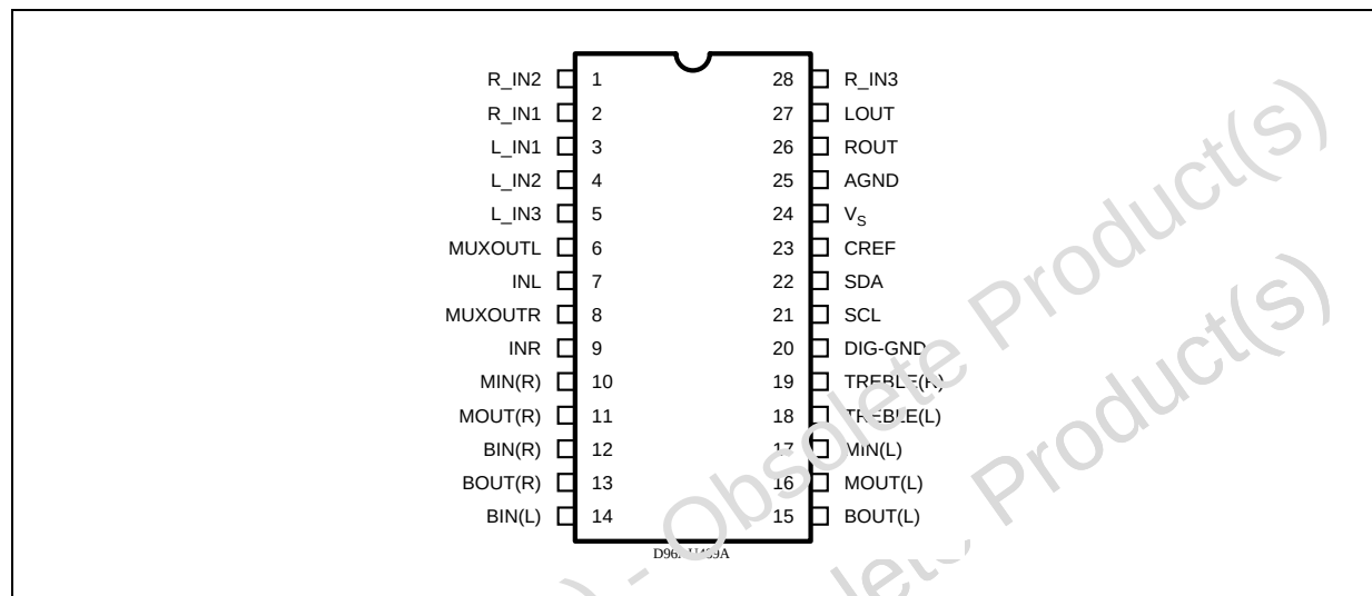
Figure 3. Pin Connection
