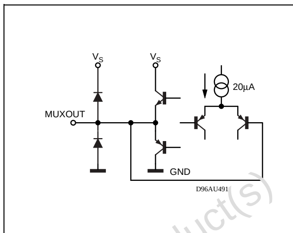
Figure 24. PINS: 7, 9
