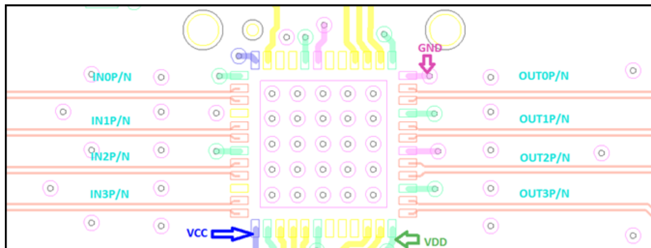
Figure 16. TBV1440 Layout
