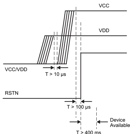
Figure 15. Power-up Sequence
