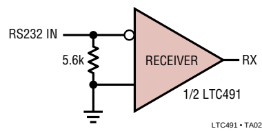
RS232 Receiver
