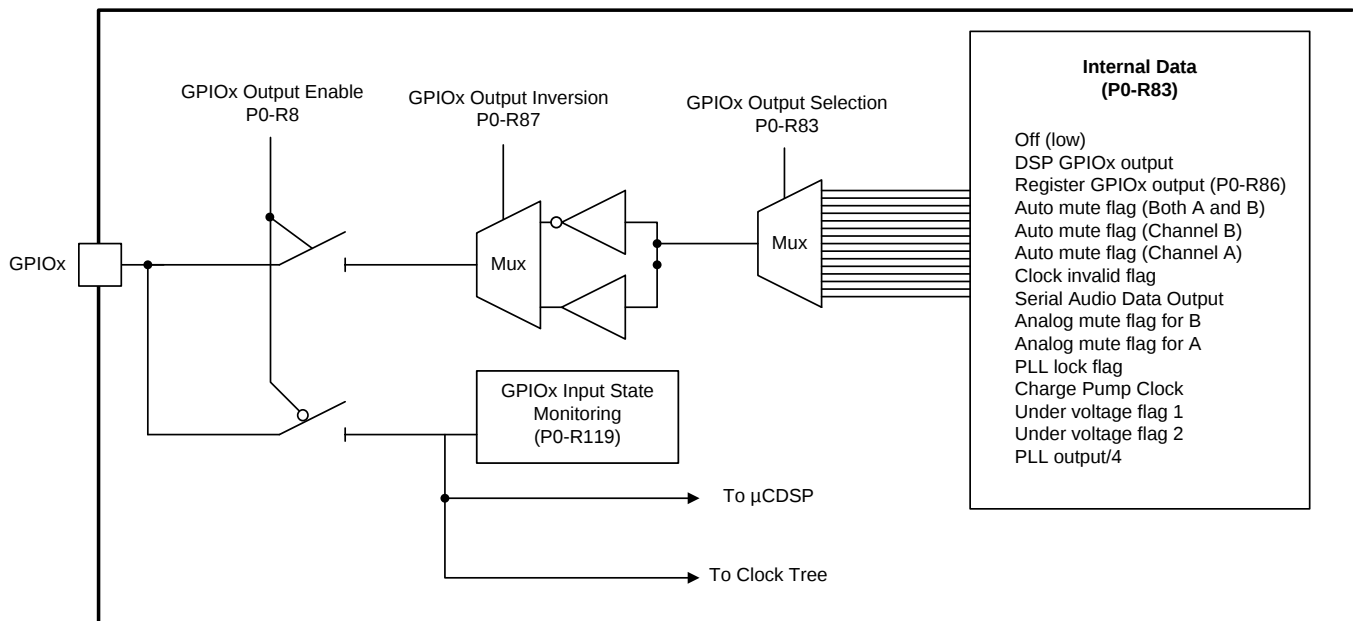
Figure 76. GPIO Port
