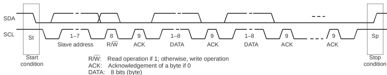
Figure 77. Packet Protocol
