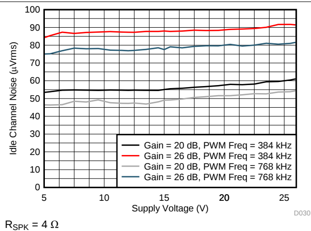
Figure 56. Idle Channel Noise vs PVDD – PBTL
