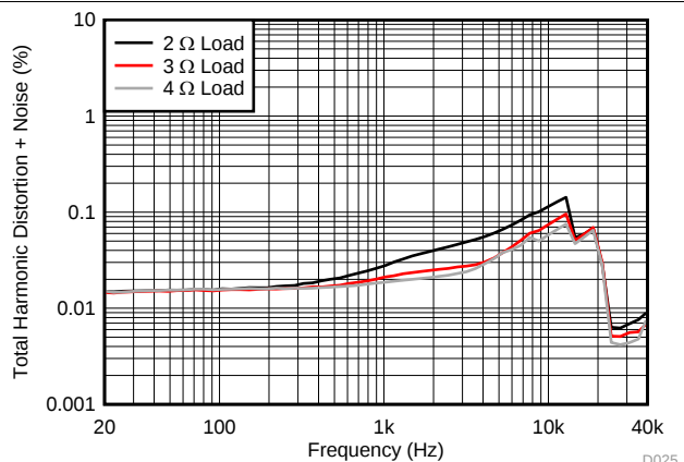
Figure 49. THD+N vs Frequency – PBTTL
