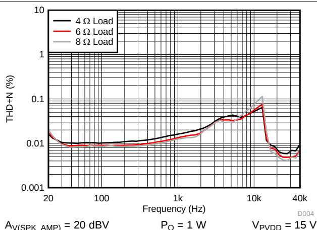
Figure 25. THD+N vs Frequency – BTL
