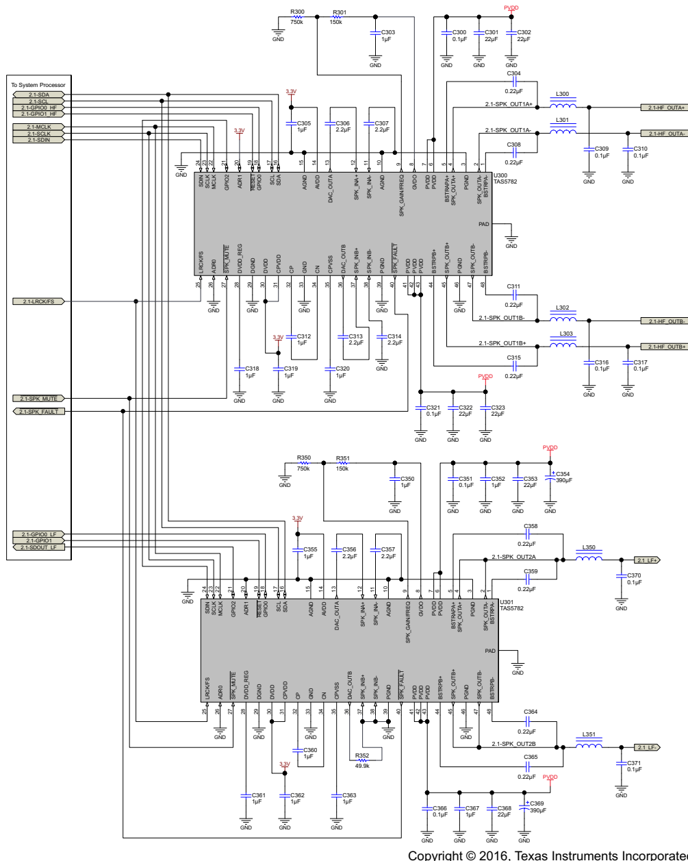
Figure 82. 2.1 (Stereo BTL + External Mono Amplifier) Application Schematic
