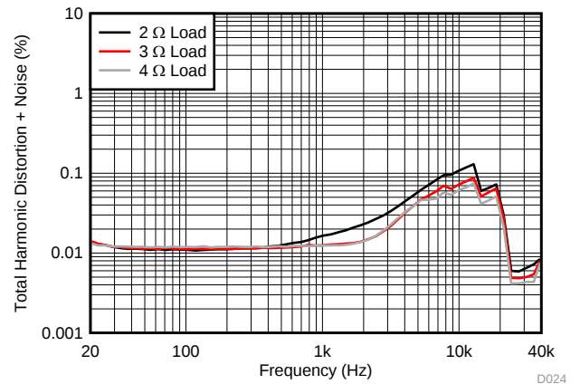
Figure 48. THD+N vs Frequency – PBTTL
