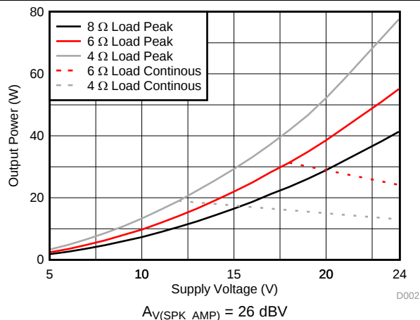
Figure 23. Output Power vs PVDD – BTL
