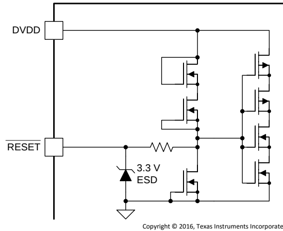
Figure 17. RESET Pin
