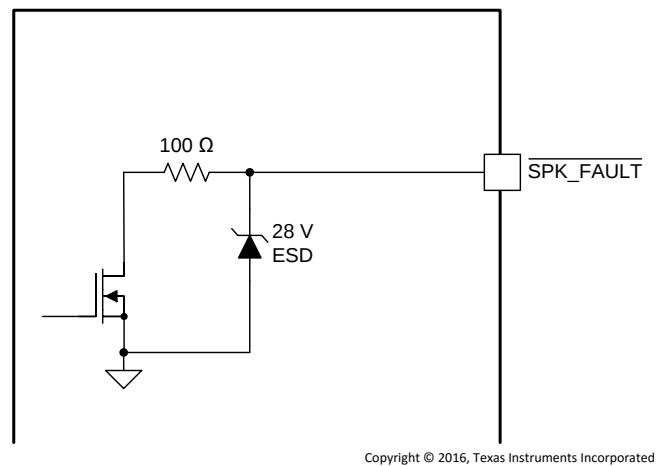
Figure 16. \overline{\text{SPK\_FAULT}} Pin
