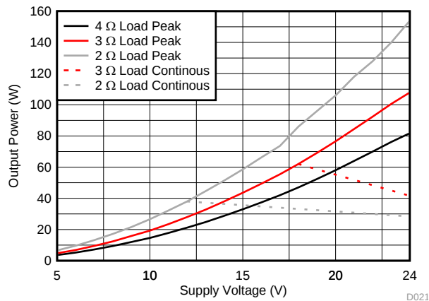
Figure 47. Output Power vs PVDD – PBTTL
