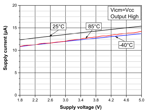
Figure 5. Supply current vs supply voltage, V_{icm} = V_{CC} , output high
