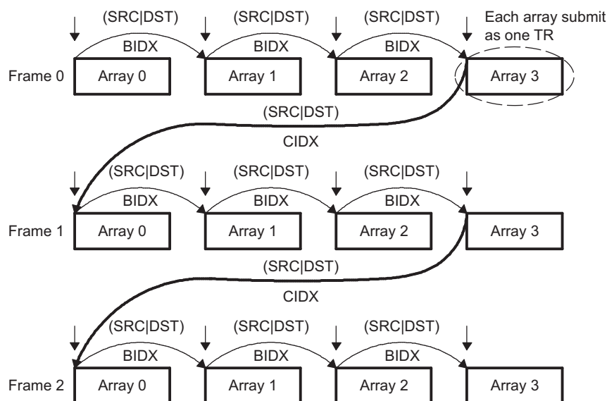
Figure 17-5. A-Synchronized Transfers (ACNT = n, BCNT = 4, CCNT = 3)
