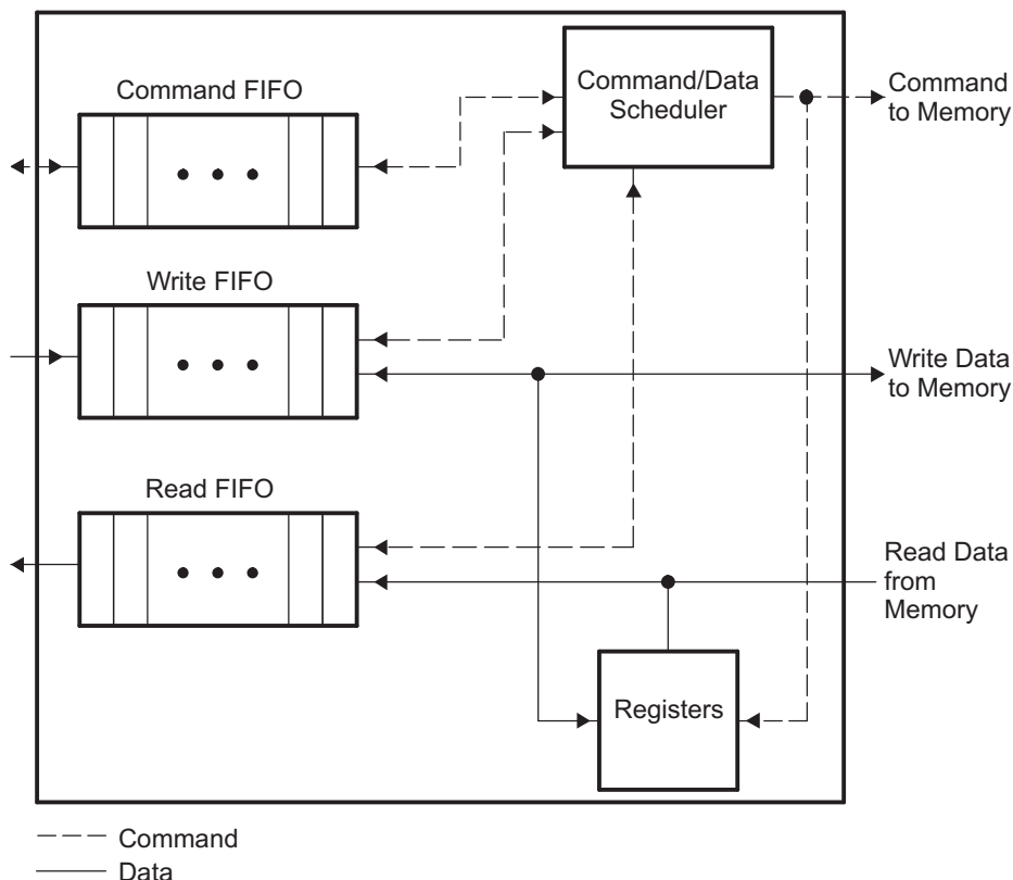
Figure 14-15. DDR2/mDDR Memory Controller FIFO Block Diagram
