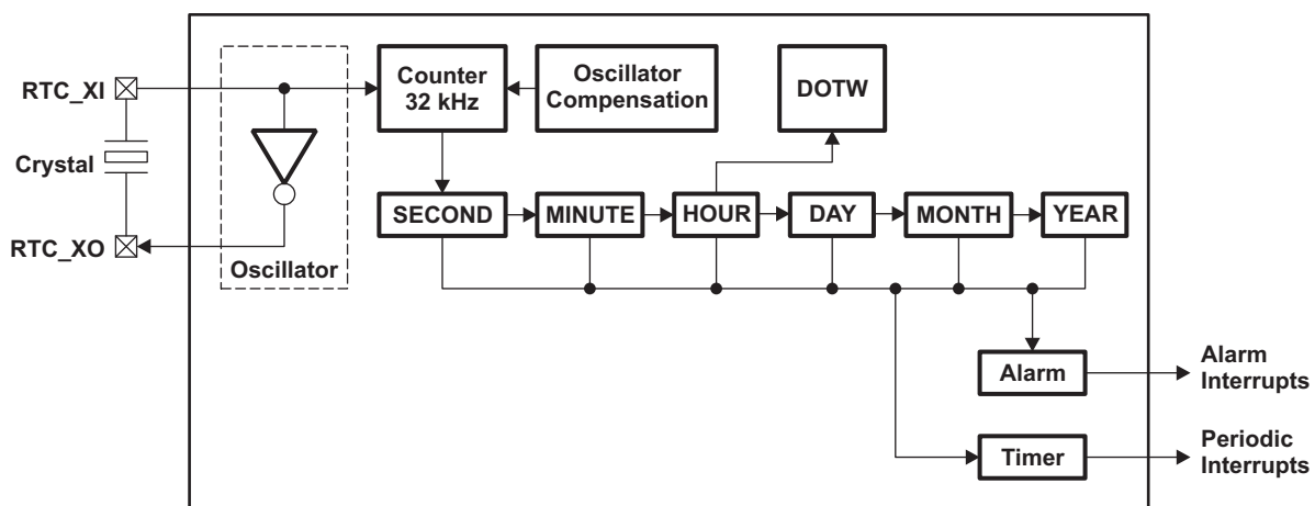
Figure 27-1. Real-Time Clock Block Diagram
