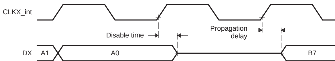
Figure 25-3. Transmit Data Clocking
