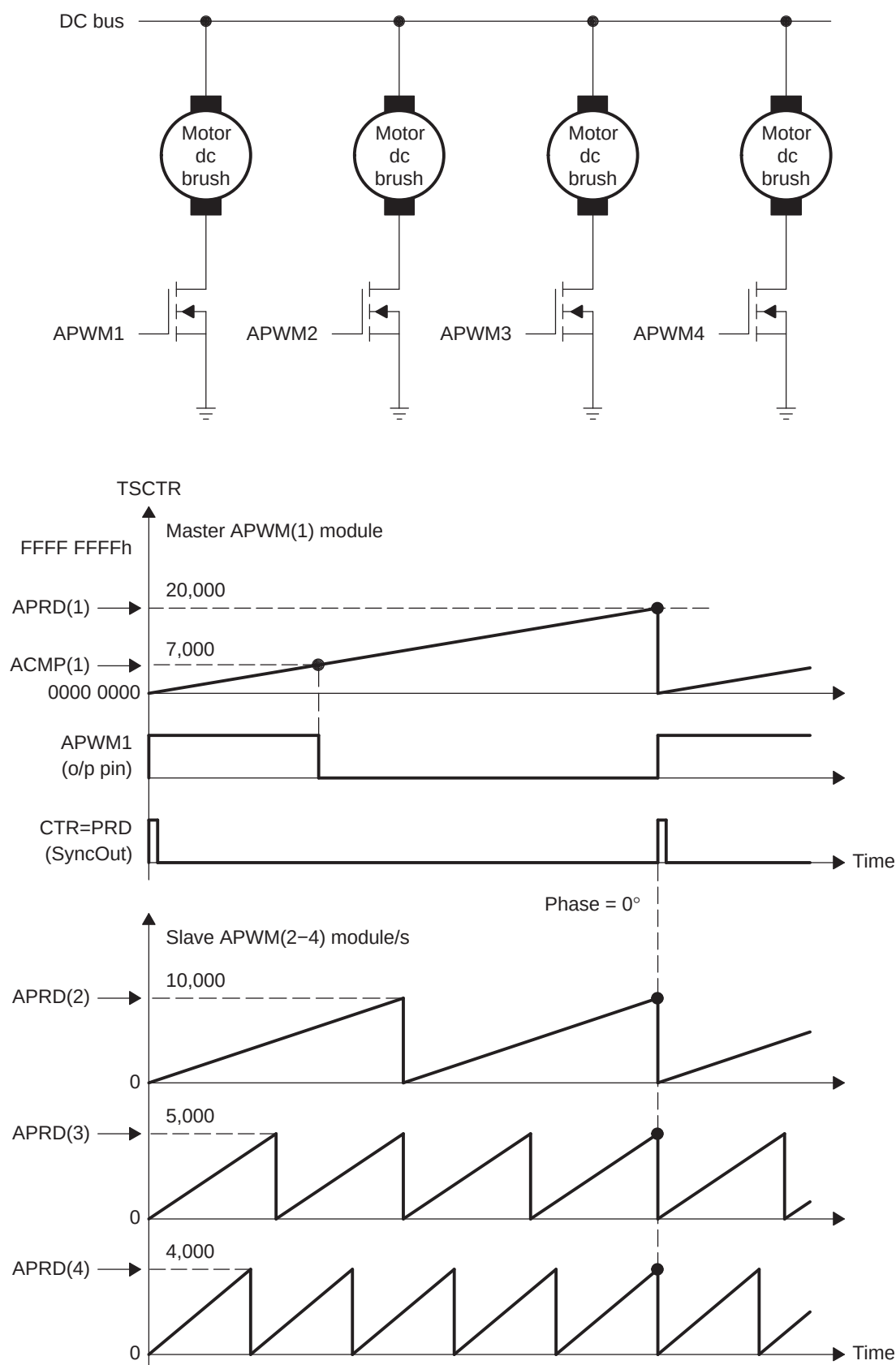
Figure 15-15. Multichannel PWM Example Using 4 eCAP Modules
