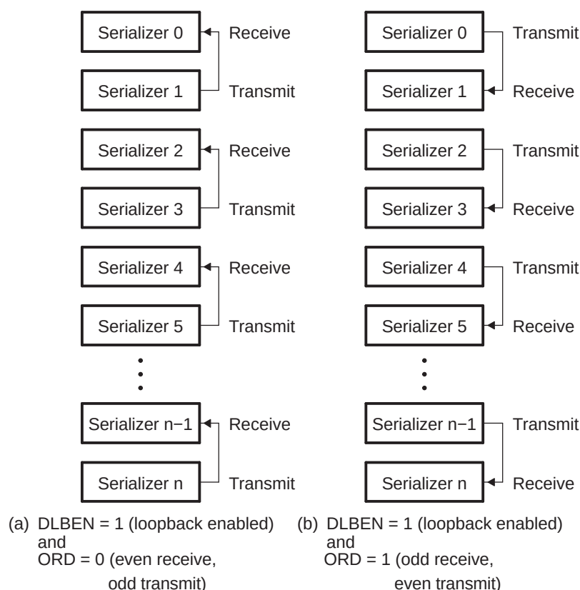
Figure 24-34. Serializers in Loopback Mode
