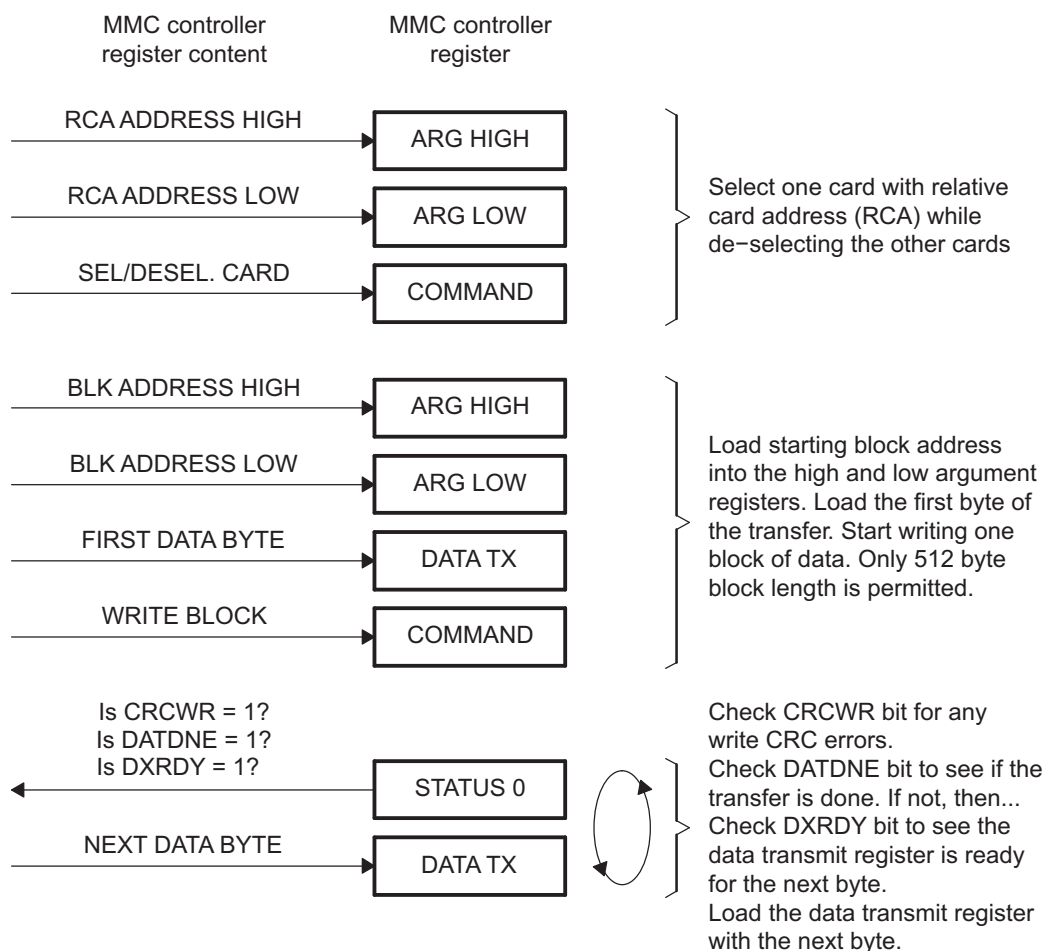
Figure 26-13. MMC/SD Mode Single-Block Write Operation
