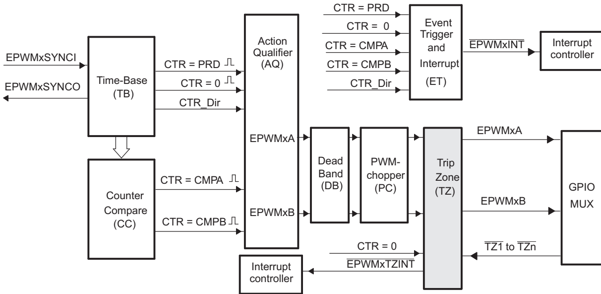
Figure 16-36. Trip-Zone Submodule
