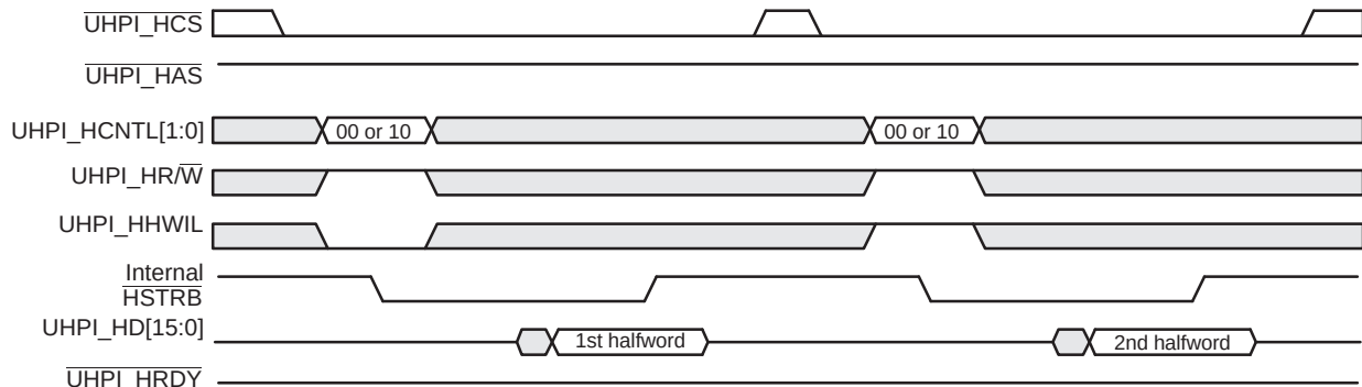
Figure 21-7. \overline{\text{UHPI\_HRDY}} Behavior During an HPIC or HPIA Read Cycle in the Multiplexed Mode
