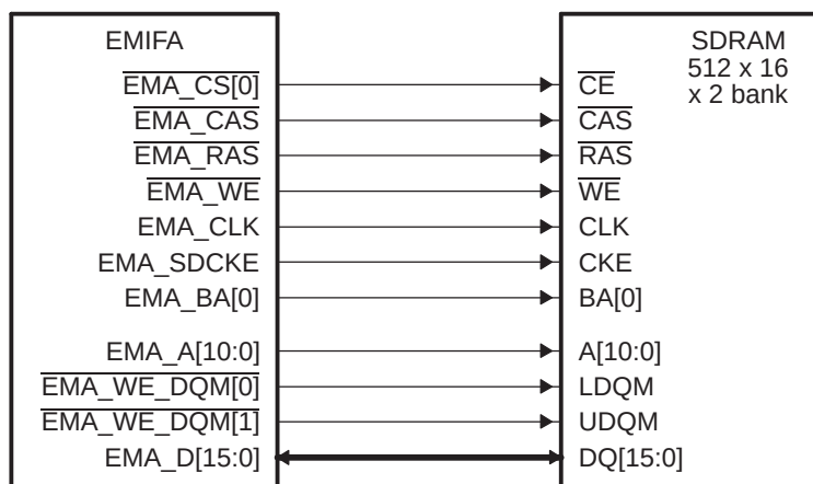
Figure 19-4. EMIFA to 512K × 16 × 2 bank SDRAM Interface
