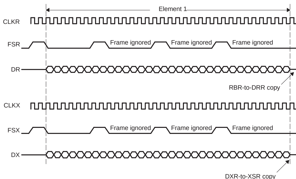
Figure 25-22. Data Packing at Maximum Frame Frequency With (R/X)FIG = 1
