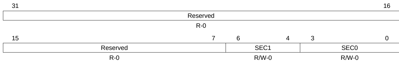
Figure 27-4. Second Register (SECOND)
