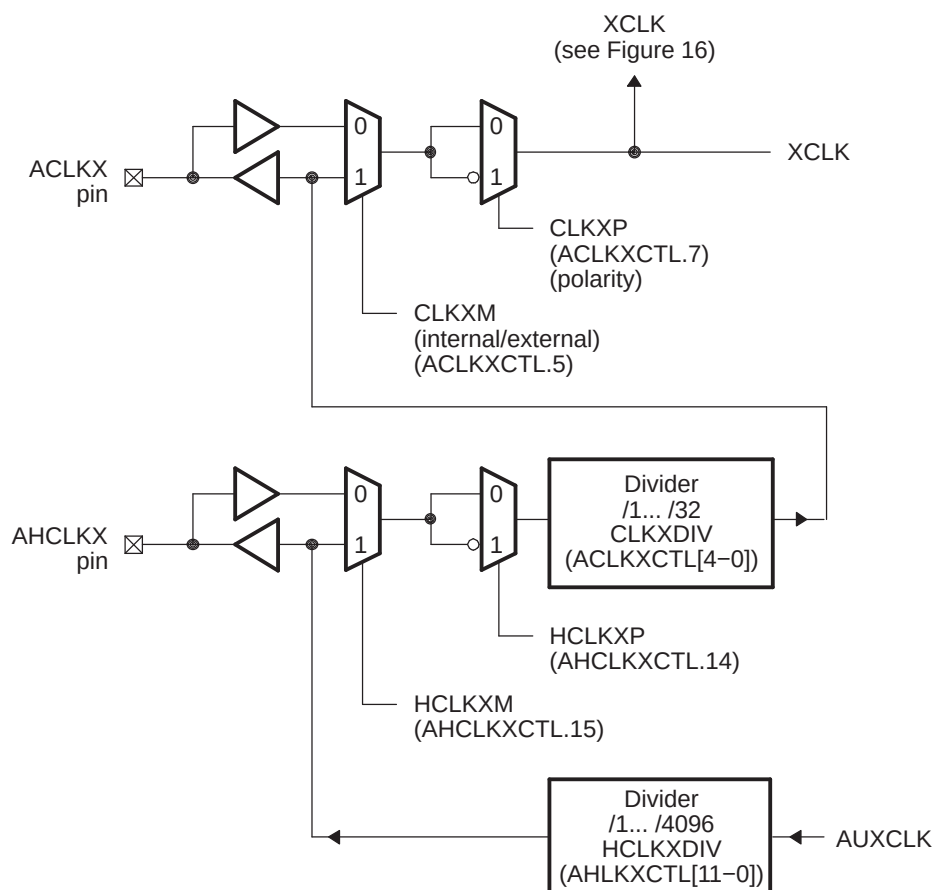
Figure 24-15. Transmit Clock Generator Block Diagram
