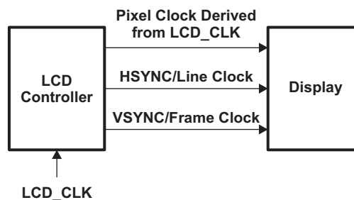
Figure 23-2. Input and Output Clocks
