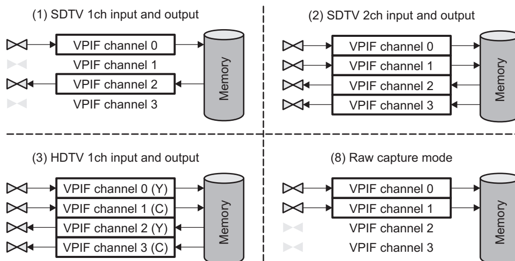
Figure 35-1. Input and Output Channels of VPIF
