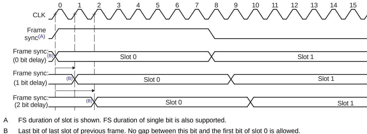
Figure 24-7. TDM Format Bit Delays from Frame Sync
