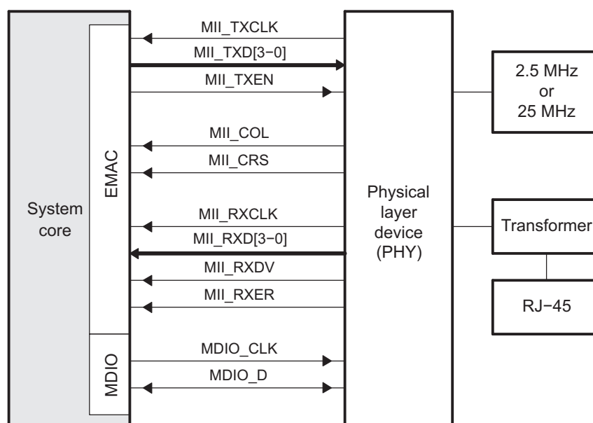
Figure 18-2. Ethernet Configuration—MII Connections
