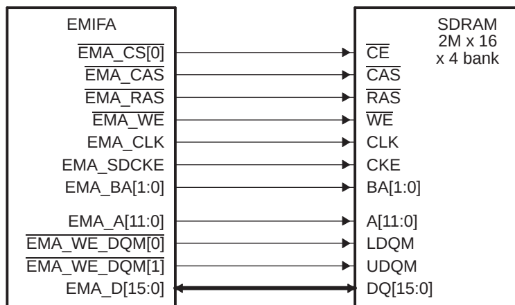
Figure 19-3. EMIFA to 2M × 16 × 4 bank SDRAM Interface
