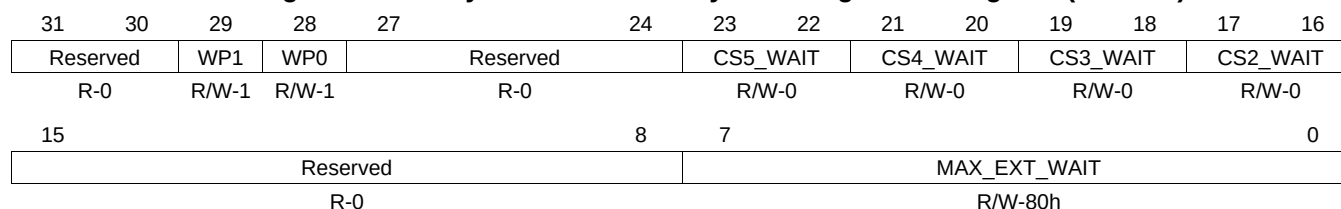
Figure 19-32. Asynchronous Wait Cycle Configuration Register (AWCCR)
