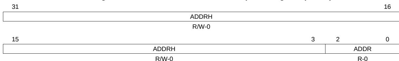
Figure 32-28. uPP DMA Channel I Descriptor 0 Register (UPID0)
