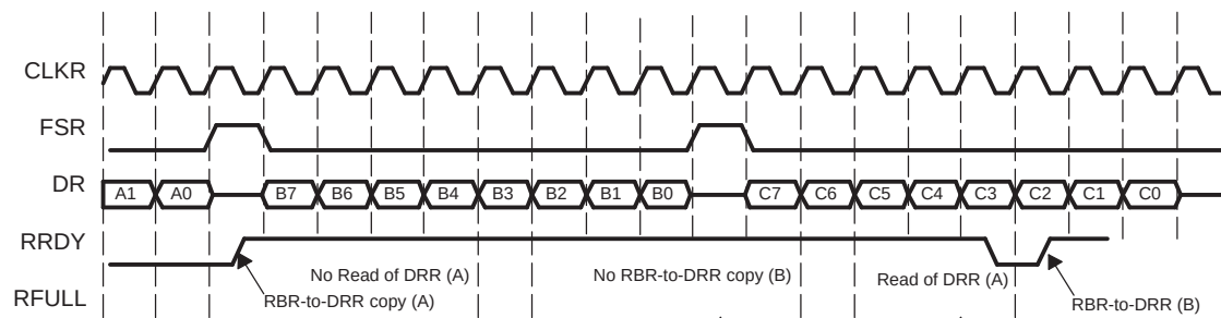
Figure 25-24. Serial Port Receive Overrun Avoided
