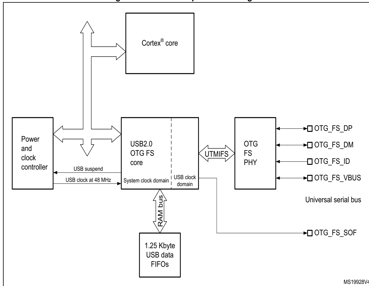
Figure 395. OTG full-speed block diagram
