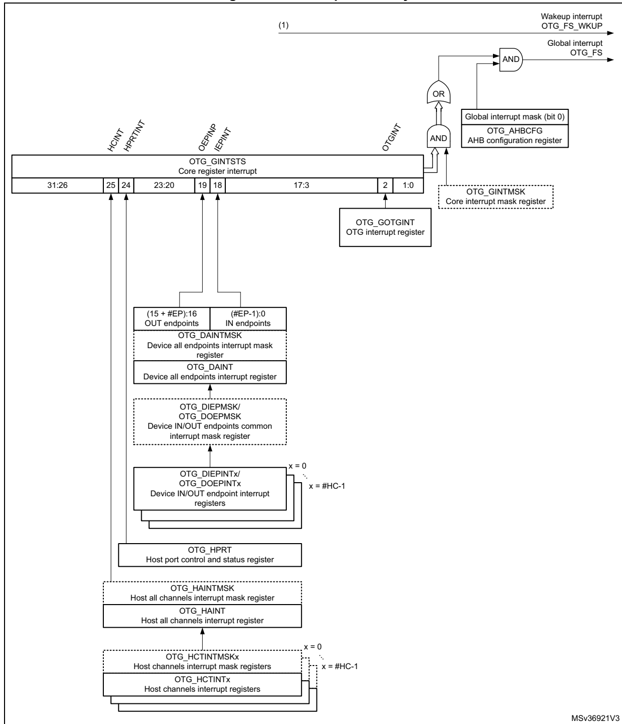
Figure 403. Interrupt hierarchy
