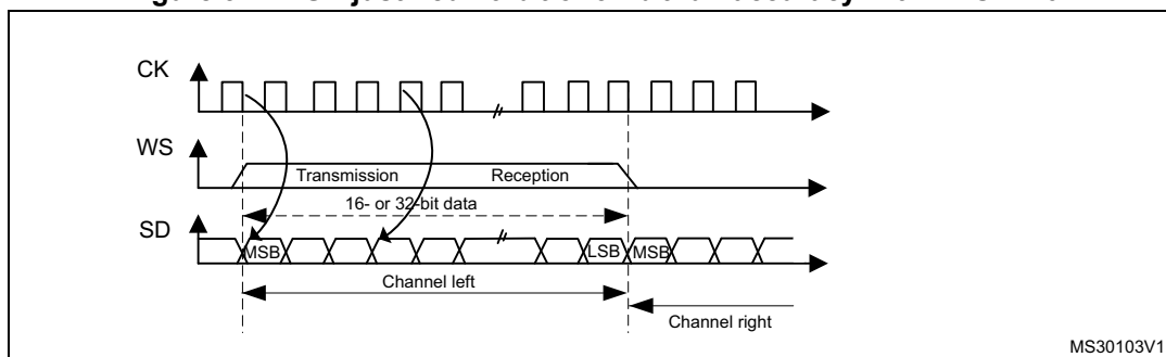
Figure 341. LSB justified 16-bit or 32-bit full-accuracy with CPOL = 0
