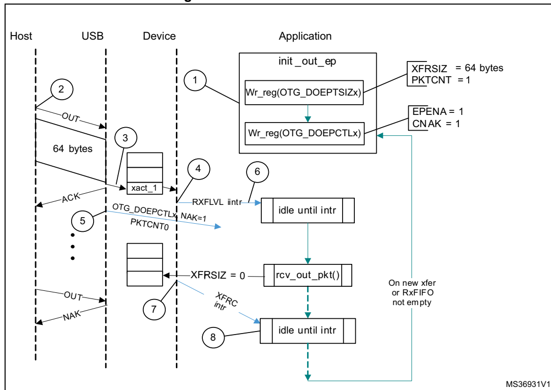
Figure 414. Bulk OUT transaction
