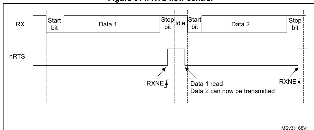
Figure 314. RTS flow control
