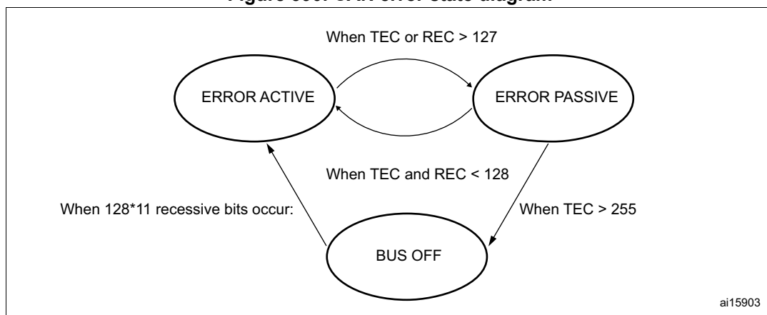
Figure 390. CAN error state diagram
