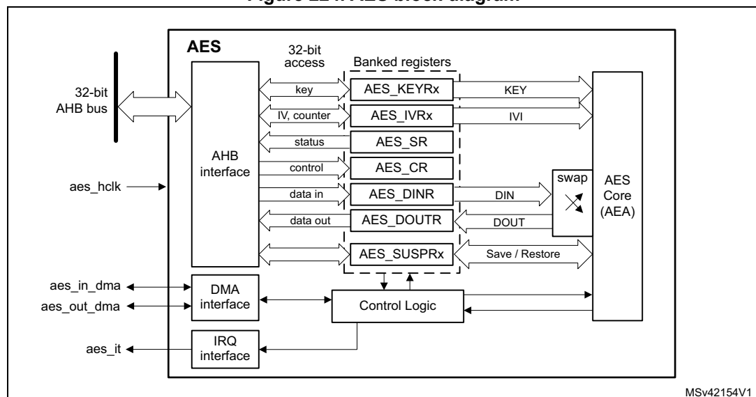
Figure 224. AES block diagram
