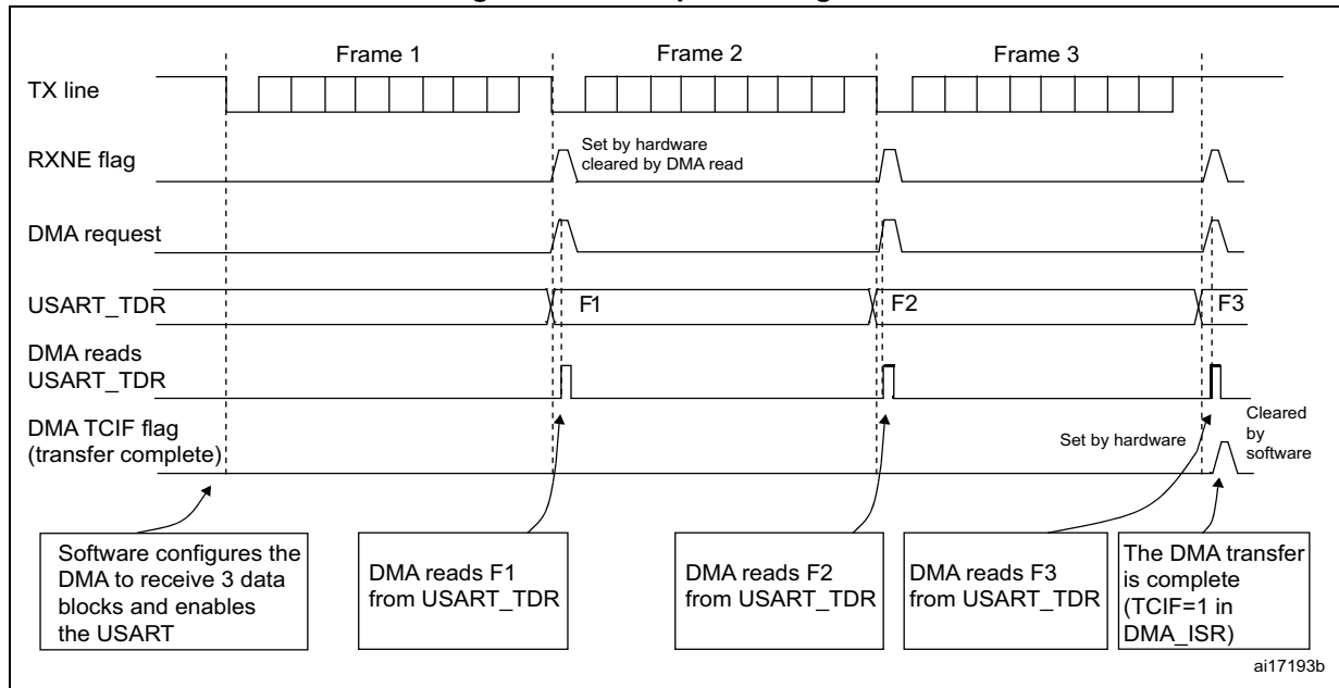
Figure 312. Reception using DMA
