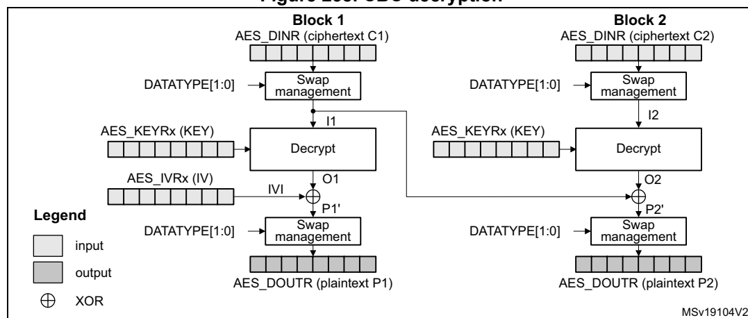
Figure 238. CBC decryption
