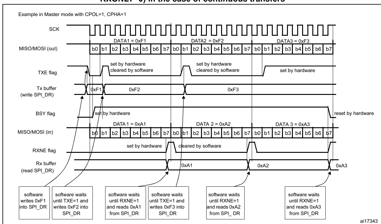
Figure 325. TXE/RXNE/BSY behavior in master / full-duplex mode (BIDIMODE=0, RXONLY=0) in the case of continuous transfers
