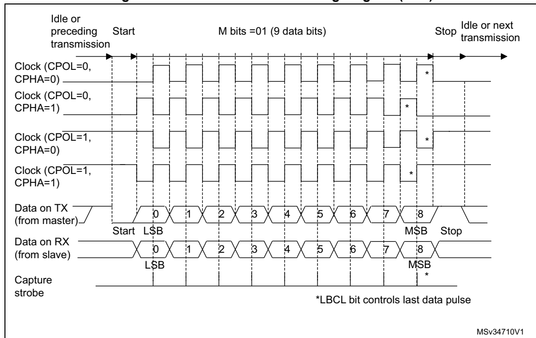
Figure 305. USART data clock timing diagram (M=1)
