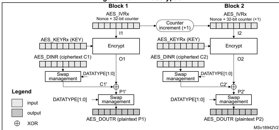
Figure 243. CTR decryption
