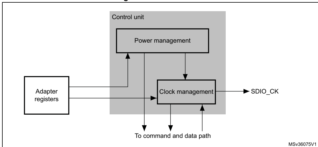
Figure 371. Control unit
