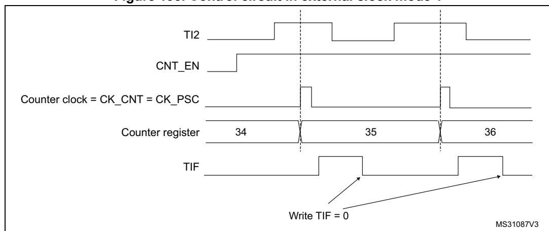
Figure 193. Control circuit in external clock mode 1
