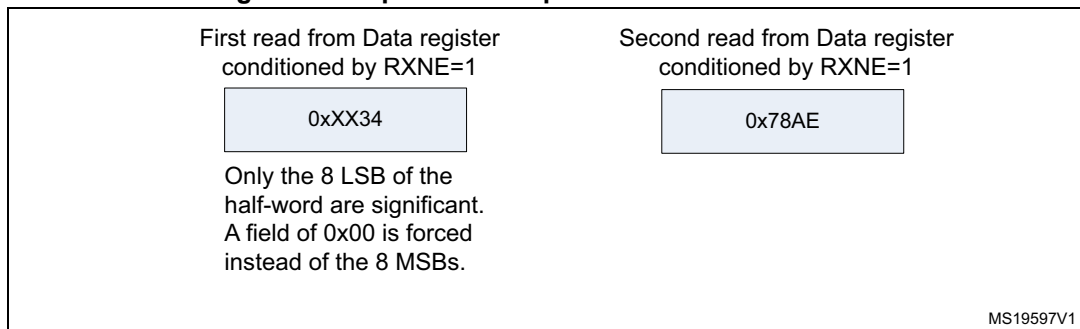
Figure 344. Operations required to receive 0x3478AE
