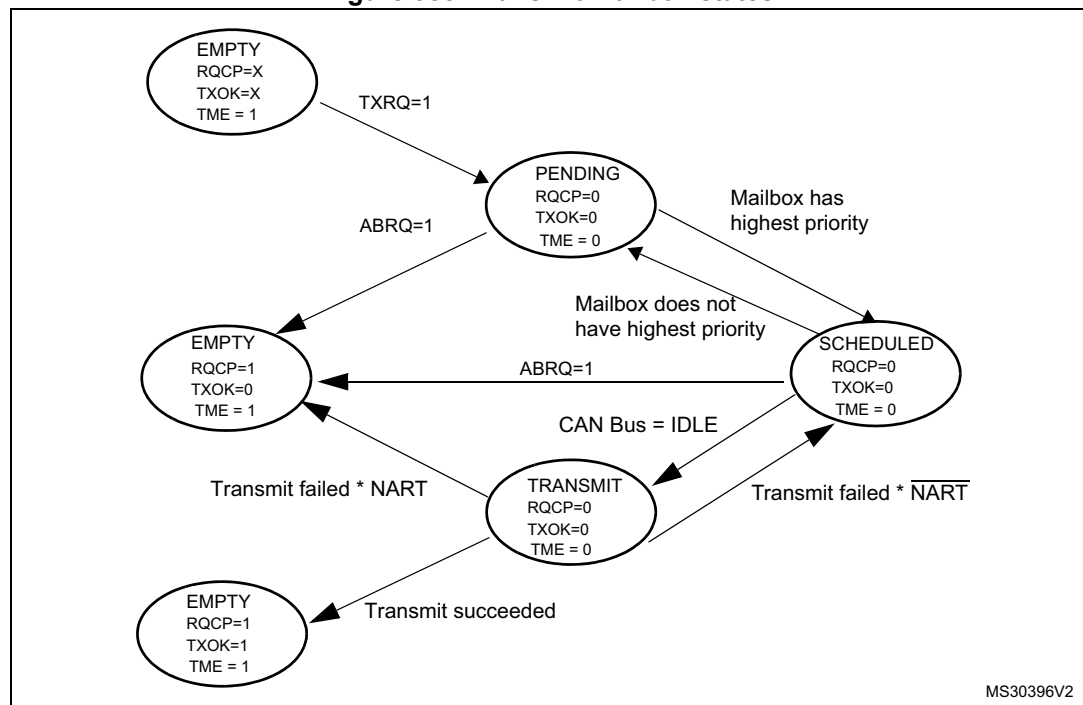
Figure 385. Transmit mailbox states
