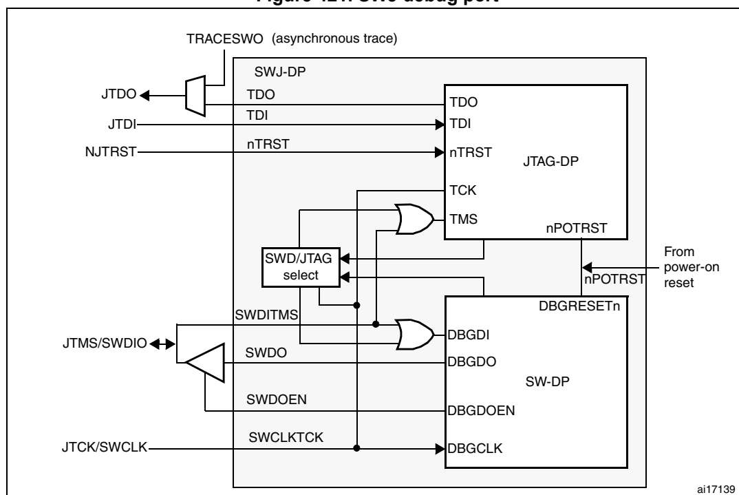
Figure 421. SWJ debug port
