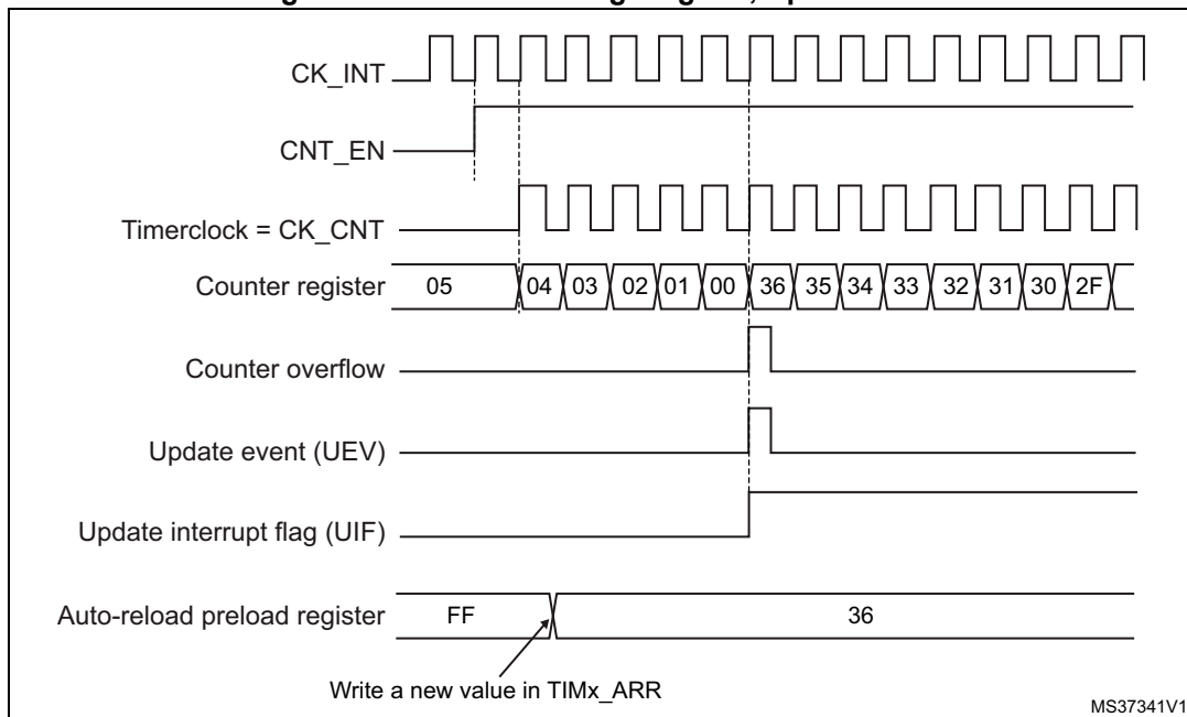
Figure 148. Counter timing diagram, Update event
