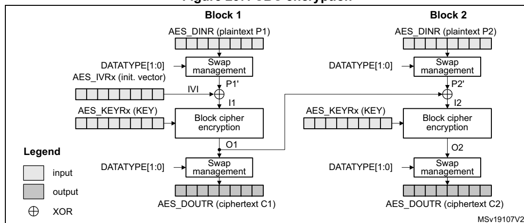
Figure 237. CBC encryption
