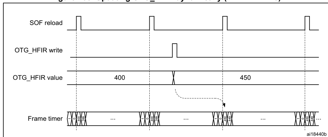
Figure 400. Updating OTG_HFIR dynamically (RLDCTRL = 0)
