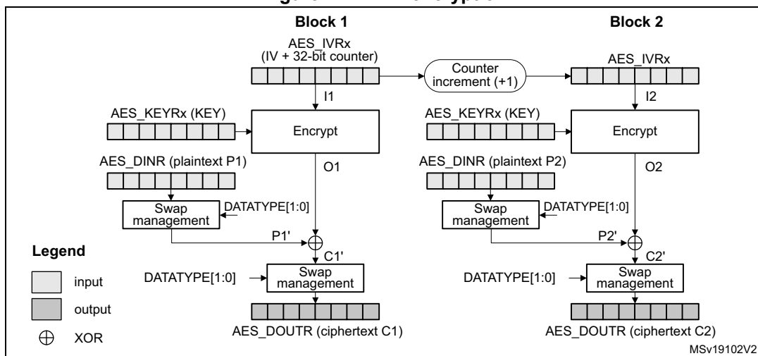
Figure 242. CTR encryption
