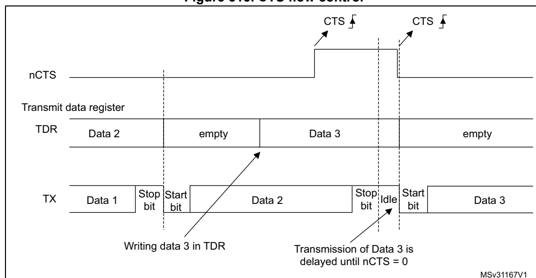
Figure 315. CTS flow control
