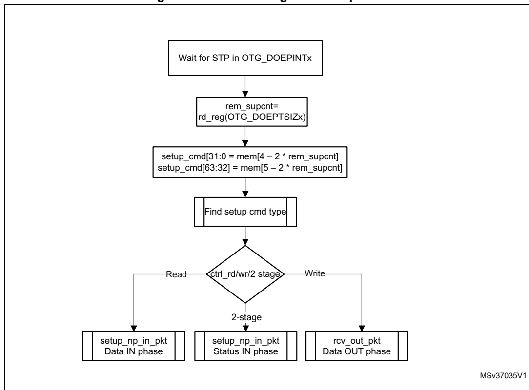
Figure 413. Processing a SETUP packet
