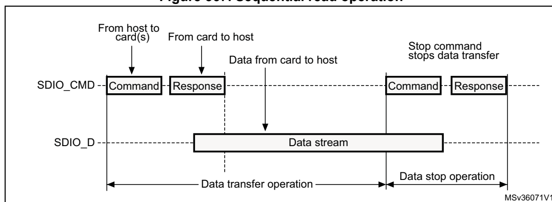
Figure 367. Sequential read operation
