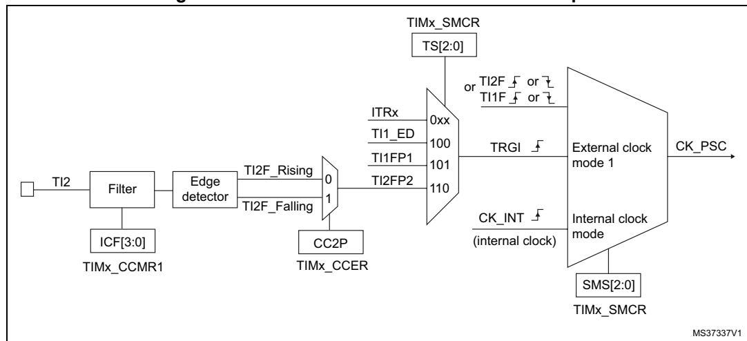
Figure 192. TI2 external clock connection example
