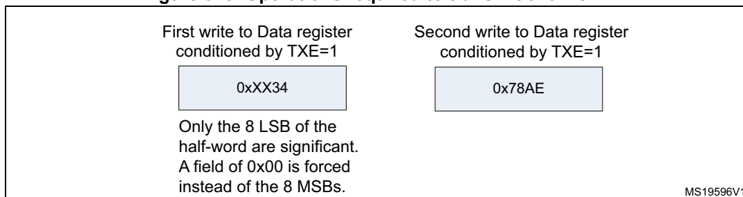
Figure 343. Operations required to transmit 0x3478AE
