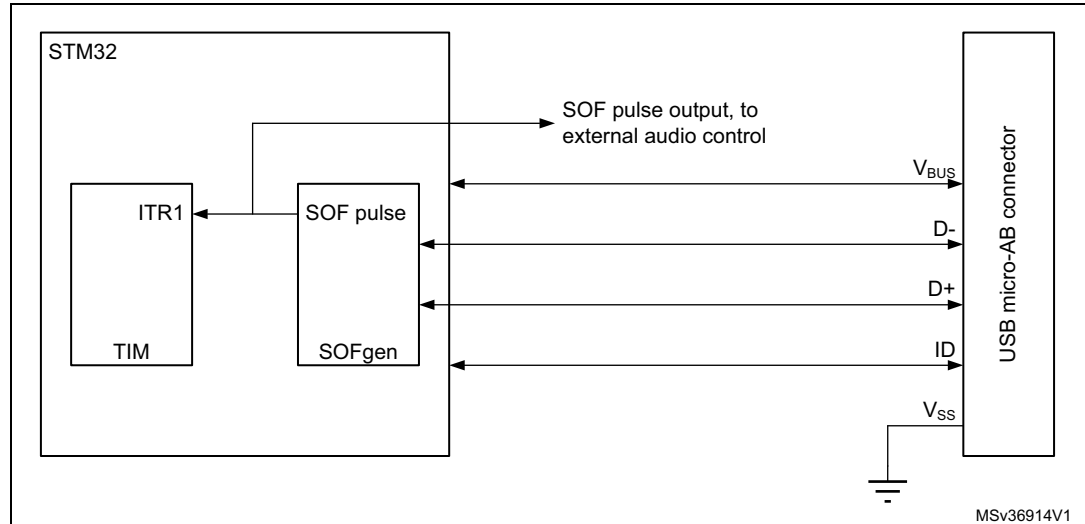
Figure 399. SOF connectivity (SOF trigger output to TIM and ITR1 connection)
