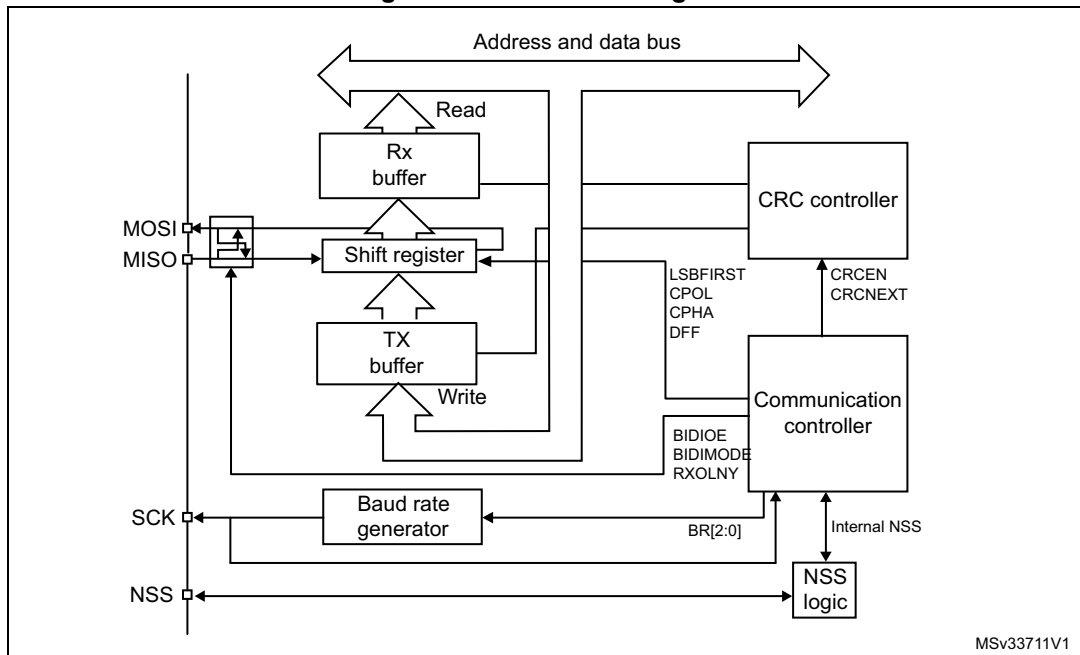
Figure 317. SPI block diagram
