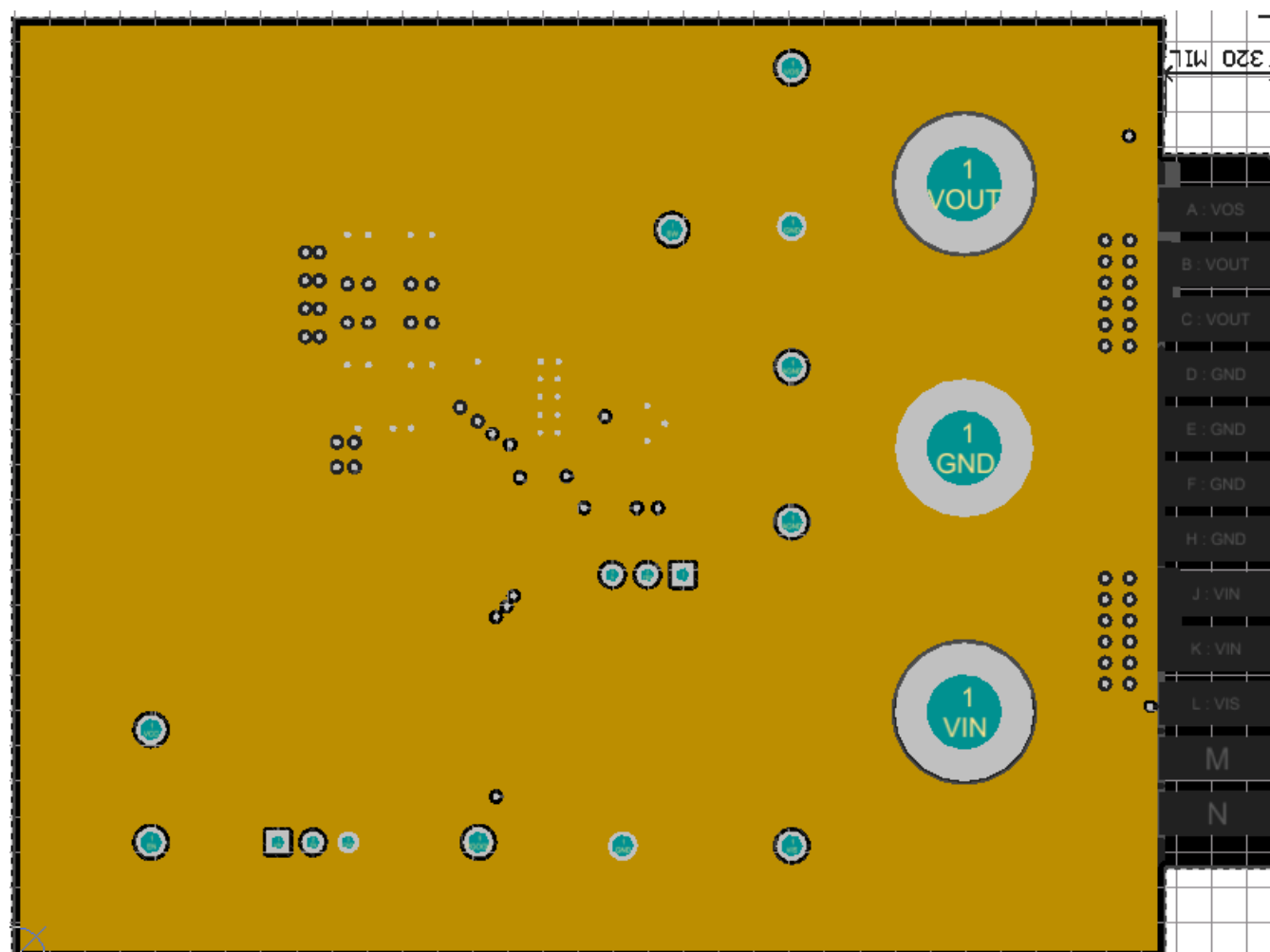
Figure 10. EVM Mid Layer One
