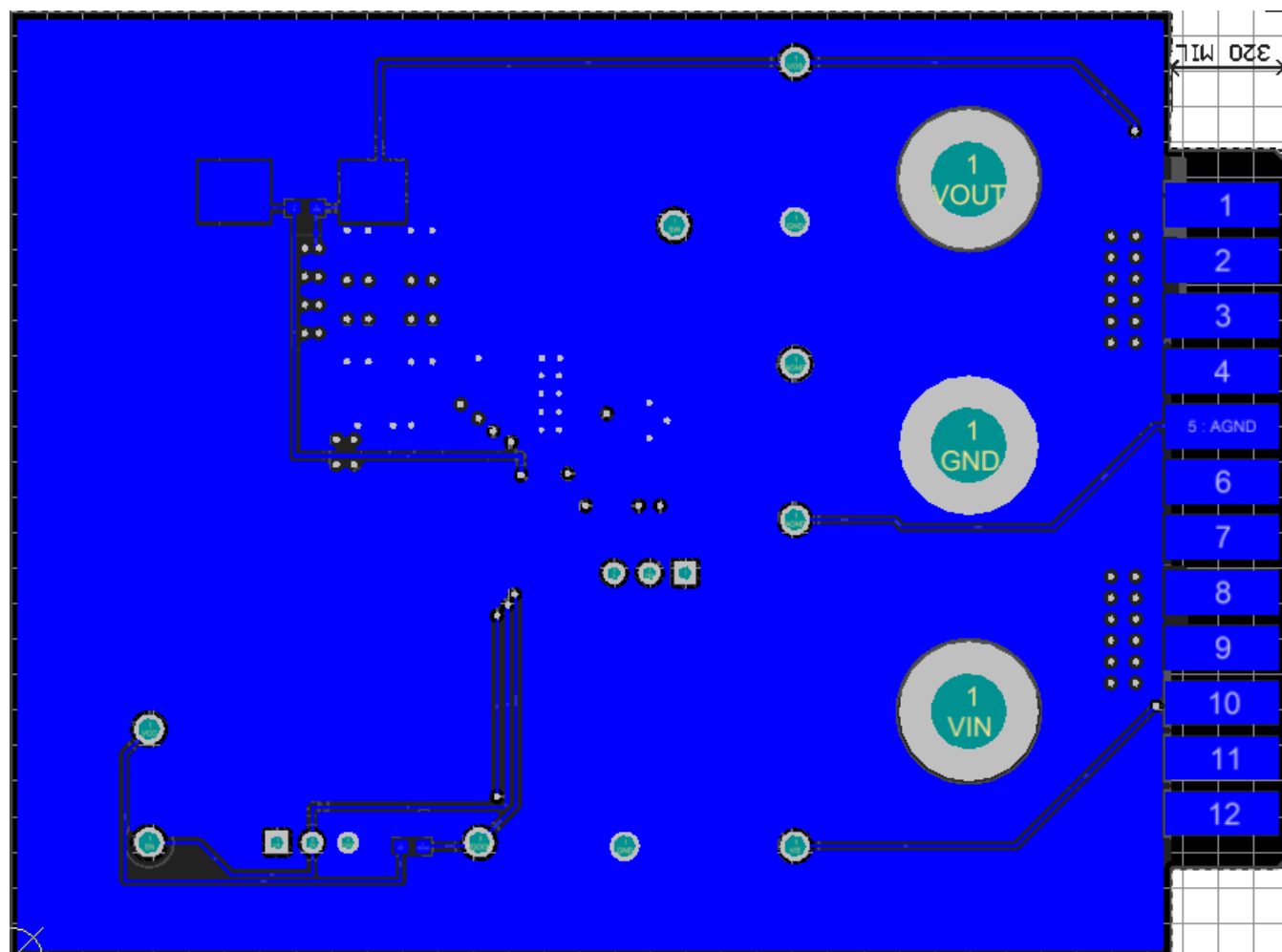
Figure 12. EVM Bottom Copper Layer
