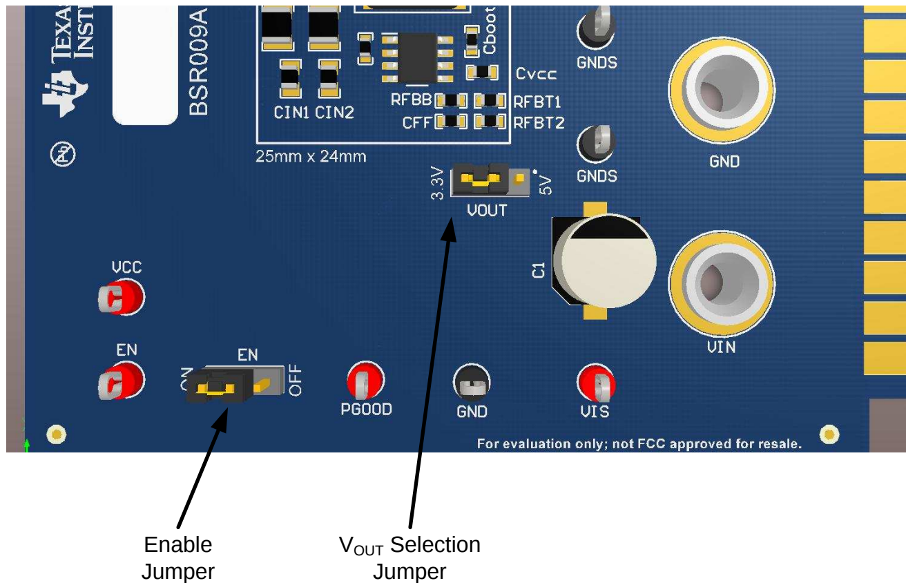
Figure 3. Jumper Locations
