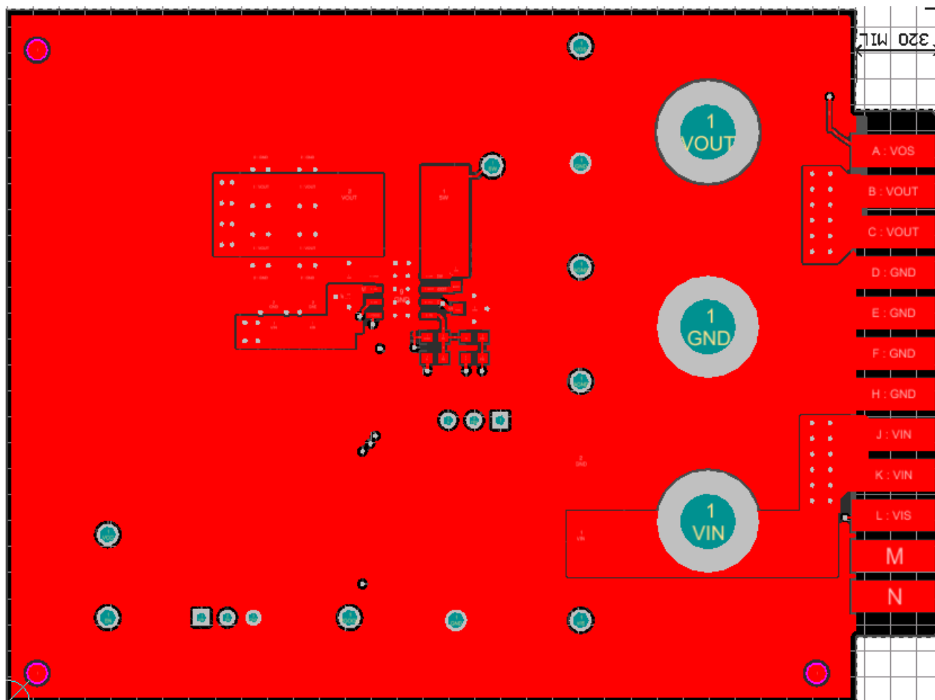
Figure 9. EVM Top Copper Layer
