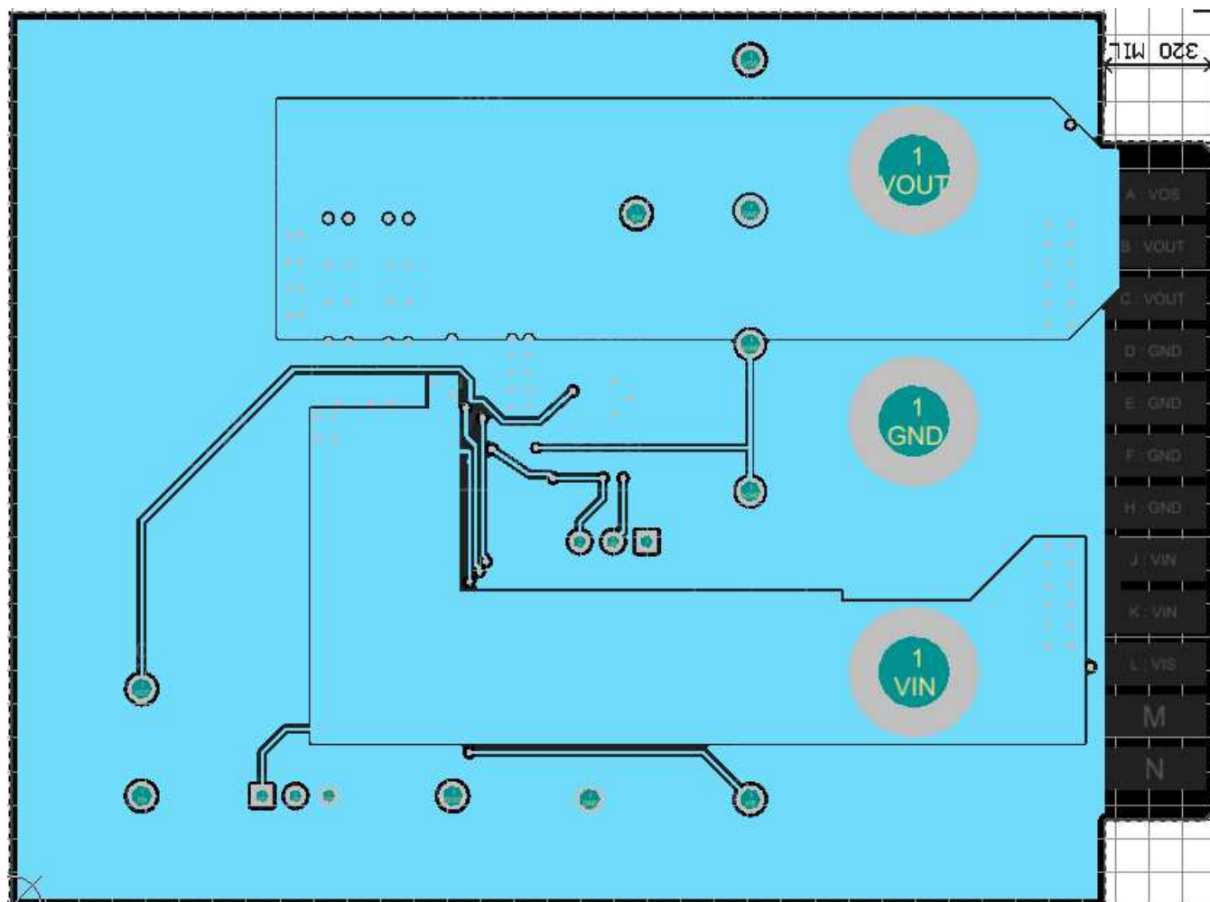
Figure 11. EVM Mid Layer Two
