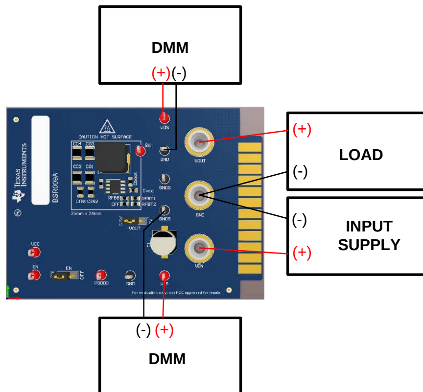
Figure 1. EVM Board Connections
