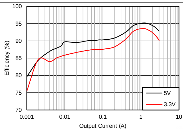
Figure 6. Efficiency: V_{IN} = 12\text{ V} , f_{sw} = 400\text{ kHz}
