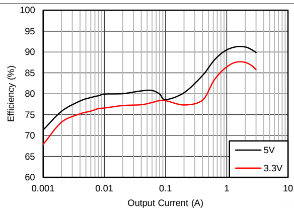
Figure 5. Efficiency: V_{IN} = 12\text{ V} , f_{sw} = 2.1\text{ MHz}
