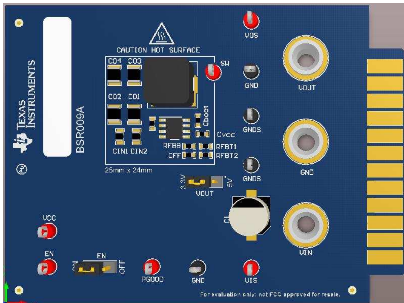
Figure 8. Top View of EVM
