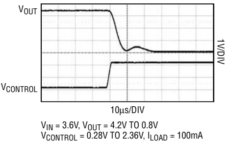
LTC3444 Dynamic Response
