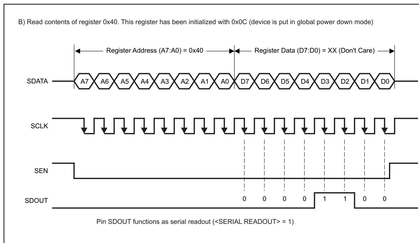
Figure 6. Serial Readout
