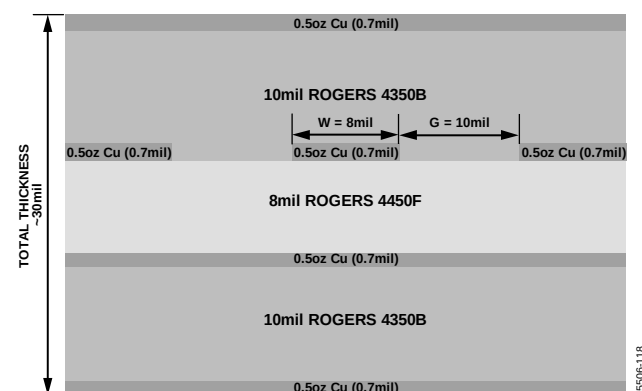
Figure 19. Evaluation Board Cross Sectional View
