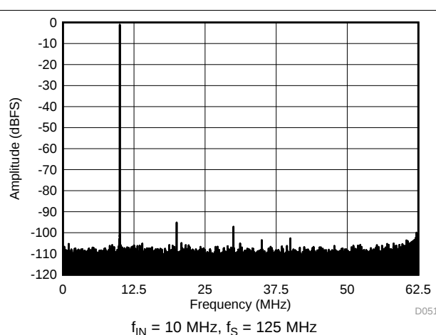
Figure 144. Chopper On
