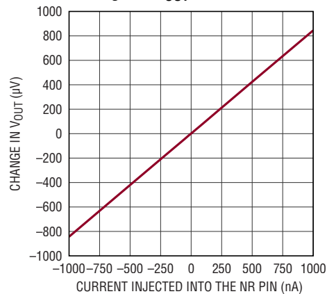
LTC6655LN-2.5 Effect of NR Pin Leakage on V_{\text{OUT}}
