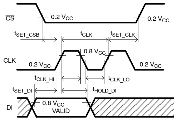
Figure 5. SPI Timing
