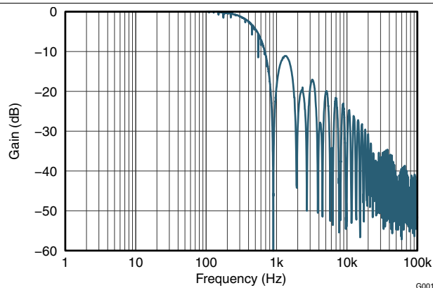
Figure 2. Frequency Response
