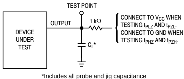
Figure 6. Test Circuit
