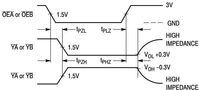
Figure 4. Switching Waveform
