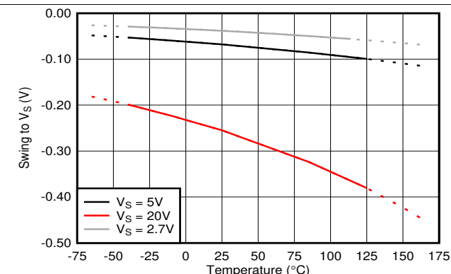
Figure 22. Swing to Supply vs Temperature
