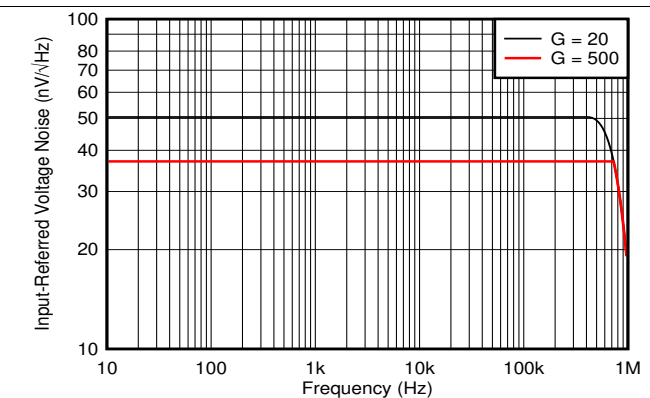
Figure 24. Input Referred Noise vs Frequency
