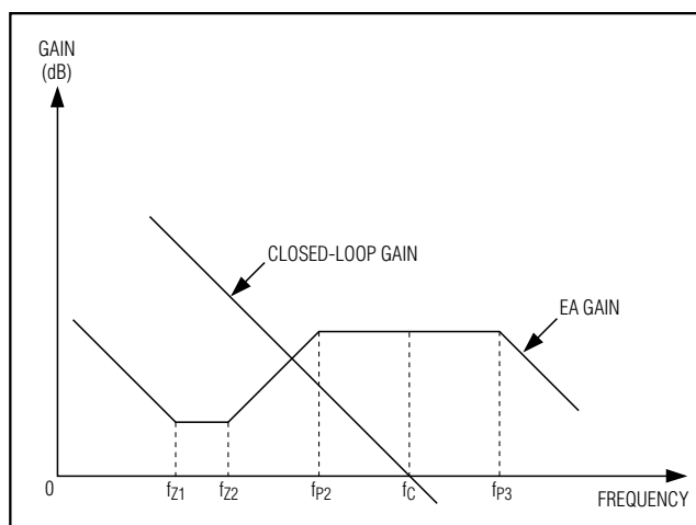
Figure 8. Closed-Loop and Error-Amplifier Gain Plot for Case 2
