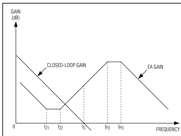
Figure 7. Closed-Loop and Error-Amplifier Gain Plot for Case 1
