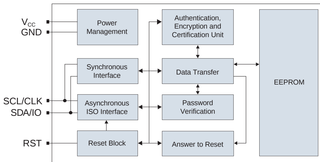
Figure 2-1. Block Diagram
