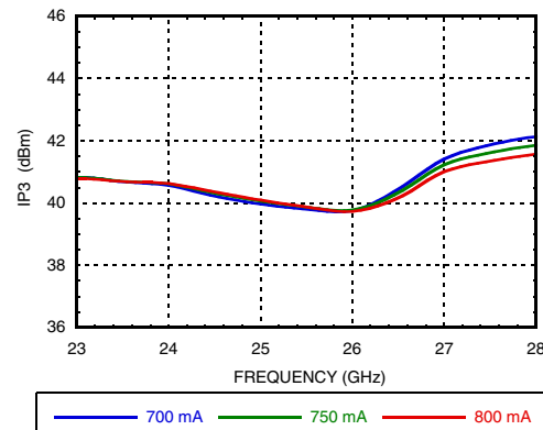
Output IP3 vs. Supply Current, Pout/Tone = +19 dBm
