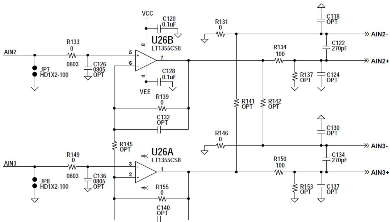
Figure 3. \pm 10.24\text{V} Pseudo-Differential DC Coupled Driver
