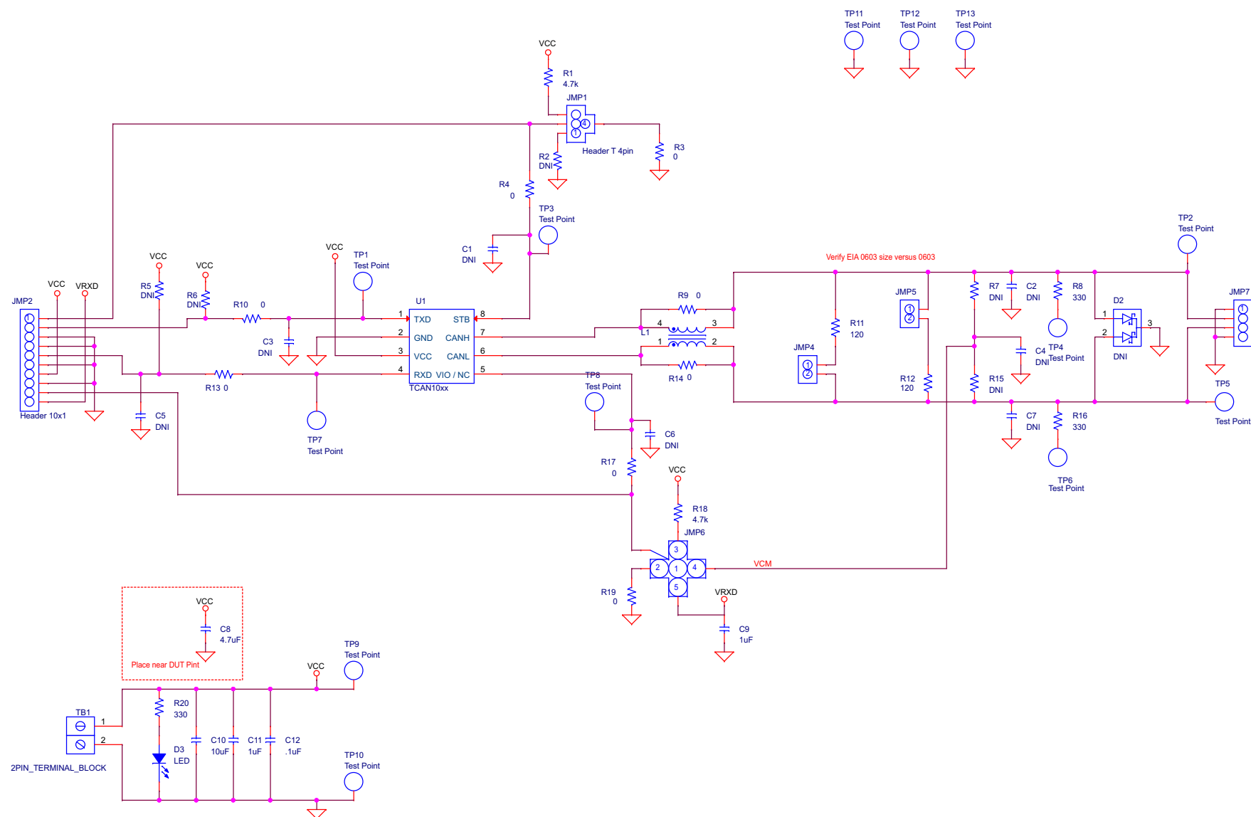
Figure 2. EVM Schematic
