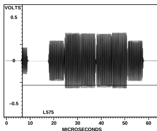
Figure 130. PAL Luma
