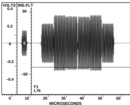
Figure 127. NTSC Luma
