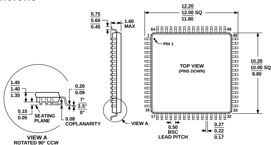
Figure 138. 64-Lead Low Profile Quad Flat Package [LQFP] (ST-64-2)
