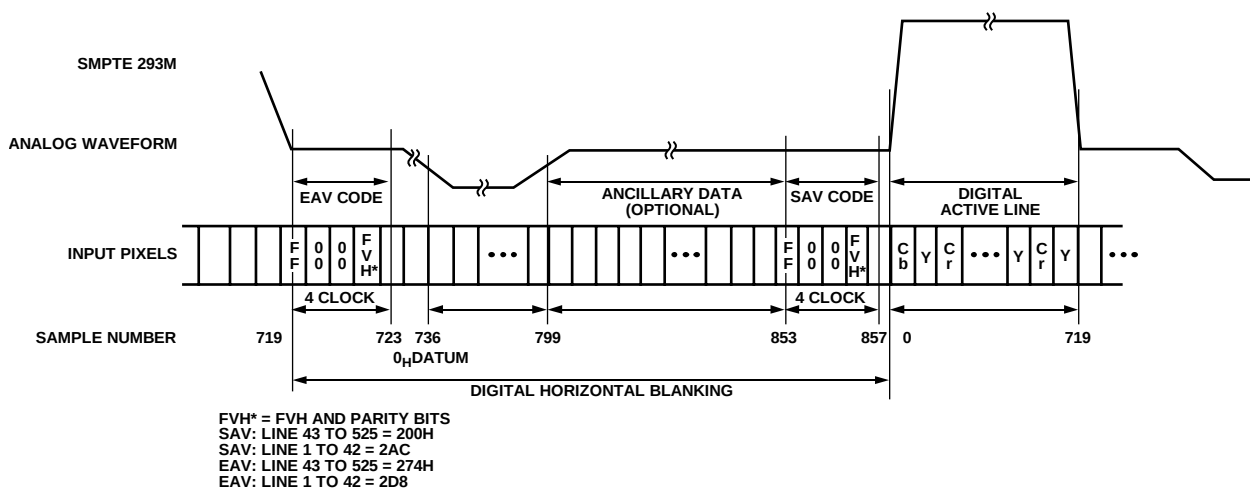
Figure 133. EAV/SAV Input Data Timing Diagram (SMPTE 293M)
