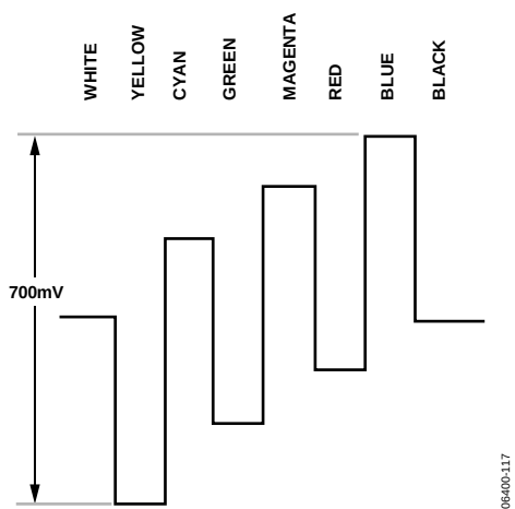
Figure 114. Pb Levels—NTSC
