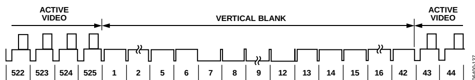
Figure 134. SMPTE 293M (525p)
