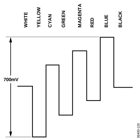
Figure 117. Pb Levels—PAL
