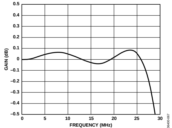
Figure 62. ED/HD Sinc Compensation Filter Enabled
