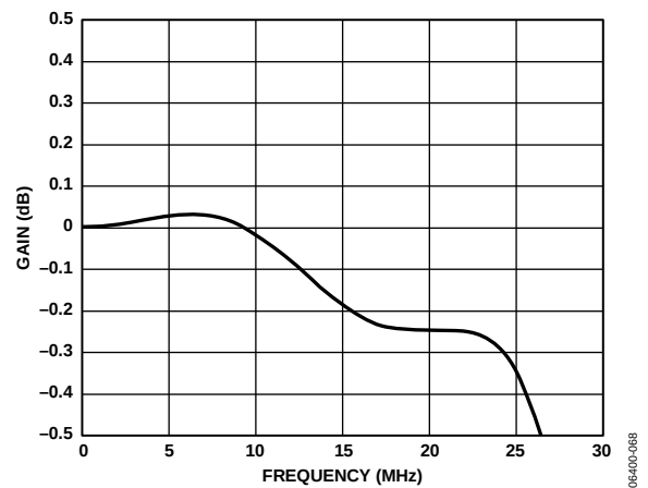
Figure 63. ED/HD Sinc Compensation Filter Disabled
