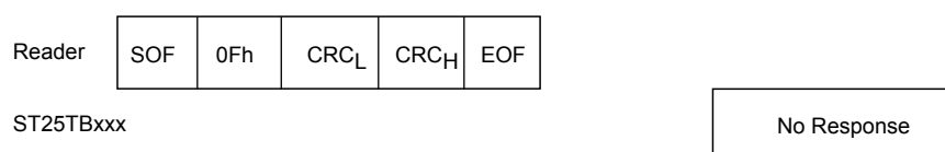
Figure 32. Completion frame exchange between reader and ST25TB512-AC
