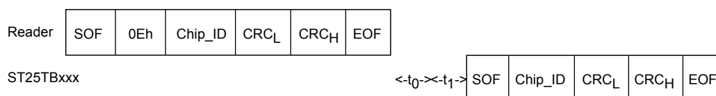
Figure 29. Select frame exchange between reader and ST25TB512-AC
