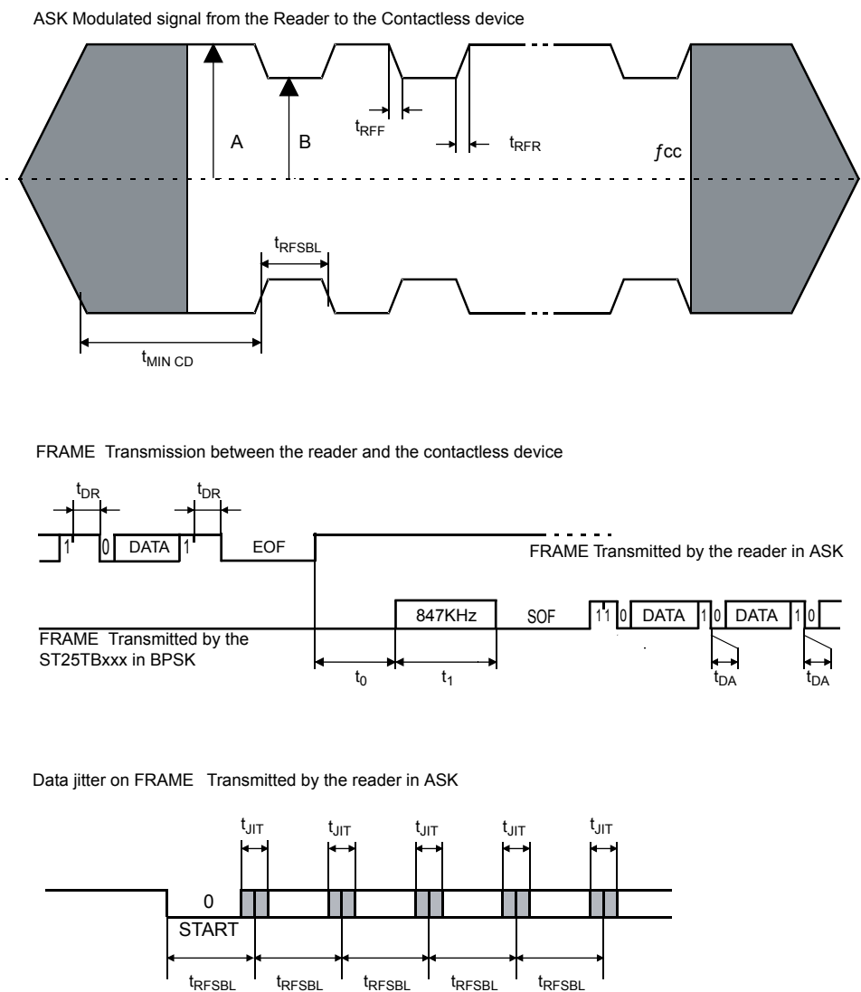
Figure 46. ST25TB512-AC synchronous timing, transmit and receive
