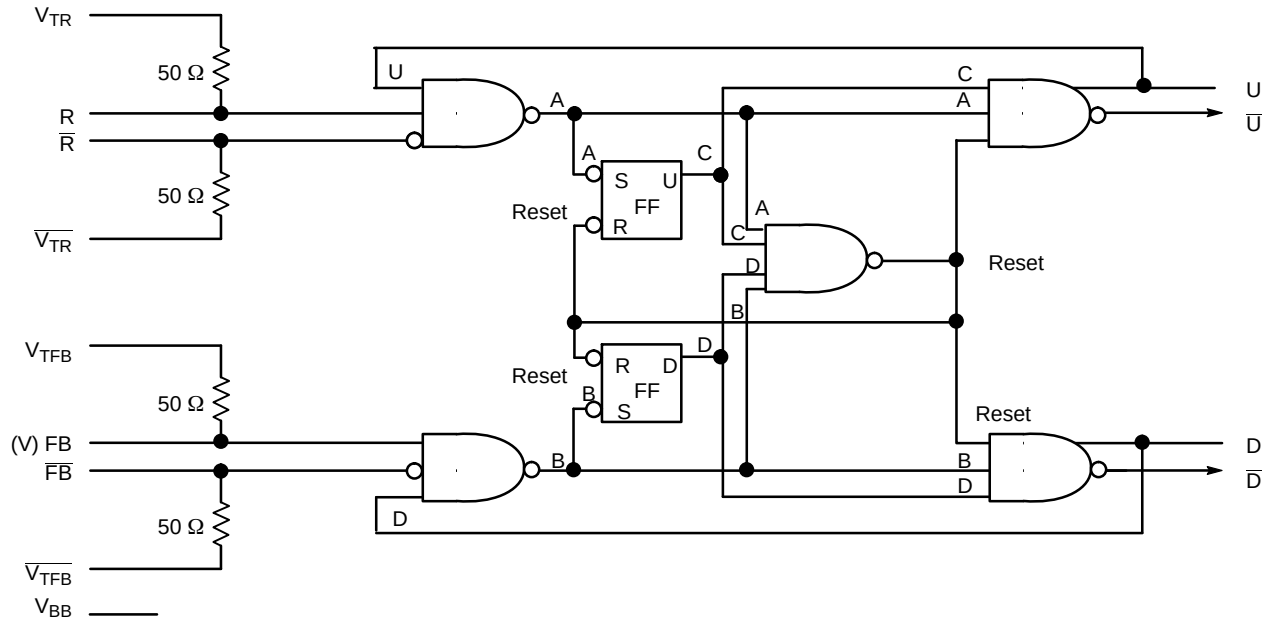
Figure 2. Logic Diagram
