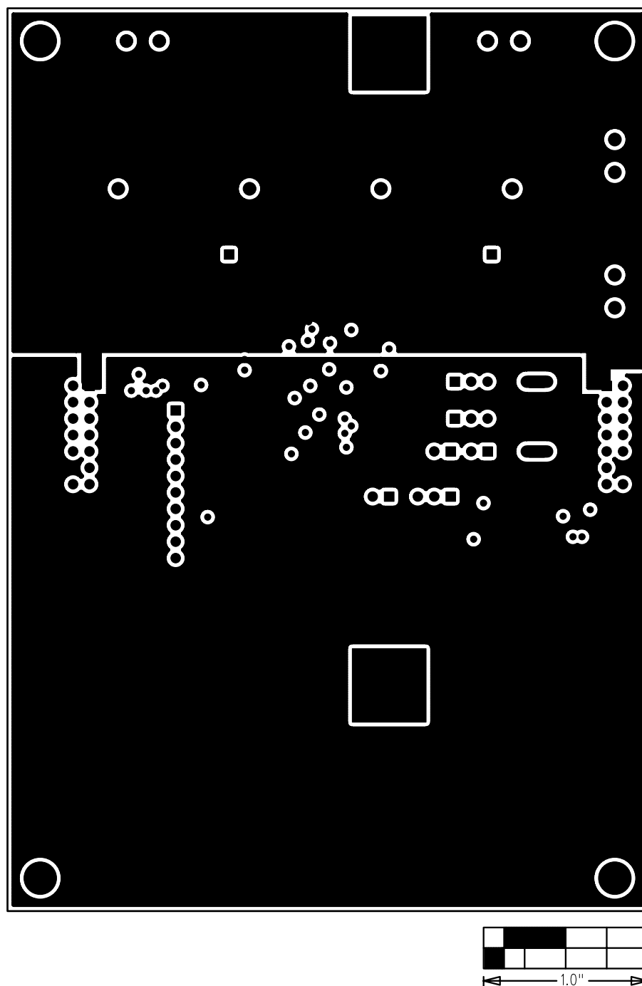
Figure 14. MAX11040K Daughterboard PCB Layout—Layer 2
