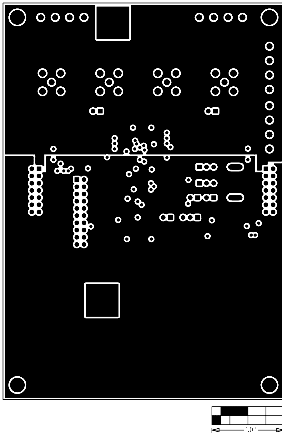
Figure 15. MAX11040K Daughterboard PCB Layout—Layer 3
