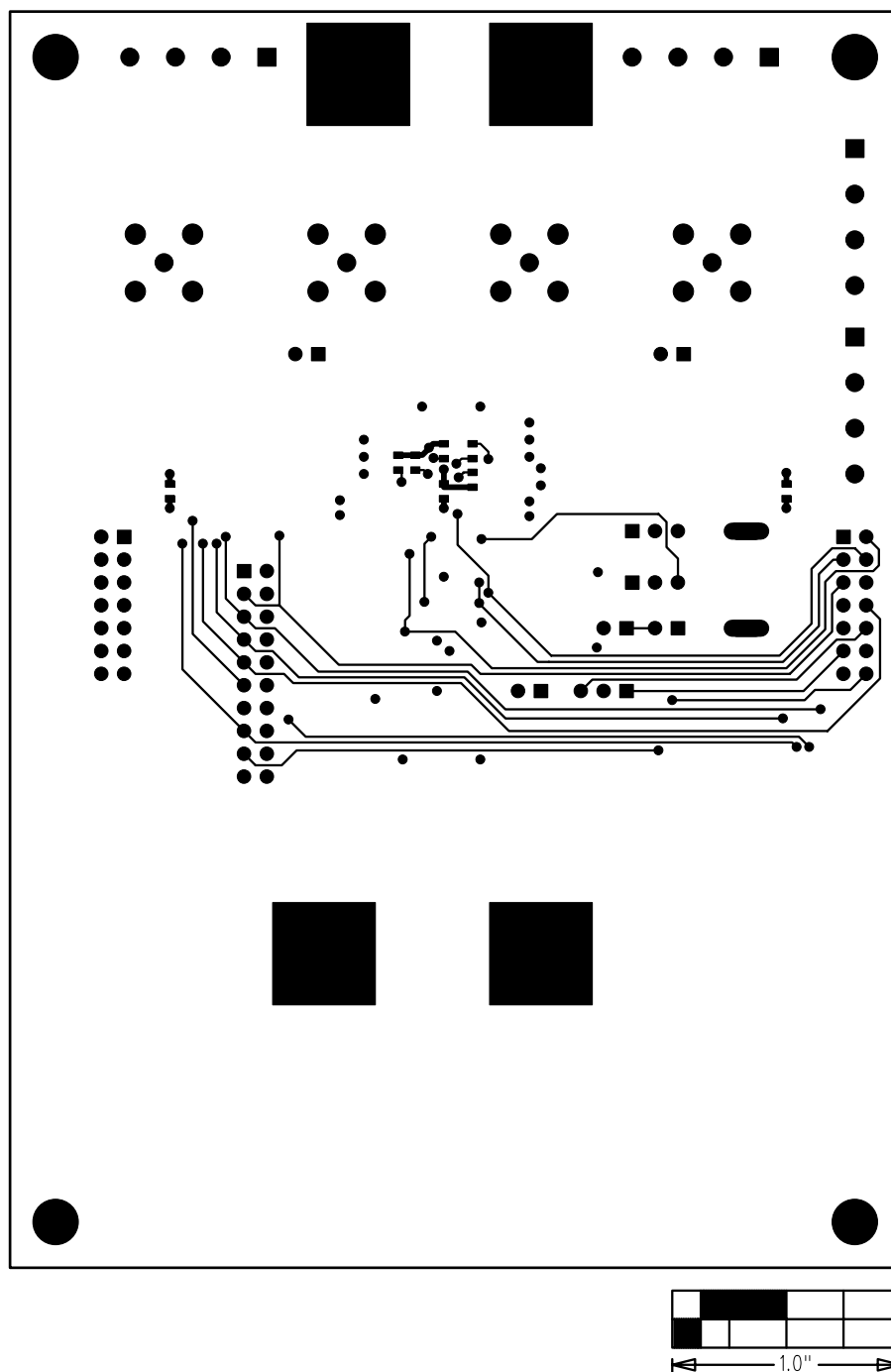
Figure 16. MAX11040K Daughterboard PCB Layout—Bottom
