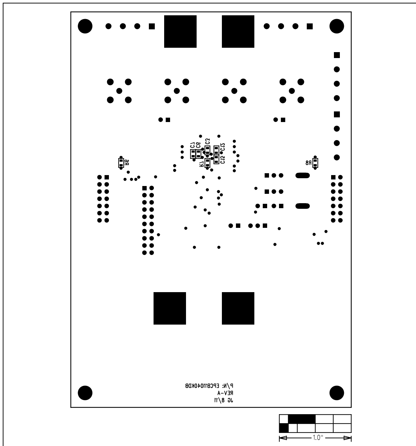
Figure 17. MAX11040K Daughterboard Component Placement Guide—Bottom
