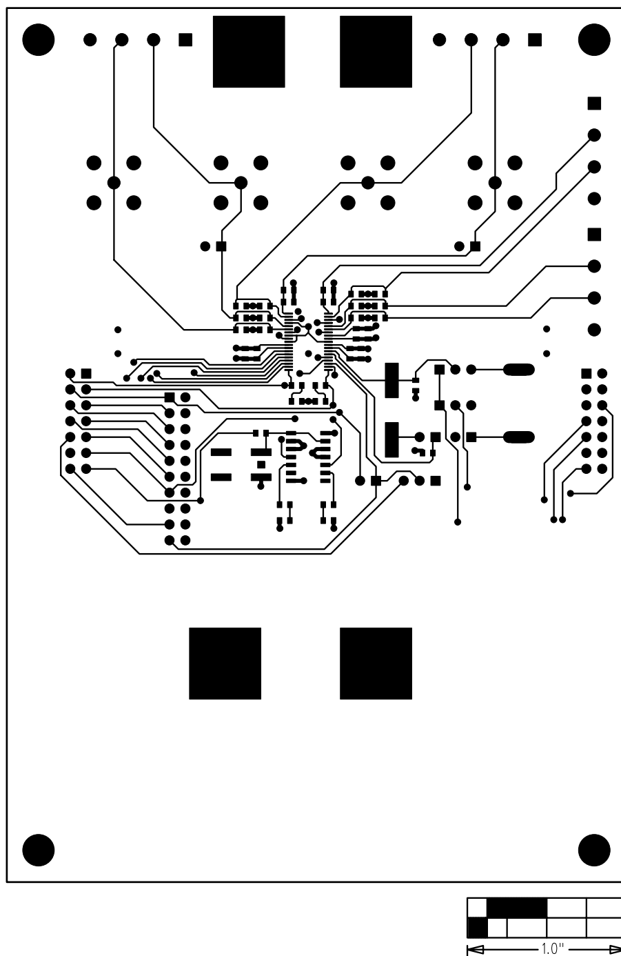
Figure 13. MAX11040K Daughterboard PCB Layout—Component Side
