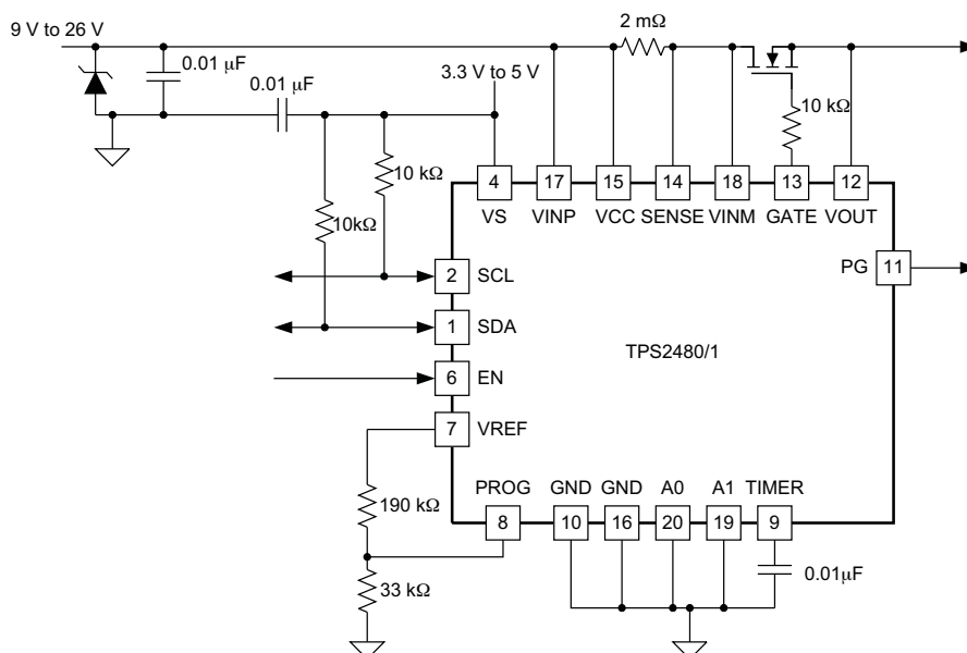
Simplified Application Diagram
