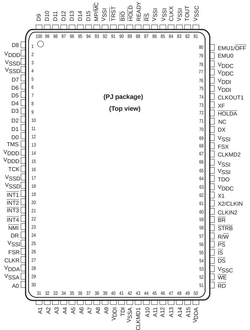
Figure A–1. Pin/Signal Assignments for the 'C52 in 100-Pin QFP
