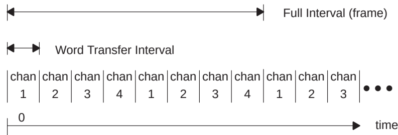
Figure 9–41. Time-Division Multiplexing
