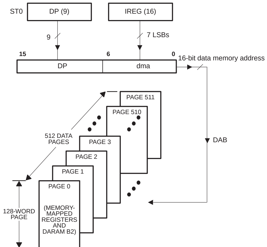
Figure 5–1. Direct Addressing
