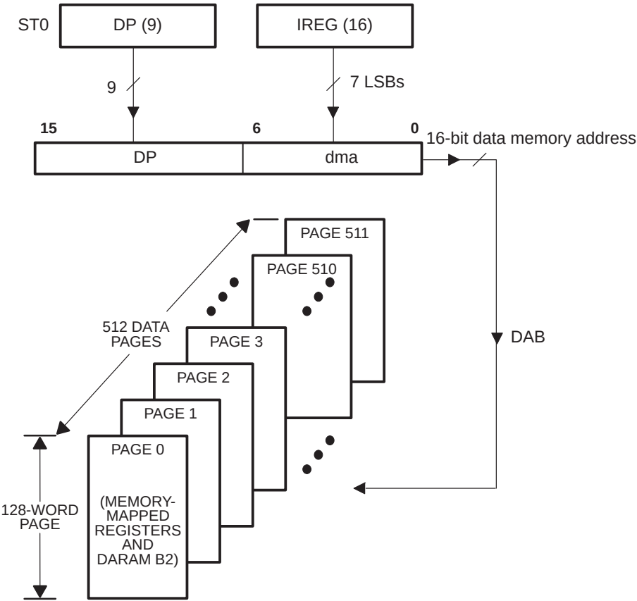
Figure 5-1. Direct Addressing
