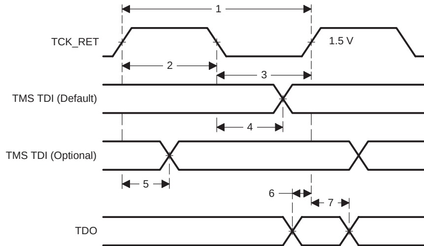
Figure D–3. Emulator Cable Pod Timings
