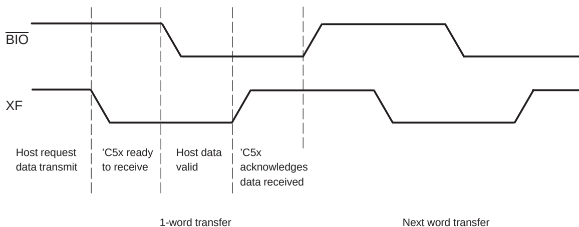
Figure 8–12. Handshake Protocol
