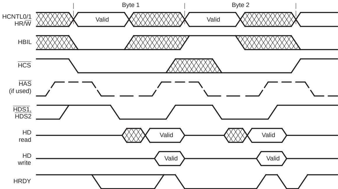
Figure 9–52. HPI Timing Diagram
