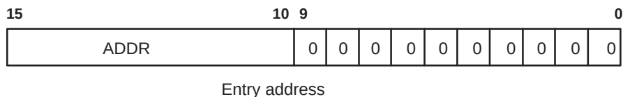
Figure 8–13. 16-Bit Entry Address for Warm Boot Mode
