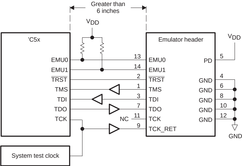
Figure D-4. Target-System Generated Test Clock
