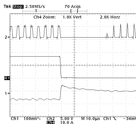
Figure 13. Load Transient Response Details
