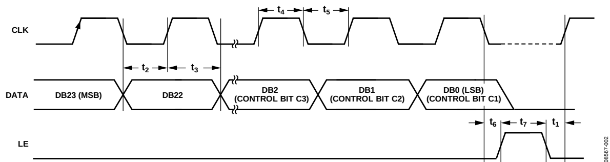
Figure 2. Timing Diagram
