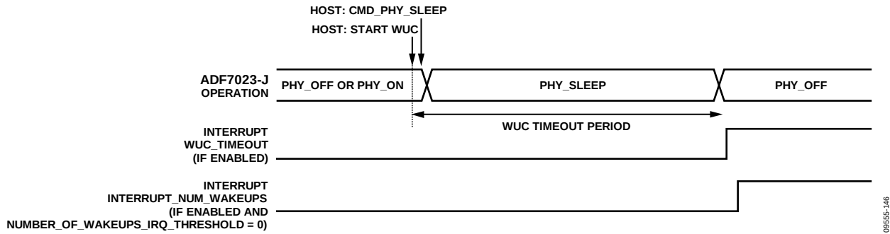
Figure 70. Low Power Mode Timing When Using the WUC
