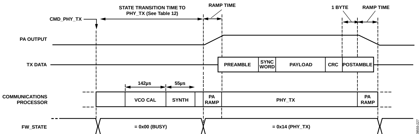
Figure 56. Transmit Packet Timing
