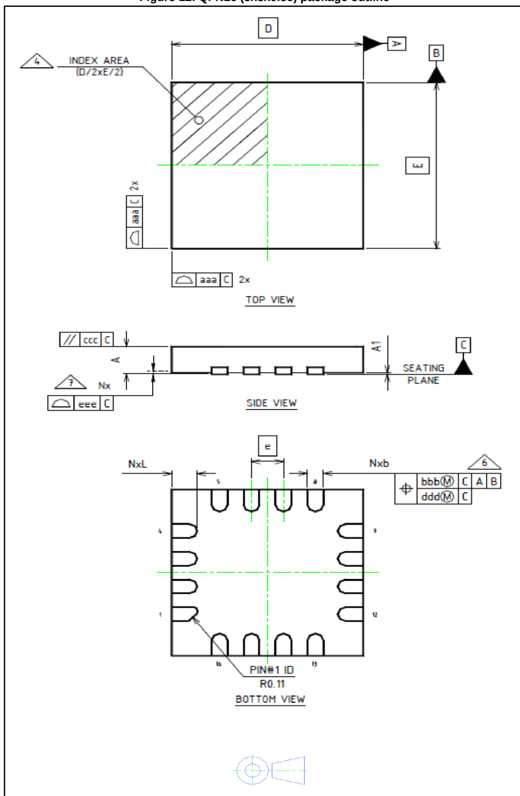
Figure 12: QFN16 (3x3x0.55) package outline
