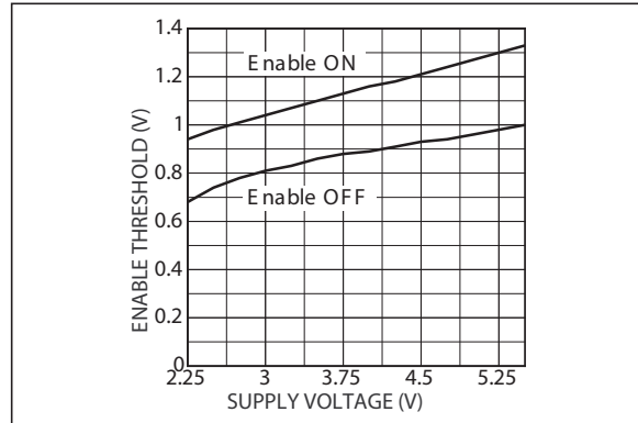
FIGURE 2-10: Enable Threshold vs. Supply Voltage for LDO 1.
