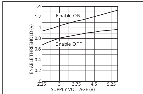
FIGURE 2-12: Enable Threshold vs. Supply Voltage for LDO 3.
