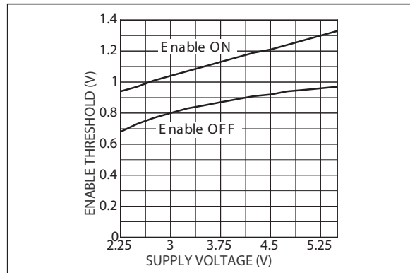
FIGURE 2-11: Enable Threshold vs. Supply Voltage for LDO 2.
