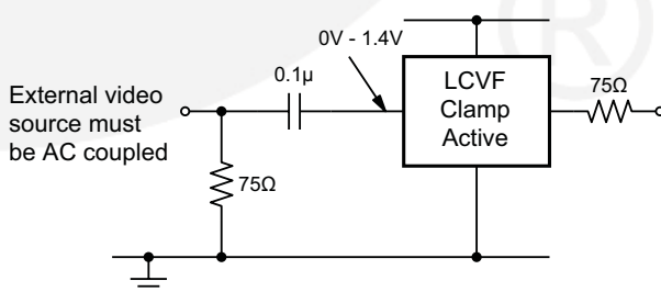
Figure 11. SCART with DC-Coupled Outputs
