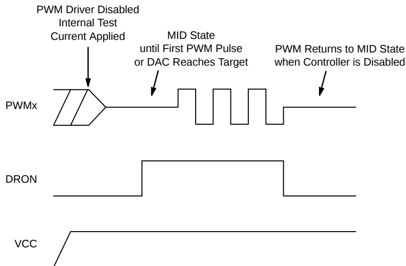
Figure 22. Soft Start
