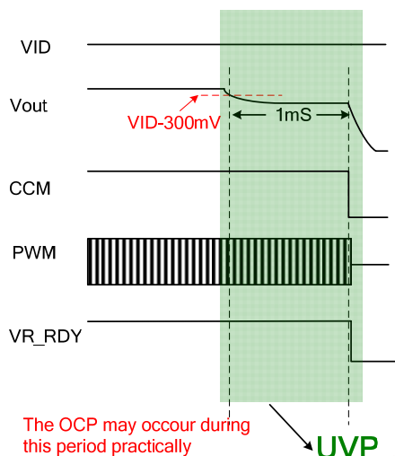
Figure 9: Under-Voltage Protection
