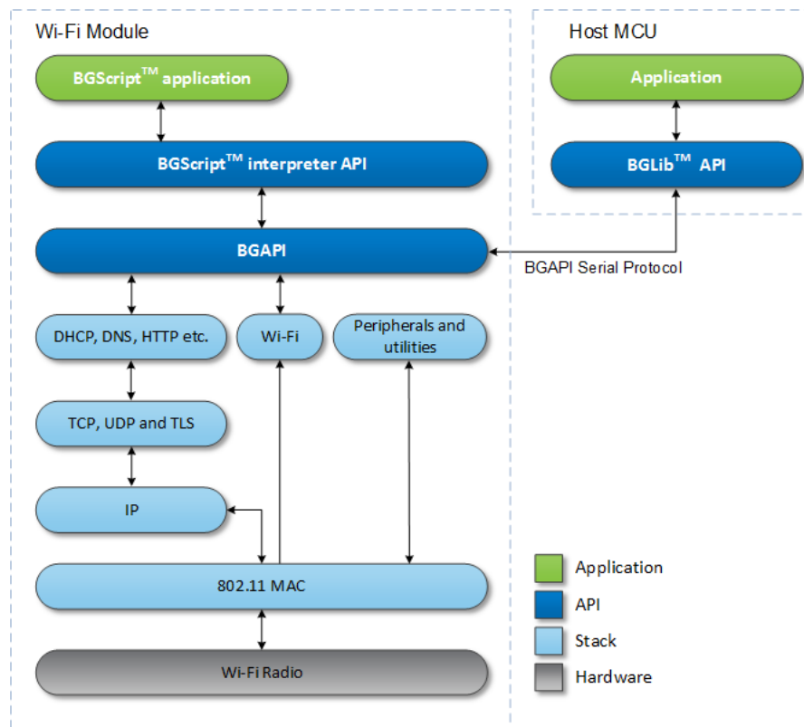
Figure 1.1. Wizard Gecko Software Architecture
