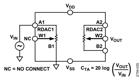
Figure 34. Analog Crosstalk
